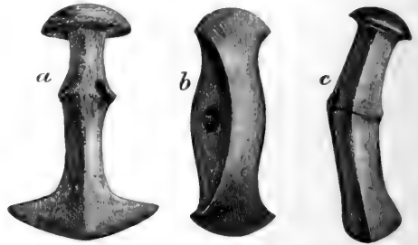
Fig. 3.—War-axes of Stone used in the Bronze Age: a , Danish, 7 inches; b , English, 5 inches; c , Swedish, 24 inches long.
