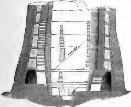
Fig. 19.—Section of Mousa, shewing Structure of a Broch, 45 feet high.
