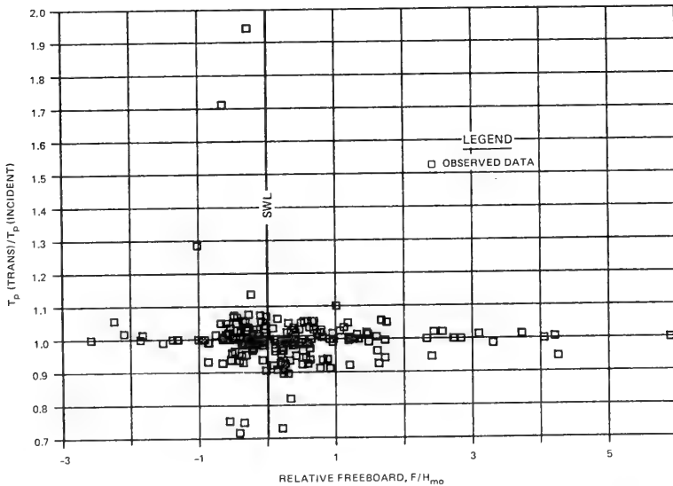
Figure 24. Ratio of the transmitted period of peak energy density to the incident period of peak energy density as a function of the relative freeboard, all subsets
