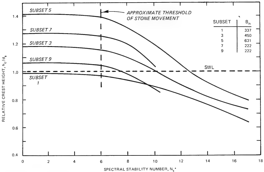
Figure 9. Damage trends of the relative crest height as a function of the spectral stability number for the stability subsets 1, 3, 5, 7, and 9
