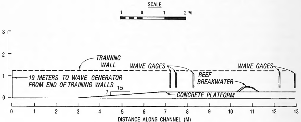
Figure 2. Cross section of test channel
