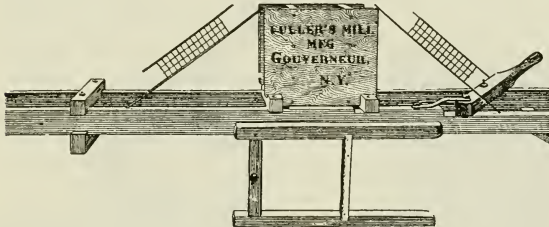
Fuller Hand-Power Curd Mill.
