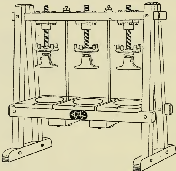
Upright Press.
