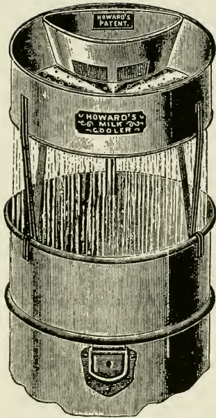
Howard's Aerator.
