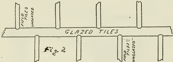
PLAN FOR A SEPTIC TANK.
