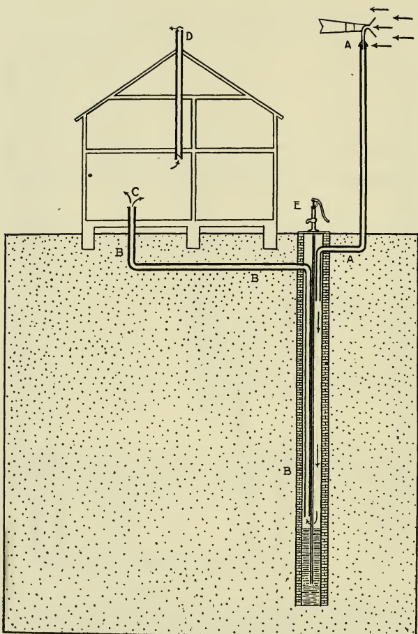
Plate showing vertical section of Mr. J. F. Steinwahn's factory and sub-earth duct in well at Colby, Wis. A, A, funnel taking air into well; B, B, B, duct leading air from well to curing room, C; D, ventilator.
