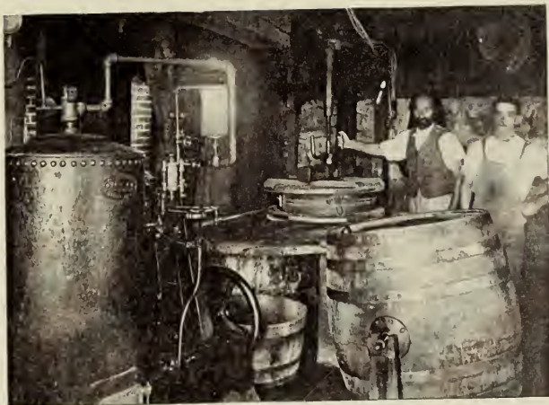
Interior of a Swiss factory, showing a cheese in the press and the means of adjusting the pressure. The small engine and churn are for making whey butter.
