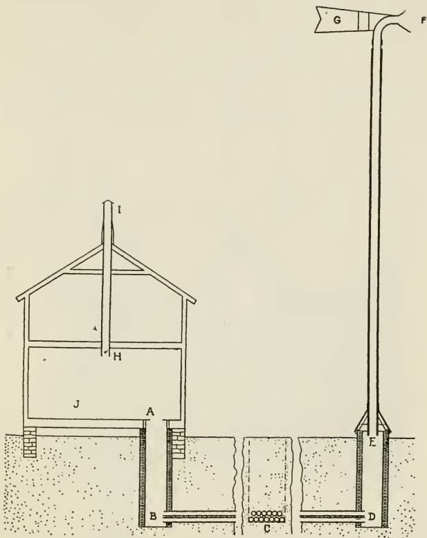
Plate showing section of cheese curing room and horizontal multiple sub-earth duct. A, inlet to curing room; B, end of sub-earth duct in bricked entrance to factory; C, cross-section of the multiple ducts as placed in the factory of A. C. Werth, Neenah, Wis. D, E, bricked entrance under funnel at outer end of sub-earth duct; F, funnel with mouth 36 inches across; G, vane to hold funnel to the wind.
