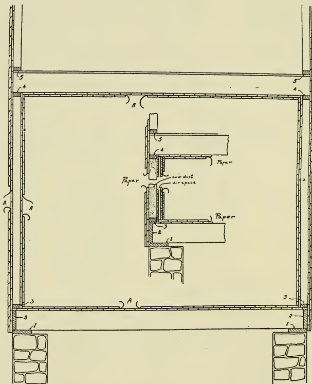
Plate showing the construction of wood curing room. 1, 1, 1, sill; 2, 2, 2, a two-by-ten spiked to ends of joist; 3, 3, 3, a two-by-four spiked down after first layer of floor is laid to toe-nail studs to; 4, 4, 4, a two-by-four spiked to upper ends of studding of first story; A, A, A, A, three-ply acid and waterproof paper. The drawing in the center shows space between studding filled with sawdust and another dead-air space to be used when the best ducts cannot be provided.
