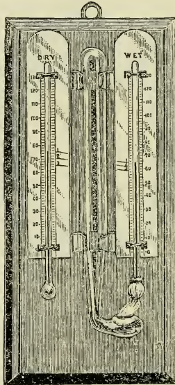
Psychrometer.
