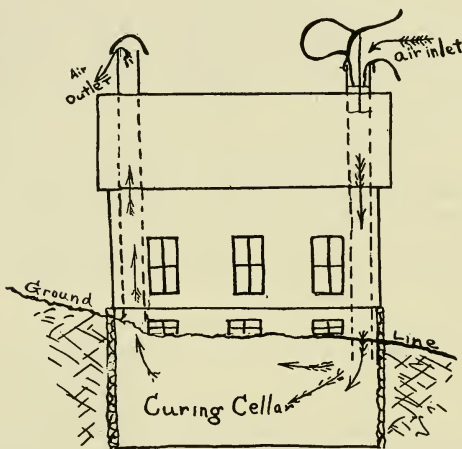
Ventilation of a cellar curing room by means of a cowl and ventilator shaft.
