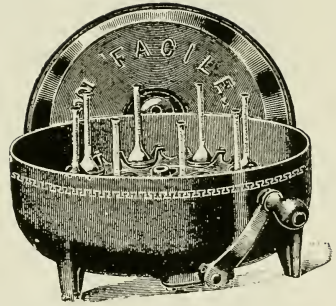
Hand-power Centrifuge, uncovered, showing position of bottles in pockets.
