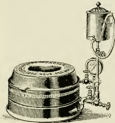
Steam Turbine Test, with steam gauge and hot water attachment.
