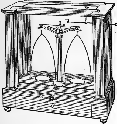
FIG. 26.—Analytical balance.
