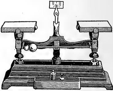
FIG. 20.—Type of knife-edge cream balance.
