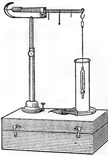
FIG. 27.—Westphal balance.
