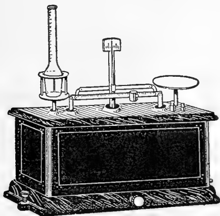
FIG. 18.—Type of torsion balance for single bottle.
