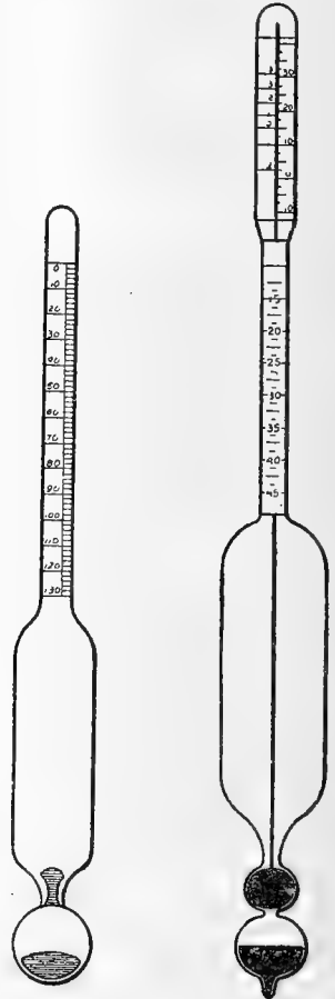
FIG. 28.—Types of ordinary lactometers.
