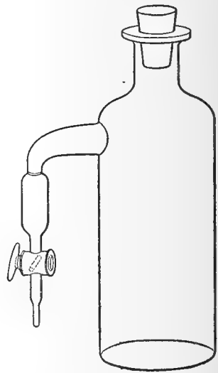
FIG. 6.—A combined bottle and acid measure.
