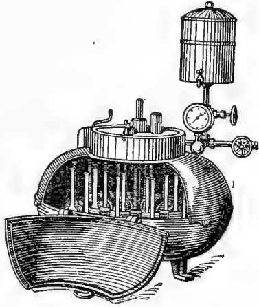
FIG. 10.—A type of steam tester with an arrangement for heating the water used in the test.
