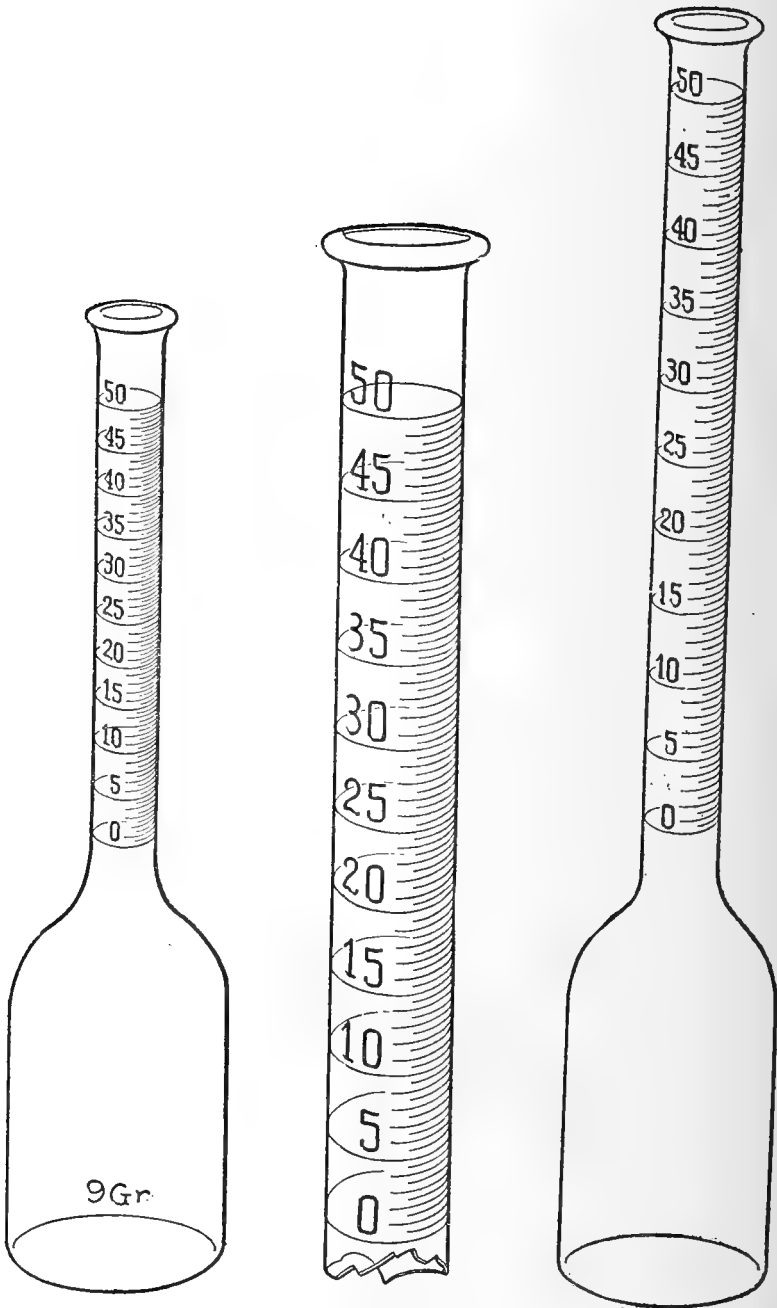
FIG. 16.—Types of 9-gram and 18-gram cream bottles conforming to the requirements of the United States Bureau of Standards.
