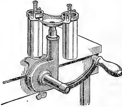
FIG. 8.—A 2-bottle hand tester.
