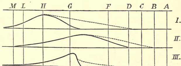
FIG. 6.—SPECTRUM PHOTOGRAPHED ON THE SILVER HALOIDS.
