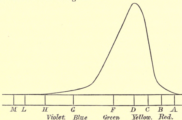
FIG. 5.—VISUAL INTENSITY OF COLOURS OF SOLAR SPECTRUM.
