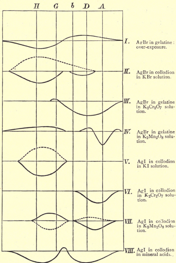
FIG. 9.—REVERSALS IN SPECTRUM IN PRESENCE OF REVERSING AGENTS.
