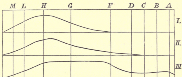
FIG. 11.—SPECTRA PHOTOGRAPHED ON DIFFERENT FORMS OF SILVER CHLORIDE (I. and II.) AND ON THE RED-SENSITIVE FORM OF SILVER BROMIDE (III.).
