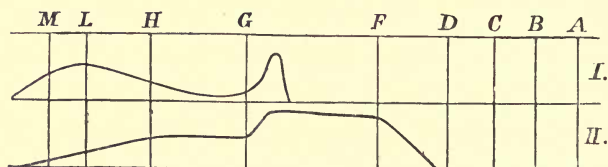
FIG. 8.—ORDINARY REVERSAL IN SPECTRUM. I. Pure AgI + AgNO 3 ; II. 3AgI + AgBr + AgNO 3 .
