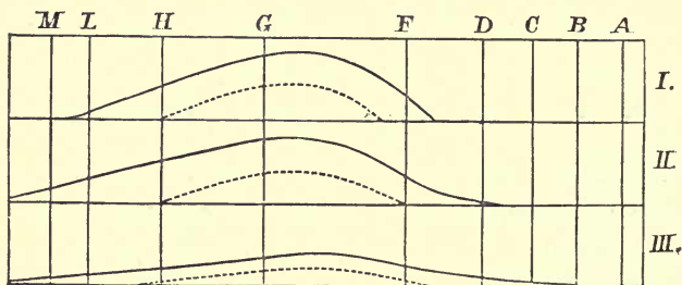
FIG. 10. — SPECTRA PHOTOGRAPHED ON DIFFERENT FORMS OF SILVER BROMIDE
