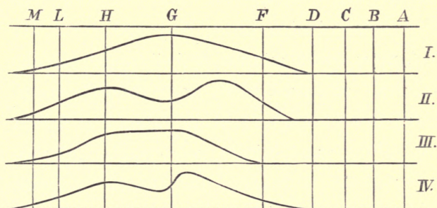
FIG. 7.—CONCURRENT REVERSALS IN MIXTURES OF SILVER HALOIDS.
