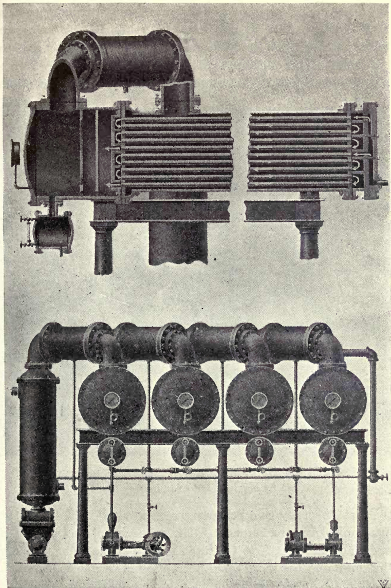
FIG. 17. YARYAN EVAPORATOR Courtesy of Mr. Chas. Ordway
