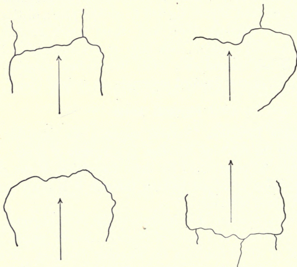
FIG. 43. LINES OF RUPTURE IN MULLEN TEST
