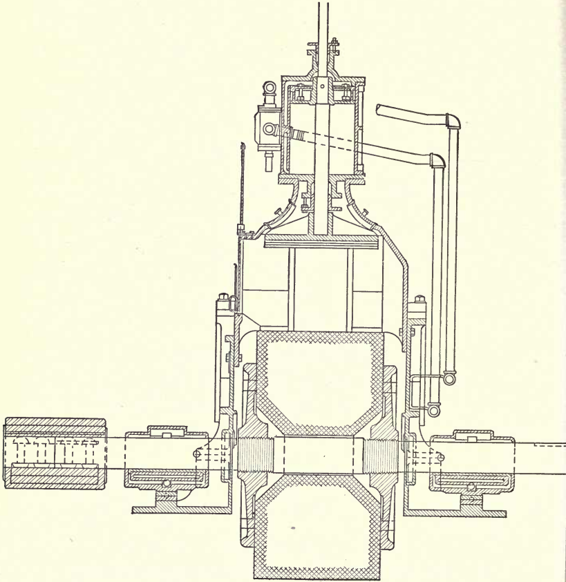
FIG. 32. THREE-POCKET GRINDER SECTIONAL ELEVATION
