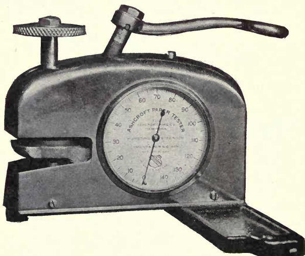
FIG. 53. ASHCROFT TESTER
