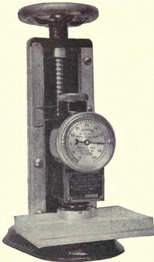
FIG. 48. PRESSURE BULKER
