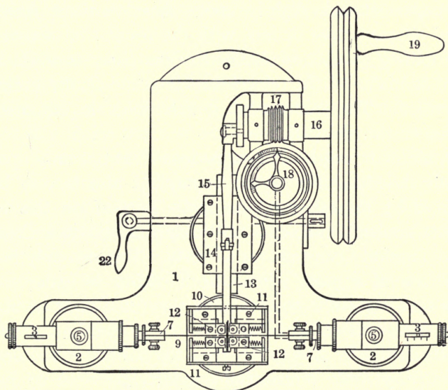
FIG. 54. SCHOPPER FOLDING MACHINE
