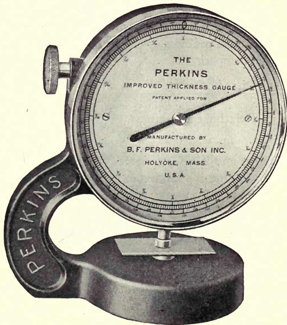
FIG. 47. THICKNESS GAUGE
