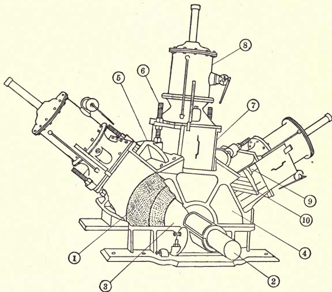
FIG. 31. THREE-POCKET GRINDER
