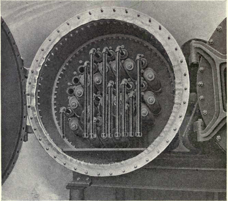
FIG. 18. YARYAN EVAPORATOR FEED END OF ONE EFFECT Courtesy of Mr. Chas. Ordway
