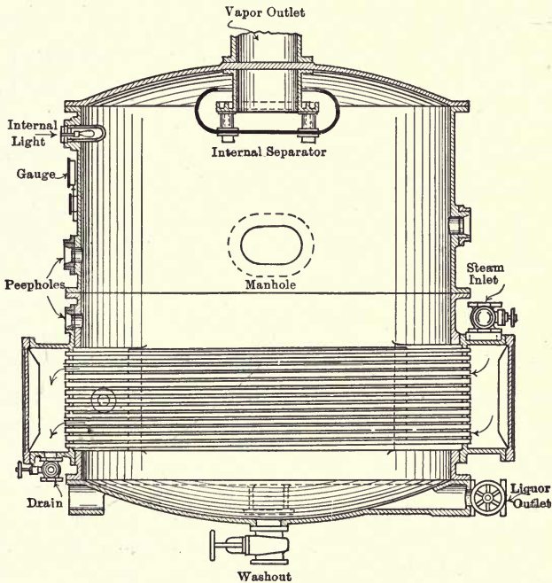
FIG. 19. ZAREMBO EVAPORATOR VERTICAL CROSS SECTION OF ONE EFFECT Courtesy of Zarembo Company
