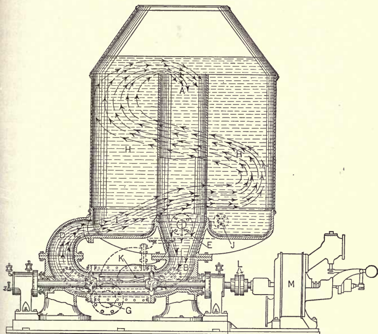
FIG. 6. WINESTOCK DEFIBERING MACHINE
