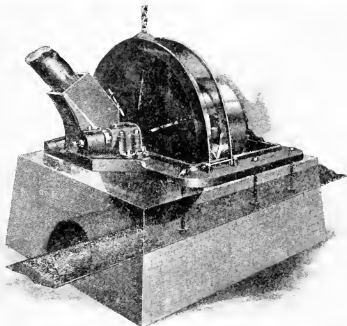
FIG. 21. PULP WOOD CHIPPER
