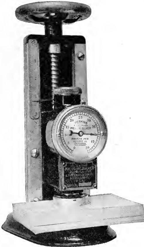
FIG. 48. PRESSURE BULKER
