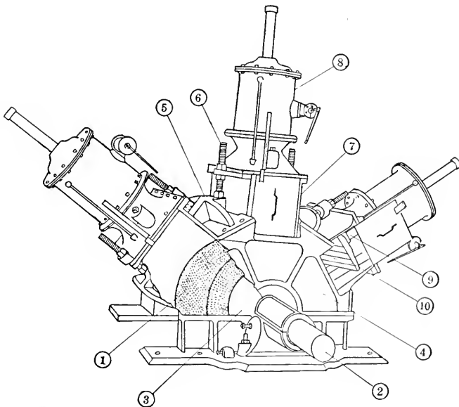
FIG. 31. THREE-POCKET GRINDER
