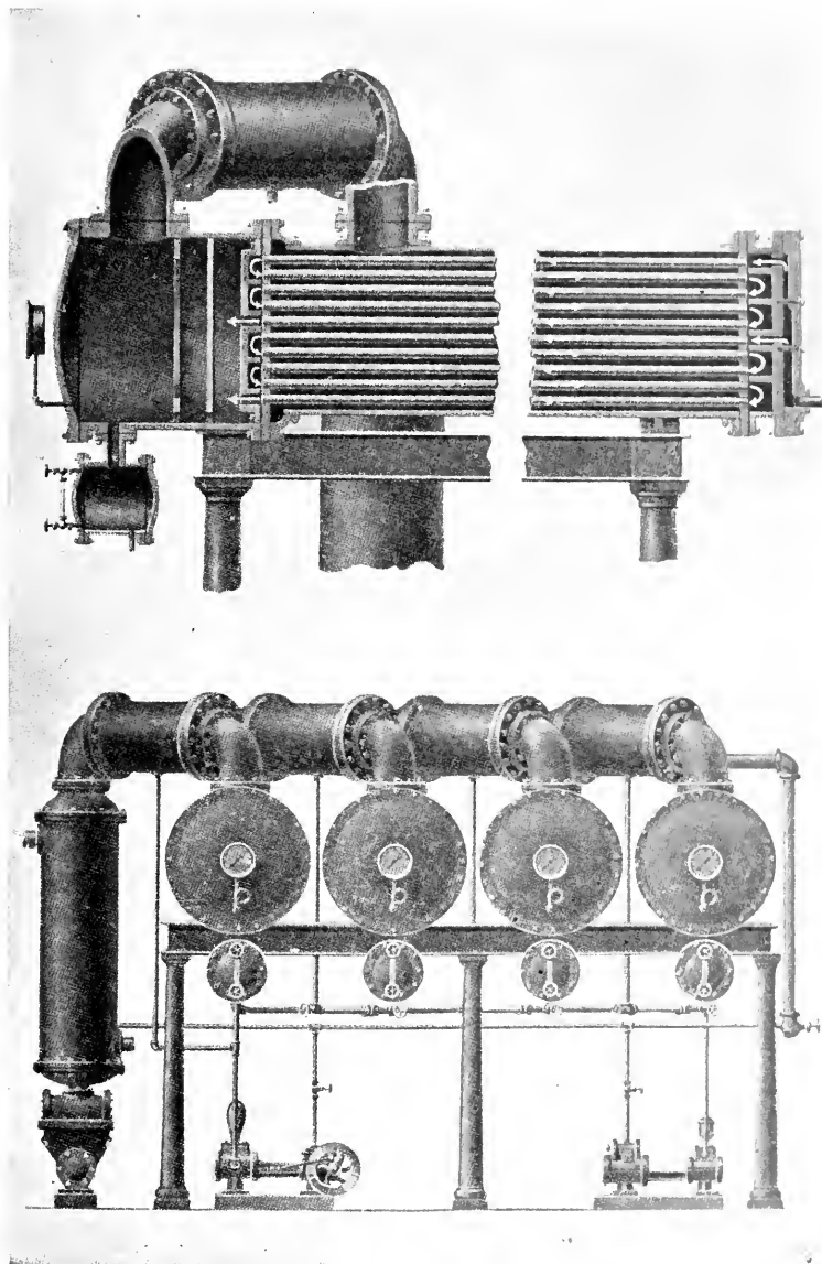
FIG. 17. VARYAN EVAPORATOR Courtesy of Mr. Chas. Ordway
