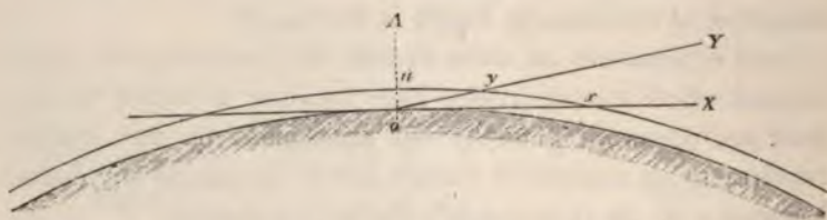
FIG. 17.—Diagram showing the increasing thickness of air through which the light of the sun has to pass as it descends towards the horizon. When the sun is in the zenith, A , its light will have to pass through a thickness of atmosphere represented by a o . When near the horizon, this distance will be increased to y o , and when actually on the horizon to x o .
