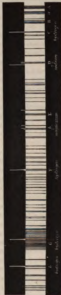
FIG. 44.—Spectrum of the sun's photosphere (below) and chromosphere (above), showing the lines ordinarily visible, and that they extend to different heights.
