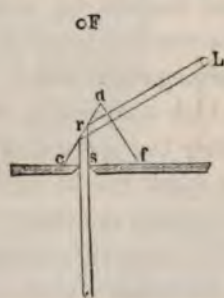
FIG. 31.—Path of light through comparison prism. a , f , c , prism; L , light-source; r , point of reflection; s , slit; F , light-source in front of slit.
