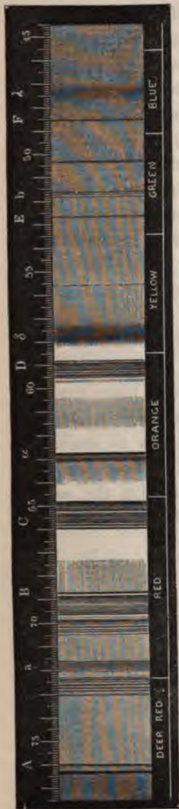
FIG. 26.—The Telluric Lines. Taken from the Atlas to Angström's Spectre Normal . The observations shown extend over the whole of the visible spectrum. The red part of the spectrum is to the left.
