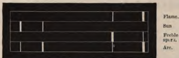
FIG. 77.—Showing the various intensities of the lines of Lithium under different conditions.
