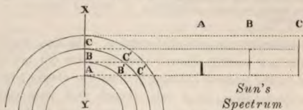
FIG. 68.—Spectral phenomena on the assumption of three layers. c , outermost layer, being represented at c' , will give us a long line as at c , as it would do if the stratum extended from c to a along the line x-y , and so with b .
