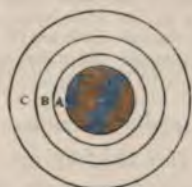
FIG. 66.—The sun and its atmosphere on Kirchhoff's hypothesis. A, luminous haze resting on liquid photosphere ; B, locus of absorption ; C, outer atmosphere.
