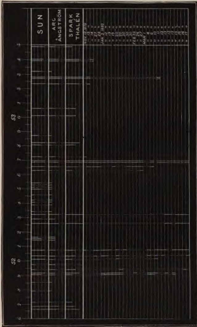
FIG. 110.—Portion of a large map, showing how the iron lines most affected in sun-spots are recorded. Region b—D. The dates of observation are given at the side. The full lines show the lines widened in each spot day.
