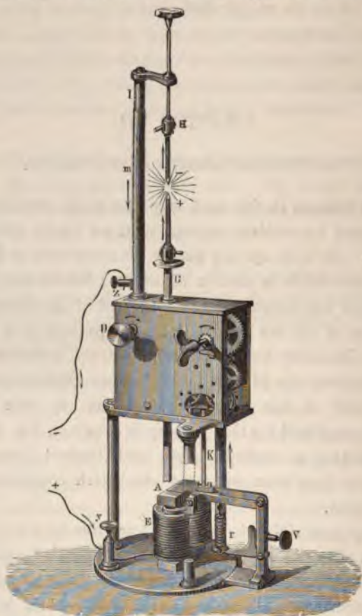
FIG. 33.—Electric lamp. y, z , wires connecting battery of fifty Grove or Bunsen elements; g, h , carbon holders; κ , rod which stops a clockwork movement which, when going, makes the poles approach until the current passes; A , armature of a magnet, which by means of κ frees the clockwork when not in contact; E , electro-magnet, around which the current passes when the poles are at a proper distance apart, causing it to attract the armature A .
