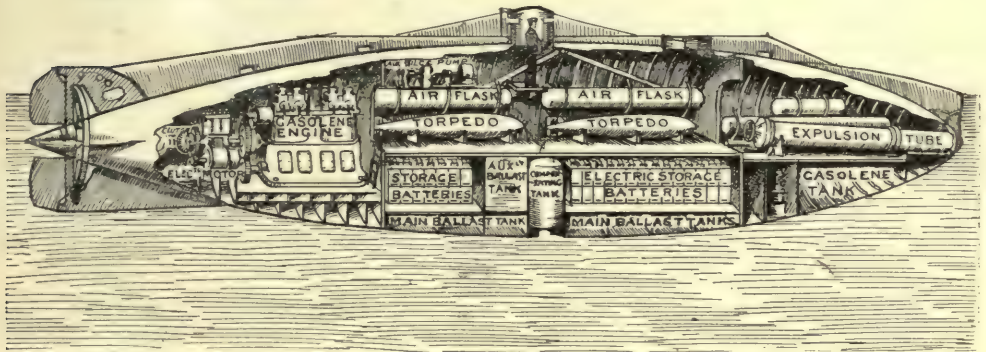
Section of a Submarine.
