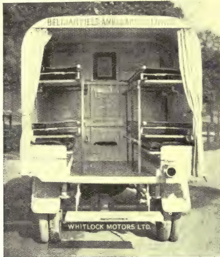
The "Prince George" Motor Ambulance. Interior arranged for four Stretcher Cases.
