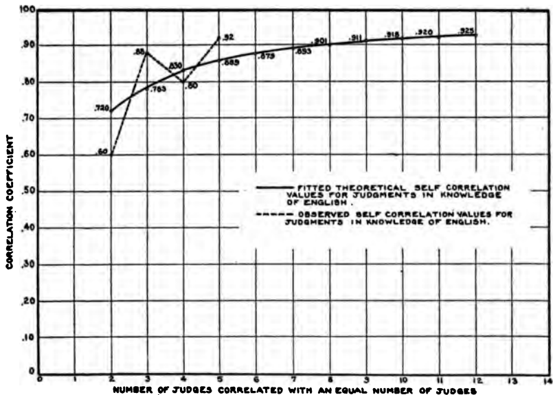
FIG. 3. Curves Showing the Fitted Theoretical and Observed Self-correlation Value for Judgments in Knowledge of English.
