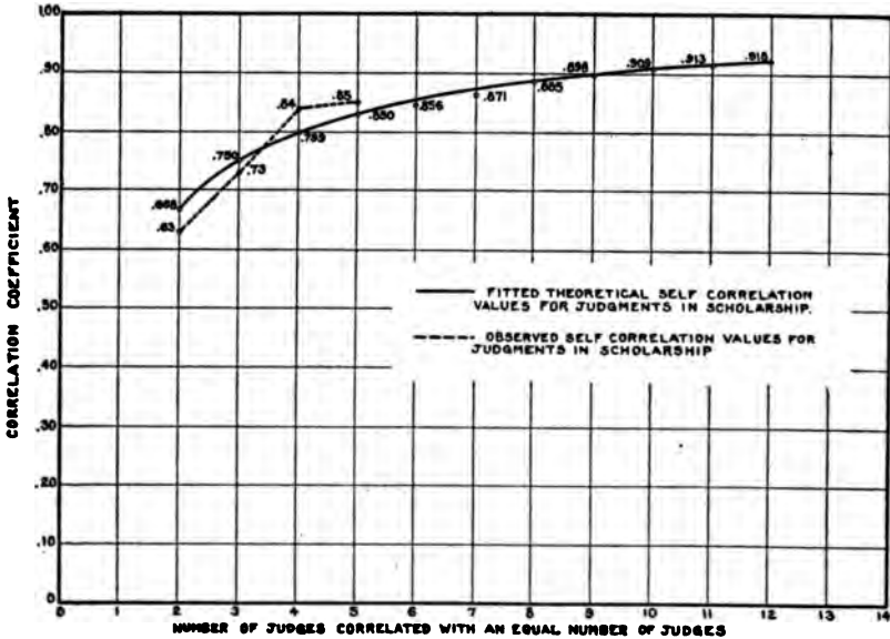
FIG. 1. Curves Showing the Fitted Theoretical and Observed Self-correlation Values for Judgments in Scholarship.
