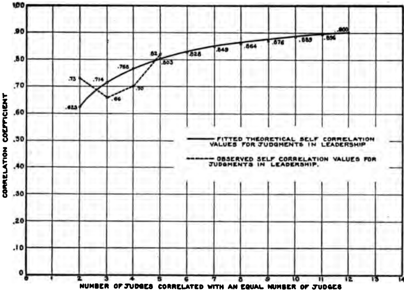
FIG. 2. Curves Showing the Fitted Theoretical and Observed Self-correlation Values for Judgments in Leadership.
