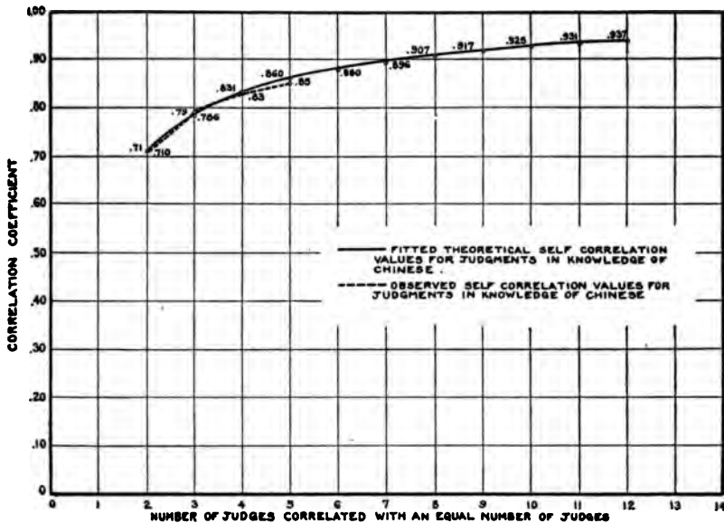
FIG. 4. Curves Showing the Fitted Theoretical and Observed Self-correlation Values for Judgments in Knowledge of Chinese.
