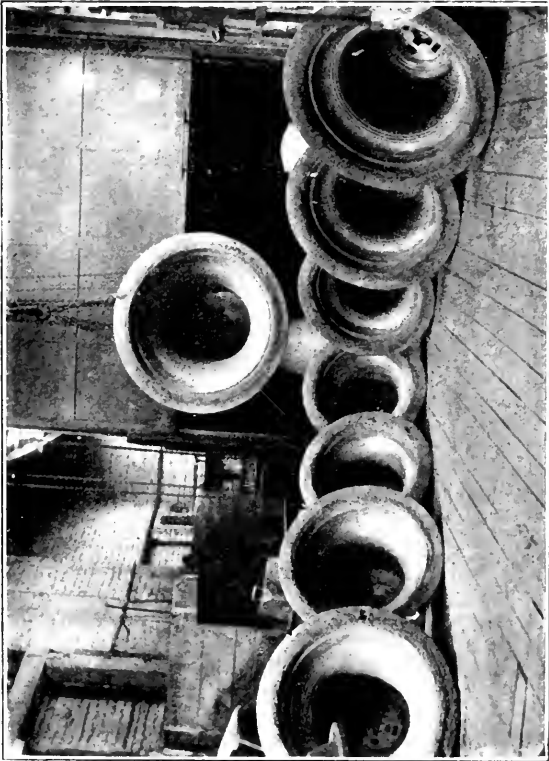
OUTER MOULDS OR COPES FOR CASTING A RING OF EIGHT BELLS. (See page 14.)
