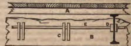
A. Joist. B. Plaster. C. Bars hooked to bolt. D. Nut. E. Round iron.
