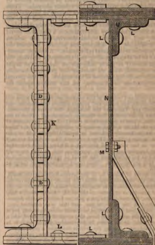
HALF SECTION, showing mode of attaching Stirrup Irons.
