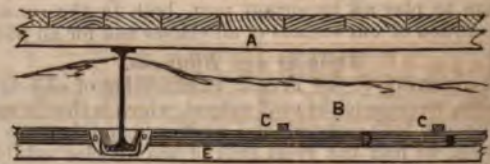
A. Joist. B. Plaster. C. Square iron. D. Flat iron bar. E. Plaster ceiling. SECTION ALONG GIRDERS.
