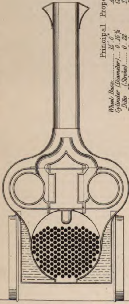
Transverse Section
