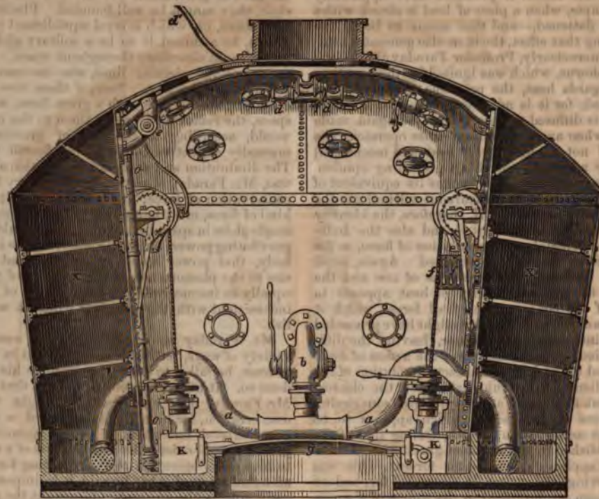
SECTIONAL VIEW OF THE NAUTILUS MACHINE.
