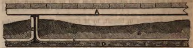
A. Wooden joist. B. Plaster. C. Iron rod. D. Plaster ceiling. E. End of rod. they are filled in; this, as will be seen at once, is the most simple of these methods, but it is deficient in the ties with which the others are strengthened.
