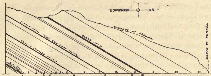
SECTION OF STRATA ON LINE OF CLAYTON TUNNEL.
