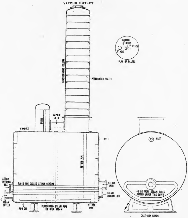
FIG. 51.—Diagram illustrating a Type of Steam-heated Blow-over Still with Fractionating Column.
