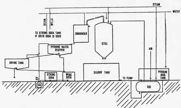
FIG. 55.—Diagrammatic Illustration of one method of arranging a Recovery Plant for Crude Pyridine.
