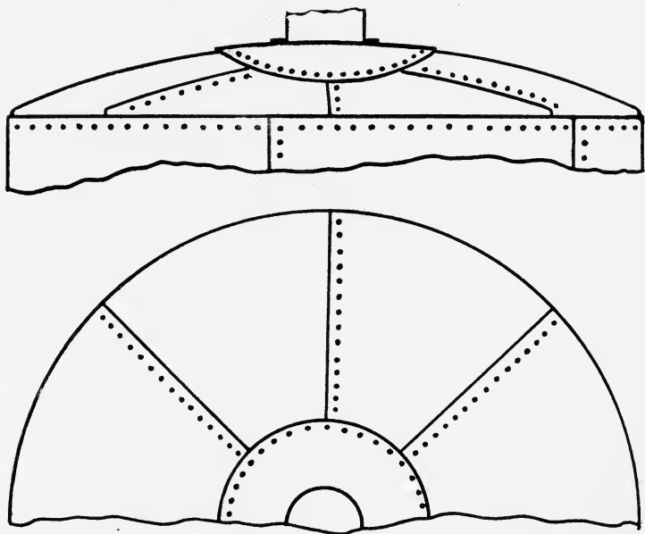
FIG. 3.—Diagram showing a Method of Arranging Sketch Plates on Still Dome.
