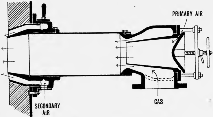
FIG. 27.—Mixing Tube of Terbeck Gas-fired Furnace.
