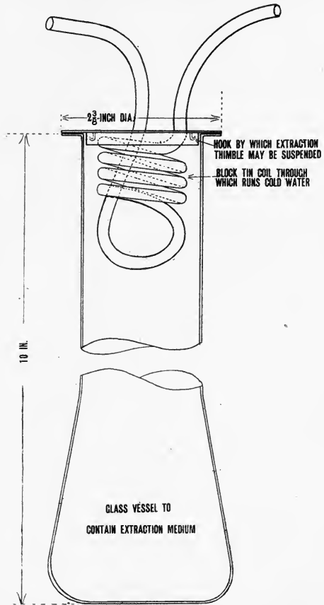
FIG. 62.—Apparatus adopted by Church for the Determination of "Free Carbon" in Tar.
