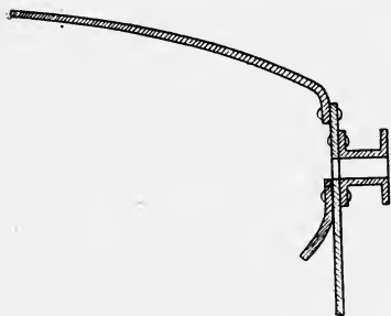
FIG. 14.—Diagram showing Method of Fitting a Protection Plate under Charge Block.
