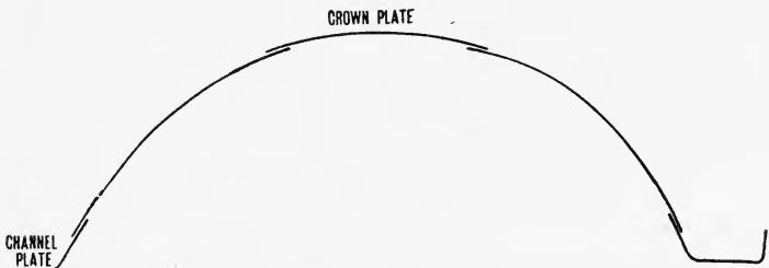
FIG. 5.—A Method of Arranging Plates for Still Bottom (Diagrammatic).
