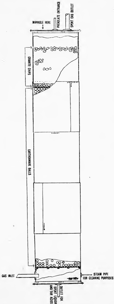
FIG. 40.—A Cylindrical Carbonating Tower, Packed Type. F
