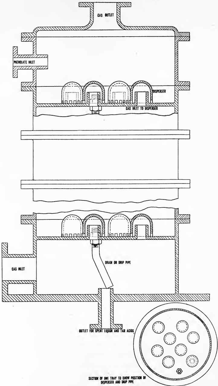
FIG. 38.—Carbonating or Reaction Tower—Plate Type.
