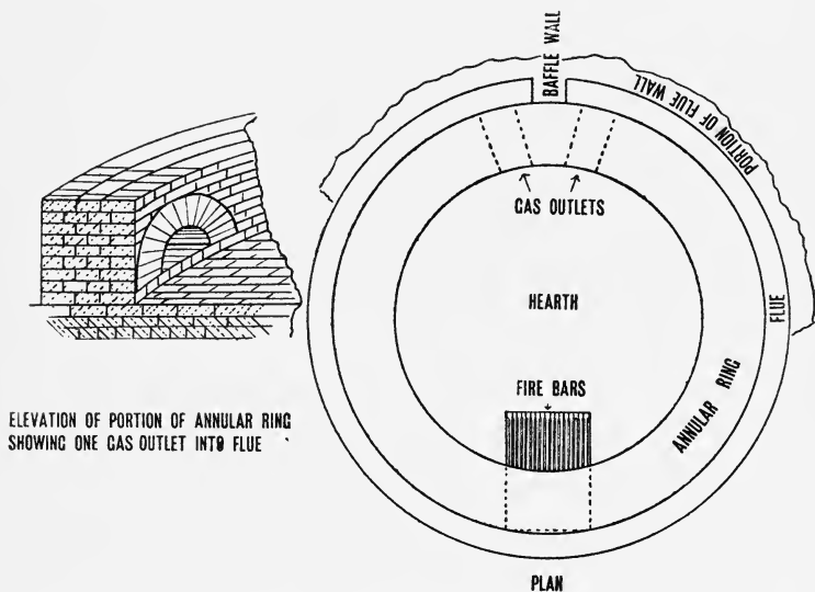
FIG. 21.—Annular Ring (Still Seat) Outlets to Flues.
