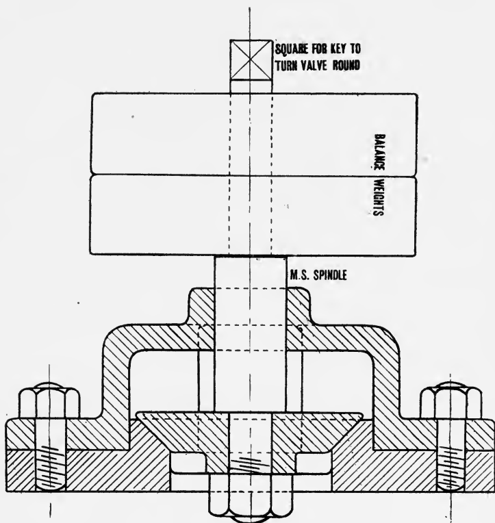
FIG. 9.—A type of Tar Still Safety Valve.
