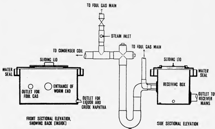
FIG. 30.—Receiving Box and Connexions.
