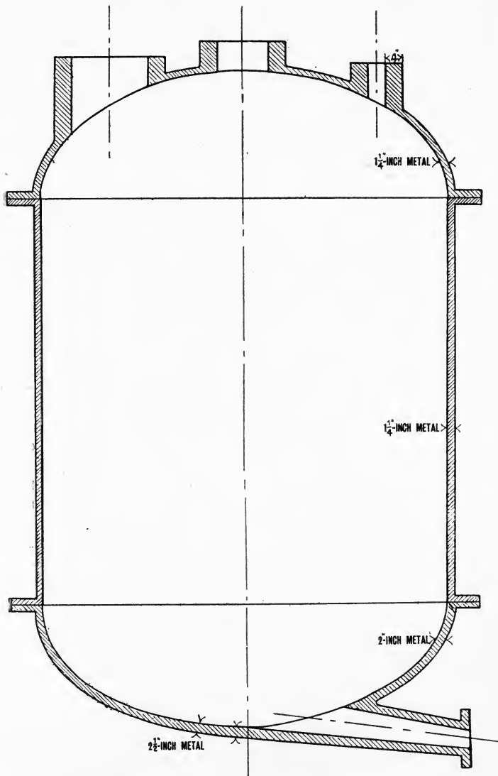
FIG. 2.—Diagram of Cast-iron Tar Still (not to be recommended).
