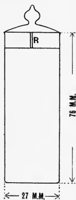
FIG. 61.—Specific Gravity Bottle for Tar Testing.
