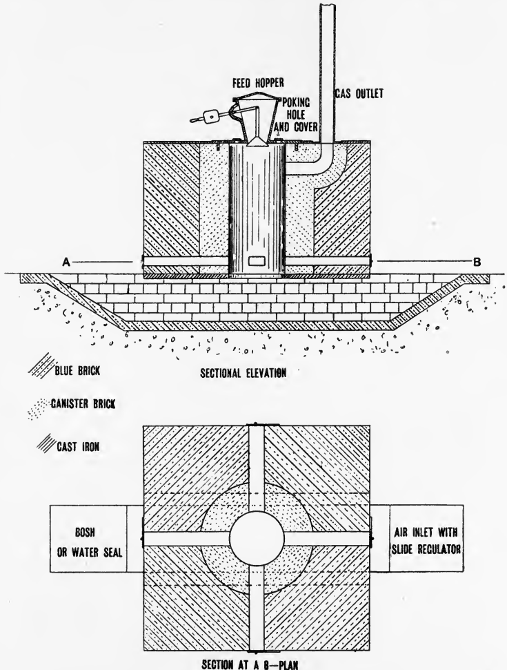
FIG. 44.—One Type of Furnace for Generation of CO 2 .
