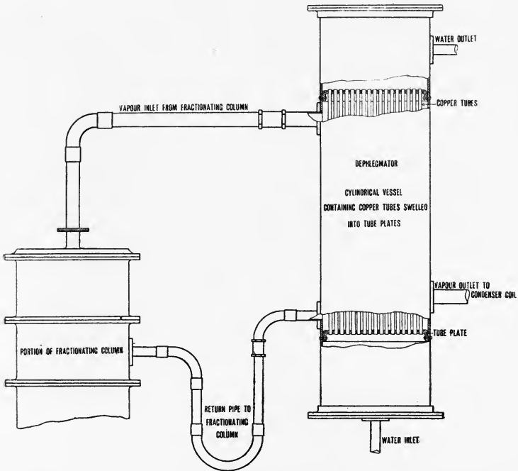
FIG. 53.—Diagram showing a Type of Dephlegmator and a Method of Connecting to the Fractionating Column.
