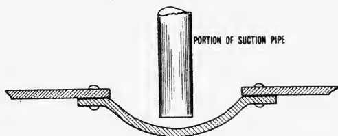
FIG. 35.—Dish Plate at Bottom of Receiver.
