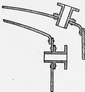
FIG. 15.—Diagram showing Methods of Fitting Charge Blocks to Still.
