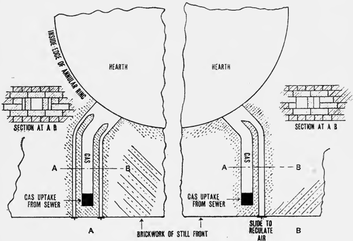
FIG. 26.—Diagrams A and B, showing, in Plan, two Methods of Building a Producer Gas Burner of Brick.
