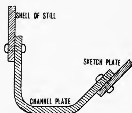
FIG. 8.—Another Method of Joining Bottom of Still to Shell.
