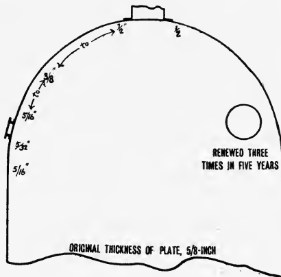
FIG. 4.—Diagrammatic Illustration showing Extent of Corrosion which can take place on a High-pitched Dome.
