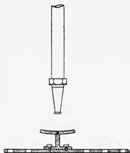
FIG. 39.—Gurney's Jet arranged for Carbonating Tower.
