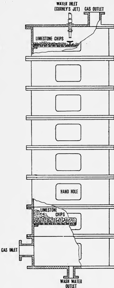
FIG. 47.—Diagram illustrating a Type of Purifying Tower without Dust Separator.
