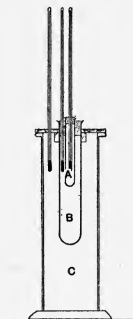
FIG. 64.—Apparatus used in Mann's method of estimating Naphthalene in Creosote.
