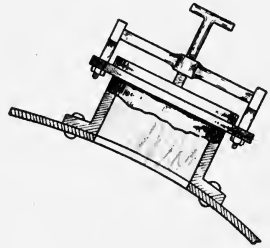
FIG. 16.—Manhole and Lid, Wrong Type.
