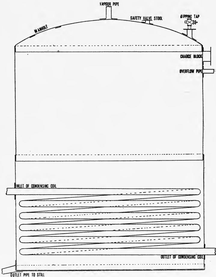
FIG. 28.—Preheater, Diagrammatic Figure.
