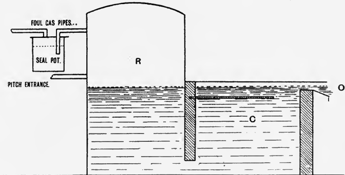
FIG. 36.—French Weir for Pitch Cooling.
