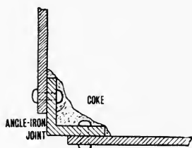
FIG. 7.—A Method of Joining Bottom of Still to Shell.
