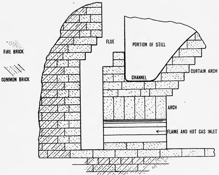
FIG. 23.—Diagram showing one Method of Protecting Bottom of Still Shell, also Channel Plate and Bottom.
