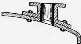
FIG. 10.—Safety Valve Stool.
