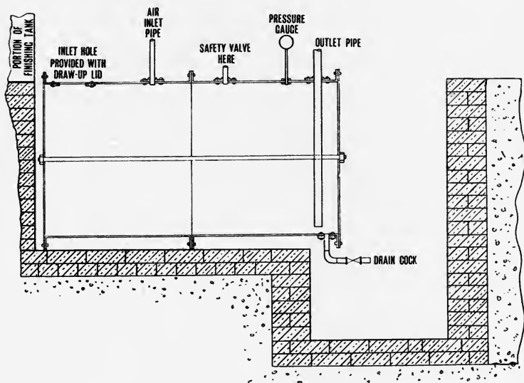
FIG. 43.—Egg for use on Carbolic Plant, etc.
