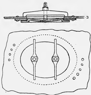
FIG. 17.—Draw-up Manlid, Correct Type.
