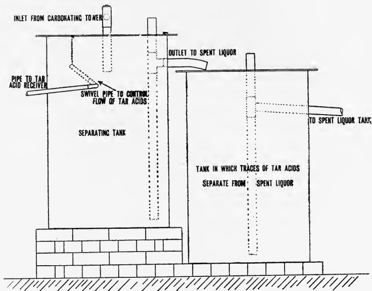
FIG. 41.—Divider Tanks, CO 2 Tar Acid Recovery Process.
