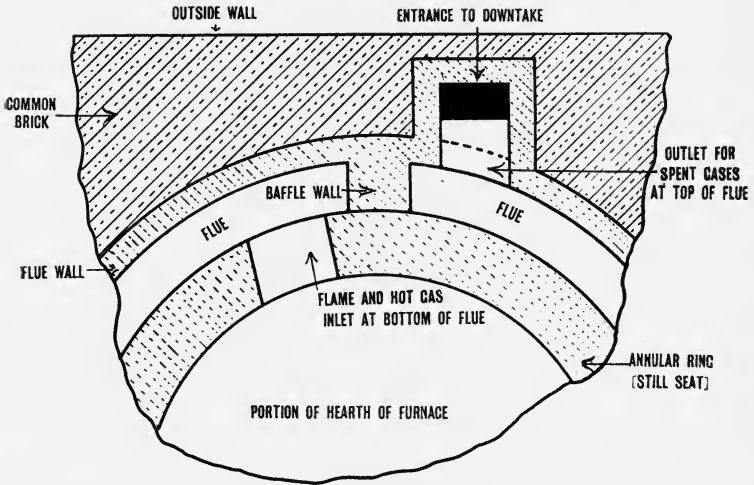
FIG. 22.—Diagrammatic Representation of Gas Inlet and Outlet in Single Wheel Flue (plan).
