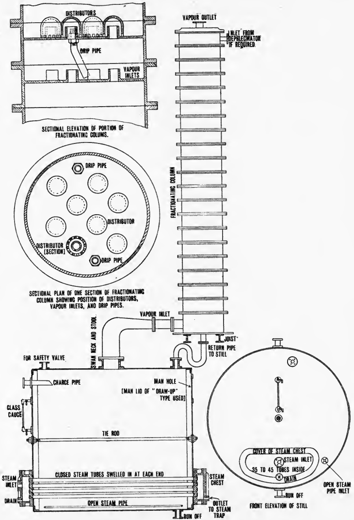
FIG. 52.—Fractionating Still and Column.
