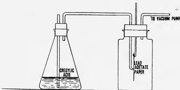
FIG. 65.—Apparatus used in Testing Cresylic Acid for Sulphur.
