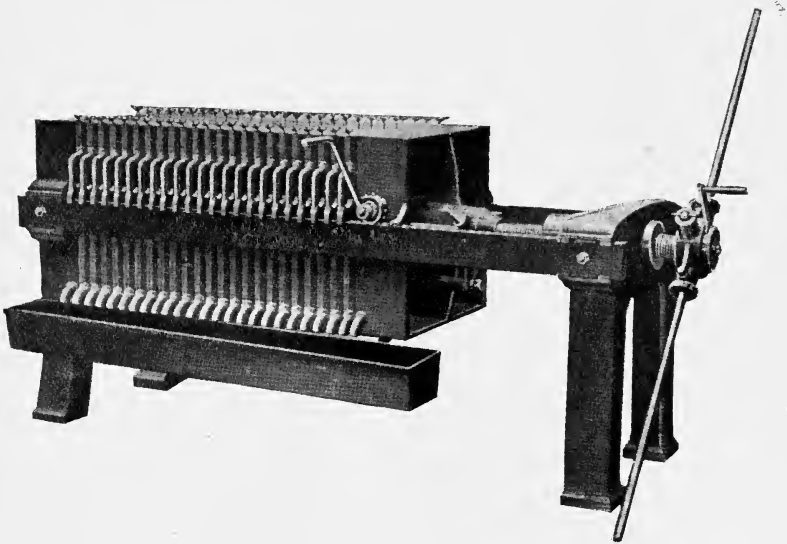
FIG. 59.—Filter Press.
