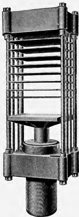
FIG. 57.—Hydraulic Press.
