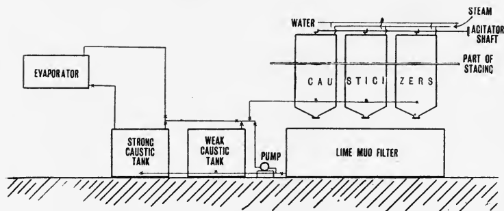
FIG. 49.—Diagram showing one method of arranging Causticizing Plant.
