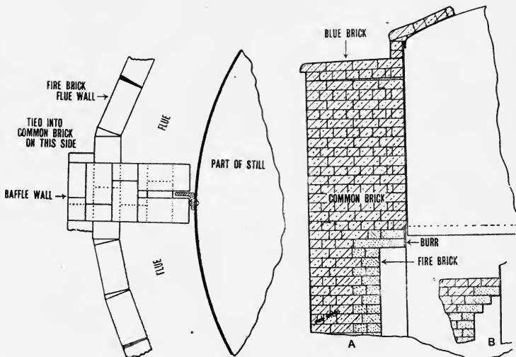
FIG. 24.—Diagram showing a Method of Keeping Flue Light at Baffle Wall.
