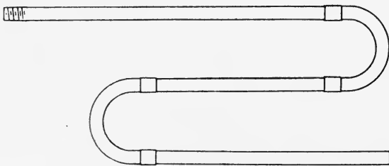
FIG. 11.—S Pipe Safety Contrivance: used instead of a Safety Valve.
