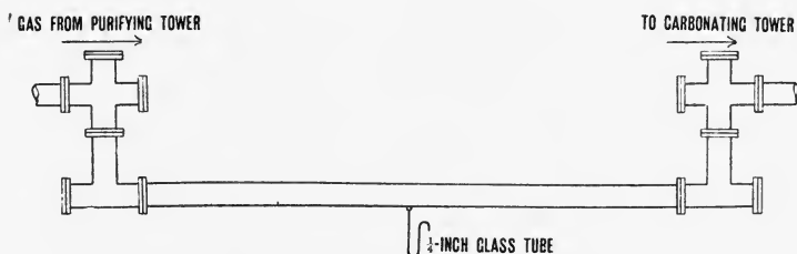
FIG. 48.—U Bend to separate Water from Gas.
