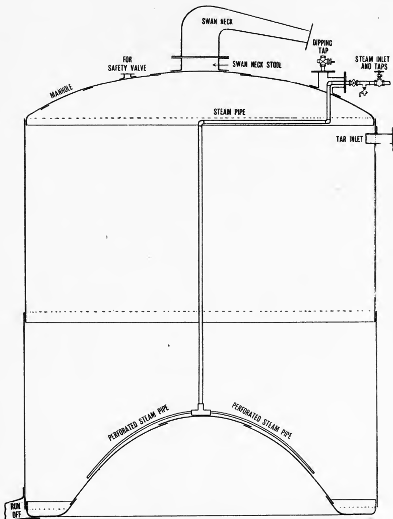
FIG. 12.—Diagrammatic Illustration of Tar Still.
