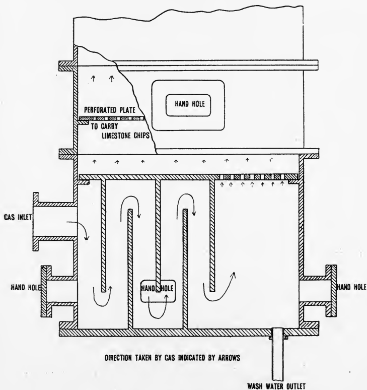
FIG. 46.—Purifying Tower with Dust Separator built in bottom.
