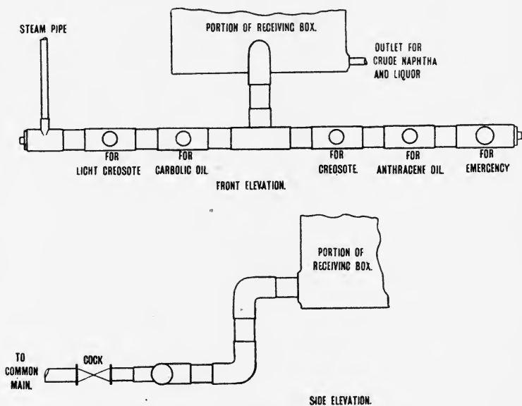
FIG. 34.—One Method of Connecting Common Mains to Receiving Box.
