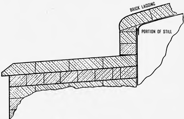
FIG. 20.—Brickwork of Still Top with Coping.
