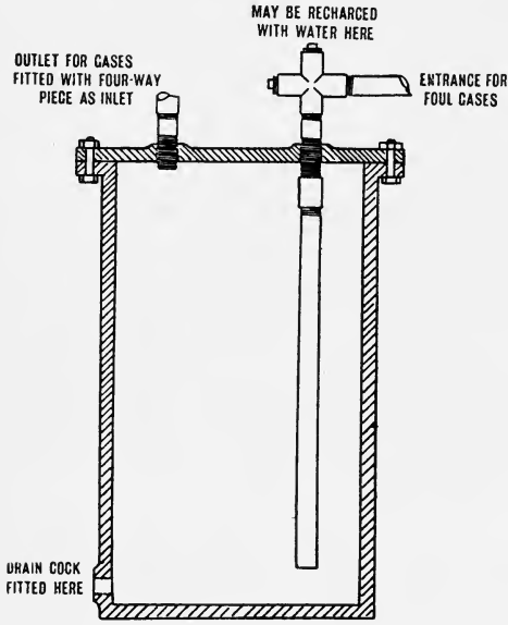
FIG. 33.—Seal Pot for Foul Gas Main.
