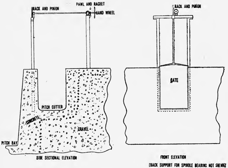
FIG. 37.—Pitch Gutter Outlet, showing Gate Valve.
