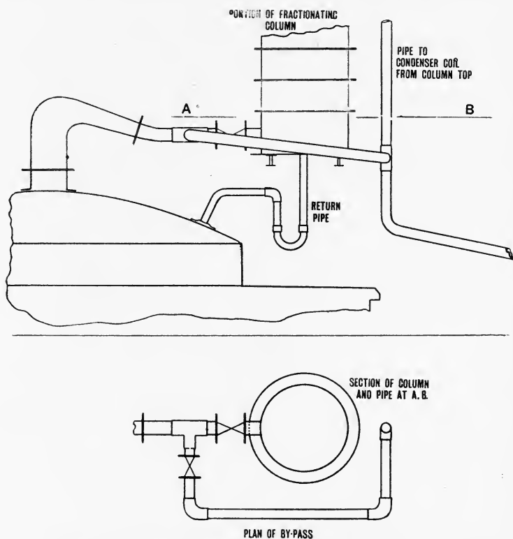
FIG. 50.—Diagram illustrating a method of Attaching Fractionating Column to a Cresylic Still and arranging a By-pass.
