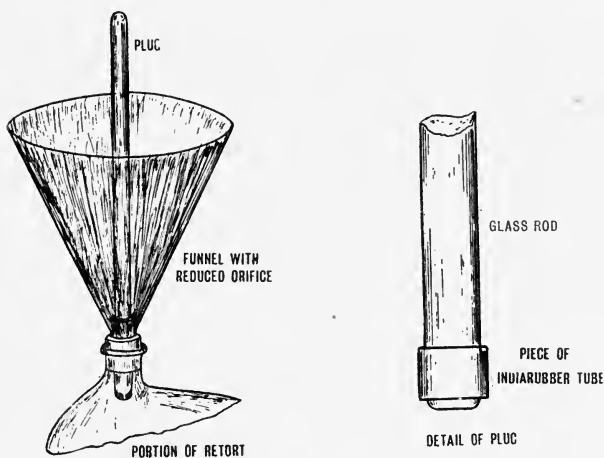
FIG. 60.—Funnel and Plug used in determining Water in Tar.
