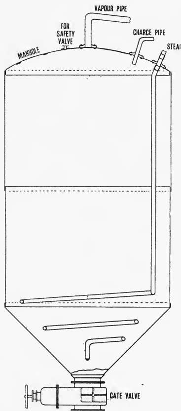
FIG. 54.—Still for the Distillation of Neutralized Pyridine Acid.
