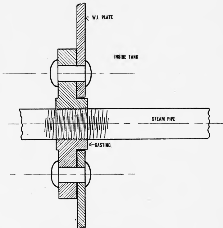
FIG. 1.—A method of inserting Steam Pipe into Storage Tanks.
