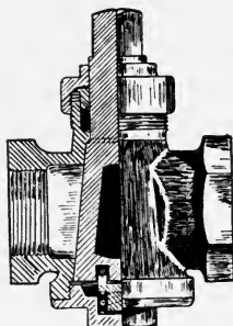
FIG. 18.—Butterfield Cock.
