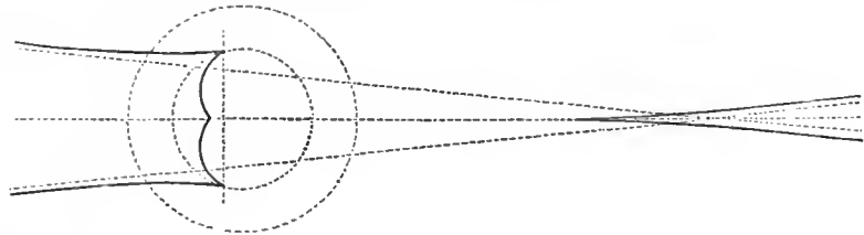
Fig. 12. a = \frac{1}{2} .
