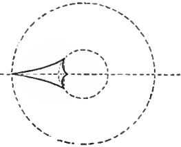
Fig. 13. a = \frac{1}{3} .
