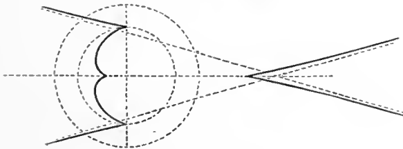
Fig. 10. a = \frac{1}{\sqrt{2}} .
