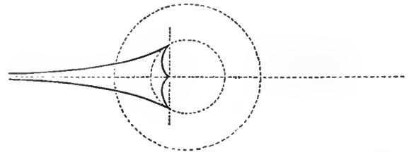
Fig. 12. a = \frac{1}{2} .
