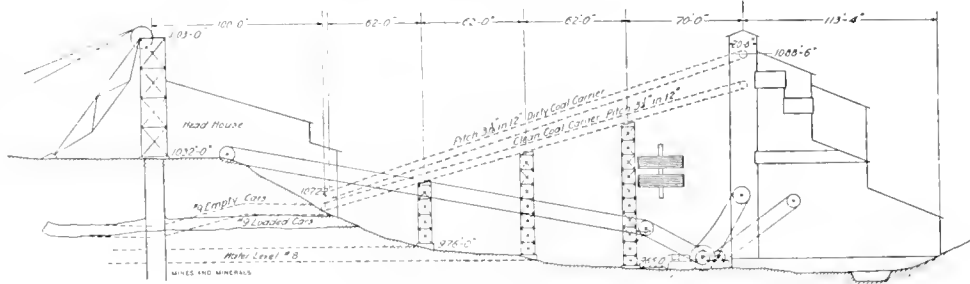
FIG. 3. PROFILE OF COALDALE PLANT
