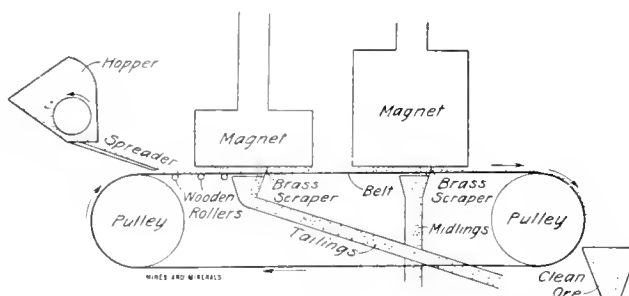
FIG. 4. SECTION THROUGH MAGNETIC CONCENTRATOR
