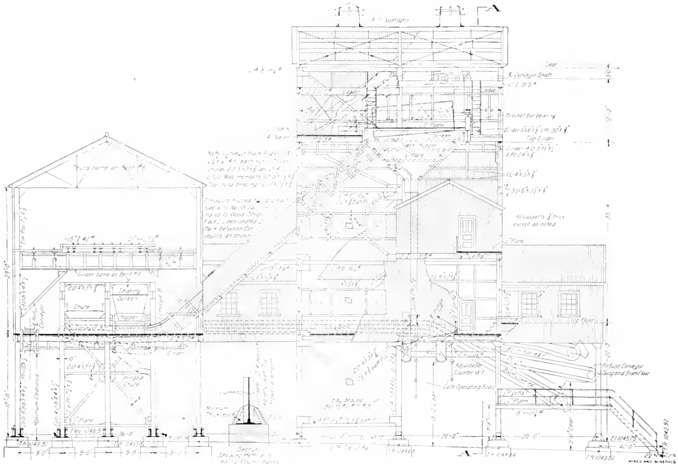
FIG. 6. SIDE ELEVATION OF HOISTING SHAFT TIPPIL
