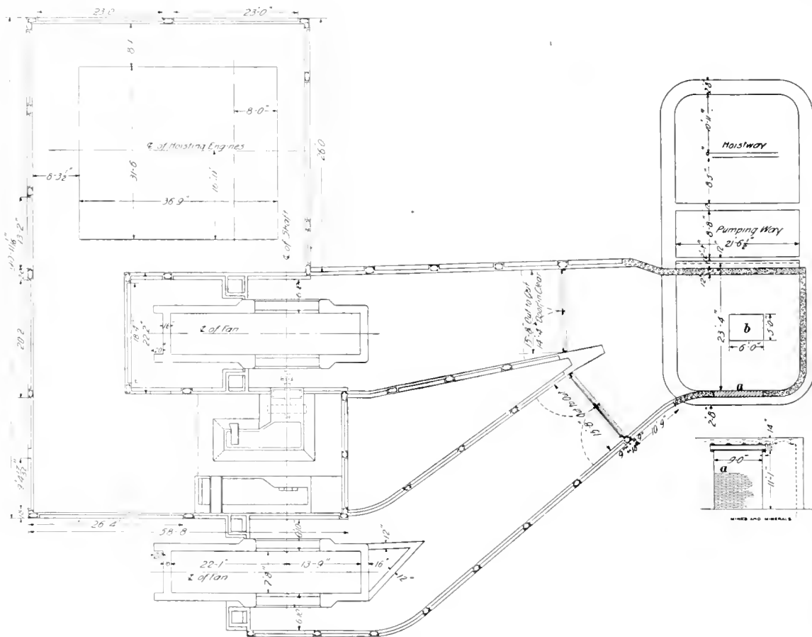
FIG. 2. PLAN OF SHAFT AND SURFACE WORKS, WOODWARD NO. 3 SHAFT
