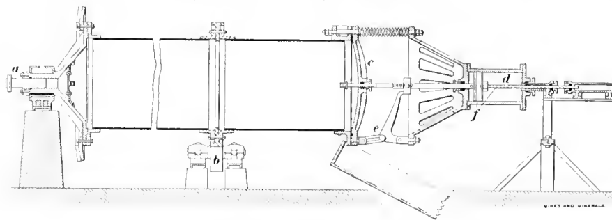
FIG. 1. SECTION, BURT REVOLVING FILTER
