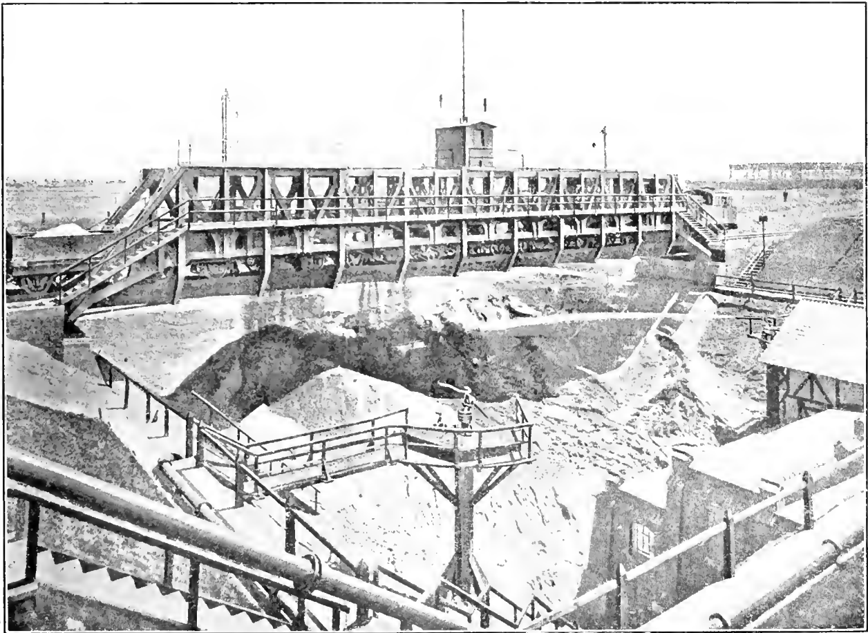
FIG. 8. HYDRAULIC FILLING AT KOENIGIN-LOUISEN MINE
