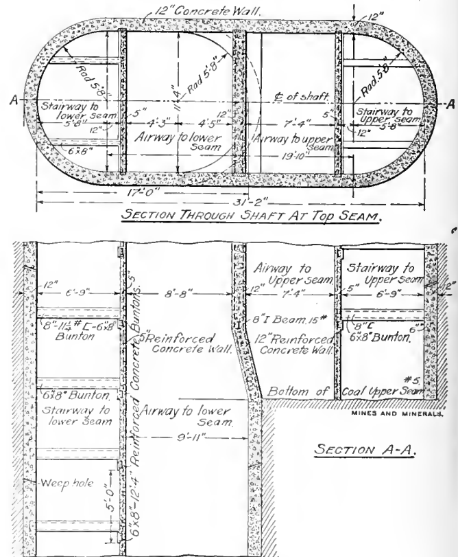
FIG. 3. SECTION AND ELEVATION OF SHAFT LINING
