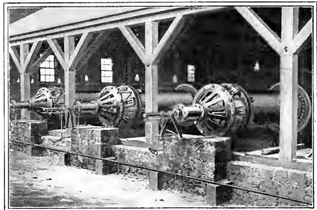
FIG. 5. BATTERY OF REVOLVING FILTERS AT EL ORO
