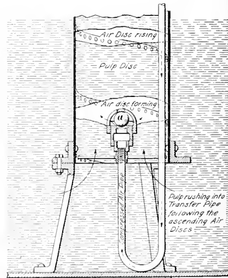
FIG. 7. OPERATION OF BALL VALVE
