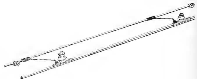
FIG. 6. METHOD OF CONNECTING FEEDER WIRE TO THE TROLLEY BY MEANS OF TWO OR MORE TAPS TO OBTAIN FULL CAPACITY OF FEEDER WIRE
