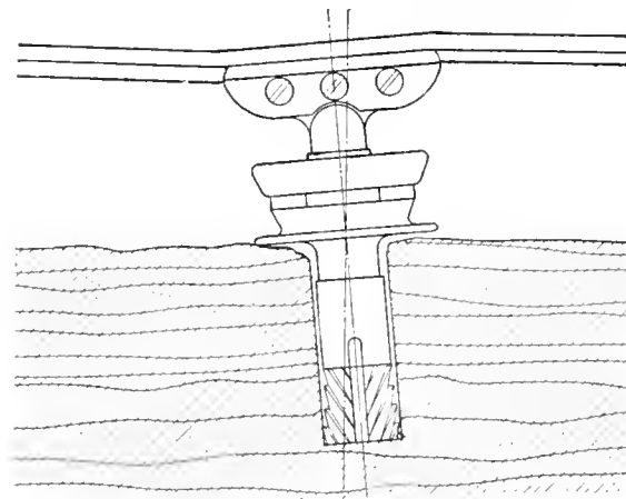
FIG. 5. EFFECT ON TROLLEY WIRE OF INSTALLING HANGER OUT OF PLUMB
