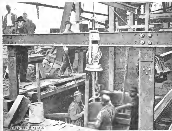
FIG. 1. FIREPROOFING MAIN SHAFT
