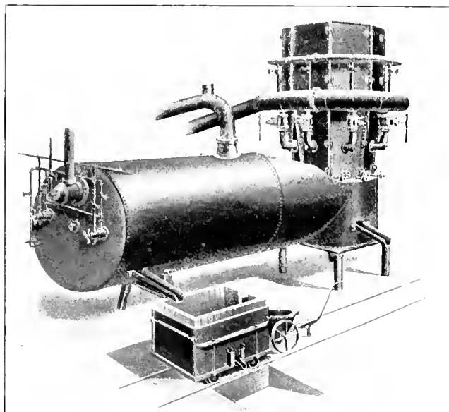
OIL BLAST FURNACE
