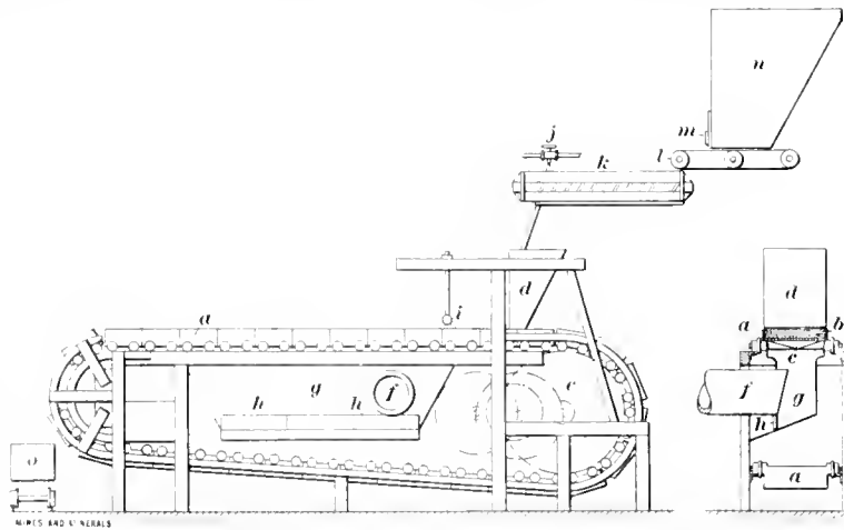
FIG. 1. LONGITUDINAL AND CROSS SECTION OF SINTERING MACHINE
