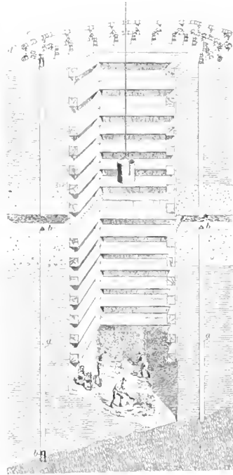
FIG. 1. SINKING IN FROZEN GROUND
