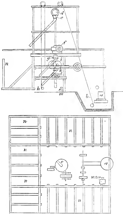
FIG. 6. PLAN AND ELEVATION OF SAMPLING MILL
