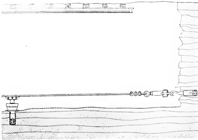
FIG. 3. APPROVED METHOD OF DEAD ENDING TROLLEY WIRE
