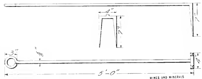
PLAN AND SECTION OF CHUTE HOOK
