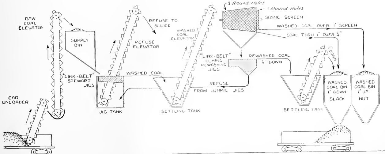
FIG. 4. FLOW SHEET SHOWING METHOD OF TREATMENT, CONSOLIDATED COAL COMPANY WASHERY
