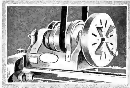
FIG. 1. GEAR GUARD
