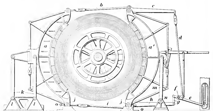
FIG. 6. POST BRAKE
