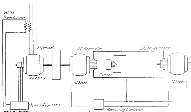
FIG. 1. DIAGRAM OF ELECTRIC HOIST
