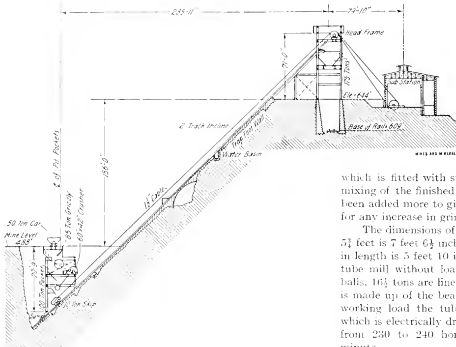
FIG. 7. SECTION THROUGH INCLINE
