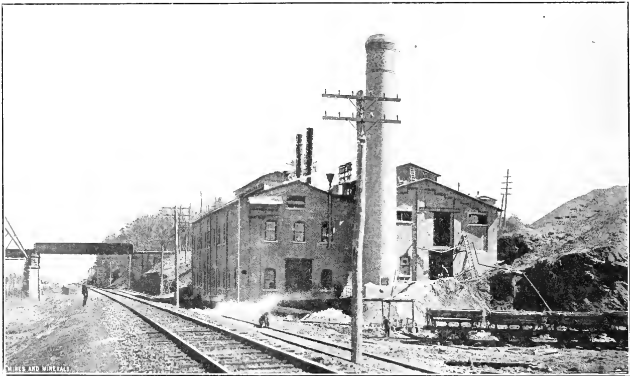
FIG. 6. NANTICOKE POWER HOUSE.
