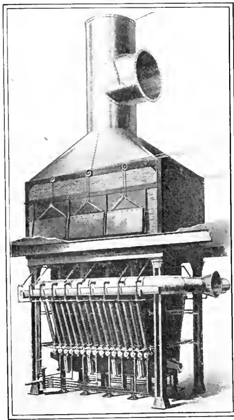
FIG. 2. RECTANGULAR COPPER FURNACE
