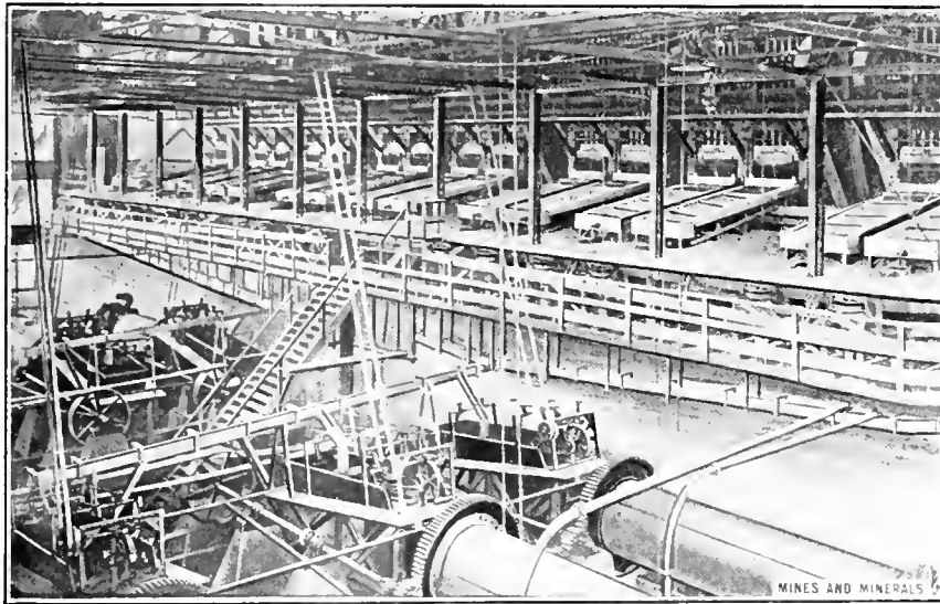
FIG. 1. BATTERY AND TUBE-MILL FLOOR OF CONCENTRATING MILL
