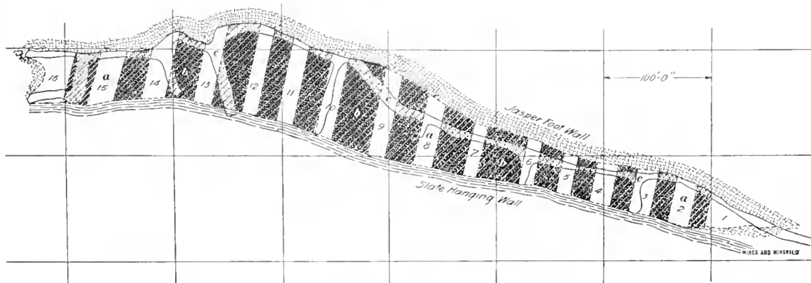
FIG. 1. PLAN, SHOWING DEVELOPMENT DRIFT AND OUTLINE OF ROOMS AND PILLARS
