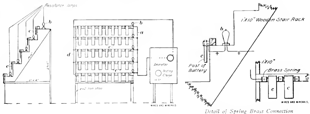
FIG. 2. CHARGING RACK
