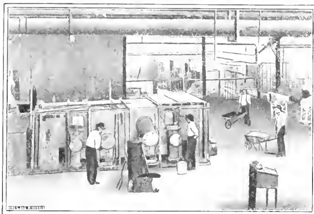
FIG. 1. REVERBERATORY FURNACE AT PORT PIRIE
