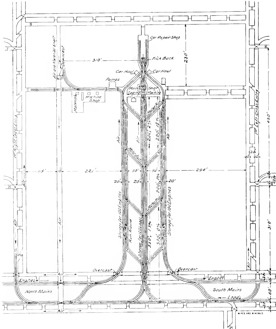
PLAN FOR SHAFT BOTTOM
