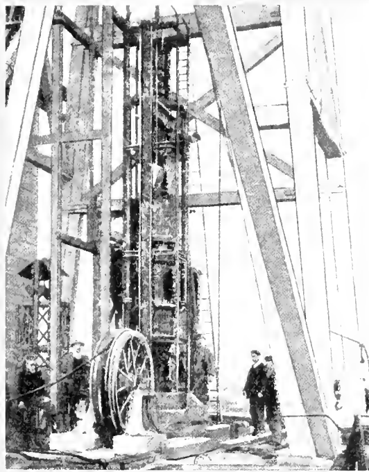
FIG. 2. SINKING PUMP, HARVEY'S SHAFT
