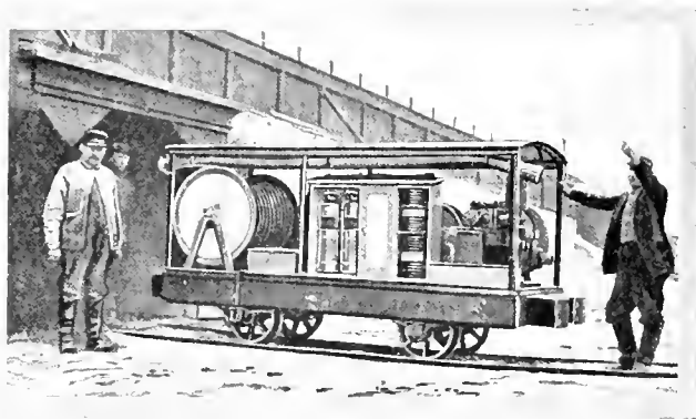
FIG. 2. ELECTRIC FIRE-FIGHTING CAR (LEFT-HAND SIDE)
