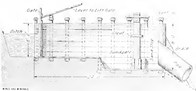
FIG. 5. PENSTOCK CONNECTING PIPE LINE WITH DITCH
