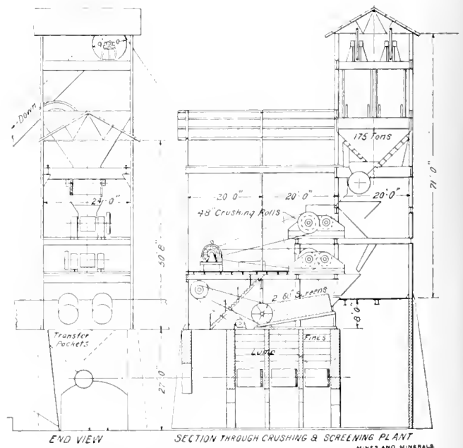
FIG. 8. END VIEW AND SECTION, ORE PREPARING PLANT
