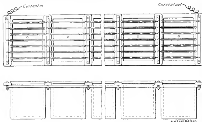
FIG. 9. PATH OF CURRENT THROUGH GOLD CELLS
