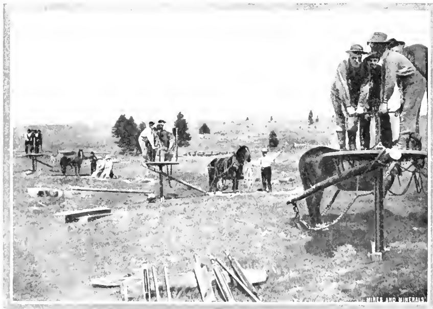
TESTING ALLUVIAL DEPOSITS WITH EMPIRE DRILLS
