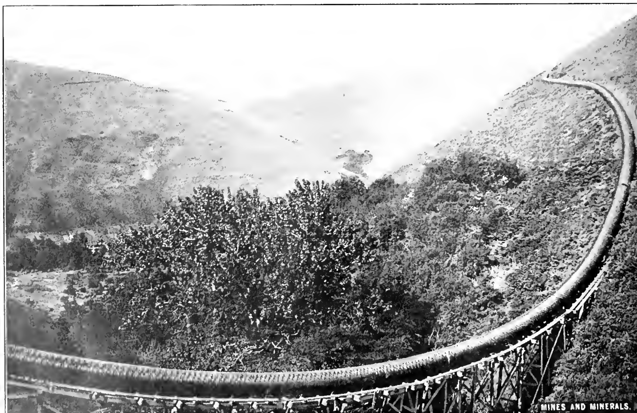
FIG. 1. CONTINUOUS WOODEN-STAVE PIPE, 5 MILES LONG, 48 INCHES DIAMETER
