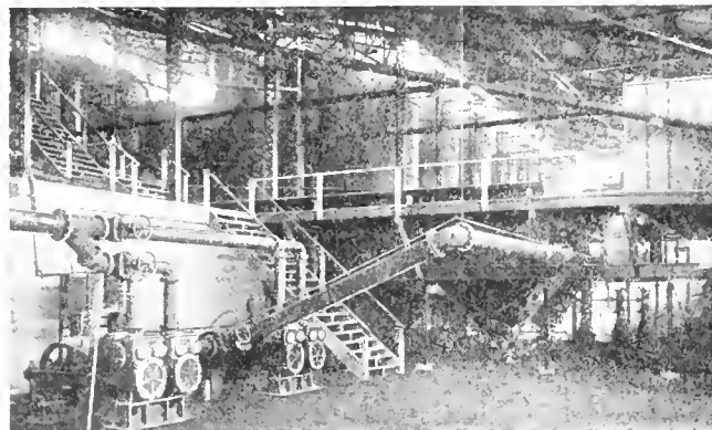
FIG. 4. VACUUM PUMPS AND ENDS OF FILTER BOXES
