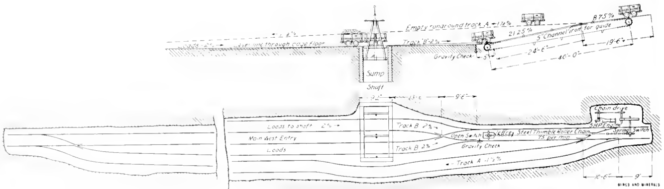
FIG. 2. PLAN OF SECTION OF SHAFT BOTTOM AND CAGING ARRANGEMENTS
