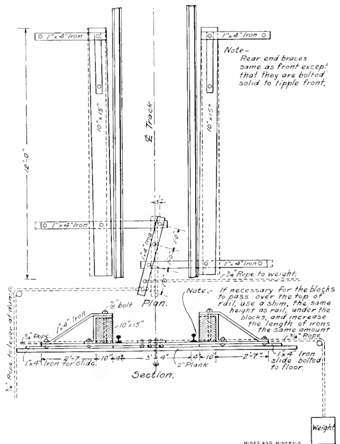
SAFETY BLOCKS, CASTLE GATE TIPPLE
