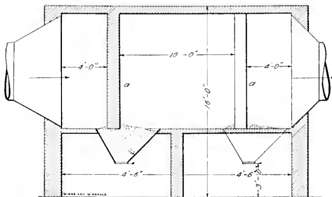
FIG. 1. SECTIONAL ELEVATION OF FUME CHAMBER
