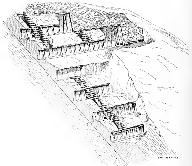
FIG. 4. PERSPECTIVE VIEW OF METHOD OF MINING
