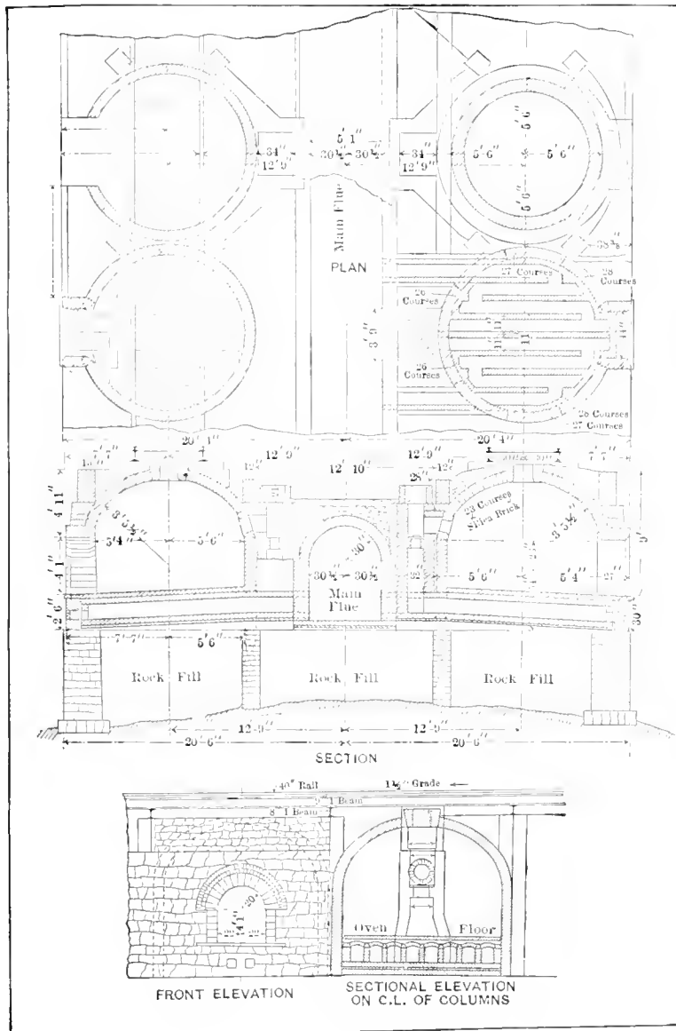
FIG. 3. DETAILS OF UNDER-FLUE COKE OVENS
