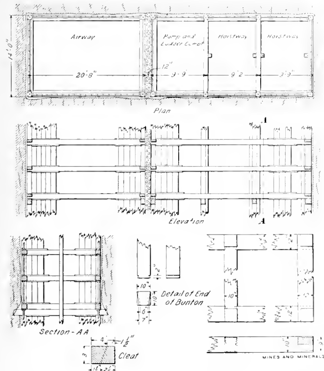
FIG. 3. PLAN AND DETAILS OF TIMBERING, LOOMIS SHAFT
