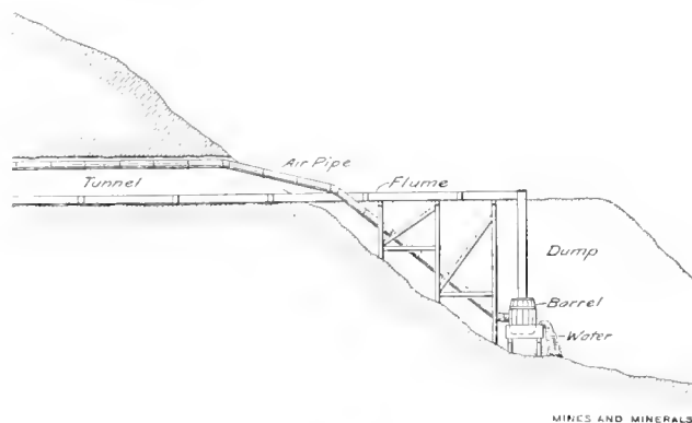
FIG. 1. ORE MINE VENTILATOR
