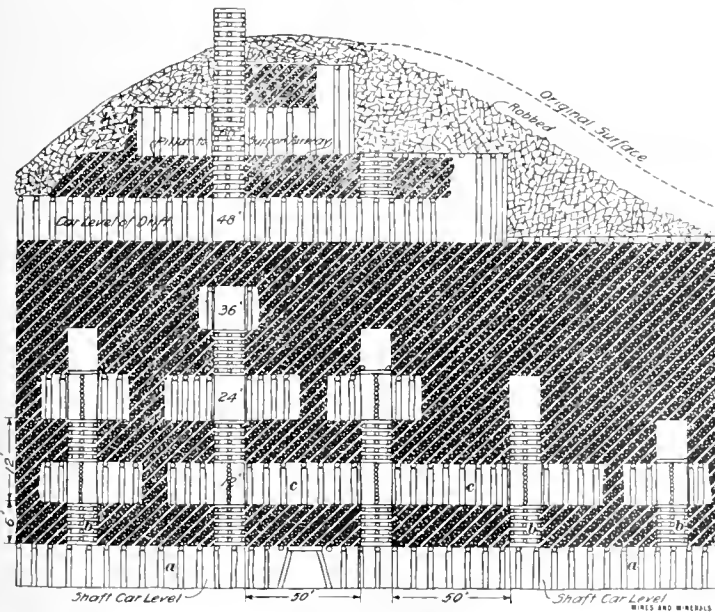
FIG. 5. ELEVATION, SHOWING METHOD OF MINING BY LOW MOOR IRON CO.
