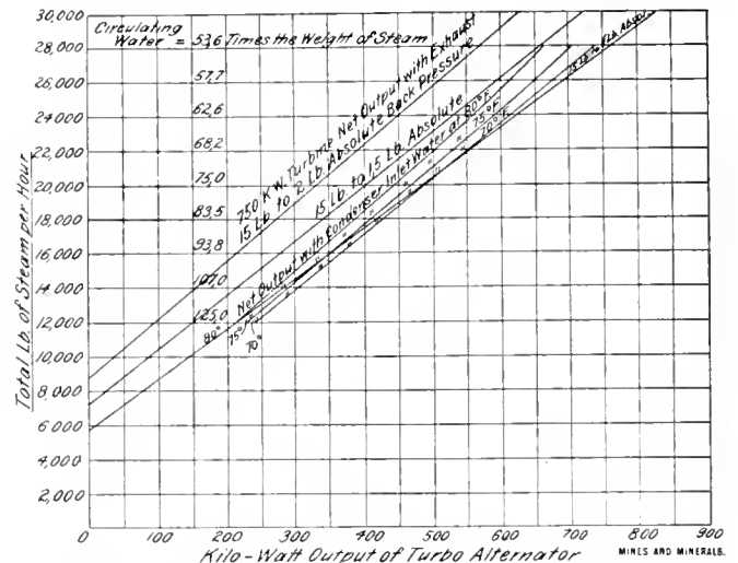
FIG. 2. EFFECT OF TEMPERATURE OF CONDENSER INLET ON VACUUM AND NET OUTPUT OF AN EXHAUST TURBINE WITH COOLING TOWER IN CIRCUIT
