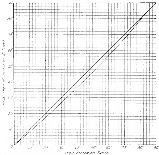
Curve of Correction For Error Due to Capillarity in Testing Diamond Drill Holes Curve for Tubes
