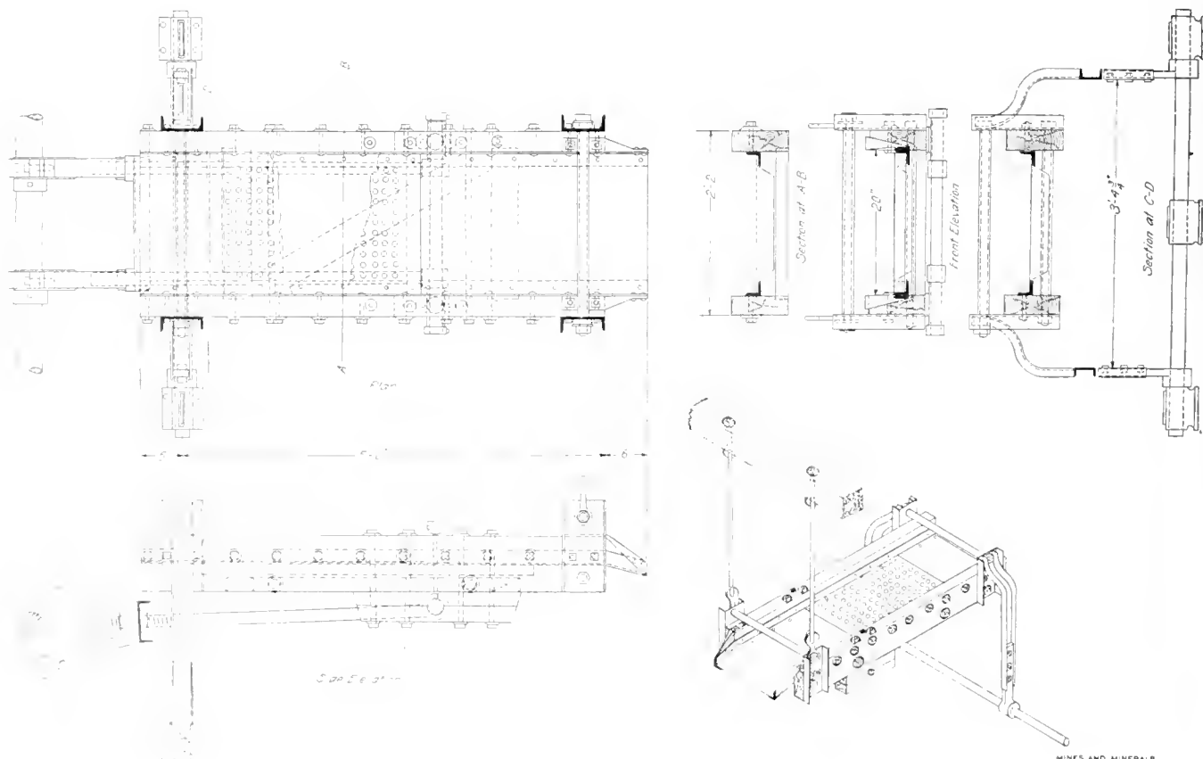
FIG. 1. SHAKING SCREEN
