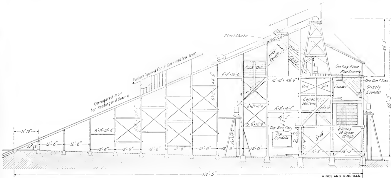
FIG. 1. HEAD-FRAME AND ORE BIN
