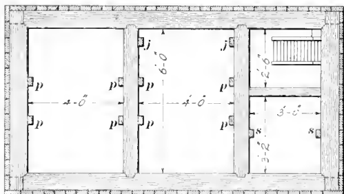
FIG. 3. PLAN OF SHAFT
