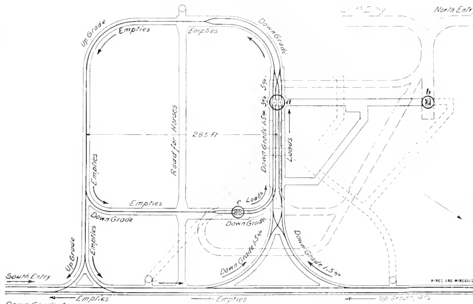
FIG. 1. PLAN OF SHAFT BOTTOM AT ARENBERG MINE
