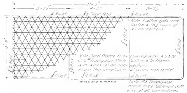
FIG. 10. STEEL FRAME SUPPORTING REINFORCEMENT
