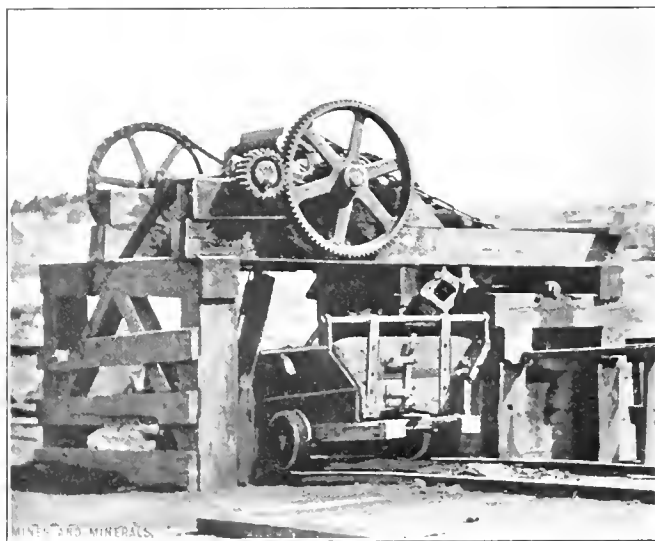
TOP OF BOILER-COAL ELEVATOR, NAVAJO MINE
