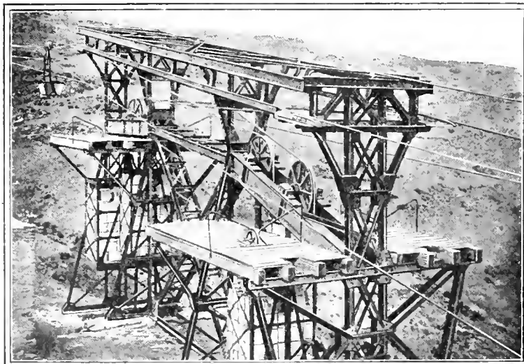
FIG. 1. TENSION DEVICES, TESORERO MINES
