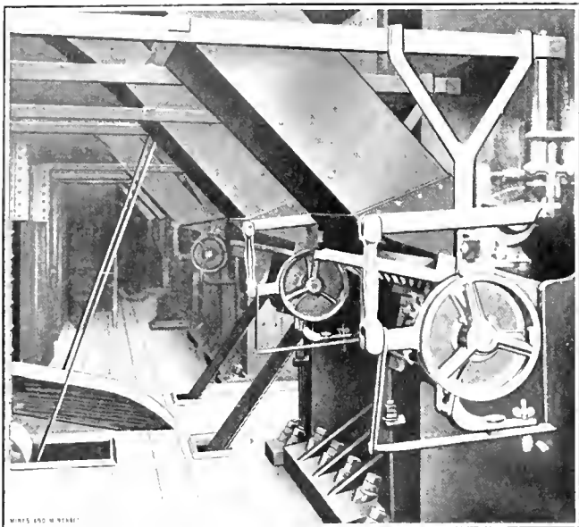
FIG. 2. AUTOMATIC FEEDERS
