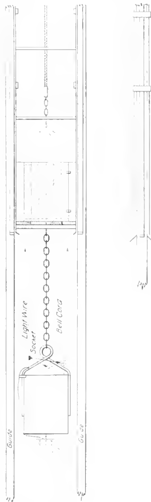
FIG. 1. ARRANGEMENT OF GUIDES AND CAGE
