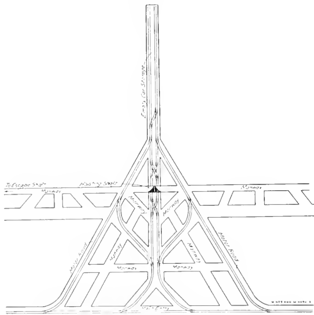
FIG. 5. PLAN OF SHAFT BOTTOM
