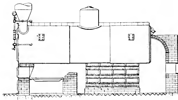
FIG. 2. SECTIONAL ELEVATION SHOWING GAS CONSUMER
