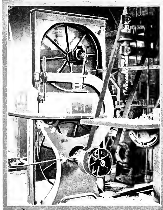
FIG. 3. BAND SAW GUARD
