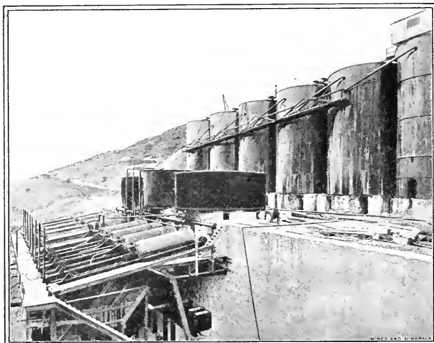
FIG. 2. PARRAL AND PACHUCA TANKS
