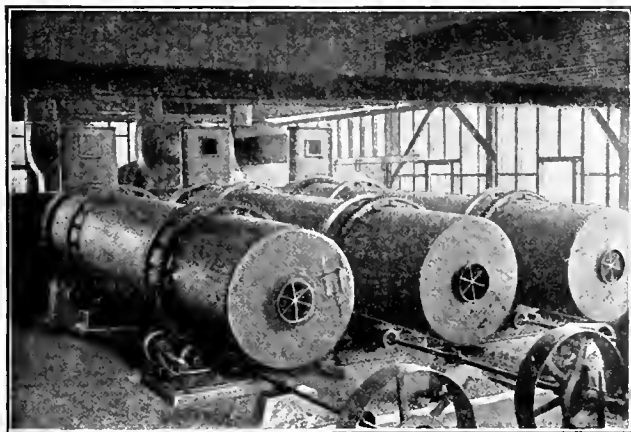
FIG. 1. ROTARY DOUBLE-SHELL DRYER, OUTSIDE
