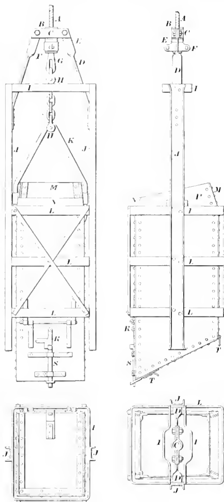
FIG. 1. SINKING SKIP
