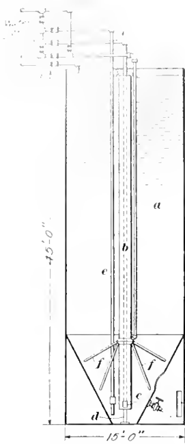
FIG. 4. PACHUCA TANK
