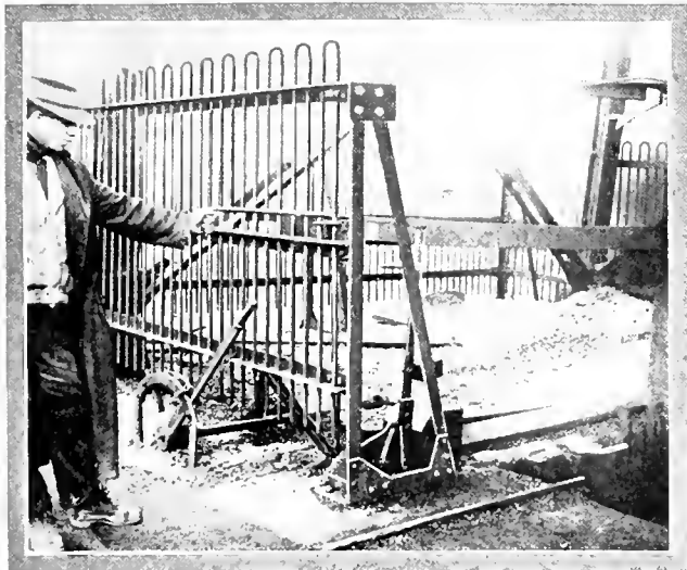
FIG. 9. SHAFT GATE LOCKING DEVICE
