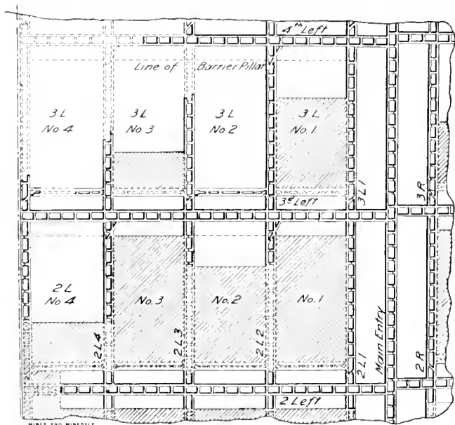
FIG. 1. LONGWALL MINING WORKED ADVANCING
