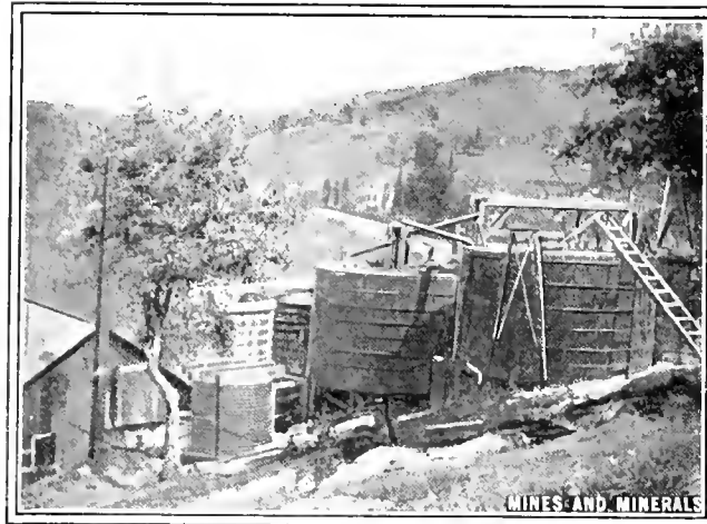
FIG. 1. DARROW-HAMBRIC PLANT, BUNKER HILL MILL
