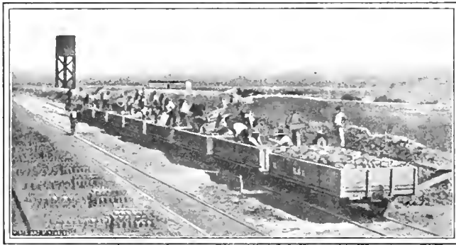
FIG. 4. HEAP ROASTING AND SINTERING NEAR BROKEN HILL.
