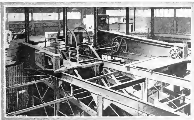
FIG. 3. MOTORS DRIVING TIPPIE MACHINERY
