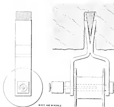
MINES AND MINERALS SELF-OILING ROLLER
