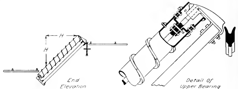
FIG. 2. DETAILS OF SPIRAL FOR RAISING ROPE TO KNUCKLE SHEAVE
