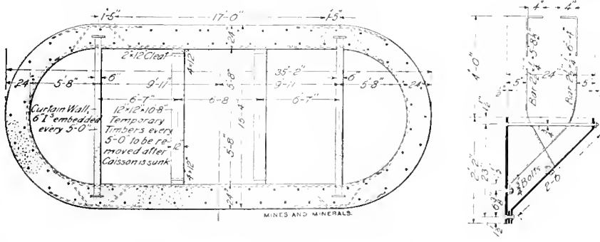
FIG. 6. STEEL SHOE USED AT VENTILATING SHAFT
