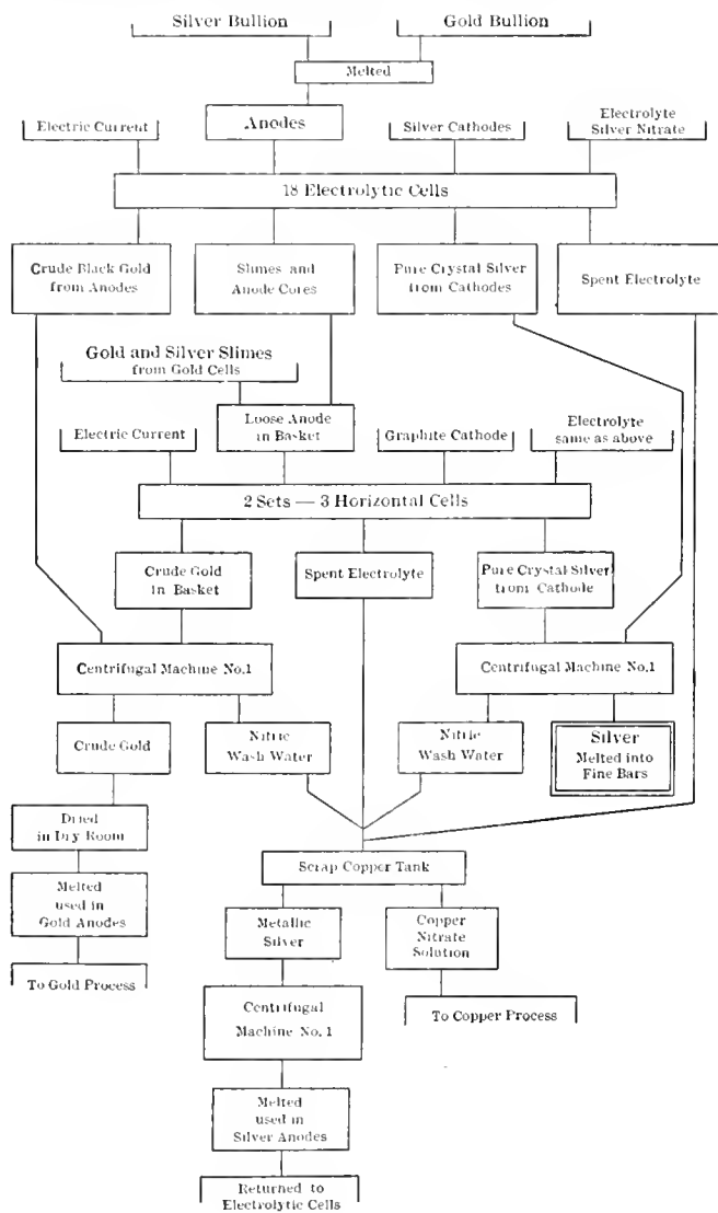
FIG. 1. DIAGRAM OF SILVER PROCESS
