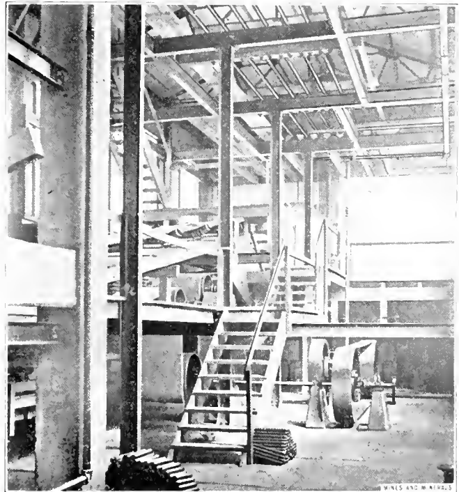
FIG. 5. LOADING CONVEYOR
