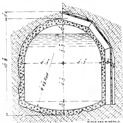
FIG. 1. SECTION OF TUNNEL NO. 17, JAWBONE DIVISION
