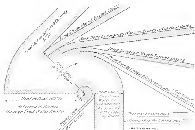
FIG. 8. SHOWING APPROXIMATE THERMAL EFFICIENCY OF A STEAM PLANT ARRANGED AS IN FIG. 6
