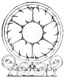
FIG. 3. END SECTION ROTARY DRIER, SHOWING CONCENTRIC SHELLS
