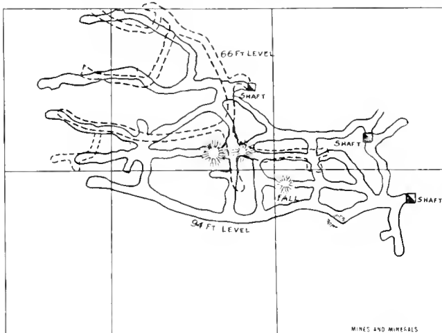
FIG. 3. SOFT GROUND MINE
