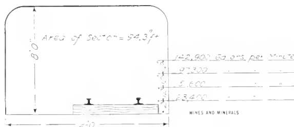
FIG. 1. CROSS-SECTION OF DRAINAGE TUNNEL
