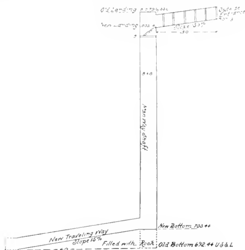
FIG. 1. SKETCH OF MANWAY SHAFT AT IMPERIAL MINE
