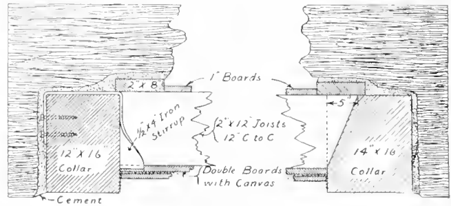
FIG. 2. DETAILS OF OVERCAST
