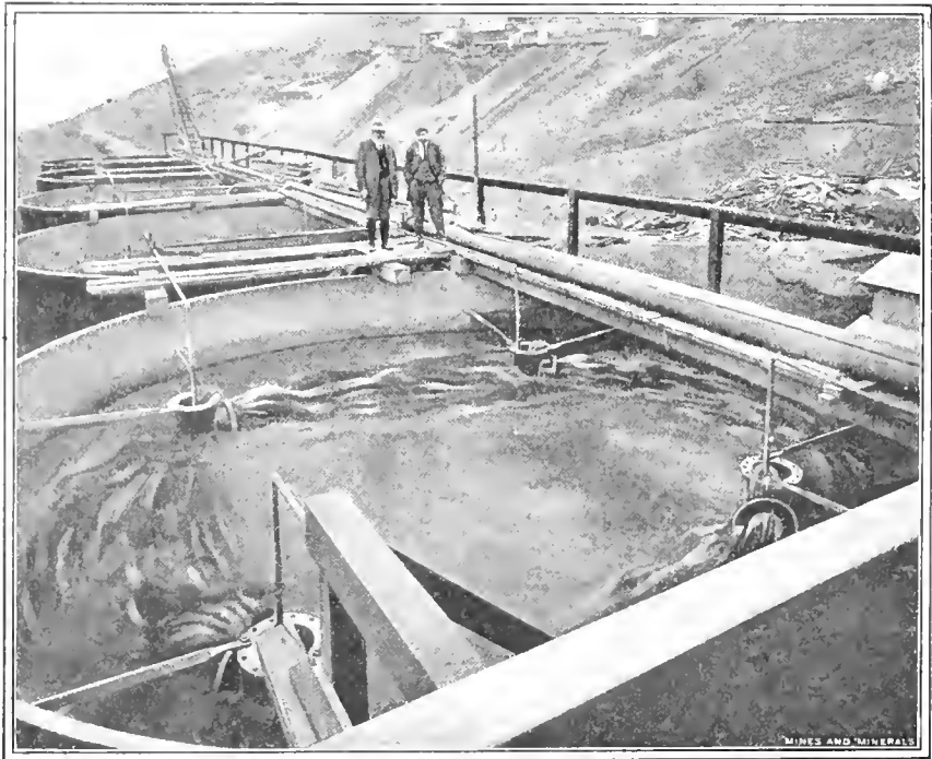
FIG. 3. ROTARY FLOW IN TANKS
