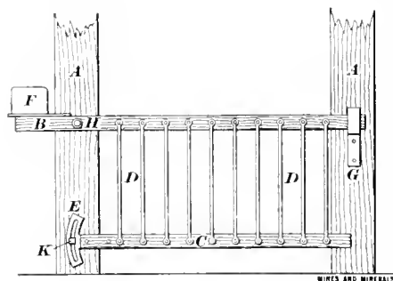
SHAFT GATE
