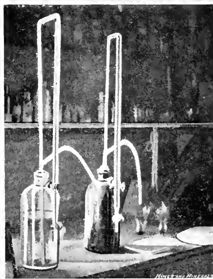
BURETTE STAND
