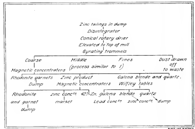
FIG. 8. BROKEN HILL CENTRAL MINE PROCESS
