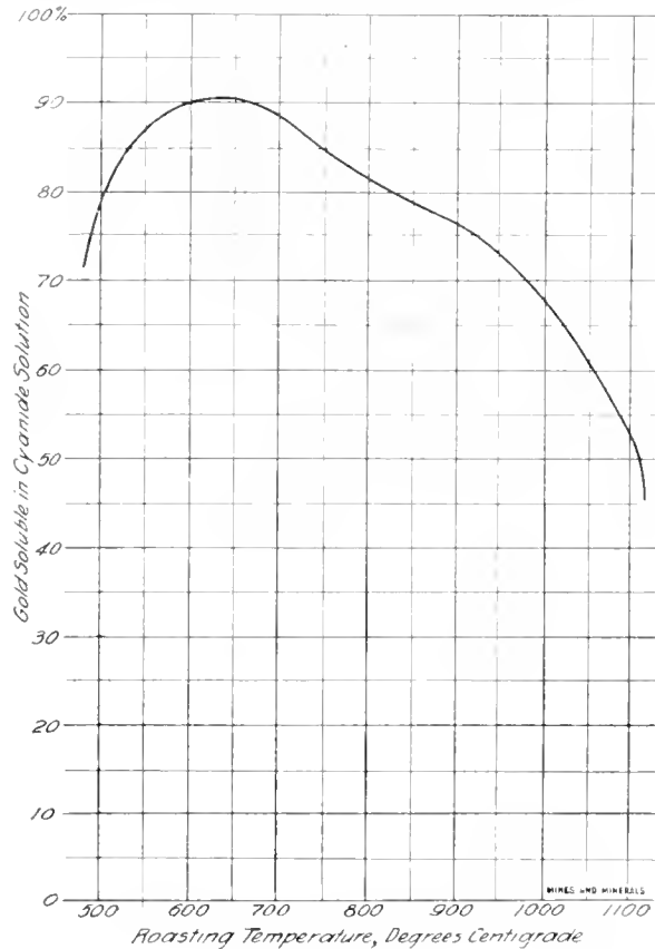
FIG. 1. ROASTING RESULTS
