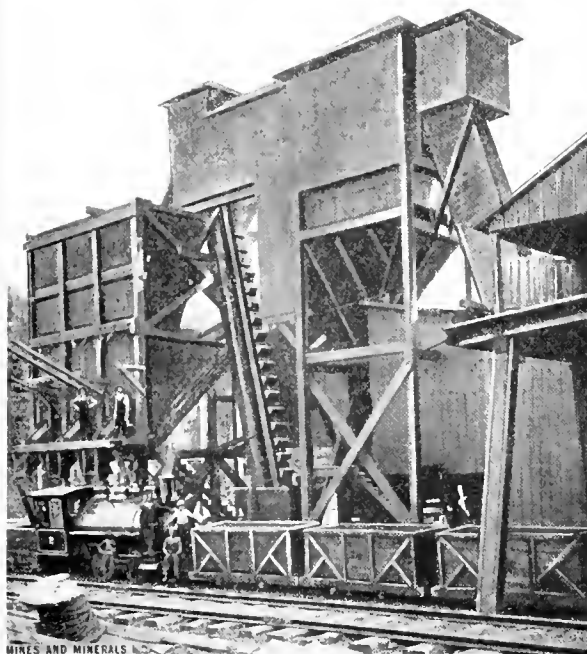
CONVEYORS FOR UNLOADING CARS AT LAHAUSAGE WASHERY
