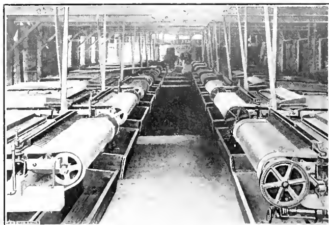
FIG. 3. VANNER ROOM
