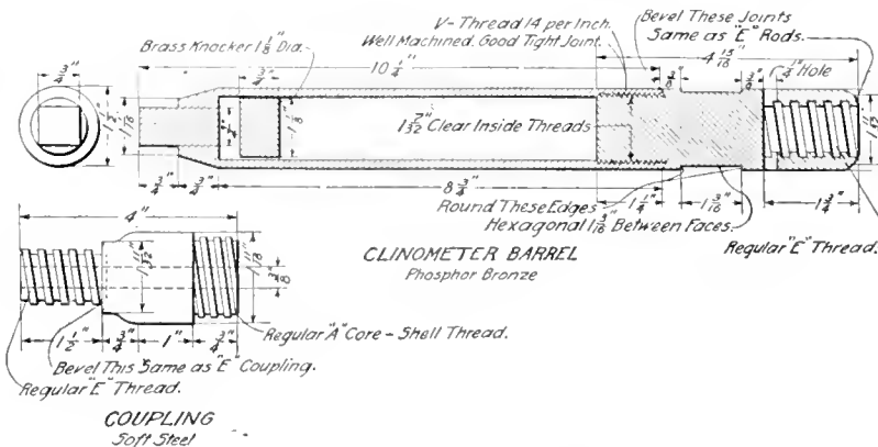
FIG. 1. DRILL HOLE CLINOMETER
