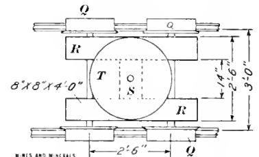
FIG. 3. TRUCK
