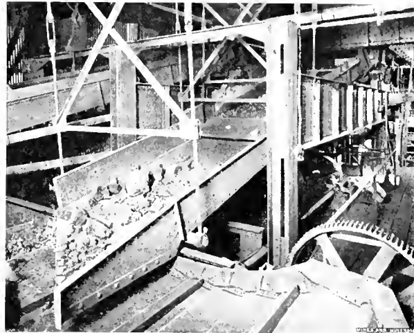
FIG. 7. SCREEN DISCHARGING TO PICKING BAND
