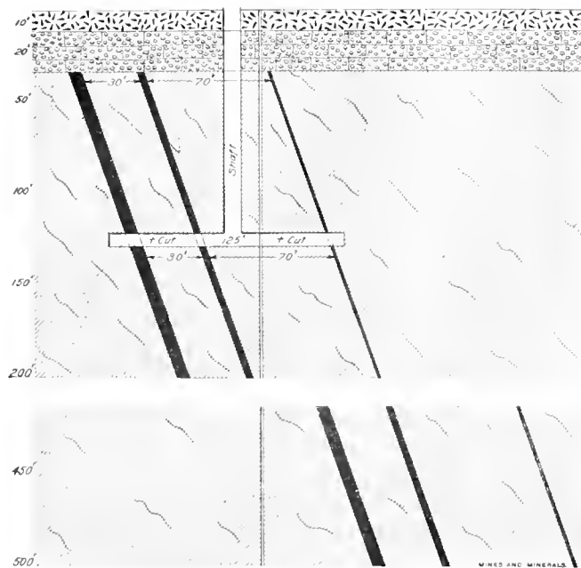
FIG. 2. SECTION AT CHARLEY COAL MINES
