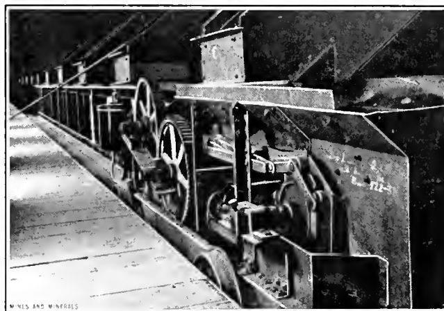
FIG. 2. MECHANICAL FEEDER AT SAMPLE BINS
