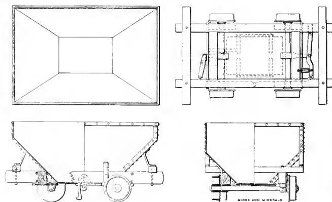
FIG. 3. COAL CAR
