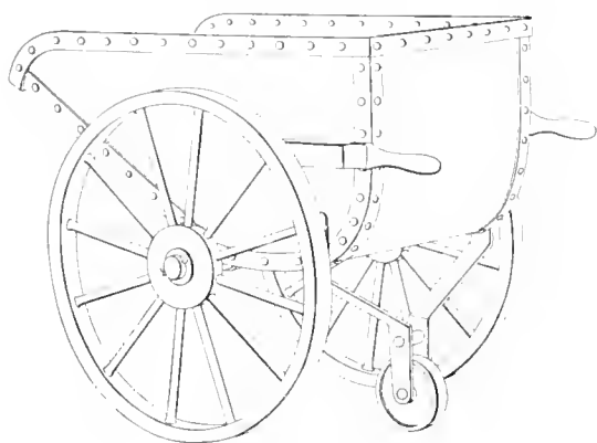
FIG. 2. FEED BARROW
