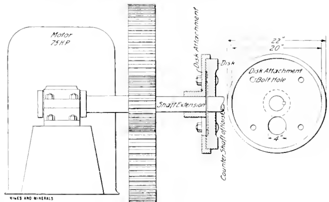
FIG. 1. CONNECTION FOR HOIST AND MOTOR
