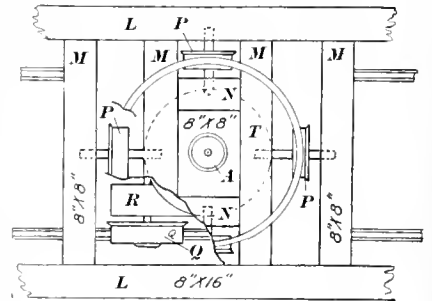
FIG. 2. TURNTABLE
