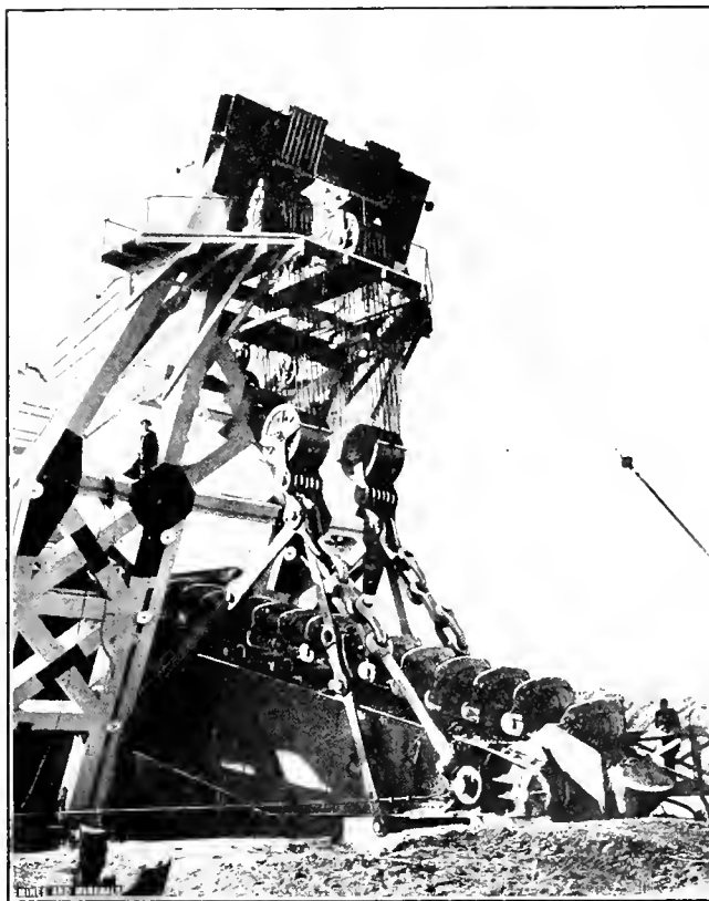
FIG. 3. SIDE VIEW OF DREDGE BUCKETS
