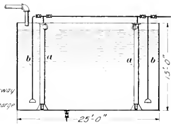
FIG. 5. PARRAL TANK (Same capacity as Fig. 1)
