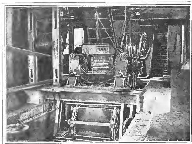
FIG. 2. EDISON 4' \times 3' ROLLS AND CONVEYER
