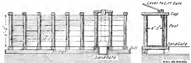
FIG. 4. FLUME WITH SAND GATE
