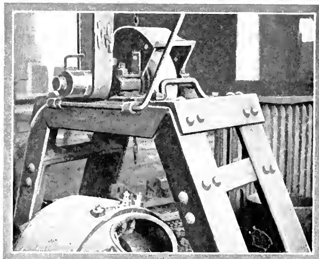
FIG. 2. EMERY WHEEL GUARD
