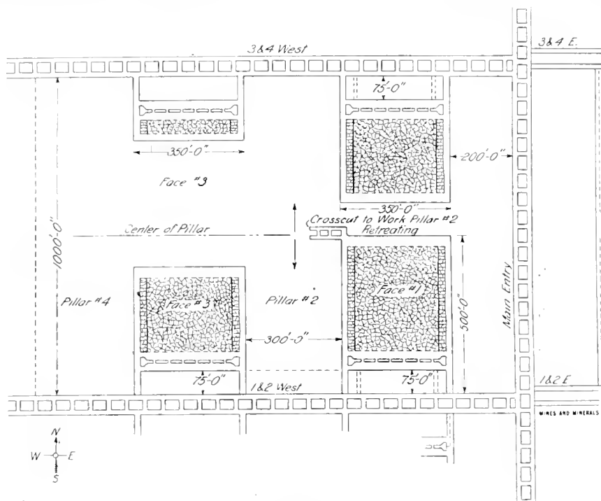
PANEL SYSTEM OF LONGWALL
