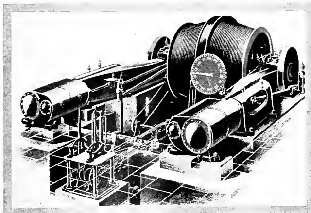
FIG. 5. ENGINE STOP
