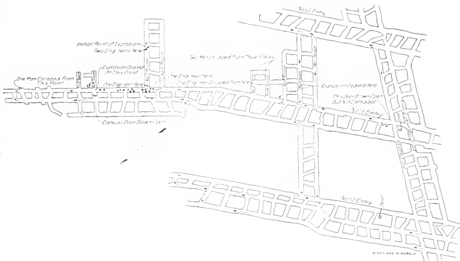
FIG. 2. PLAN OF NO. 1 MINE, BOTTOM CREEK COAL AND COKE CO.
