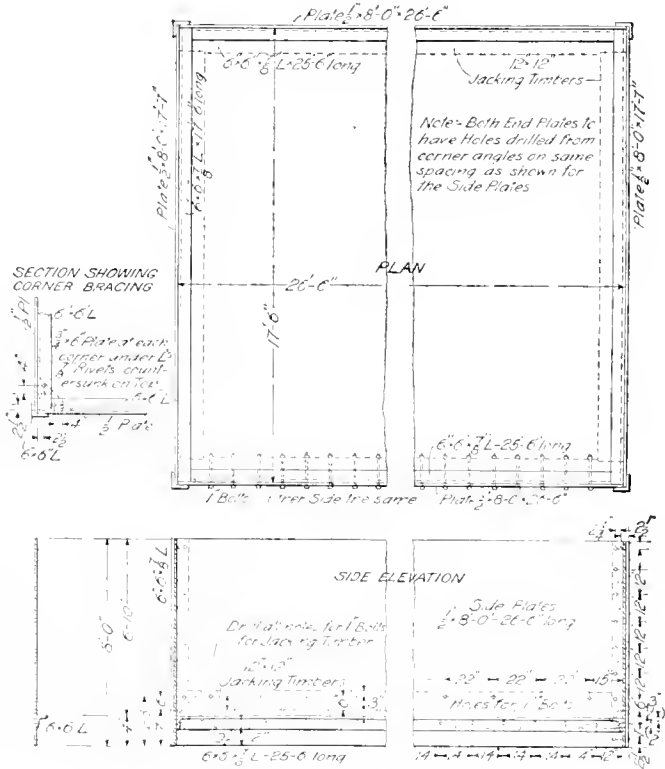
FIG. 5. STEEL SHOE USED AT HOISTING SHAFTS
