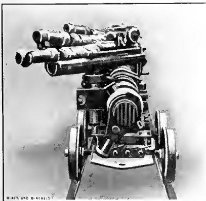
FIG. 1. CARRIAGE WITH DRILLS
