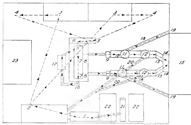
FIG. 3. FLOW SHEET
