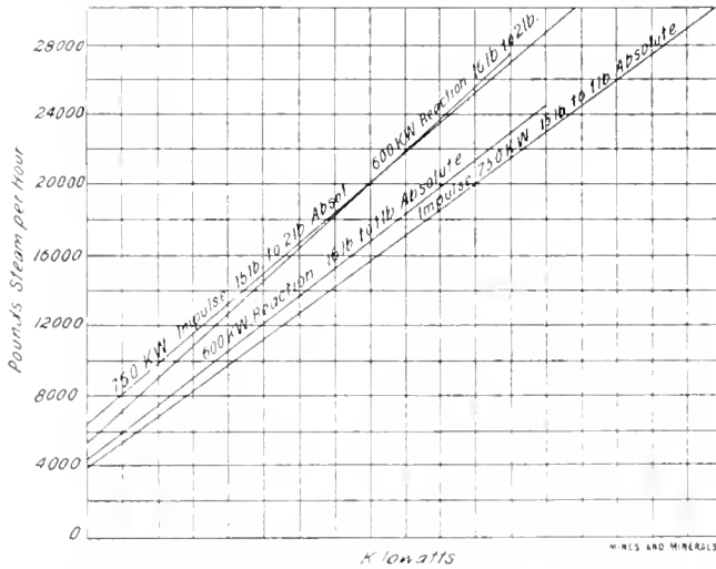
FIG. 9. EXHAUST STEAM CONSUMPTIONS OF IMPULSE AND REACTION MIXED PRESSURE TURBINES, WITH VARIOUS ABSOLUTE BACK PRESSURES
