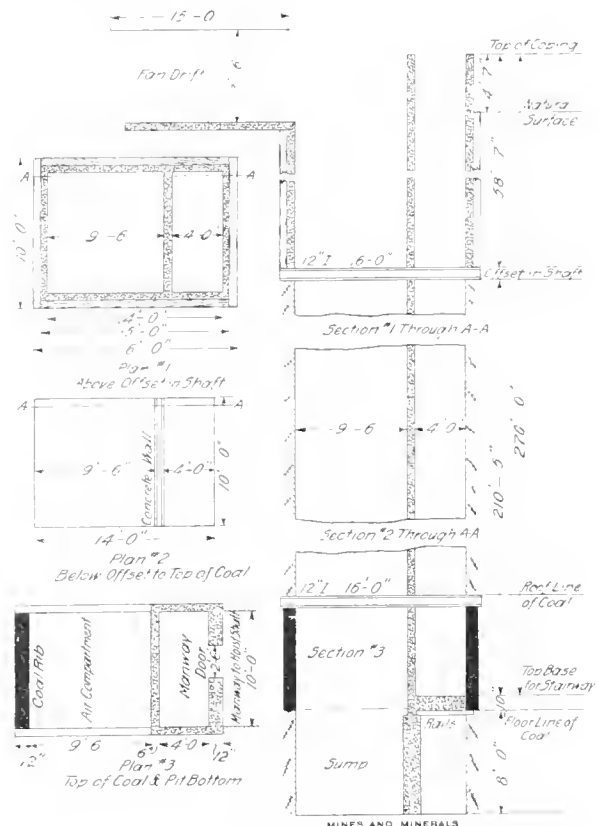
FIG. 8. PLANS AND LONGITUDINAL SECTIONS OF AIR SHAFT
