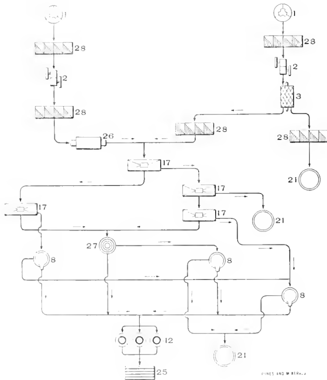
FIG. 2. FLOW SHEET, GOLDEN GATE MILL.
