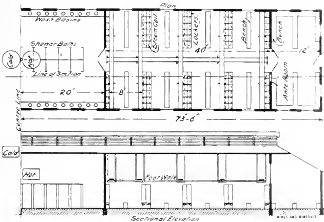
FIG. 1. SUGGESTED PLAN FOR WASH HOUSE
