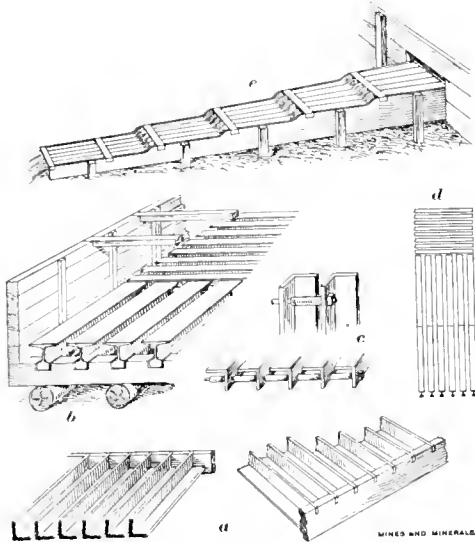
FIG. 3. RIFFLES AT KINGSBURY PLACER a, Angle Iron Riffles; b and d, Arrangement of Riffles; c, Vibratory Riffles; e, Bent Metal Riffles
