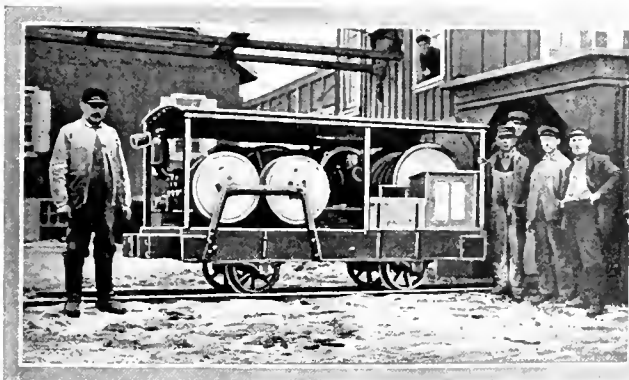
FIG. 1. ELECTRIC FIRE-FIGHTING CAR (RIGHT-HAND SIDE)
