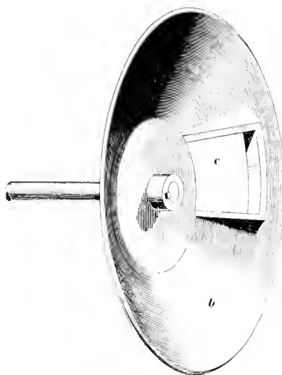
FIG. 2. SNYDER SAMPLER
