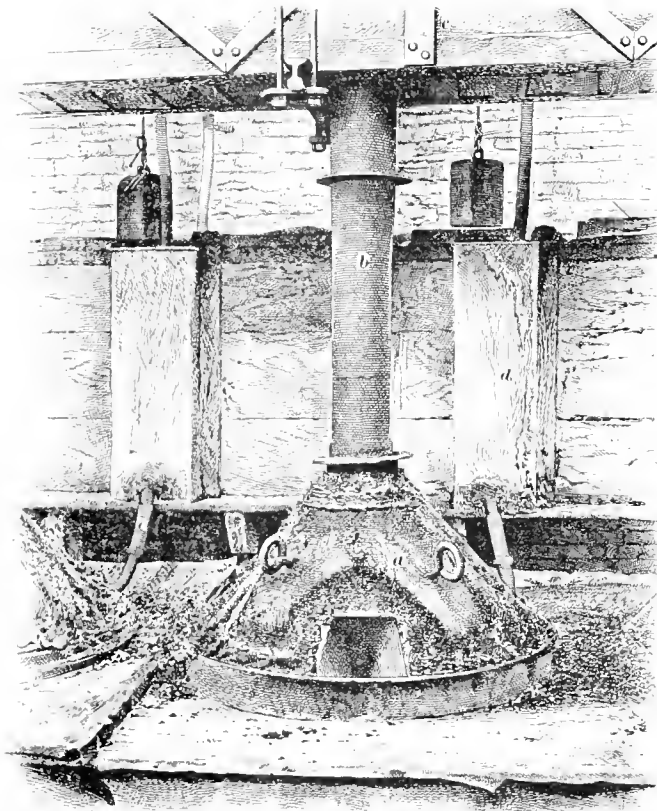
FIG. 2. UPPER PART OF PARTING KETTLE
