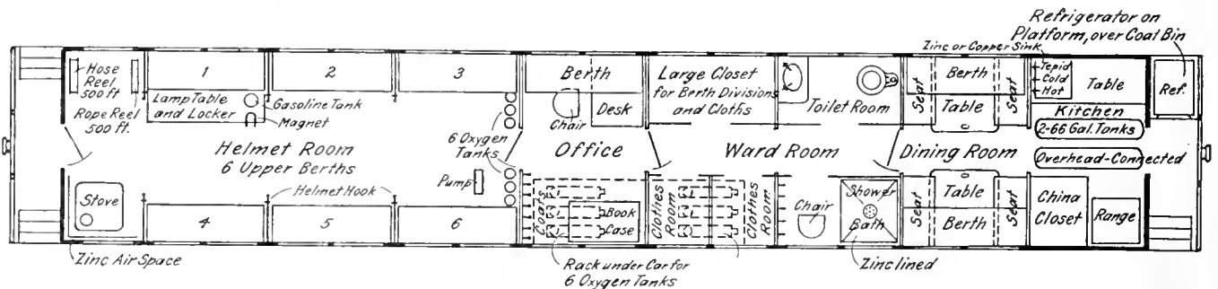
FIG. 2. PLAN OF INSTRUCTION CAR
