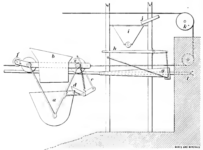
FIG. 1. TAILING DISPOSAL DEVICE
