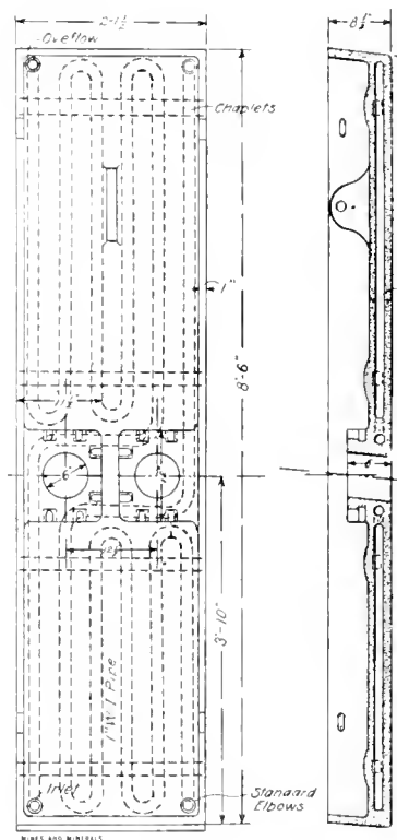
FIG. 1. WATER JACKET
