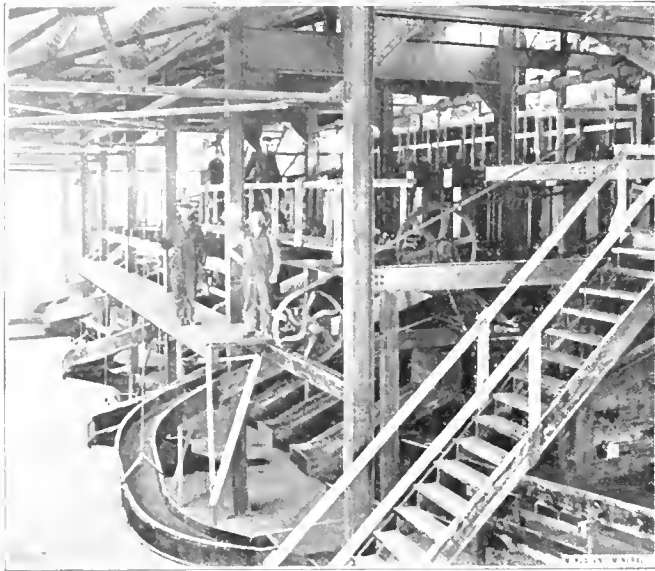
FIG. 2. JIG FLOOR
