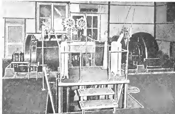
FIG. 2. ELECTRIC HOIST IRISH MAG MINE
