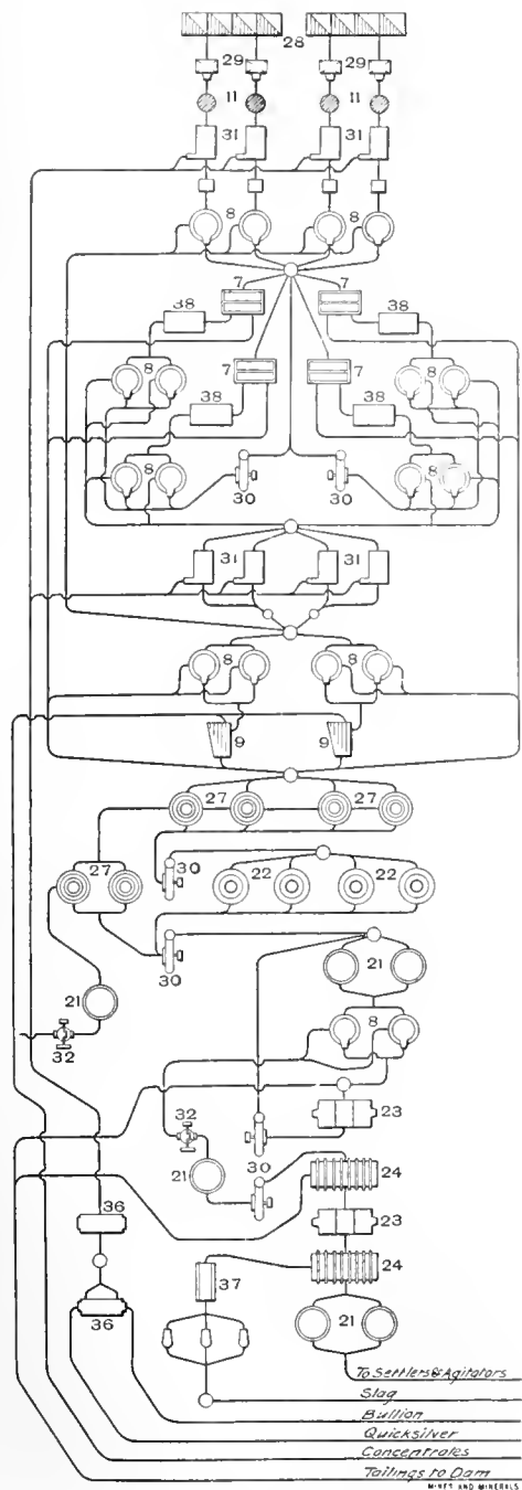
FIG. 3. FLOW SHEET OF CYANIDE MILL
