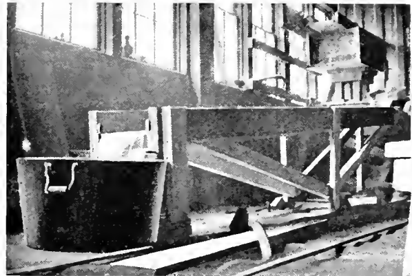
CANVAS TABLE
