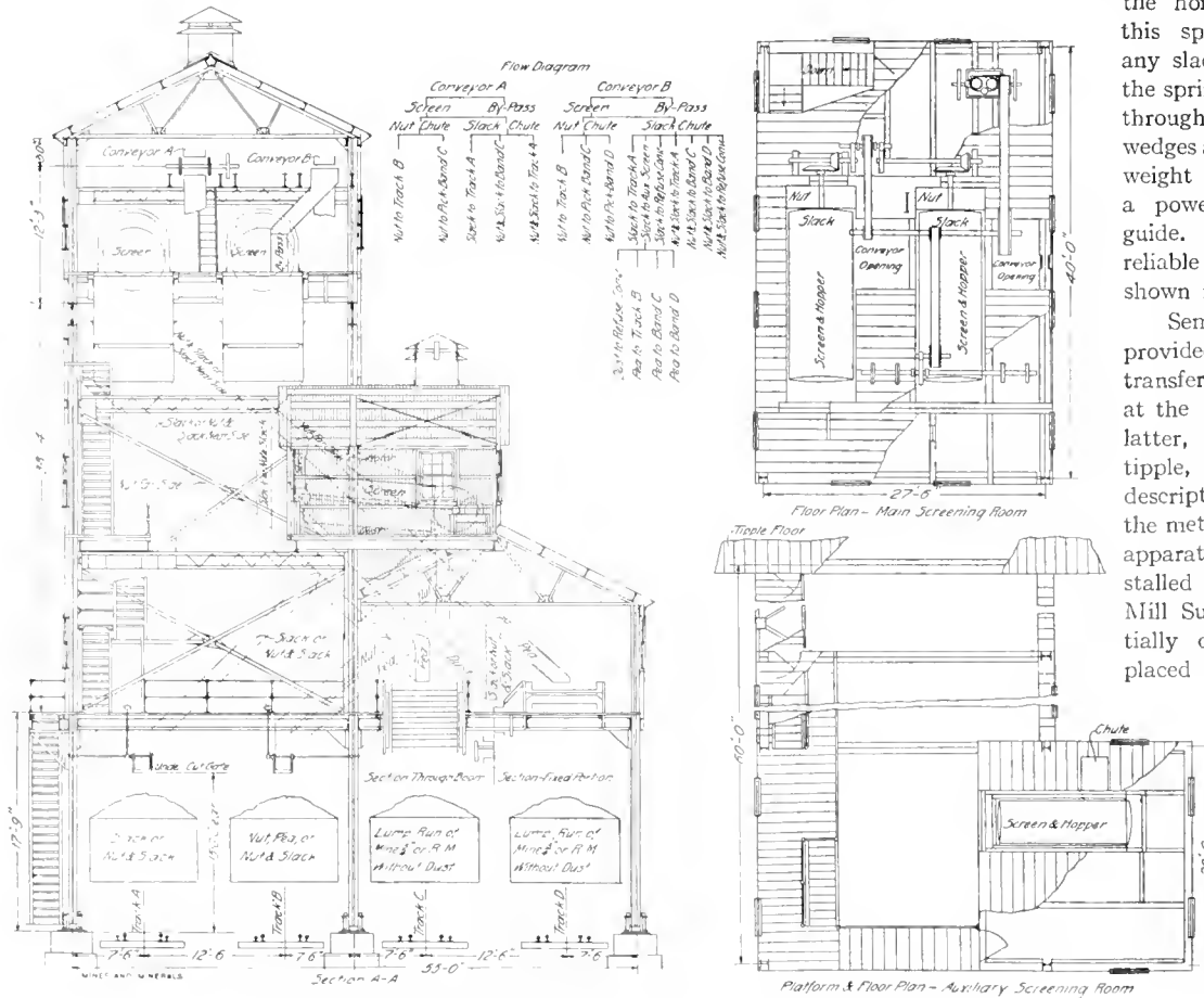
FIG. 5. PLAN, SECTIONS, AND FLOW SHEET OF TIPPLE, ANNABELLE MINE
