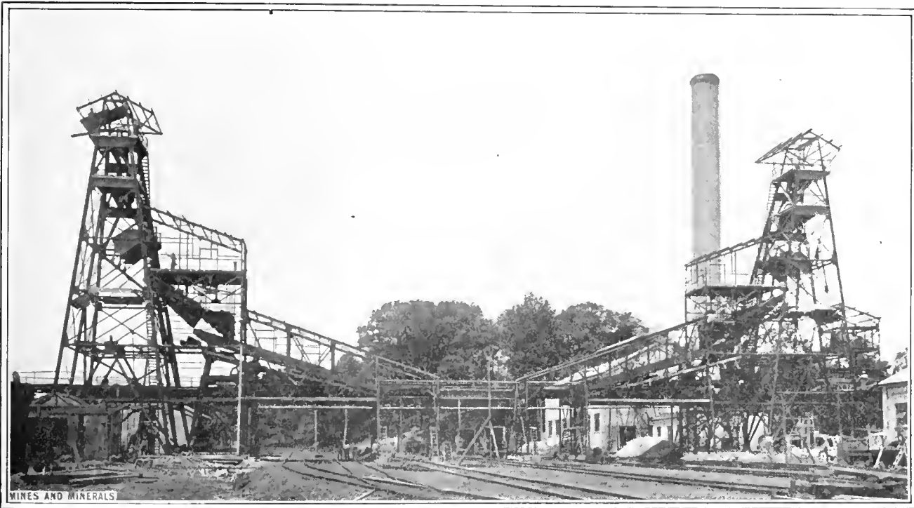
FIG. 1. TWIN TIPPLES BEFORE COVERING, UNIVERSAL MINE
