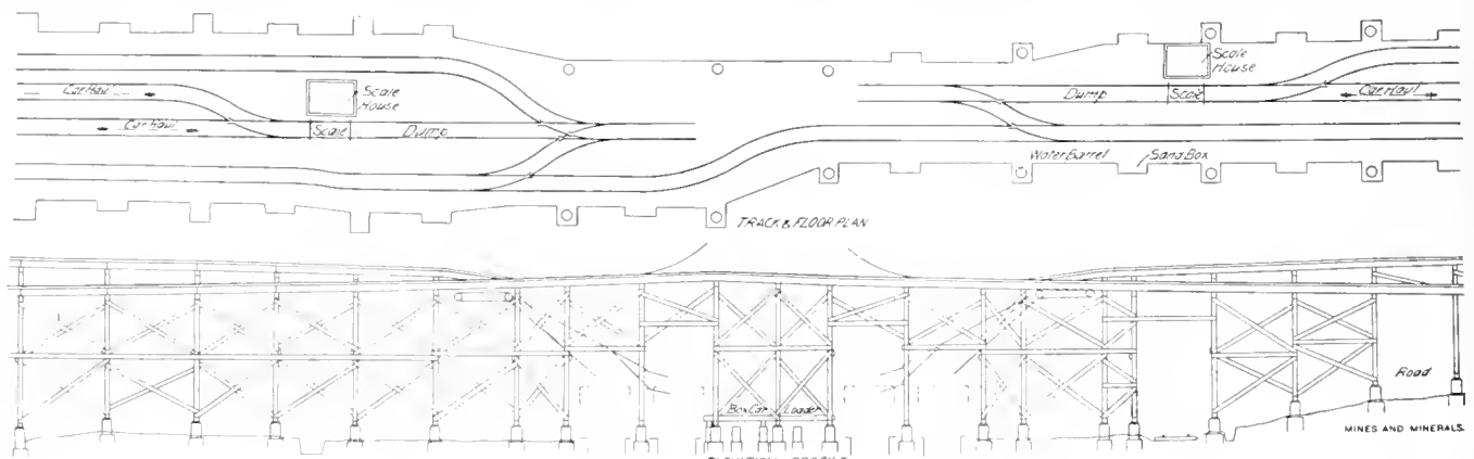
FIG. 2. PLAN AND ELEVATION OF TIPPLE AT DELAGUA MINE
