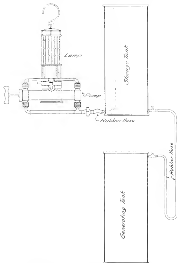
FIG. 3. GAS PUMP ARRANGED FOR EXPERIMENTS
