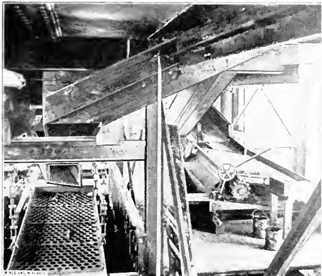
FIG. 4. SHAKING SCREEN AND SLATE PICKER
