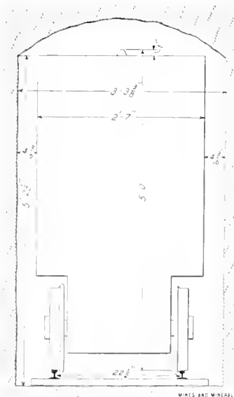
FIG. 1. CROSS-SECTION OF ADIT AND LOCOMOTIVE
