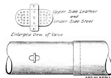
FIG. 6. PIPE LINE WITH AIR VALVE
