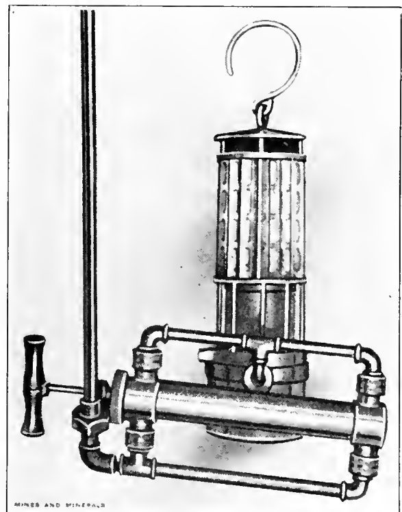
FIG. 2. GAS PUMP AND LAMP
