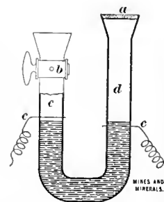
NEW FIREDAMP DETECTOR
