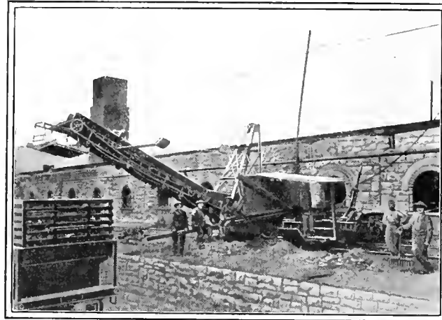
FIG. 4. ELECTRIC COKE PULLER
