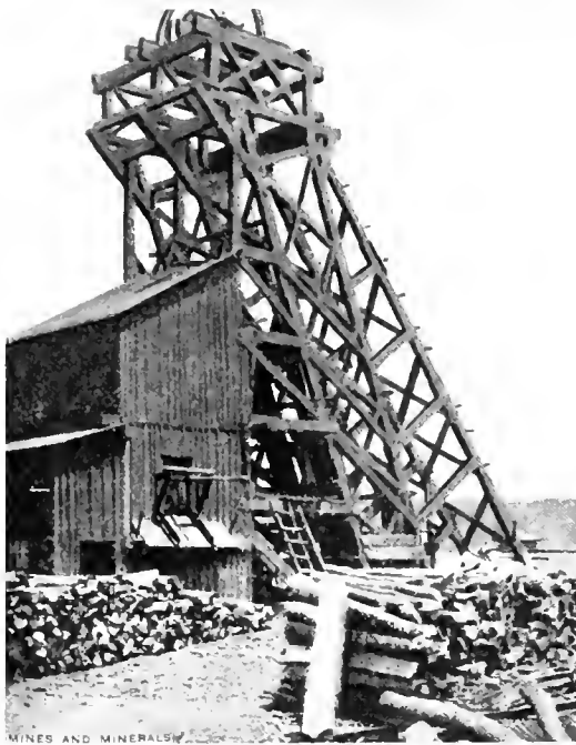
FIG. 3. HEAD-FRAME AT NO. 3 FENWICK MINE
