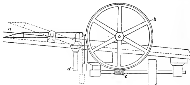
FIG. 5. HOPKINS SAMPLER
