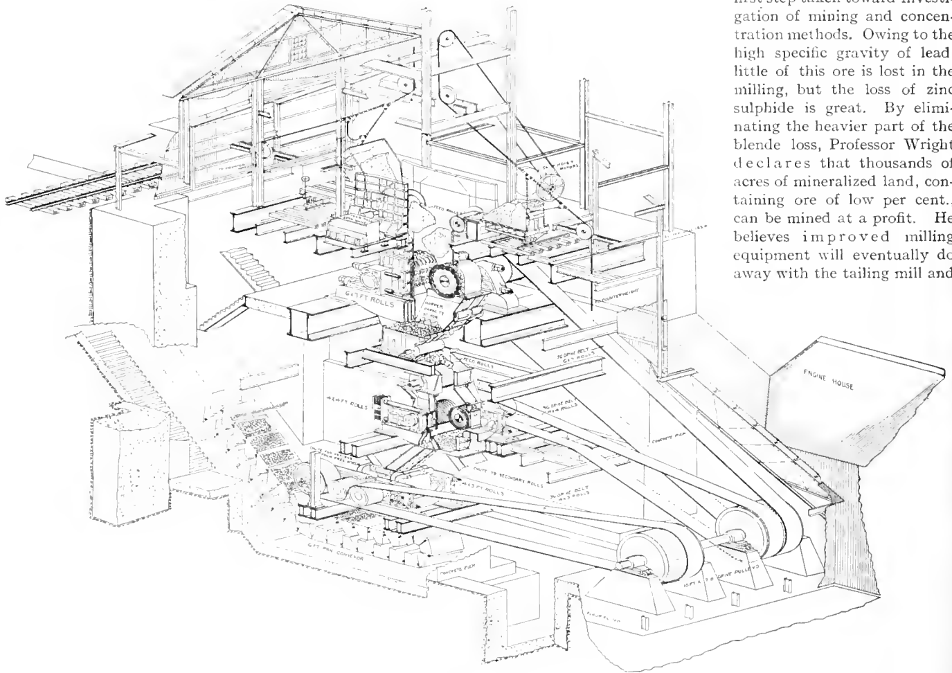
FIG. 3. TOMKINS COVE CRUSHING AND SIZING PLANT
