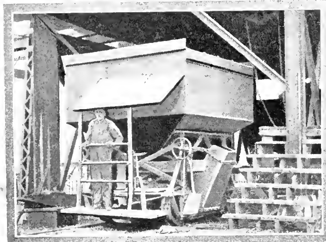
FIG. 10. GUARD FOR LARRY DRIVER
