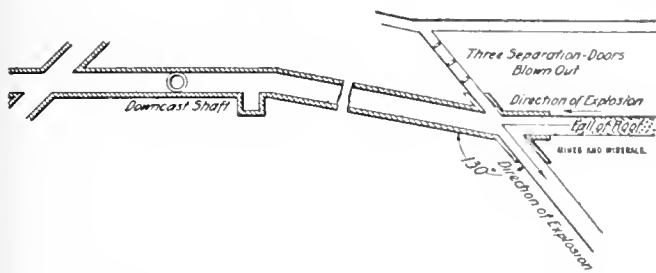
FIG. 1. PART OF WORKINGS AT BLACKWELL COLLIERY
