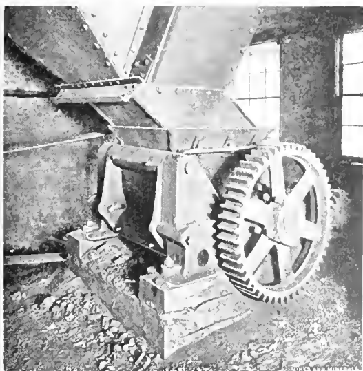
FIG. 1. SINGLE-ROLL CRUSHER
