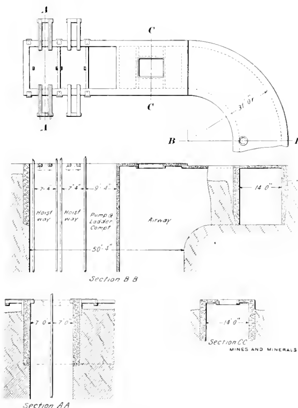
FIG. 5. PLAN AND SECTION OF AIRWAY, LOOMIS SHAFT
