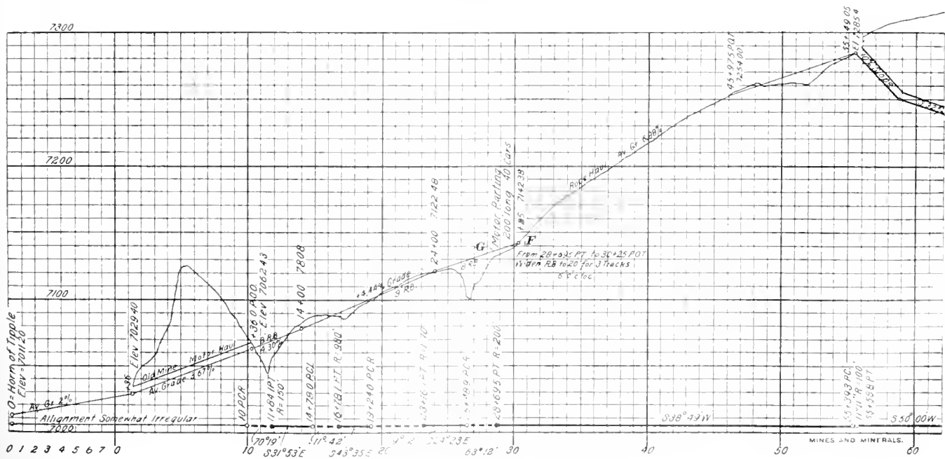
FIG. 5. ELEVATION AND Haulage GRADES
