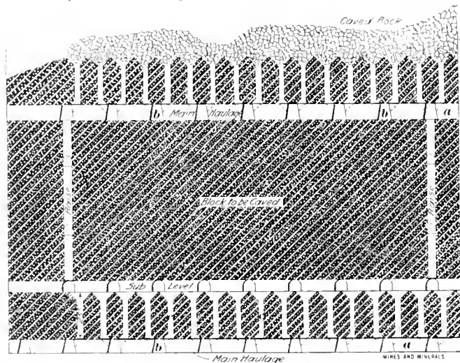
FIG. 1. LONGITUDINAL SECTION, BLOCK CAVING SYSTEM
