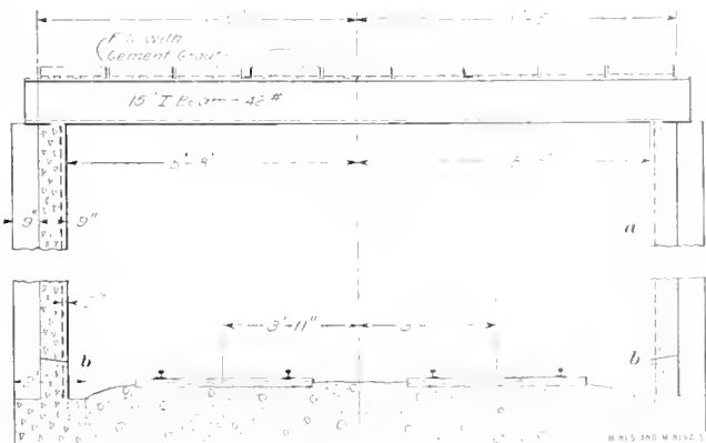
FIG. 13. SECTION OF HEADING, SHOWING CONCRETE SLAB WORK
