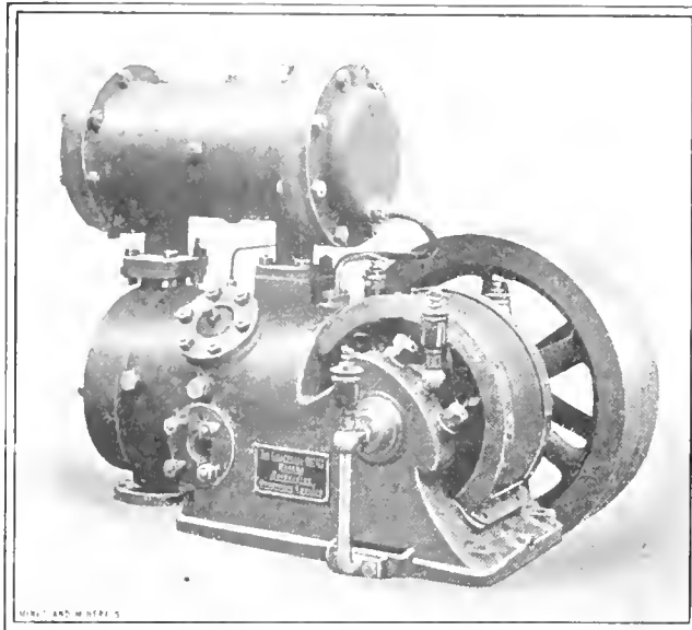
FIG. 1. SINGLE CYLINDER TWO-STAGE AIR COMPRESSOR
