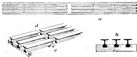
FIG. 4. RIFFLES AT STOFER PEABODY PLACER a, Plan; b, Section; c, Riffles Showing Space for Nuggets at d
