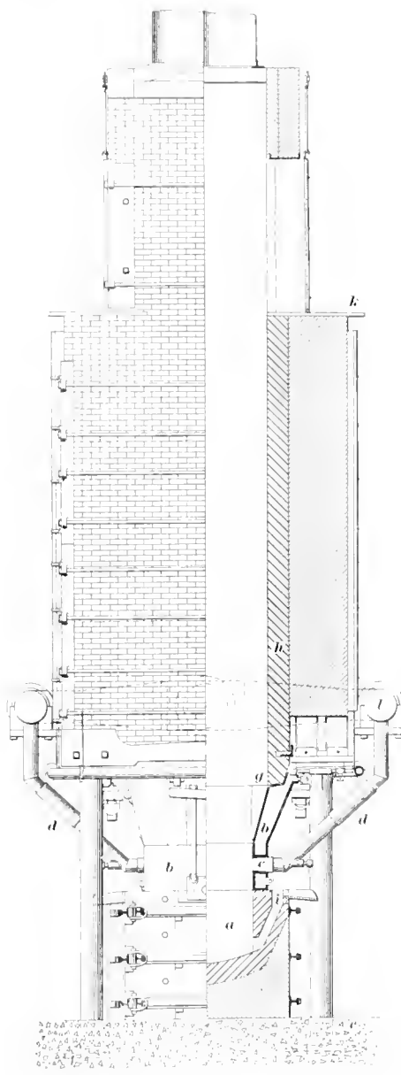
FIG. 1. LEAD SMELTING FURNACE
