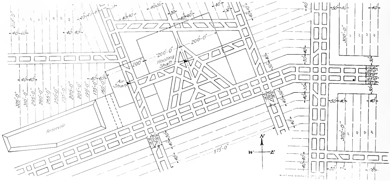
FIG. 4. DEVELOPMENT PLAN, MINE NO. 3, SALINE COUNTY COAL CO.
