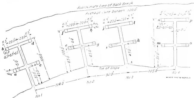
FIG. 1. PLAN OF TUNNELS FOR BLAST
