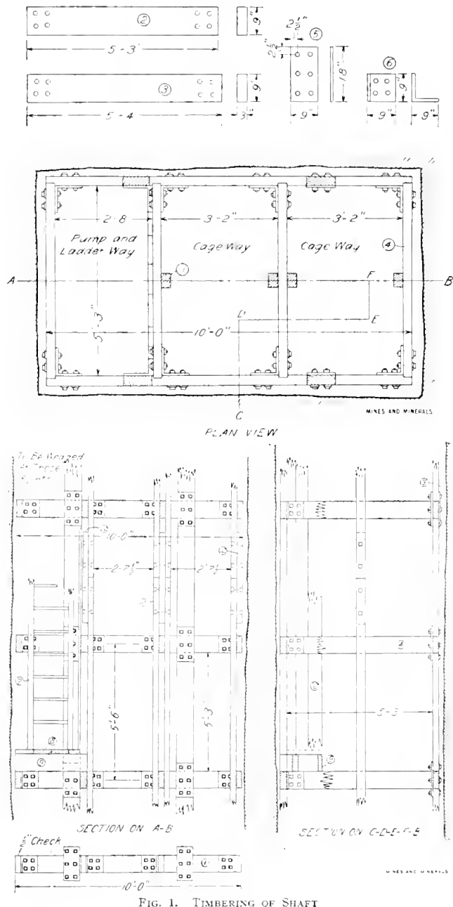
FIG. 1. TIMBERING OF SHAFT
