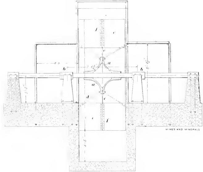
FIG. 2. SECTION THROUGH FAN
