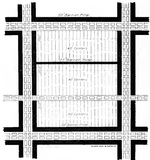
FIG. 6. METHOD OF WORKING
