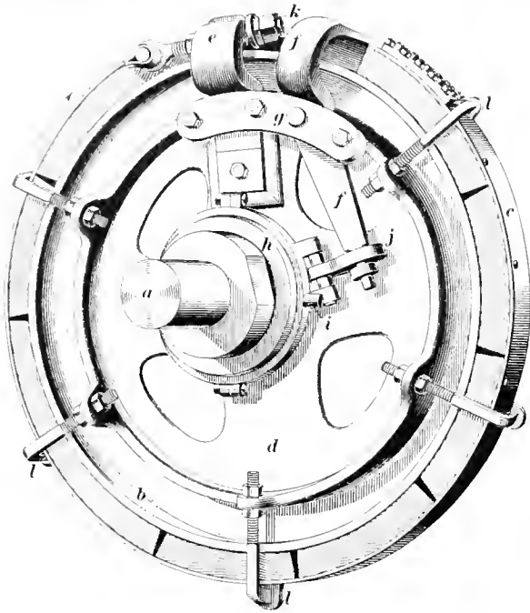
FIG. 5. BAND FRICTION CLUTCH
