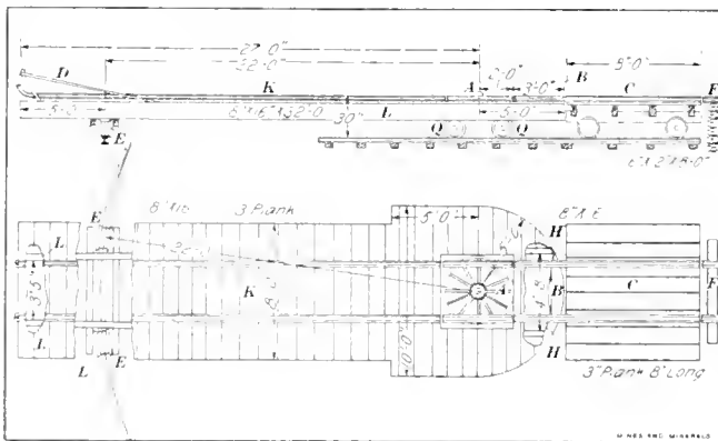
FIG. 1. SWINGING ROCK DUMP
