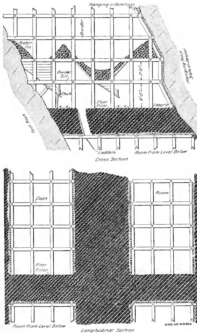
FIG. 3. VERTICAL SECTIONS SHOWING SQUARE SET TIMBERING AND SCHEME OF MINING
