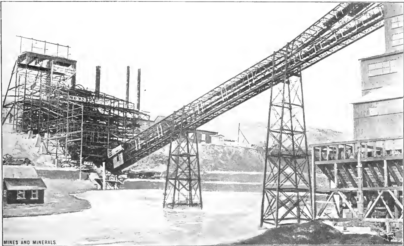
FIG. 1. HEAD-HOUSE, HEAD-FRAME AND CONVEYER AT COALDALE
