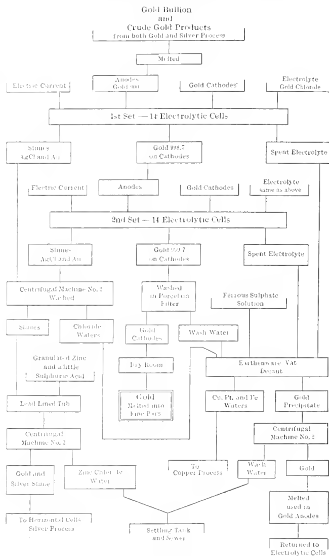
FIG. 5. DIAGRAM OF GOLD PROCESS
