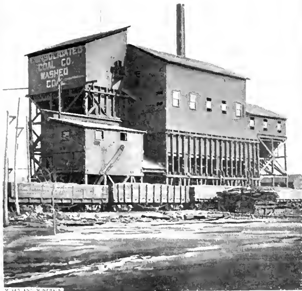
FIG. 1. COAL WASHERY, 1,000 TONS CAPACITY, SAGINAW, MICH.
