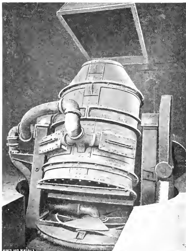
FIG. 1. OIL-FIRED CONVERTER
