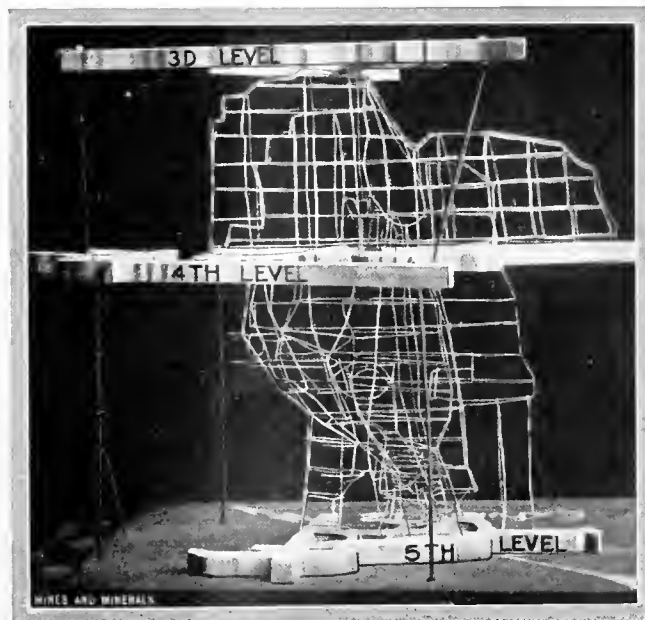
STOPE MODEL
