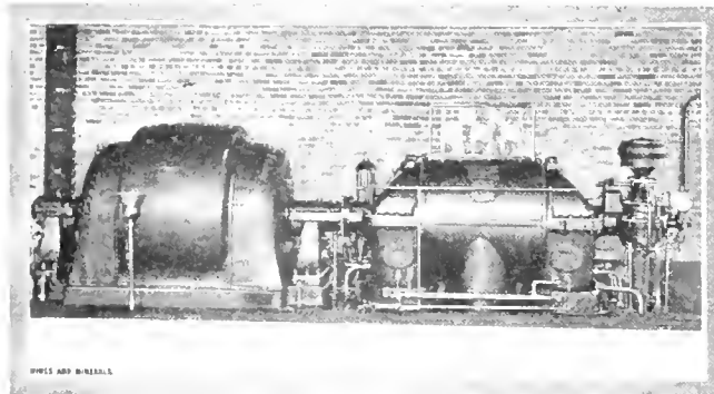
FIG. 6. LOW-PRESSURE TURBINE GENERATOR
