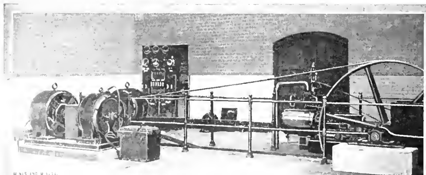
FIG. 2. MOTOR-GENERATOR SET AT CLOCK FACE COLLIERY
