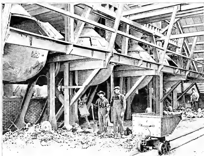
FIG. 2. DESULPHURIZING AND SINTERING FURNACES
