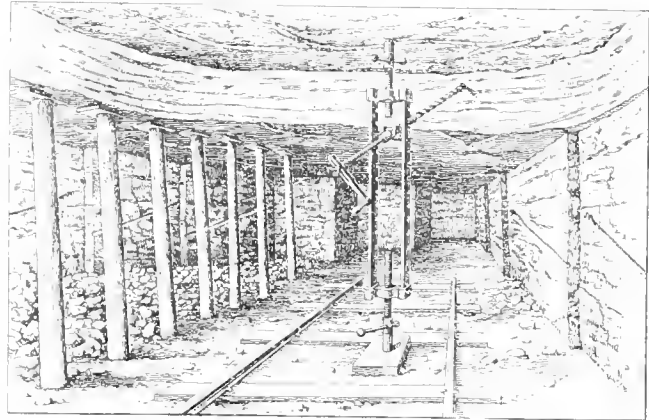
FIG. 7. BRUSHED ENTRY IN HIGHER COAL
