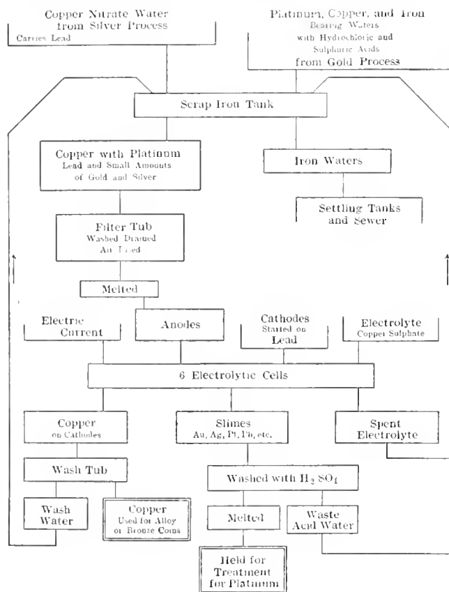
FIG. 11. DIAGRAM OF THE COPPER PROCESS
