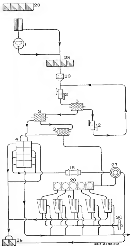
FIG. 4. FLOW SHEET
