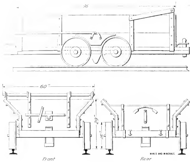
FIG. 3. MINE CAR, PENN-MARY COAL CO.
