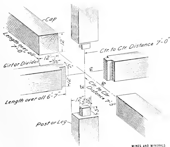
FIG. 4. SQUARE-SET JOINTS
