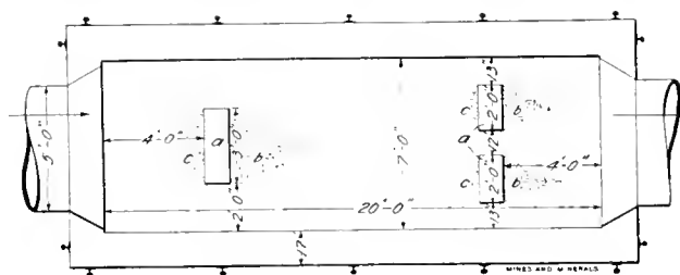
FIG. 2. PLAN OF SETTLING CHAMBER
