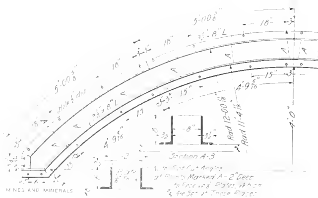
FIG. 14. STEEL FORM FOR MAKING CONCRETE BLOCK ARCH
