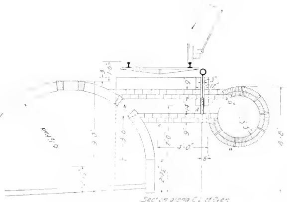
FIG. 7. SECTION OF OVEN, CONTINENTAL CORE CO
