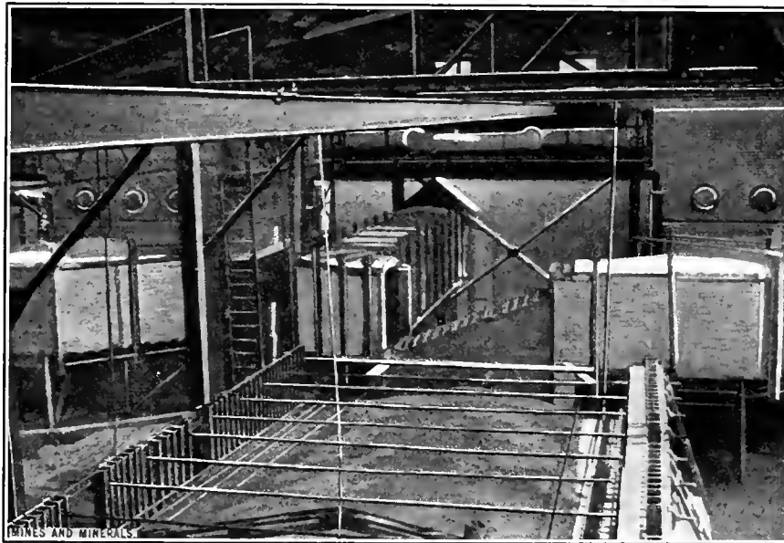
FIG. 3. TOP OF REVERBERATORY, SHOWING BRACING, WASTE HEAT BOILER, AND BY-PASS
