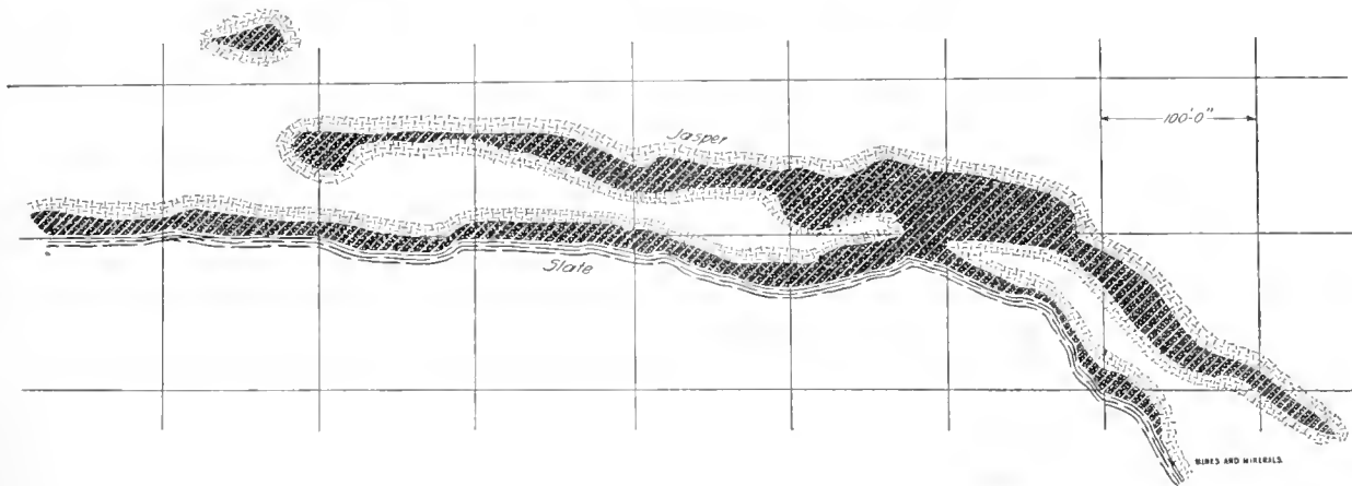
FIG. 2. PLAN, SHOWING IRREGULAR SHAPE OF ORE BODIES
