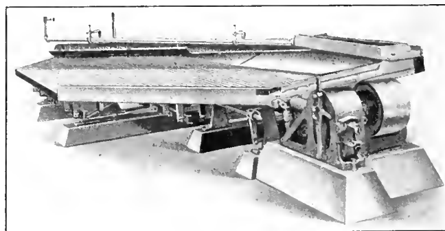
FIG. 1. DIAGONAL PLANE CONCENTRATING TABLE
