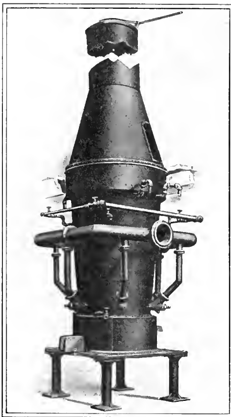
FIG. 1. ROUND COPPER FURNACE
