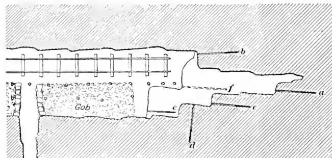
FIG. 4. PLAN OF TRIPLE-BENCH ENTRY
