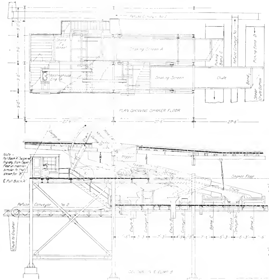
FIG 4. PLAN AND SECTION OF SCREENING FLOOR
