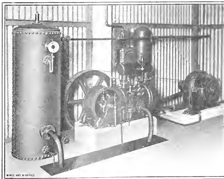
FIG. 2. ELECTRIC DRIVEN COMPRESSOR
