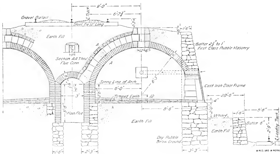
FIG. 5. CONSTRUCTION OF OVENS AND FLUE FOR UTILIZING HEAT
