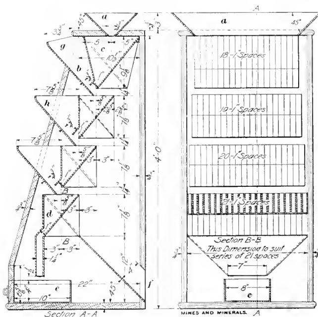
FIG. 1. LABORATORY COAL SAMPLER
