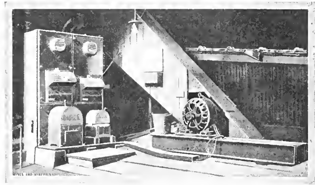
FIG. 4. PROTECTION OF MACHINERY AT CLOCK FACE COLLIERY
