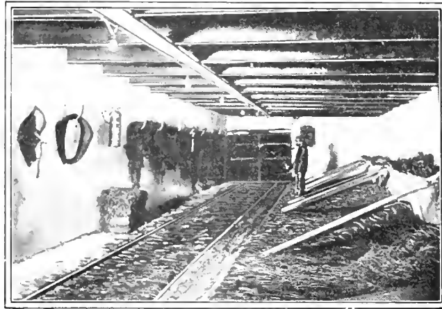
FIG. 6. UNDERGROUND STABLE, H. C. FRICK COKE CO.
