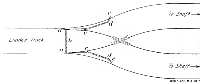
FIG. 1. AUTOMATIC SWITCH
