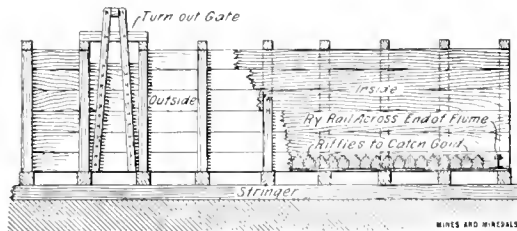
FIG. 3. SECTION OF FLUME
