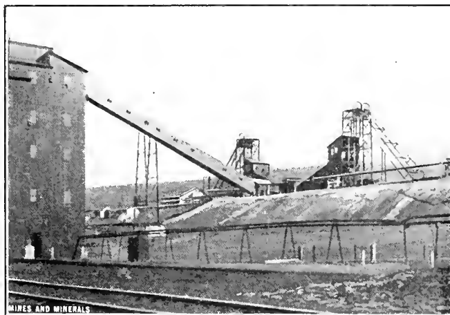
FIG. 4. TWIN SHAFTS, TRUESDALE COLLIERY
