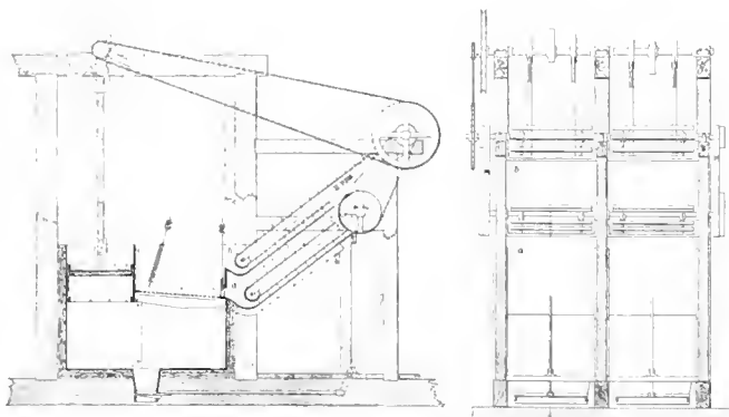
FIG. 6. LEHIGH VALLEY JIG
