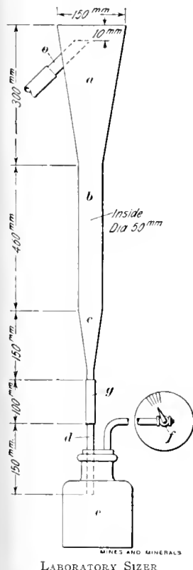
LABORATORY SIZER
