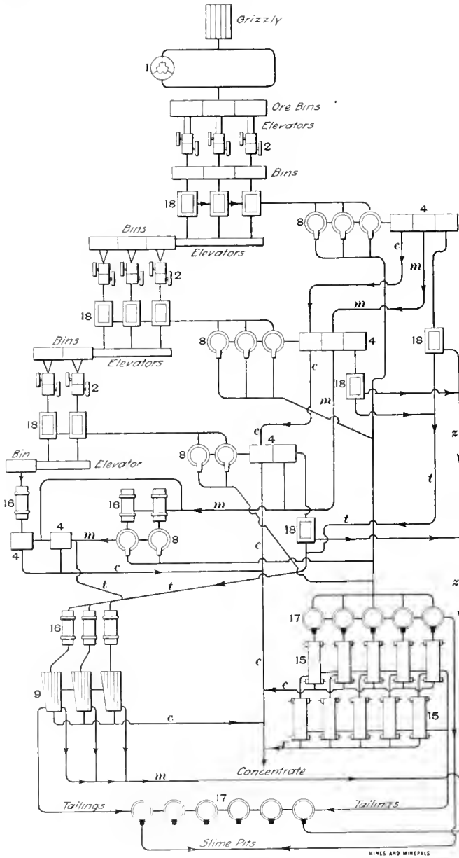
FIG. 2. BROKEN HILL PROPRIETARY COMPANY'S TREATMENT 1 crusher; 2 rolls; 4 jigs; 8 classifiers; 9 concentrating tables; 15 Frue vanners; 16 tube mill; 17 spitzkasten; 18 shaking screen; c concentrate; m middling; t tailing
