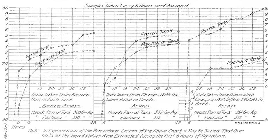
FIG. 6. RECORDS OF REGULAR OPERATIONS OF PARRAL AND PACHUCA TANKS Chemical Constituents of Solution KCN, 15 per cent.; Protective Alk. dimity, S50 Gm.; Lead, 3 Gm. Physical Condition of Pulp: Dilution 2 to 1; Specific Gravity 1.26; Screen Sizes +200, 15 to 20 per cent.; -200, 75 to 80 per cent.
