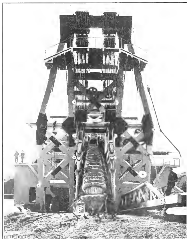
FIG. 2. FRONT VIEW OF DREDGE
