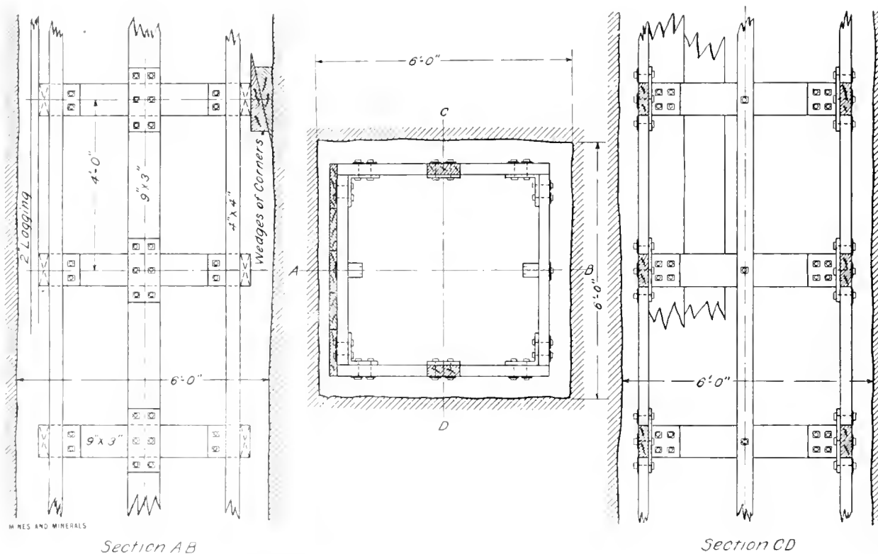
FIG. 2. METHOD OF TIMBERING FOR SMALL SINGLE COMPARTMENT SHAFT
