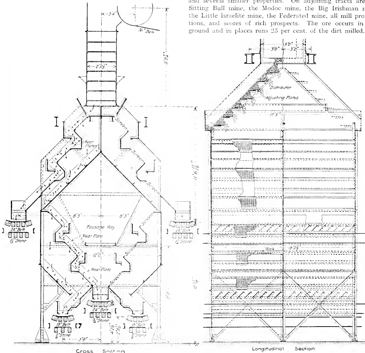
FIG. 4. DIAGRAM OF SCREENS, TOMKINS COVE PLANT
