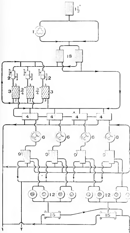
FIG. 3. BROKEN HILL SOUTH MINE PROCESS 1 crusher; 2 rolls; 3 trommel; 4 jigs; 6 grinding pans; 9 concentrating tables; 12 pulp thickeners; 15 Frue vanners; 18 shaking screen
