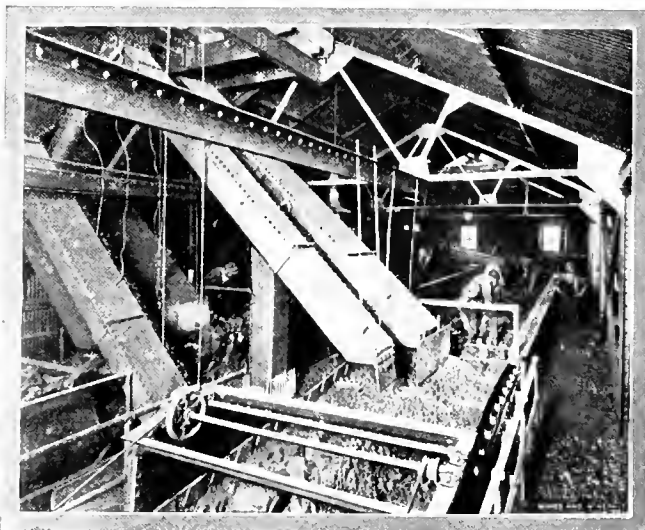
FIG. 12. CLOSED CHUTES DISCHARGING ON PICKING BAND
