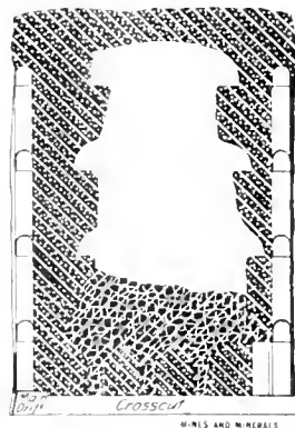
FIG. 5. CROSS-SECTION OF STOPE
