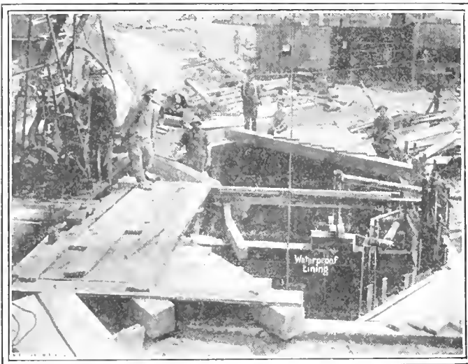
FIG. 9. WATERPROOF SHAFT LINING
