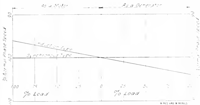
FIG. 7. SHOWING RELATION BETWEEN SPEED AND LOAD OF MOTORS OF THE INDUCTION AND THE SYNCHRONOUS TYPE
