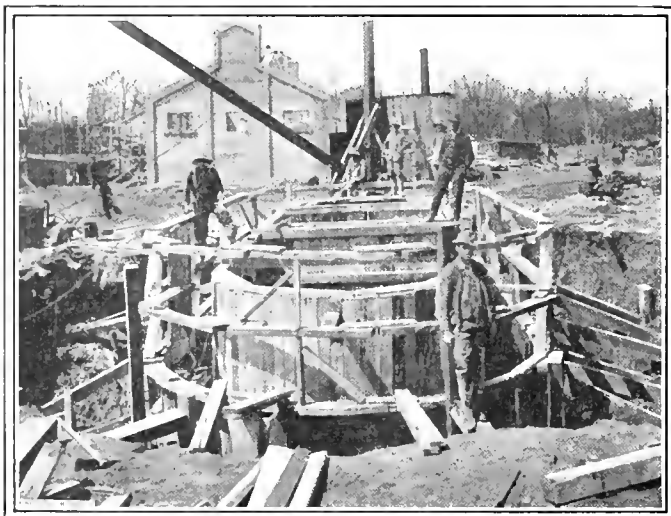
FIG. 7. FORMS IN PLACE AT VENTILATING SHAFT
