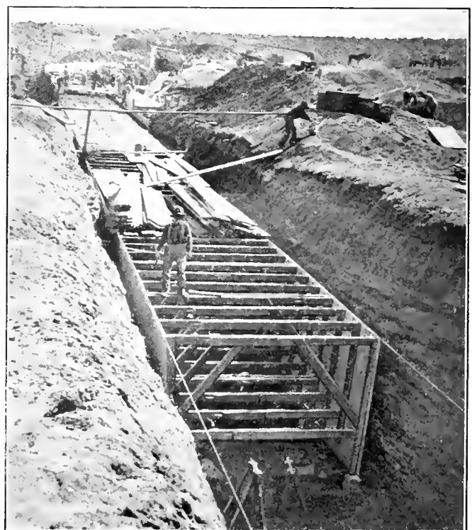
FIG. 4. CONDUIT FORM, MOJAVE DIVISION, LOS ANGELES AQUEDUCT
