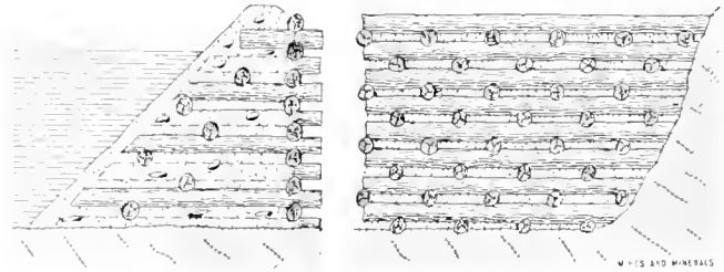
FIG. 2. MUD AND LOG DAM
