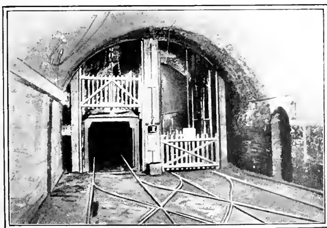
FIG. 1. CAGE AT SHAFT BOTTOM, GATE OPEN
