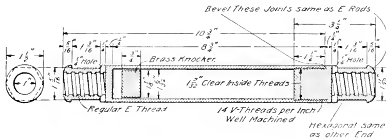
FIG. 2. PHOSPHOR BRONZE DRILL HOLE CLINOMETER
