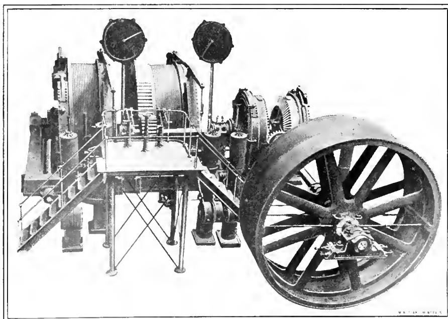
FIG. 4. ELECTRIC ROPE-DRIVE HOIST.
