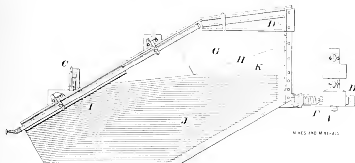
FIG. 2. PLAN OF DIAGONAL-PLANE TABLE DECK
