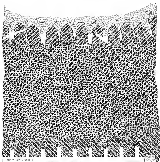
FIG. 6. CROSS-SECTION OF CAVED BLOCK
