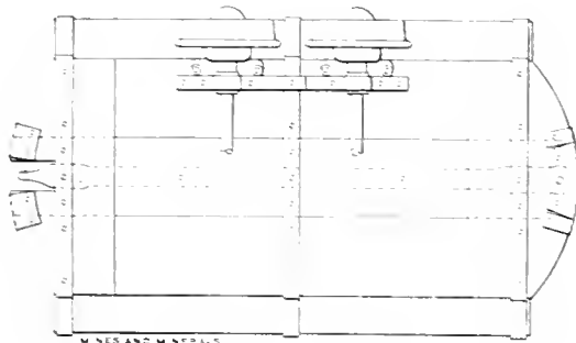
FIG. 3. CAR ADOPTED AT MINE NO. 11
