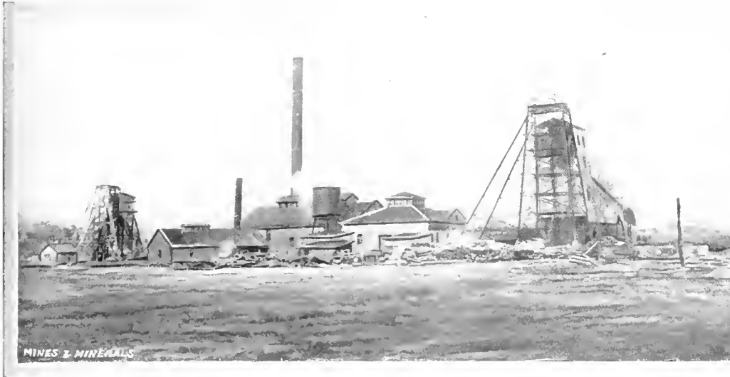
FIG. 7. SURFACE PLANT, MINE NO. 3, SALINE COUNTY COAL CO.
