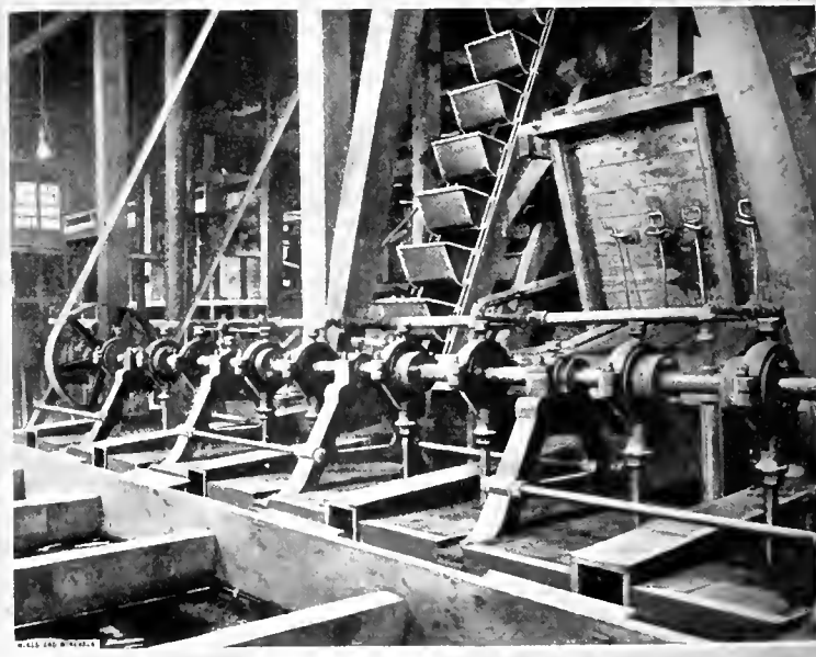
FIG. 2. LUHRIG REWASHING JIGS AND WASHED COAL ELEVATOR
