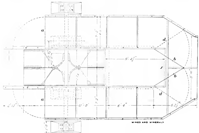
FIG. 3. REVERSING ARRANGEMENT
