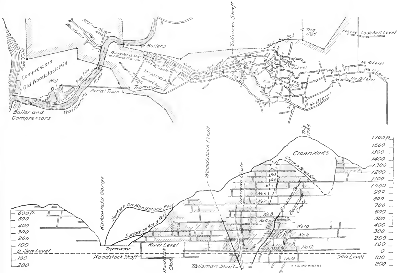
FIG. 1. PLAN AND VERTICAL PROJECTION OF PART OF TALISMAN MINE
