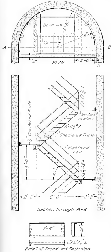
FIG. 4. STEEL STAIRWAY IN SHAFT
