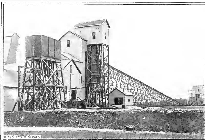
FIG. 4. ZINC MINE HOISTING ORE FROM TWO SHAFTS
