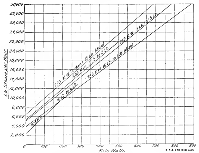
FIG. 10. RELATIVE EXHAUST STEAM CONSUMPTIONS OF DIFFERENT SIZES OF MIXED PRESSURE IMPULSE TURBINES
