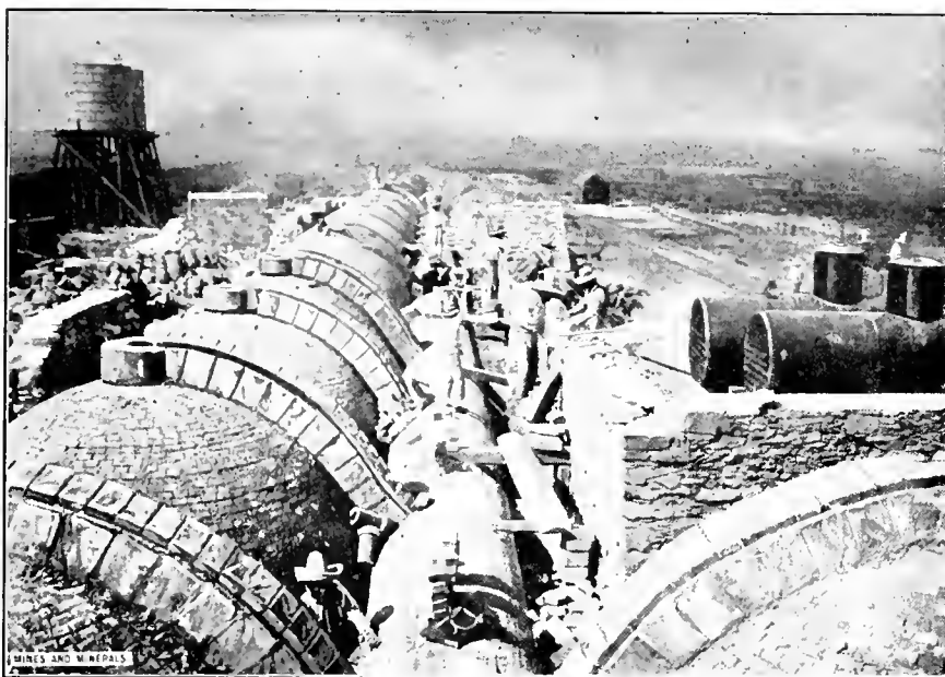
FIG. 6. OVENS AND WASTE-HEAT FLUE UNDER CONSTRUCTION, MEXICO
