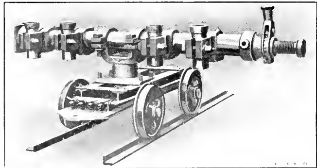
FIG. 2. CARRIAGE FOR FOUR DRILLS
