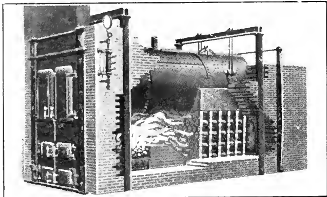
FIG. 1. FURNACE GAS CONSUMER ON RETURN TUBULAR BOILER
