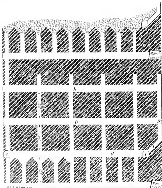
FIG. 2. CROSS-SECTION OF END OF BLOCK
