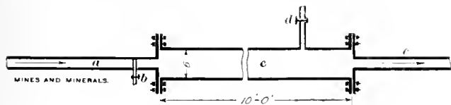
FIG. 1. JAMES WATER BLAST
