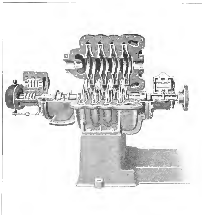
FIG. 1. DOUBLE-SUCTION TURBINE PUMP, CASING OPEN
