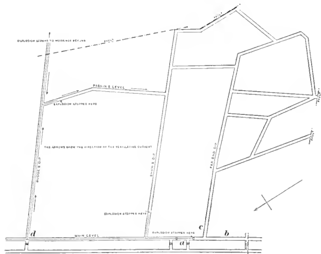
FIG. 2. PART OF WORKINGS OF TALK-O'-TH'-HILL COLLIERY
