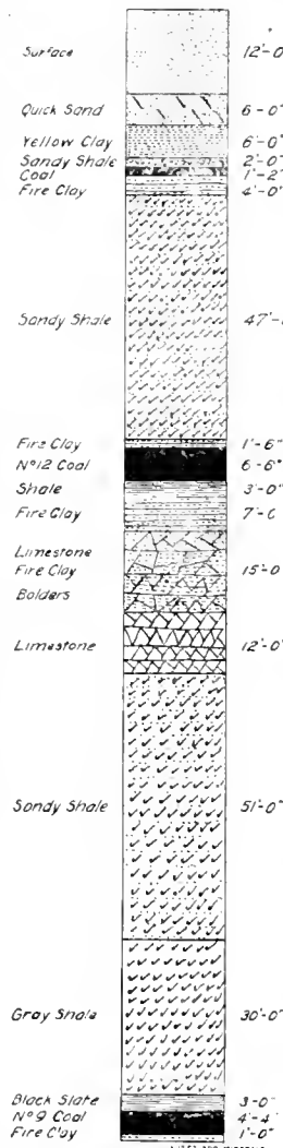
FIG. 2. SECTION
