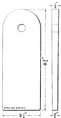
FIG. 6. DIMENSIONS OF ANODES
