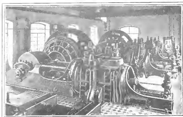
FIG. 3. TWO TWIN TANDEM GAS ENGINES AT MICHEVILLE, FRANCE
