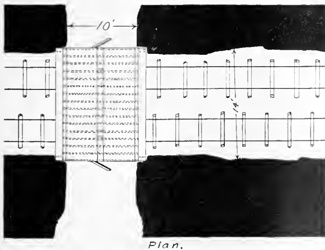
FIG. 1. PROTECTED OVERCAST WITH LIGHT WALLS
