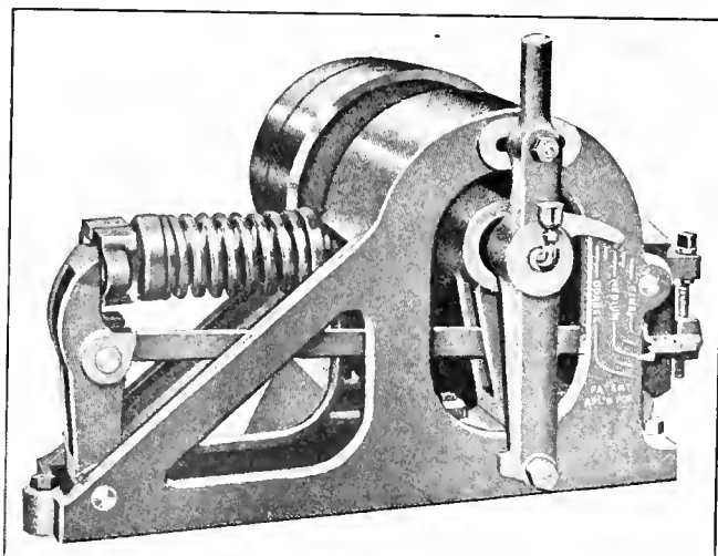
FIG. 3. HEAD MOTION OF DIAGONAL-PLANE TABLE
