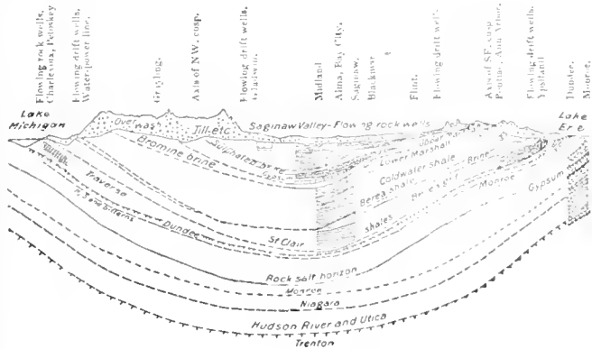
FIG. 2. CROSS SECTION, LOWER MICHIGAN BASIN
