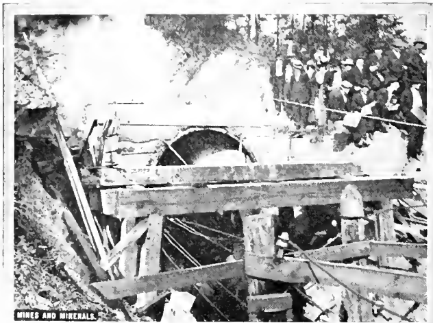
FIG. 4. EMERGENCY FAN AFTER ACCIDENT
