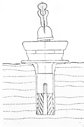
FIG. 4. BENDING OF STUD ON CLAMP DUE TO CLAMP NOT BEING SCREWED UP TIGHT AGAINST THE HANGER
