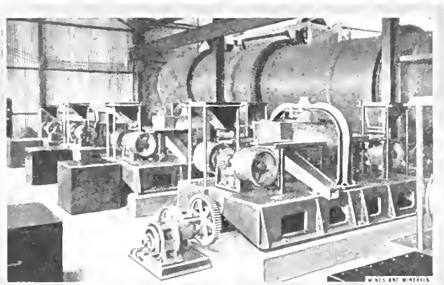
FIG. 3. MAGNETIC SEPARATING PLANT
