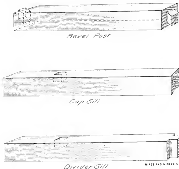
FIG. 5. DETAILS OF MEMBERS
