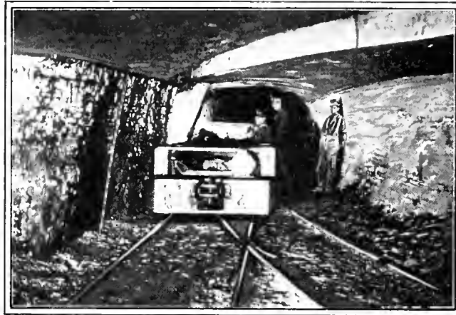
FIG. 3. PROTECTION OF TROLLEY WIRE
