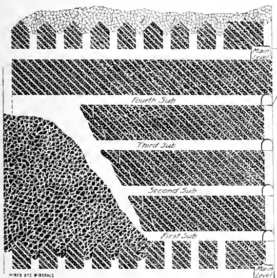
FIG. 4. LONGITUDINAL SECTION OF SUBSTOPPING
