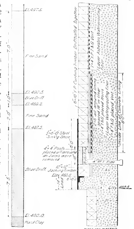
FIG. 11. PLACING OF WATERPROOF LINING
