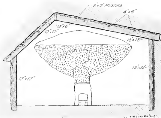
FIG. 2. METHOD OF EXCAVATING PUMP ROOM
