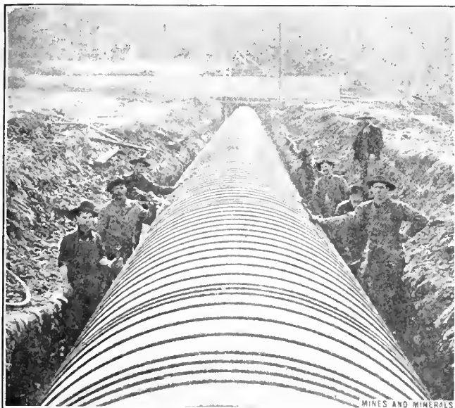
FIG. 2. WOODEN-STAVE PIPE, 56 INCHES DIAMETER
