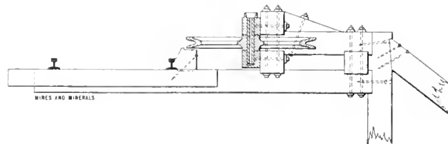
ROPE SHEAVE
