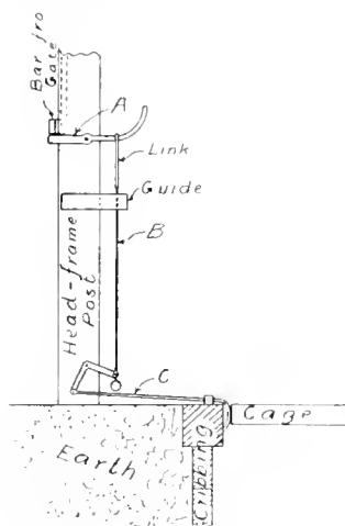
FIG. 1. LOCKING DEVICE FOR SAFETY GATE
