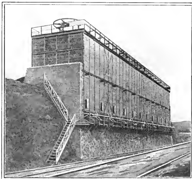
FIG. 2. UNLOADING STATION AND ORE BIN AT LA HIJATE
