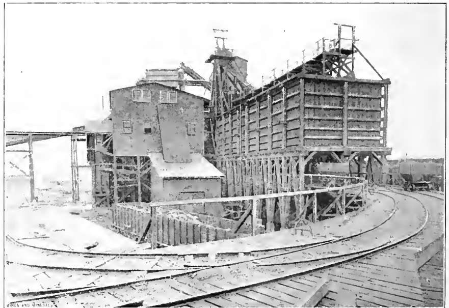
FIG. 4. END VIEW OF SODDY PLANT, SHOWING SLACK BINS, ENGINE ROOM AND WASHER BUILDING
