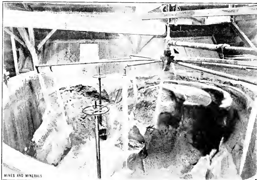
FIG. 1. AUTOMATIC SLUICER FOR SAND TANKS
