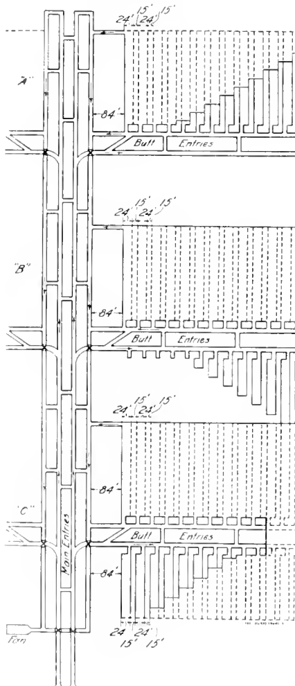
FIG. 1. METHOD OF MINING
