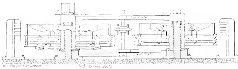
FIG. 1. LONGITUDINAL SECTION OF ROPE SHEAVE
