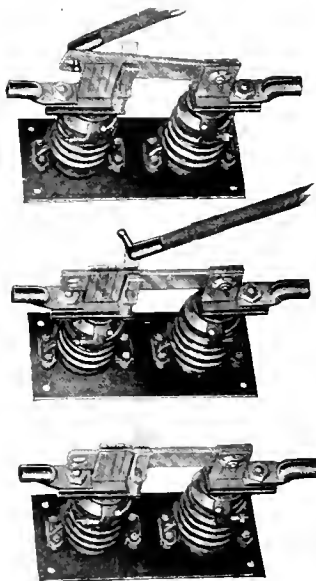
LOCKING DEVICE FOR SWITCHES
