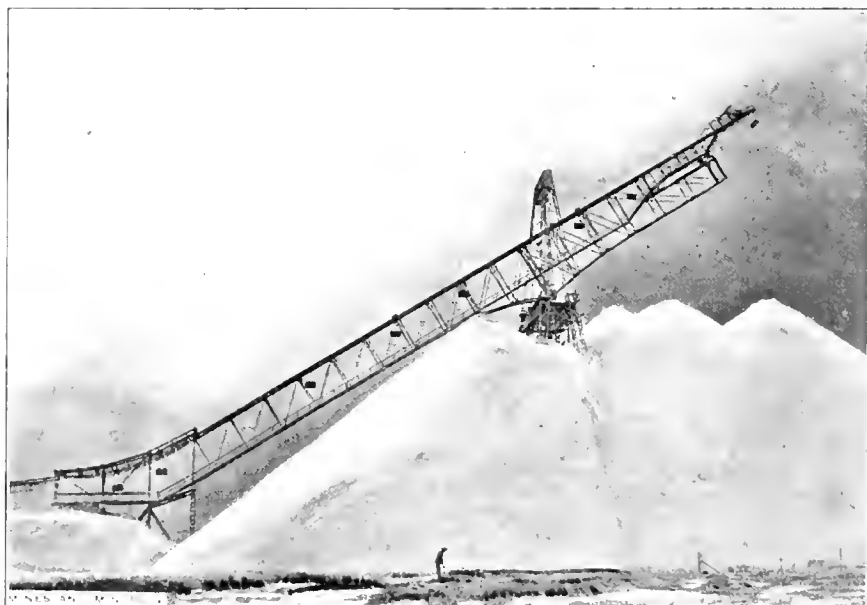
FIG. 4. AERIAL SAND DUMP
