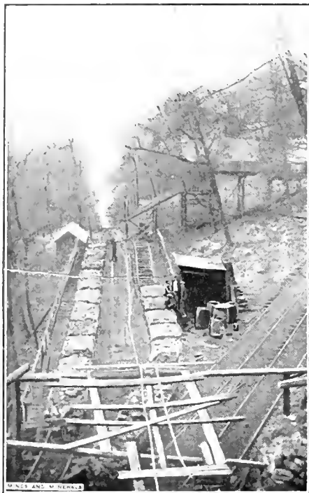
FIG. 3. UPPER TIPPLE, ORME, TENN.
