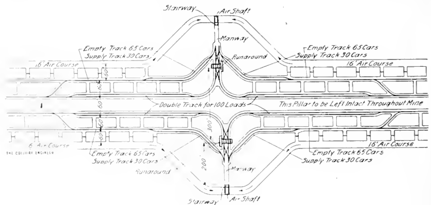
FIG. 6. PLAN OF SHAFT BOTTOM
