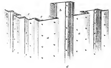
FIG. 4. CHANNEL BAR PILING
