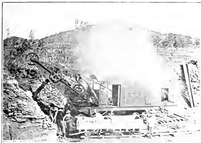
FIG. 1. STEAM SHOVEL STRIPPING, WASP NO. 2
