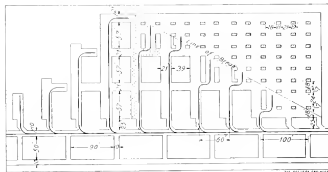
FIG. 2. EXTRACTING PILLARS WHEN THERE IS NO DRAW-SLATE
