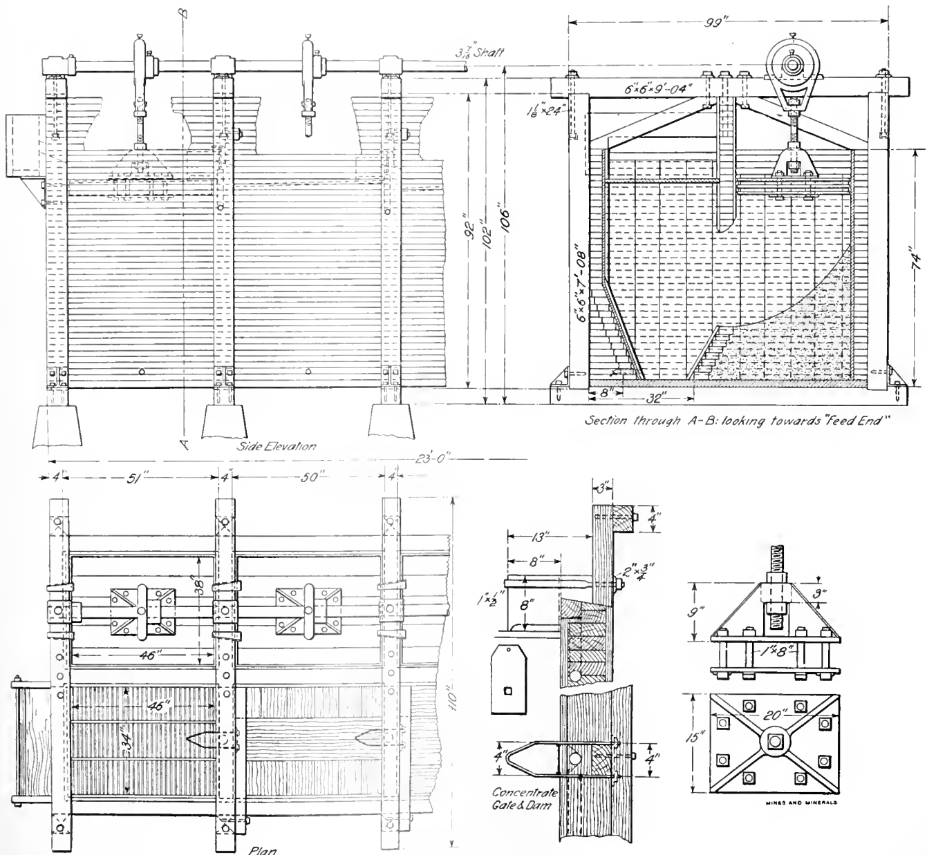
FIG. 2. ROUGHER JIG
