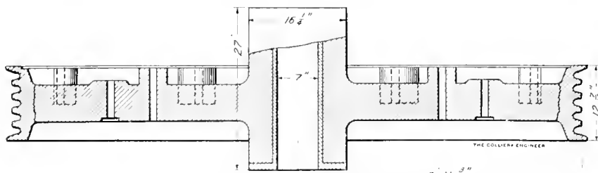
Cross Section of Rear Wheel FIG. 4. SHOWING BRACES
