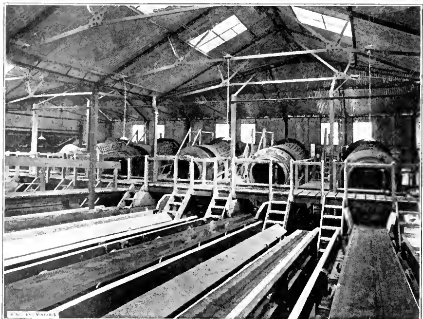
FIG. 2. TROMMELS AND SORTING BELTS
