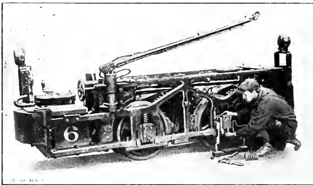
FIG. 1. LOCOMOTIVE SHOWING REMOVABLE GIB
