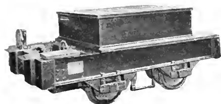
FIG. 1. STORAGE-BATTERY LOCOMOTIVE
