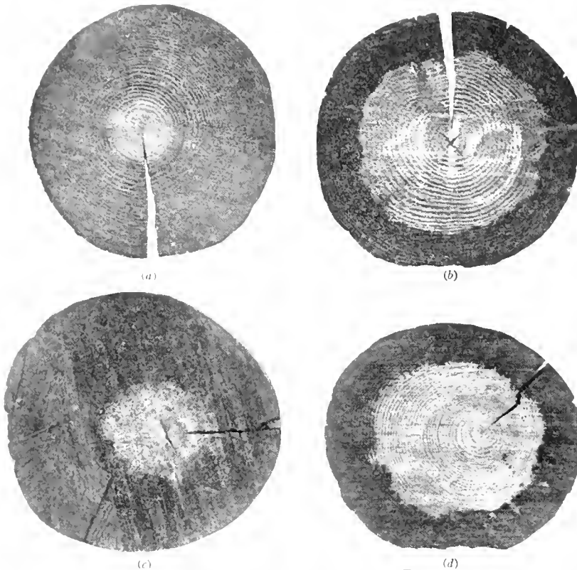
FIG. 3. SECTIONS FROM ROUND TIMBER AFTER TREATMENT
