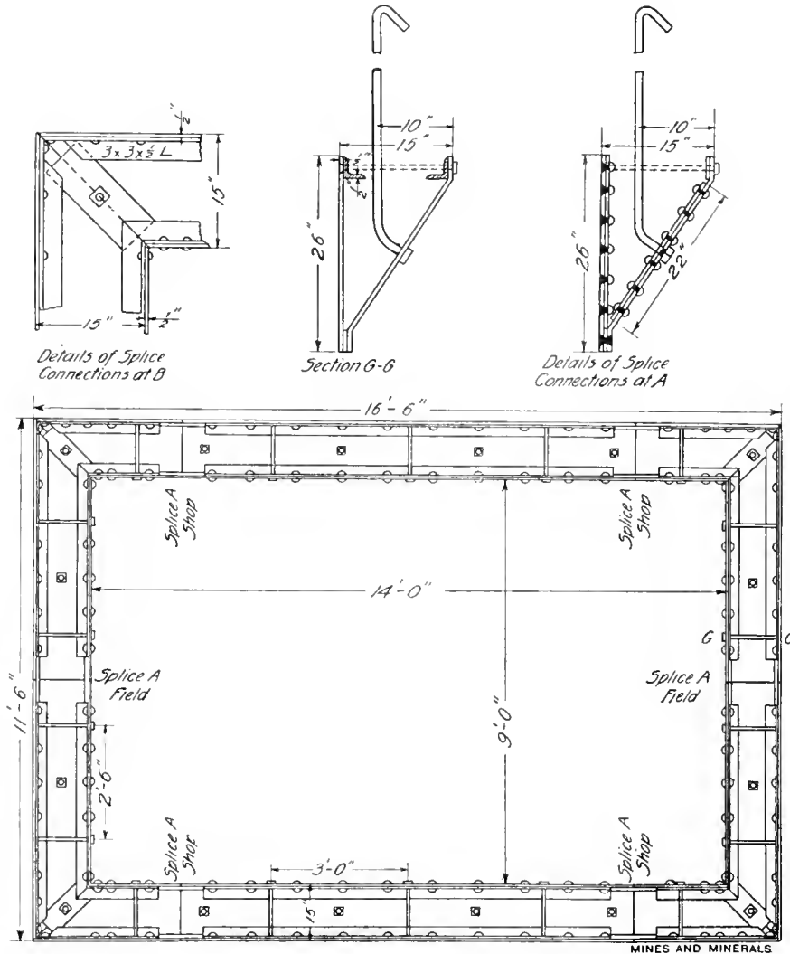
FIG. 1. PLAN AND DETAILS OF STEEL SHOE
