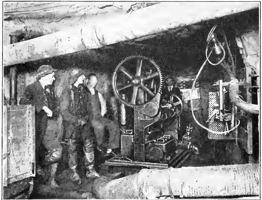
FIG. 1. GOULDS' TRIPLEX PUMP USED UNDERGROUND ON CATSKILL AQUEDUCT
