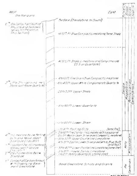
FIG. 4. GEOLOGICAL SECTION, MAGDALENA MINING DISTRICT
