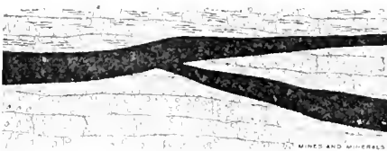
FIG. 3. SPLIT IN COAL SEAM
