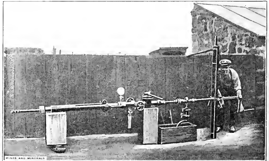
VIEW OF HORIZONTAL BORING AND TAPPING MACHINE
