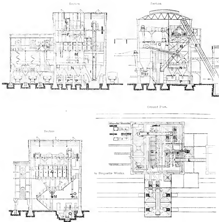
FIG. 2 COAL WASHERY
