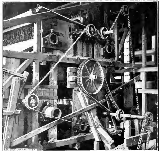
FIG. 2. DRIVING GEAR OF LANGERFELD SEPARATOR
