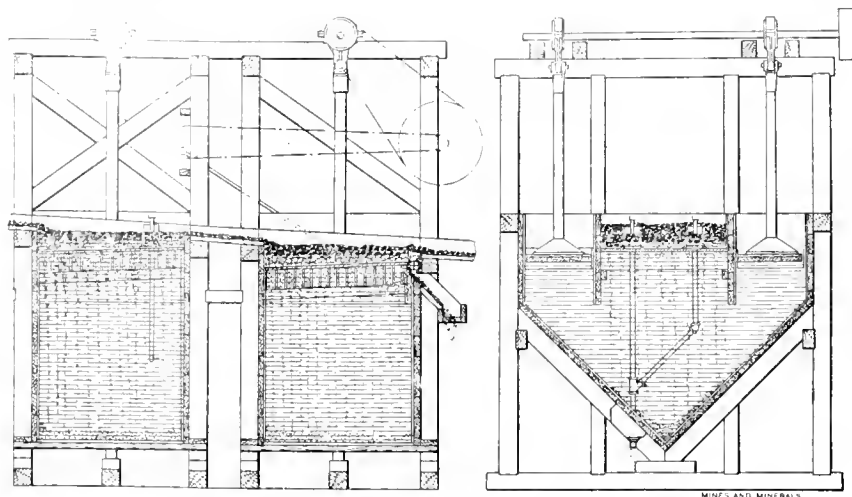
FIG. 5. SECTIONS SHOWING TWO COMPARTMENTS OF ROBERTS & SCHAEFER CO.'S JIGS
