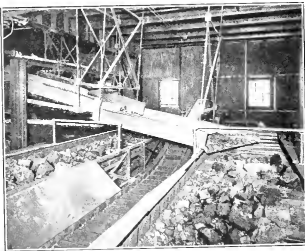
SHAKING SCREENS DISCHARGING ONTO PICKING BAND
