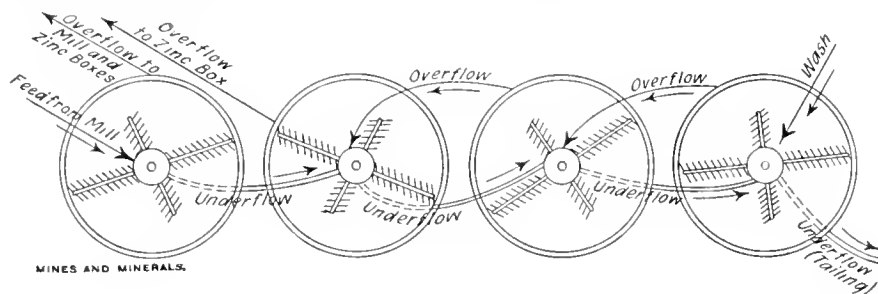
FIG. 2. THICKENERS IN SERIES
