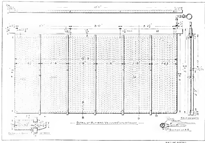
FIG. 5. BUTTERS VACUUM FILTER FRAME
