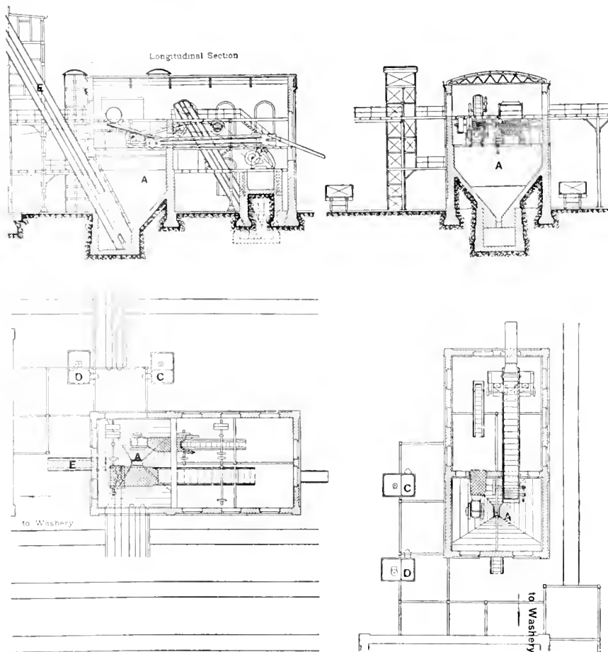
FIG. 1. SCREENING AND CRUSHING PLANT
