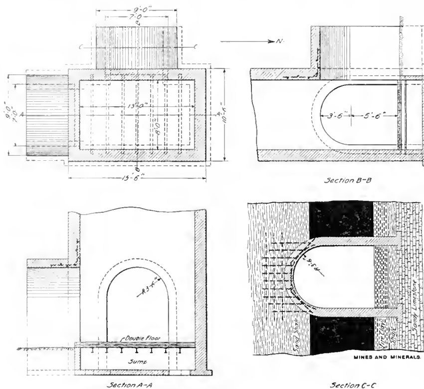
FIG. 2. CONSTRUCTION AT SHAFT BOTTOM
