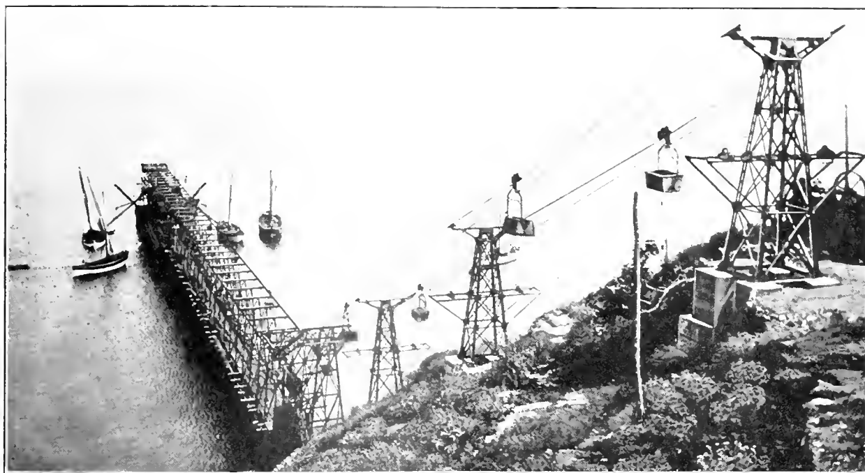
FIG. 1. LOADING PIER IN THE SEA, RIO ALBANO MINE, ISLAND OF ELBA
