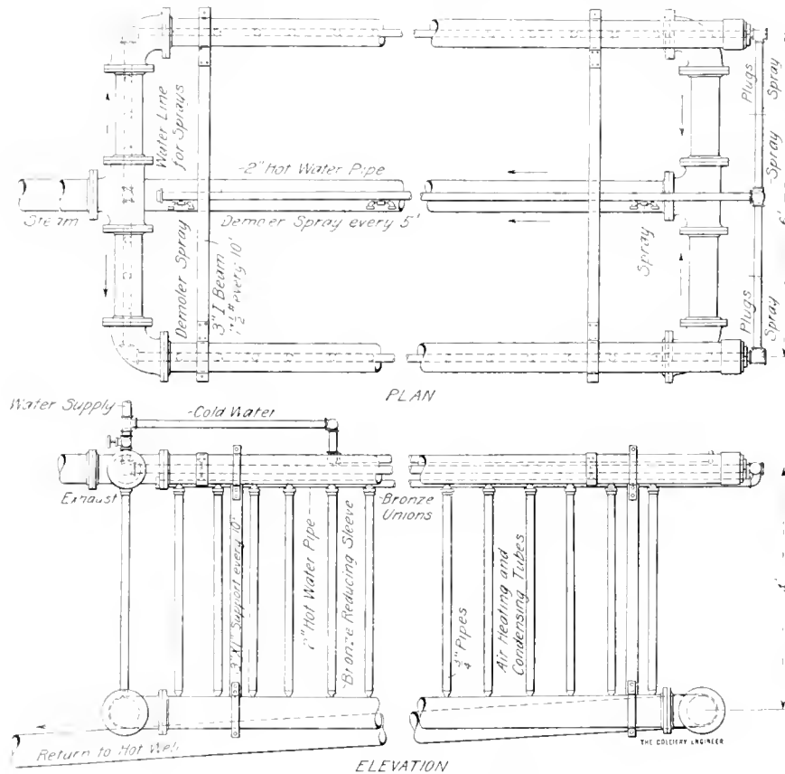
FIG. 1. HUMIDIFYING APPARATUS
