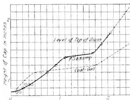
FIG. 3 PERCENTAGE OF INFLAMMABLE GAS
