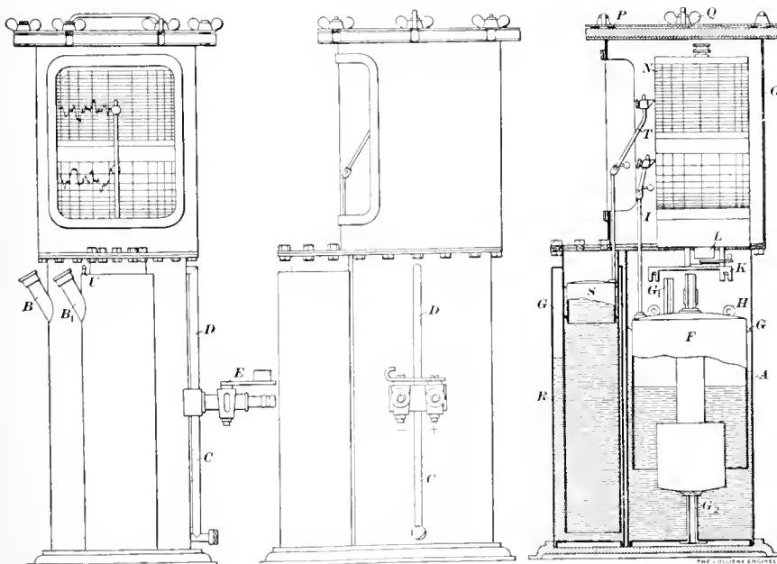
FIG. 1. FACTUM AIR METER AND VOLUME RECORDER
