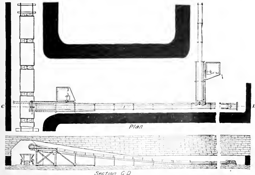
FIG. 3. ARRANGEMENT OF CONVEYER
