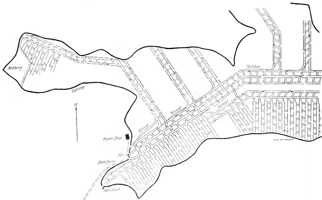
FIG. 2. METHOD OF MINING, LATHROP COAL CO.
