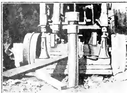
FIG. 3. BRACING FOR FRONT OF DERRICK
