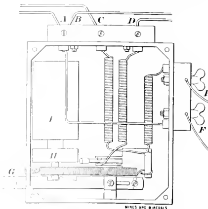
FIG. 2. INTERIOR OF SPARKER BOX
