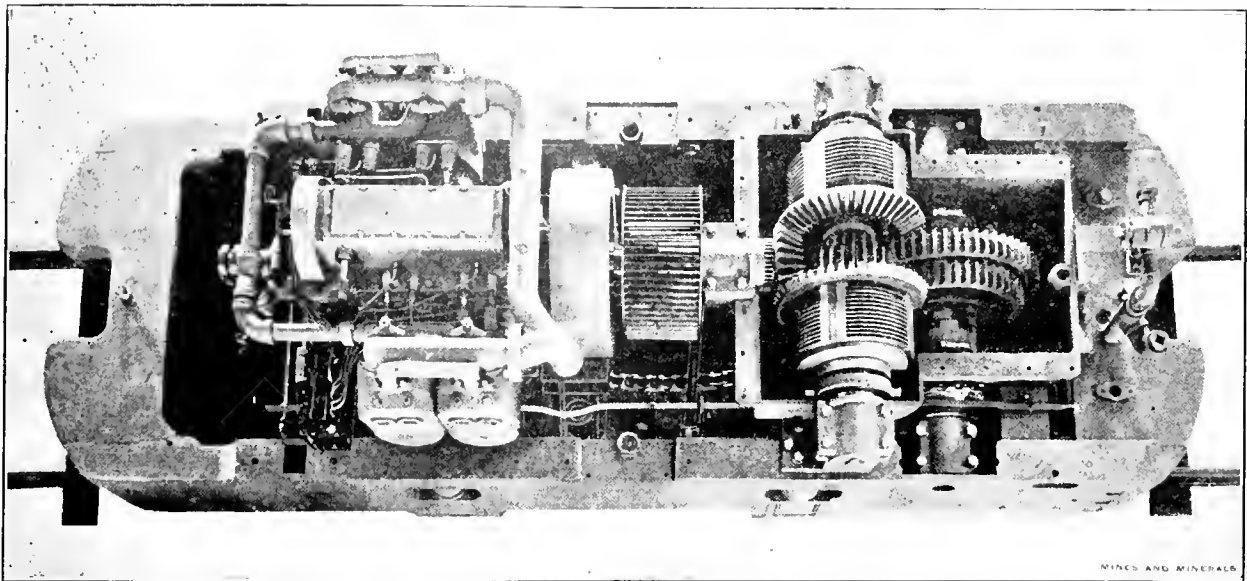
FIG. 1. TOP VIEW OF GASOLINE LOCOMOTIVE, STRIPPED
