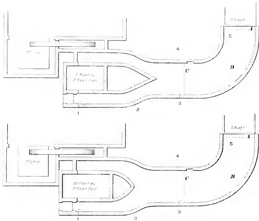
FIG. 2. CONNECTIONS OF FANS AND FAN DRIFTS WITH THE SHAFT
