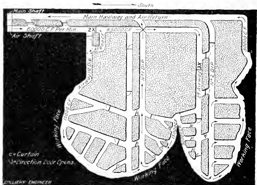
FIG. 2. INSTALLATION OF A BOOSTER FAN
