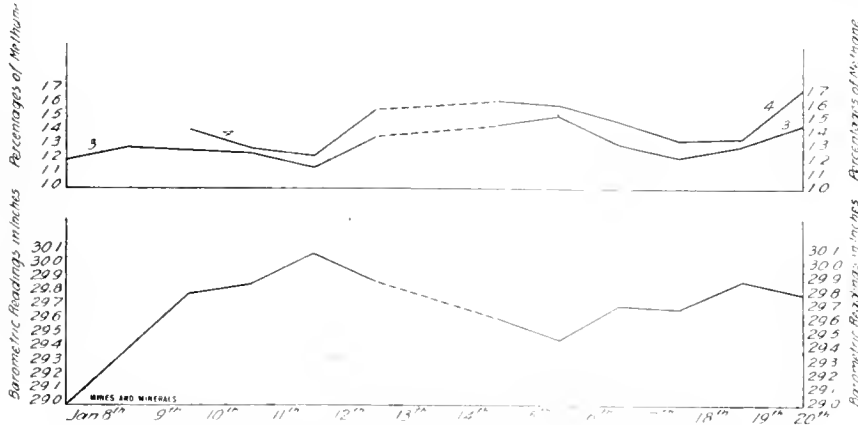
FIG. 2. INFLUENCE OF BAROMETRIC PRESSURE ON PERCENTAGE OF METHANE
