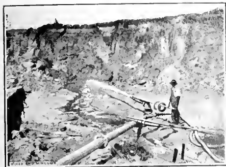
FIG. 5. HYDRAULIC NOZZLE
