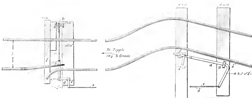
FIG. 2. DETAILS OF DERAILING SWITCH
