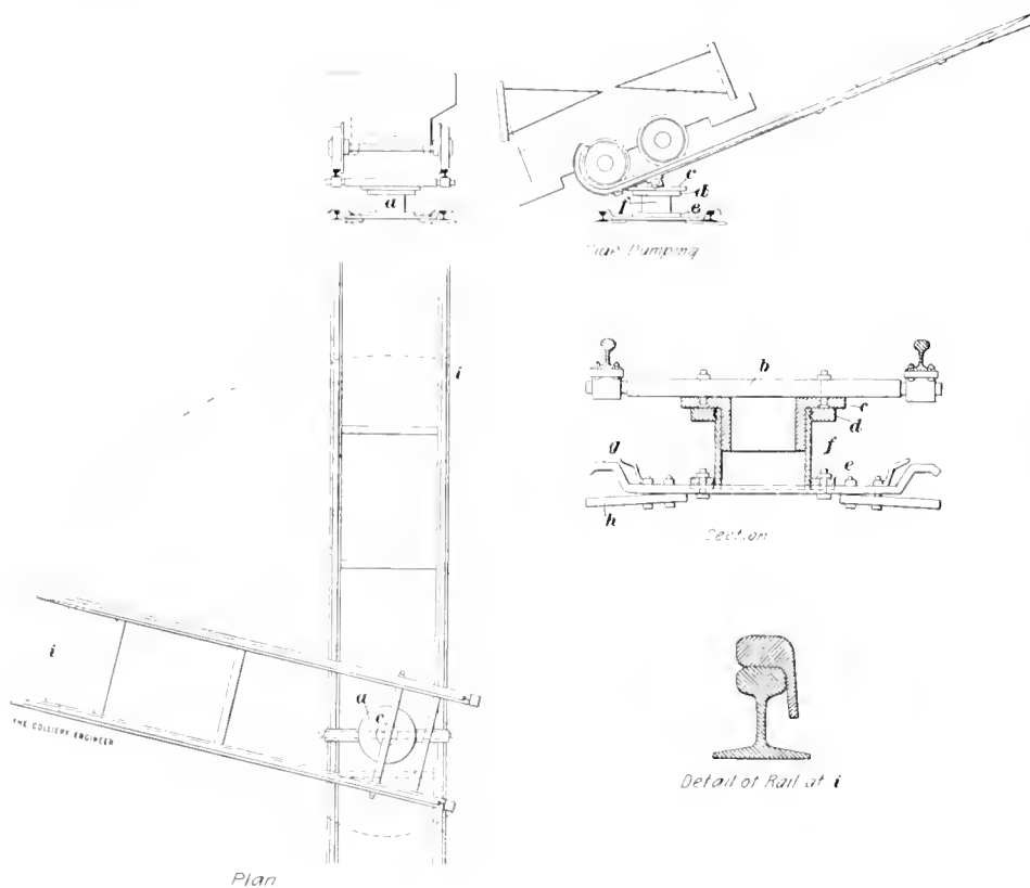
FIG. 1. ROCK DUMP FOR SLOPE
