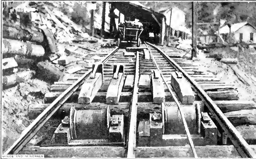
FIG. 1. AUTOMATIC SAFETY BLOCKS AT HEAD OF PLANE
