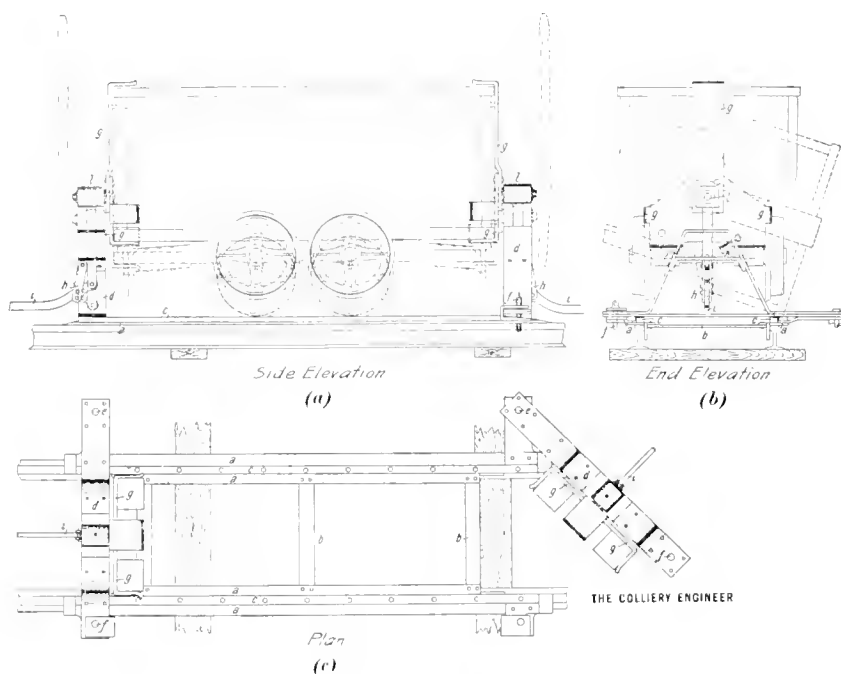
FIG. 1. DUMPER FOR MINE CARS
