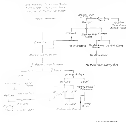
FIG. 2. FLOW SHEET, SODDY WASHER
