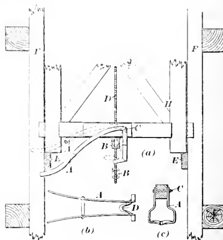
FIG. 2. SARGESON CROSSHEAD
