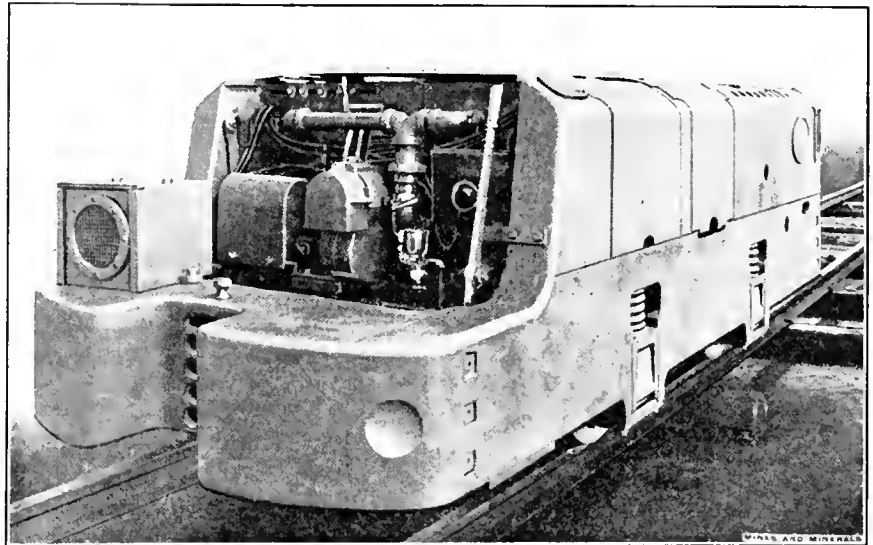
FIG. 3. REAR VIEW OF GASOLINE LOCOMOTIVE, CARBURETER ALONGSIDE BRAKE LEVER
