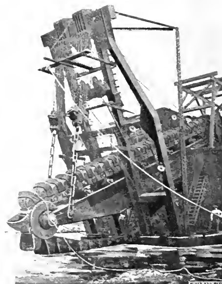
FIG. 3. LOWER TUMBLER AND BUCKET LINE, 13-FOOT DREDGE
