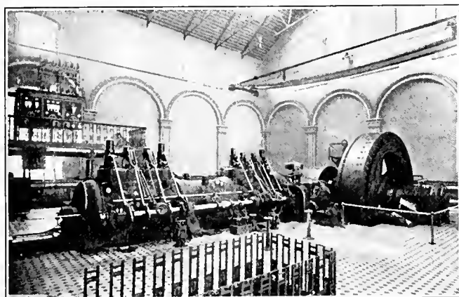
FIG. 1. TANDEM GAS ENGINES AT BARGOED COLLIERY
