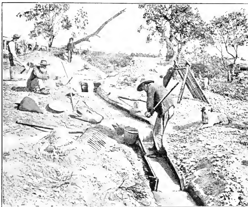
FIG. 1. TIN SLUICING
