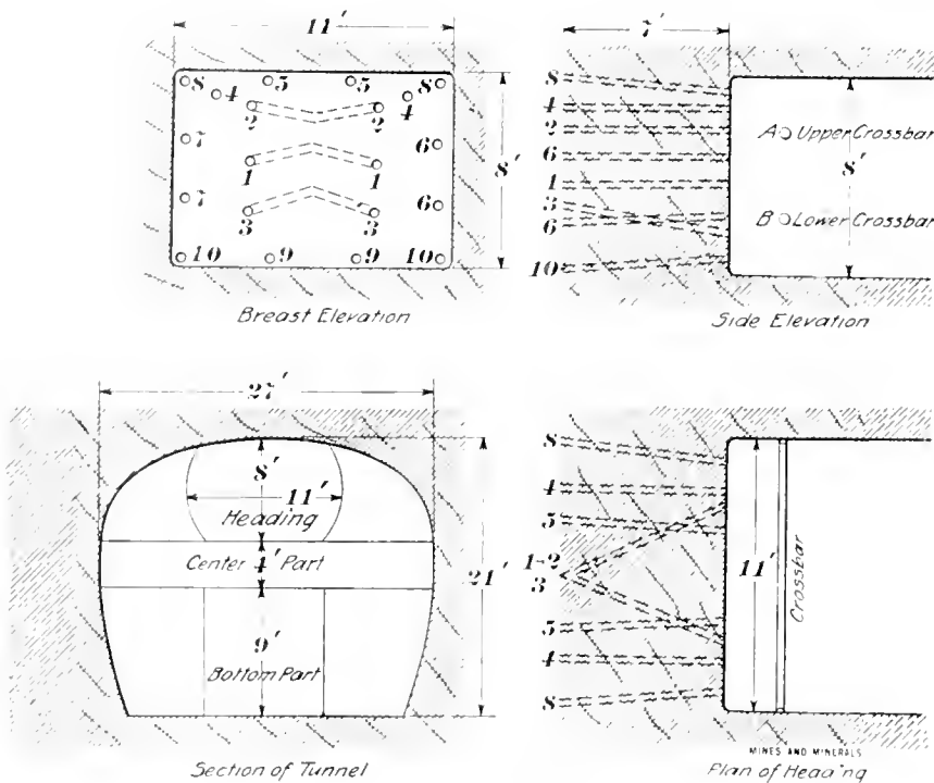
FIG. 1. METHOD OF DRIVING TUNNEL
