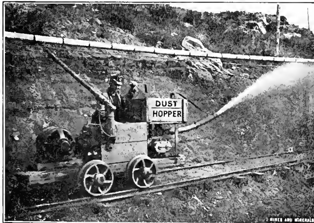
FIG. 6. DUST-BLOWING MACHINE
