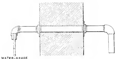
FIG. 3. FORM OF PITOT TUBE
