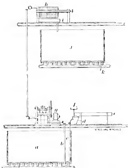
FIG. 5. MERRILL PRECIPITATION EQUIPMENT
