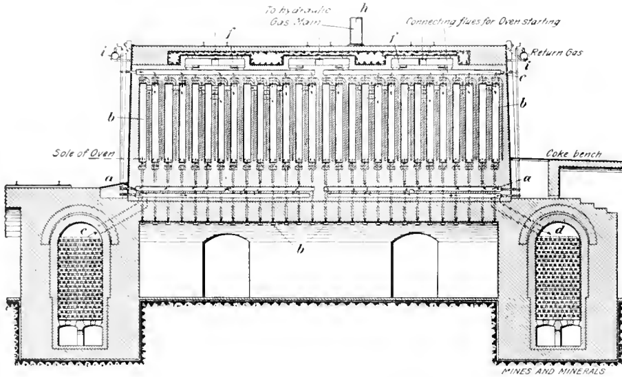
FIG. 1. SECTION THROUGH THE HEATING WALL
