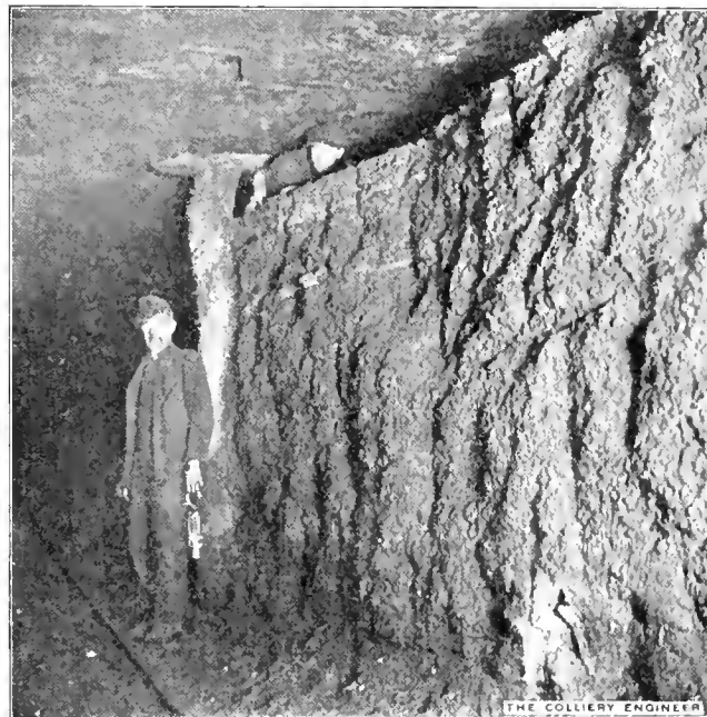
FIG. 8. ROAD DRIVEN THROUGH FLUSHED MATERIAL
