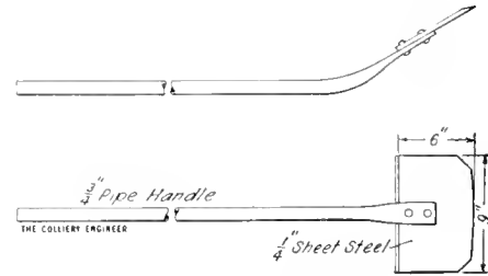
FIG. 1. CAR CLEANER
