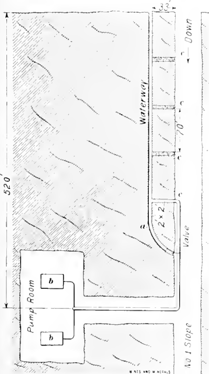
FIG. 1. PLAN OF PUMPING ARRANGEMENT
