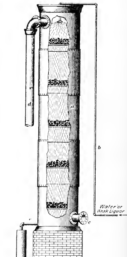
FIG. 4. GAS SCRUBBER
