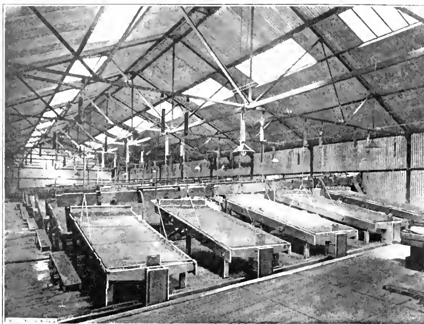
FIG. 3. AMALGAMATING TABLES
