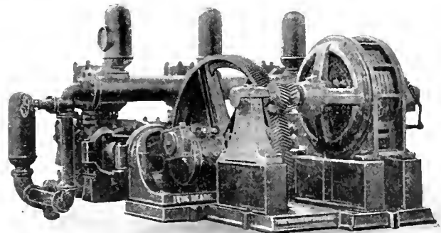
FIG 2 REAR VIEW OF ELECTRIC PUMP
