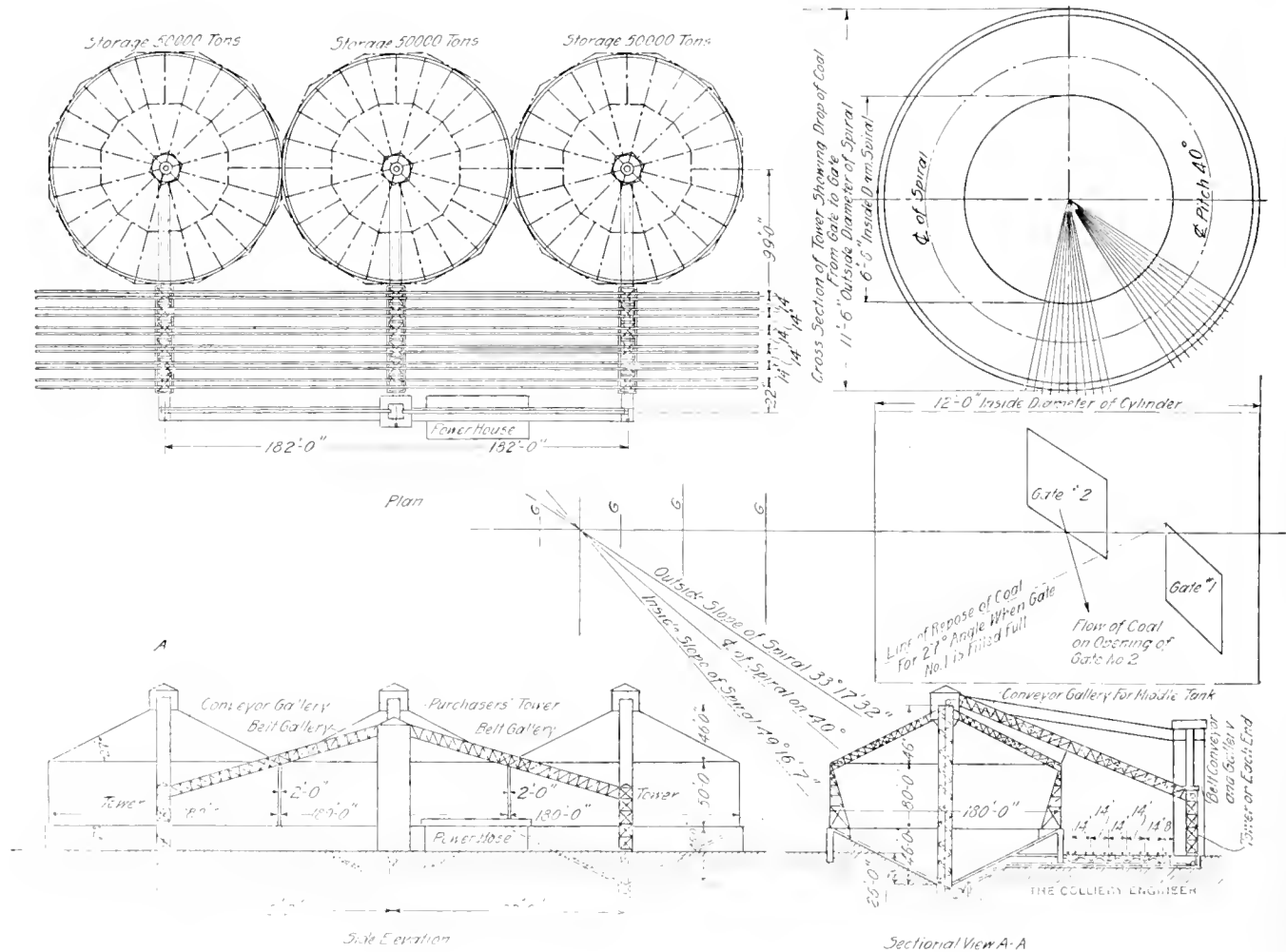
FIG. 8. PLAN AND ELEVATIONS OF COAL STORAGE APPARATUS
