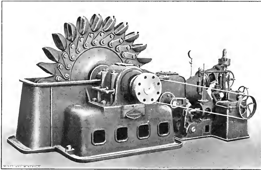
FIG. 4. PELTON WHEEL FOR 2,395-FOOT HEAD
