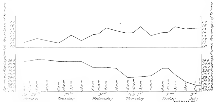
FIG. 3. INFLUENCE OF WORKING AND BAROMETRIC PRESSURE ON PERCENTAGE OF METHANE
