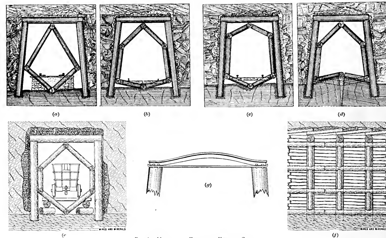
FIG. 1. METHODS OF TIMBERING USED IN GERMANY
