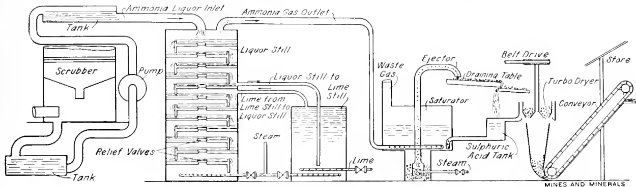
FIG. 5. DIAGRAM SHOWING SEQUENCE OF OPERATIONS IN SULPHATE OF AMMONIA PLANT
