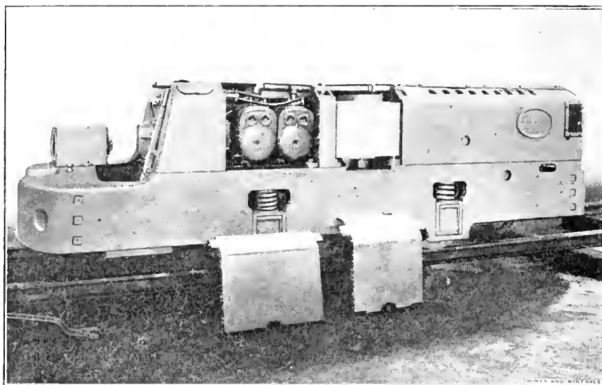
FIG. 2. LOCOMOTIVE WITH GASOLINE TANK DOORS REMOVED
