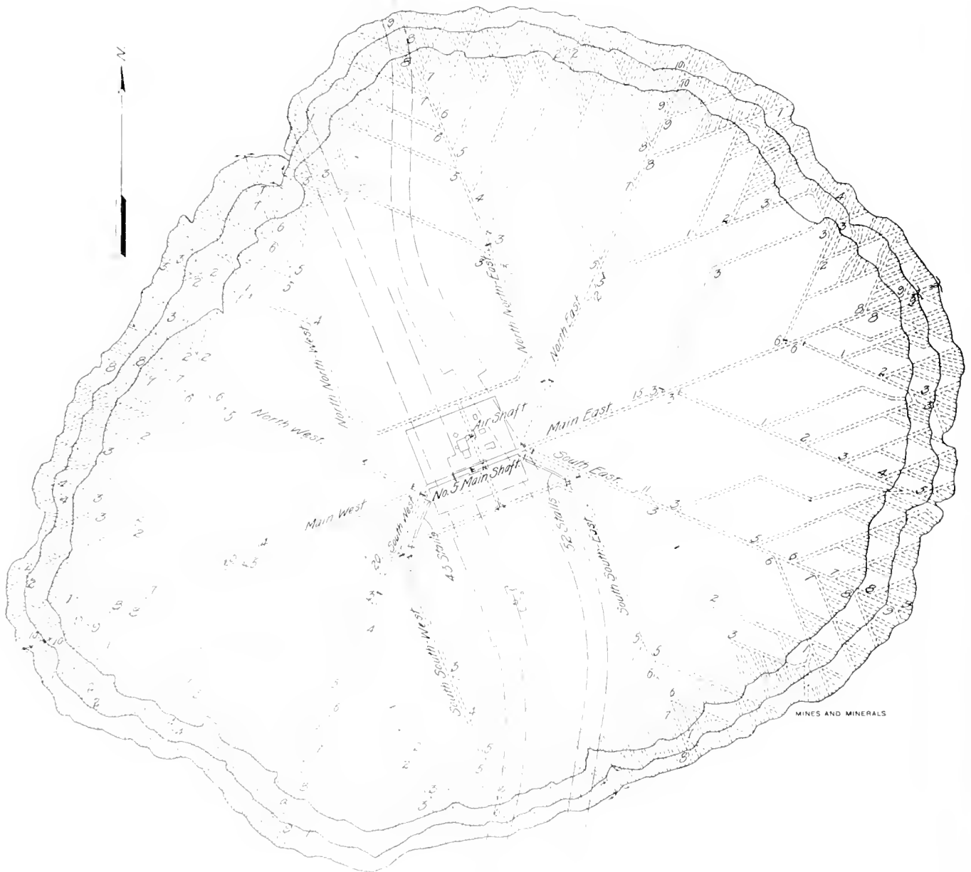
PLAN OF SPRING VALLEY MINE
