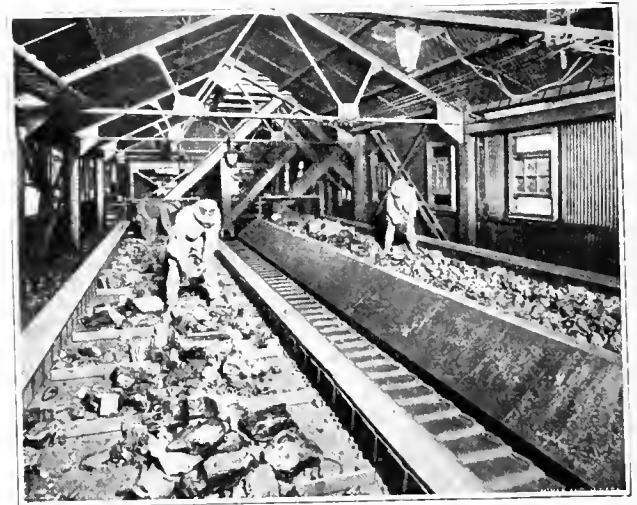
PICKING BAND AND WASTE CONVEYER
