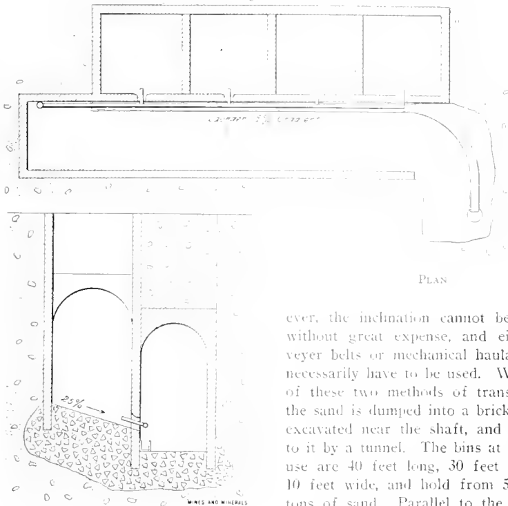
FIG. 1. PLAN AND END ELEVATION OF BINS
