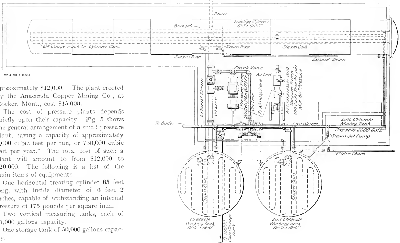
FIG. 5. PLAN OF PRESSURE PLANT FOR TREATING TIMBERS
