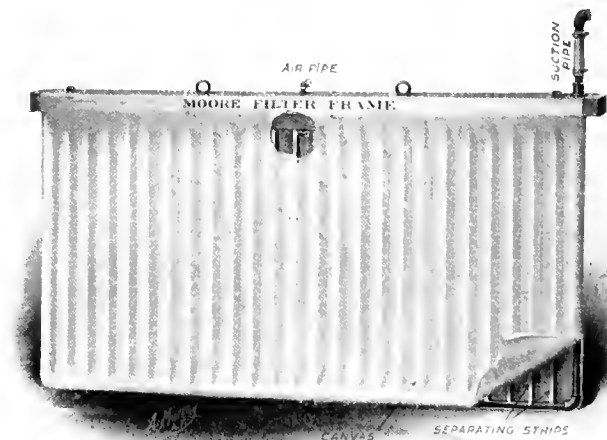
FIG. 4. MOORE FILTER FRAME
