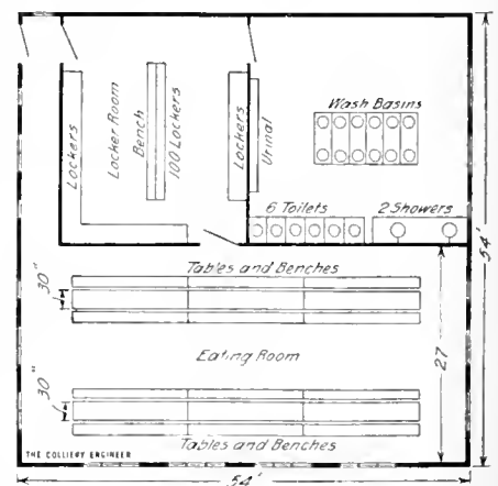
FIG. 3. PLAN OF LUNCH HOUSE, PROSPECT COLLIERY
