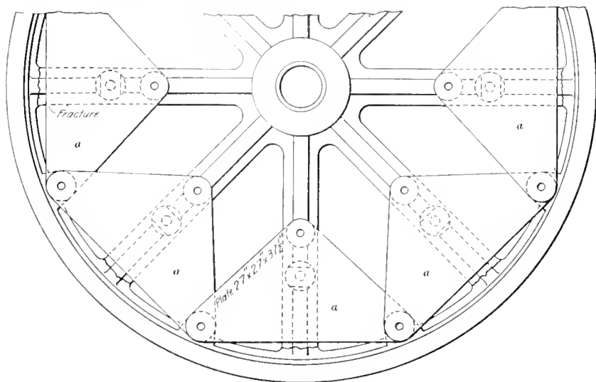
Plan of Rear Wheel
