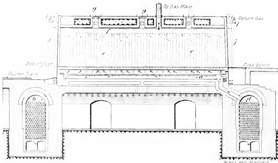
FIG. 3. SECTION THROUGH THE OVEN CHAMBER
