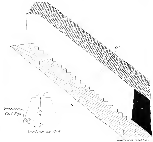
SECTION ON TYPICAL INCLINED SHAFT
