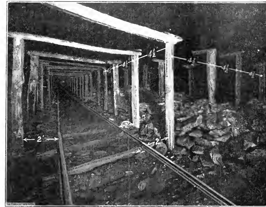
FIG. 2. SHOWING REGULAR TIMBERING
