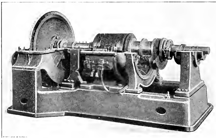
FIG. 1. DIRECT-CURRENT TURBO GENERATOR WITH CASING REMOVED
