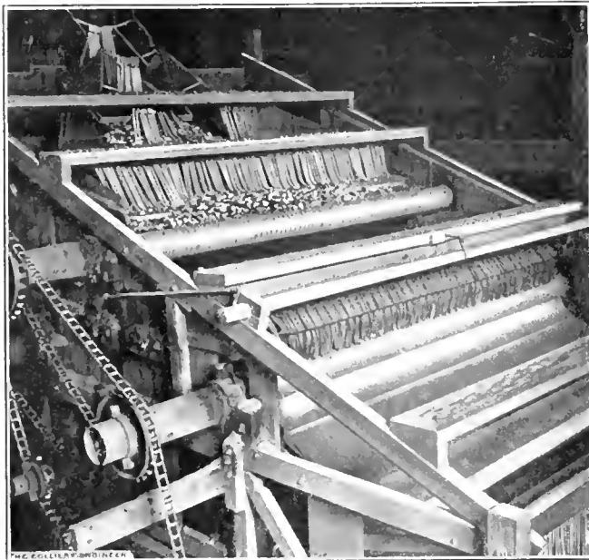
FIG. 1. TOP OF LANGERFELD COAL SEPARATOR
