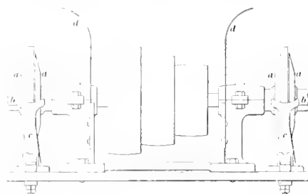
FIG. 4. ZINC SHAVING LATHE
