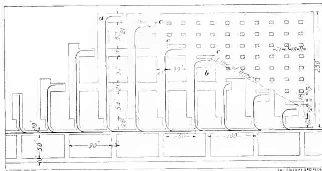
FIG. 1. EXTRACTING PILLARS UNDER DRAW-SLATE
