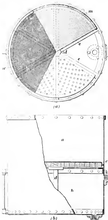
FIG. 2. VACUUM FILTER
