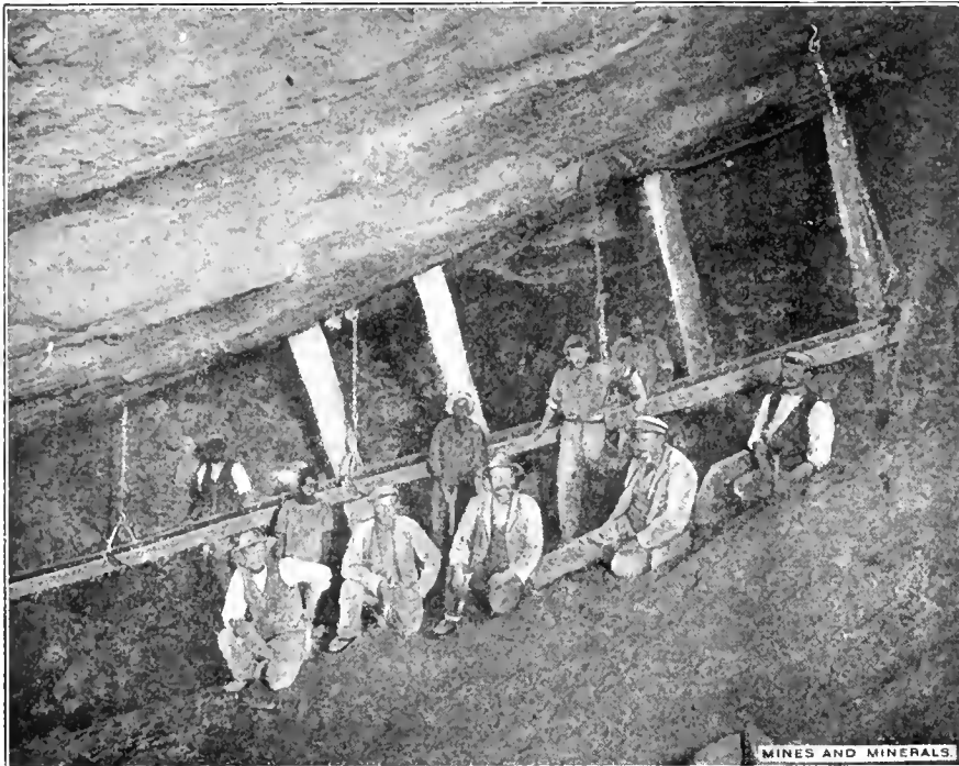
FIG. 1. SWINGING CHUTE IN STOPE, SOUTH AFRICA
