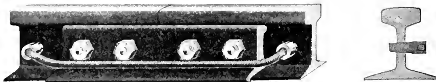
FIG. 4. REMOVABLE BOND, INSTALLED AND SECTIONAL VIEW
