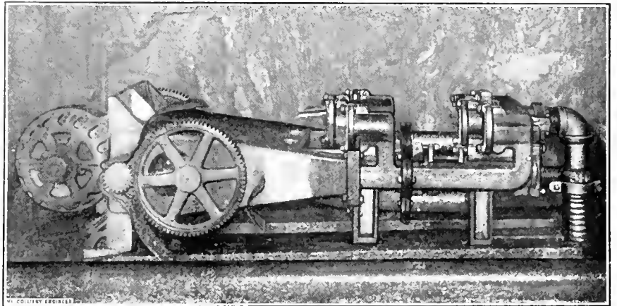
FIG. 1. GOULDS ELECTRIC SINKING PUMP INSTALLED AS A STATION PUMP
