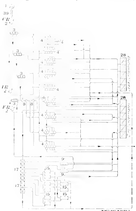
FIG. 1. FLOW SHEET, STANDARD MILL 1, Crusher; CR2, Crushing Mills; IR2, Intermediate Rolls; FR2, Fine Rolls; 3, Trommel; 4, Jigs; 8, Classifiers; 9, Concentrating Tables; 15, Frue Vanners; 17, Spitzkasten; 28, Ore Bins
