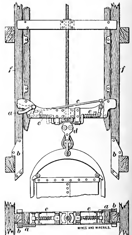
BERRY SAFETY CATCH
