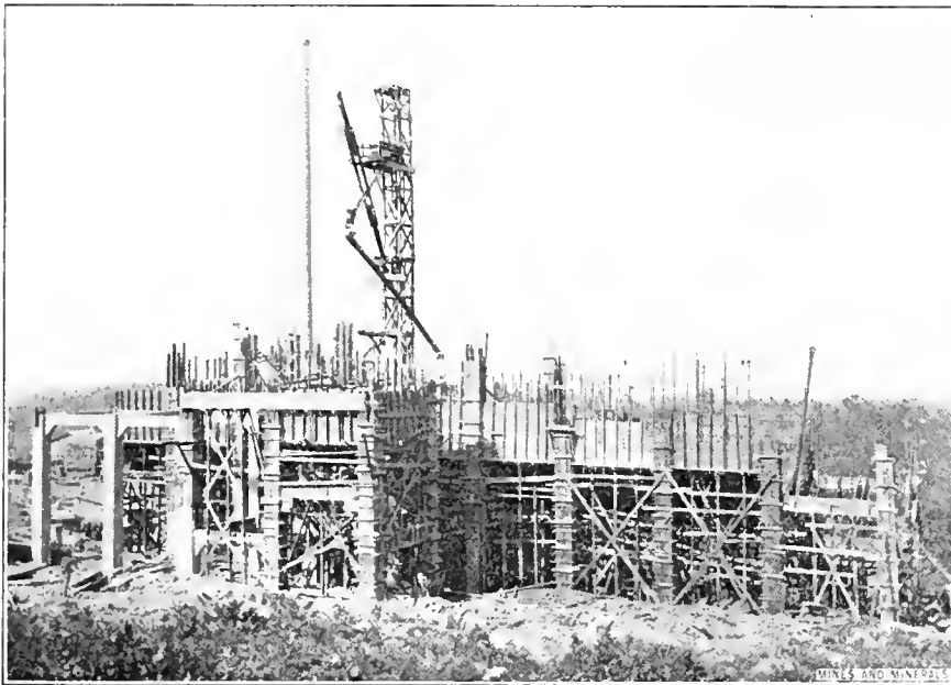
FIG. 1. UNDERWOOD BREAKER, SHOWING CHUTES FOR POURING CONCRETE
