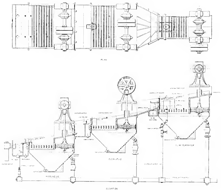
FIG. 1. CONCENTRATING PLANT
