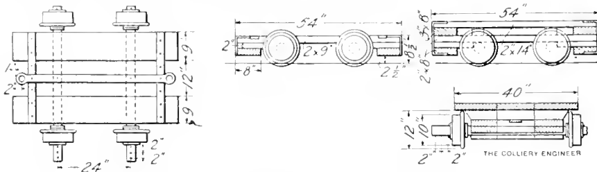
FIG. 6. TRUCK WITH MOVABLE WHEEL BASE
