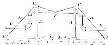
FIG. 1. STEAM LINE HANGER
