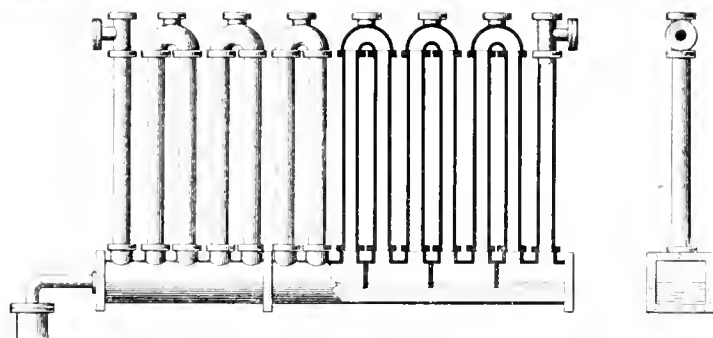
FIG. 3. VERTICAL PIPE CONDENSER
