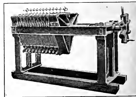
FIG. 6. ZINC DUST PRECIPITATION PRESS
