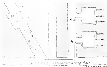
FIG. 1. WIRING FOR ELECTRIC SHOT FIRING
