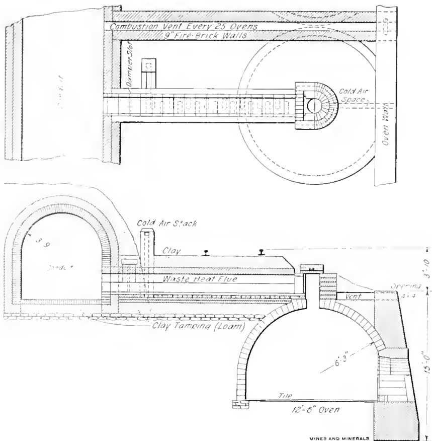
FIG. 1. PLAN AND ELEVATION OF WASTE HEAT COKE OVENS
