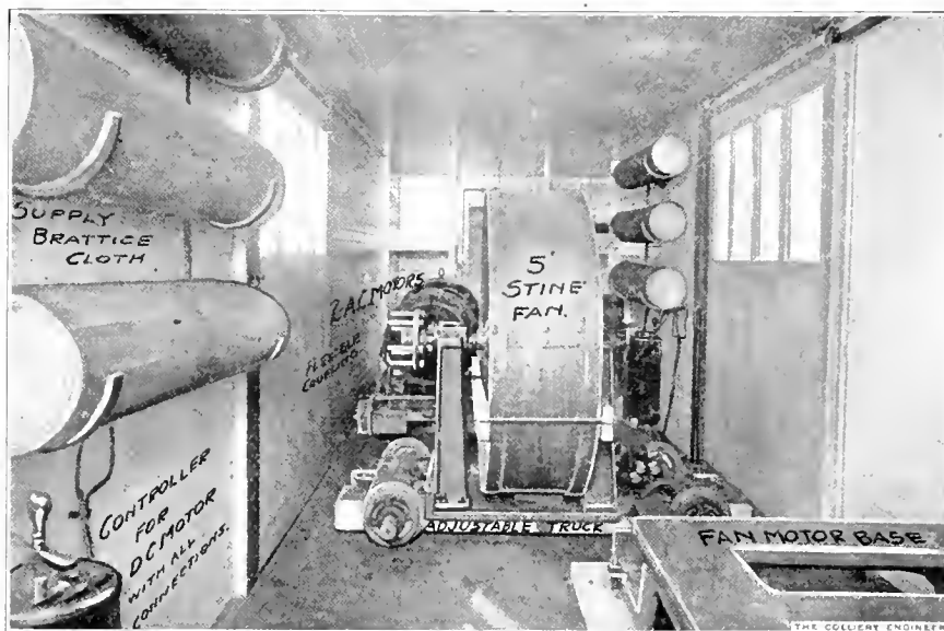
FIG. 5. PART OF INTERIOR OF EMERGENCY CAR
