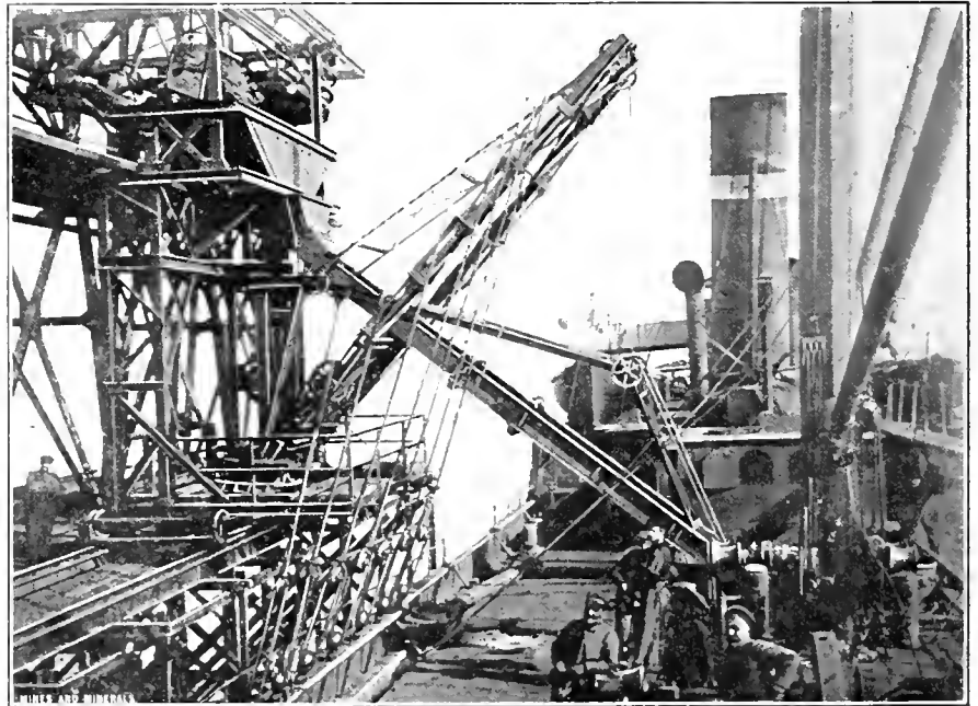
FIG. 3. MOVABLE LOADING CHUTES AT END OF PIER
