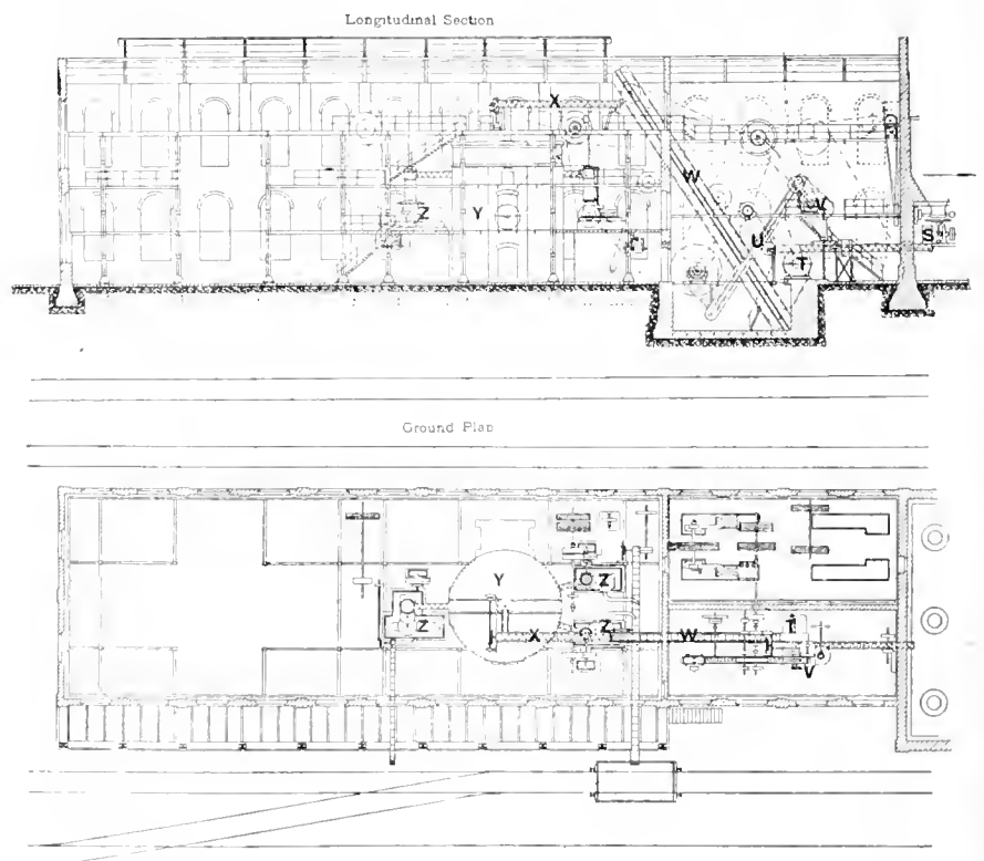
FIG. 3. BRIQUET PLANT
