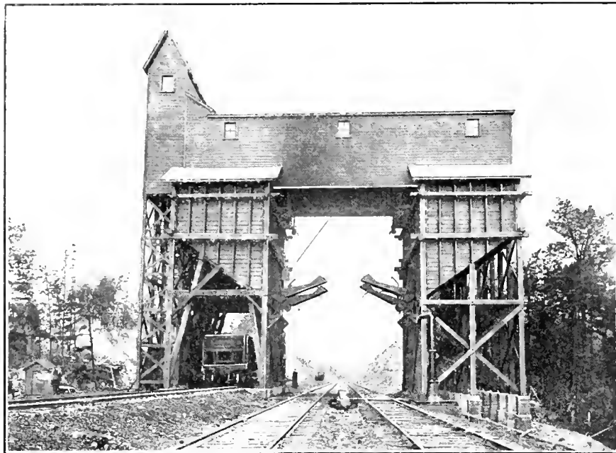
FIG. 2. COALING STATION AT STEARNS, KY.
