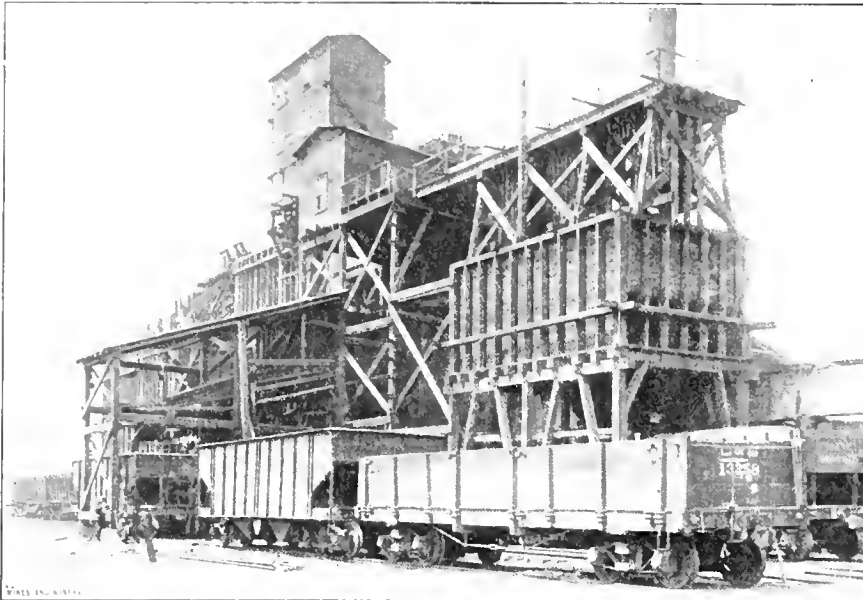
FIG. 3. SCREENS AND LOADING CHUTES, SODDY MINE
