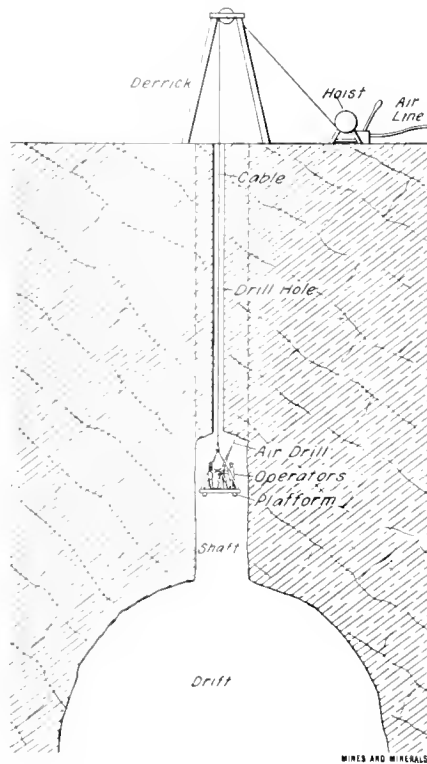
FIG. 1. METHOD OF UPRISING
