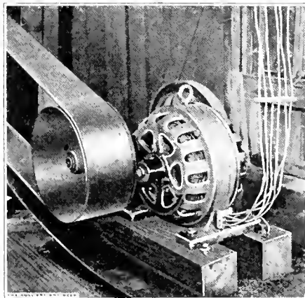
FIG. 11. TWO-SPEED A. C. MOTOR FOR MINE FAN
