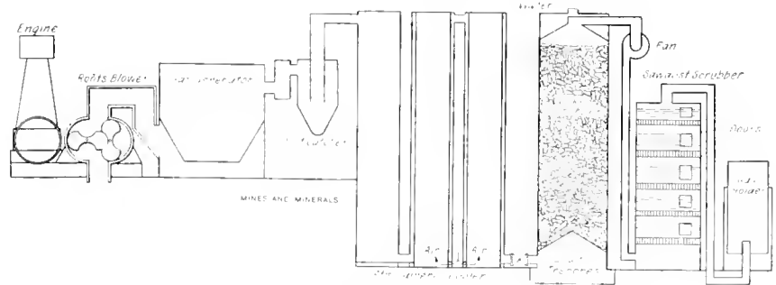
FIG. 4. APPARATUS FOR CLEANING GAS FOR ENGINES
