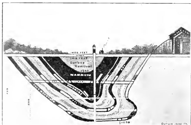
FIG. 3. SECTION AT MOREA COLLIERY
