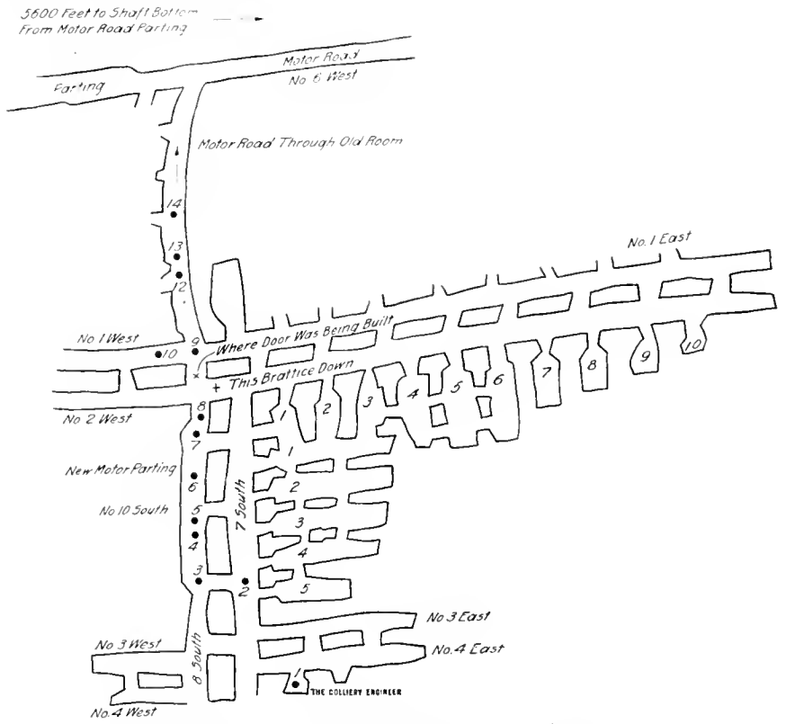
MAP OF PART OF IMPERIAL MINE WHERE EXPLOSION OCCURRED
