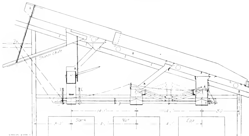
FIG. 3. SHAKING SCREENS
