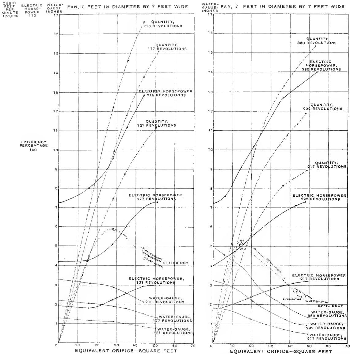
FIG. 5. RELATIONSHIP BETWEEN SPEED OF THE FAN, CUBIC FEET OF AIR, WATER GAUGE, EQUIVALENT ORIFICE AND EFFICIENCY
