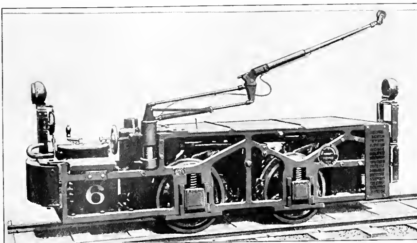
FIG. 2. WESTINGHOUSE MINE TROLLEY.
