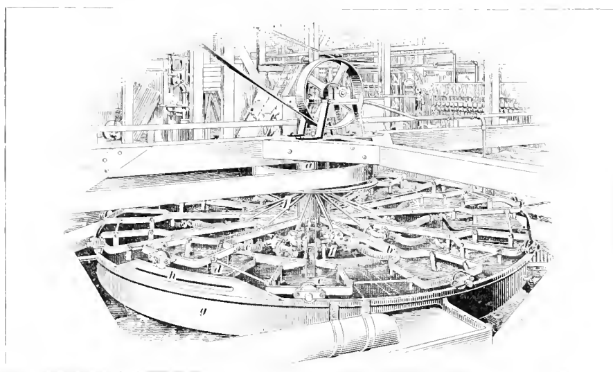
FIG. 1. OGLE-RIDGWAY FILTER
