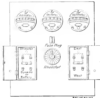
FIG. 3. SWITCHBOARD
