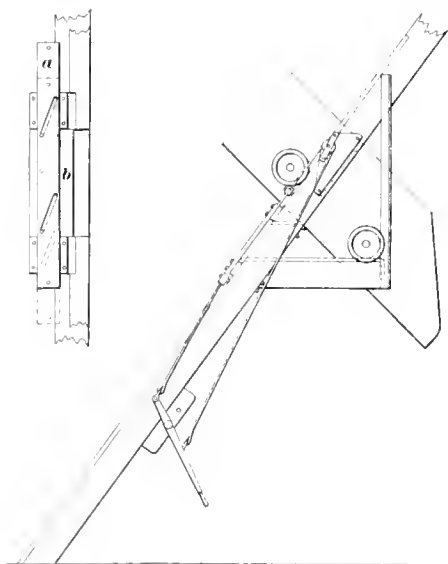
FIG. 2. SLIDING RAIL SKIP DUMP
