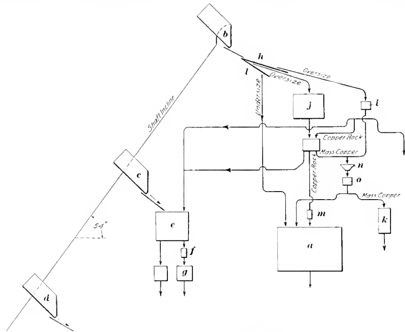
FIG. 1. FLOW SHEET, ROCK HOUSE NO. 2
