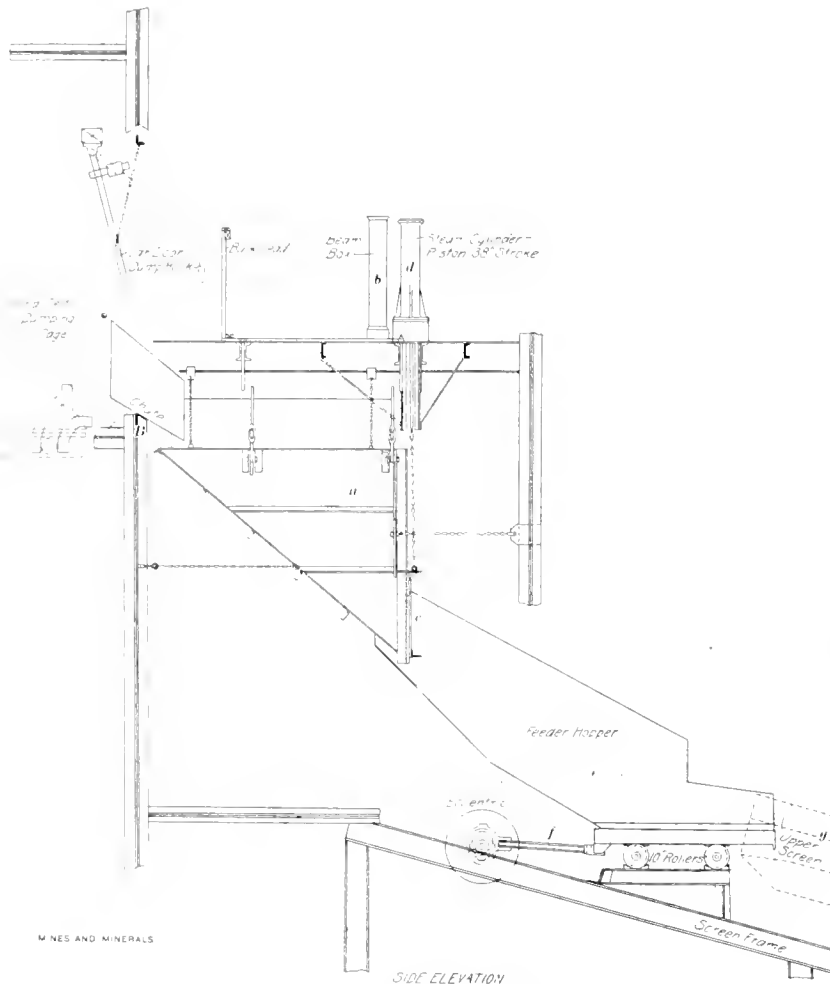
FIG. 2. FEEDER AND WEIGH HOPPER
