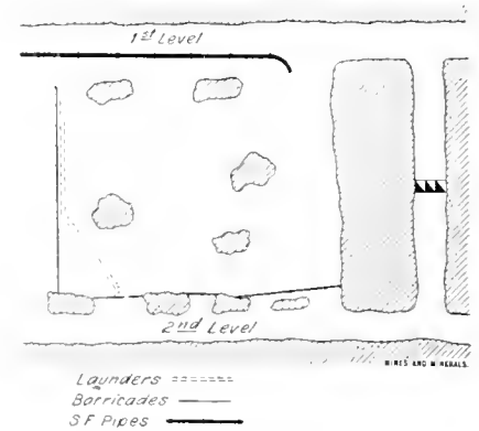
FIG. 2. STOPE READY FOR FILLING
