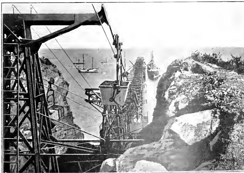
FIG. 4. GIOVE PORTELLO LOADING PIER
