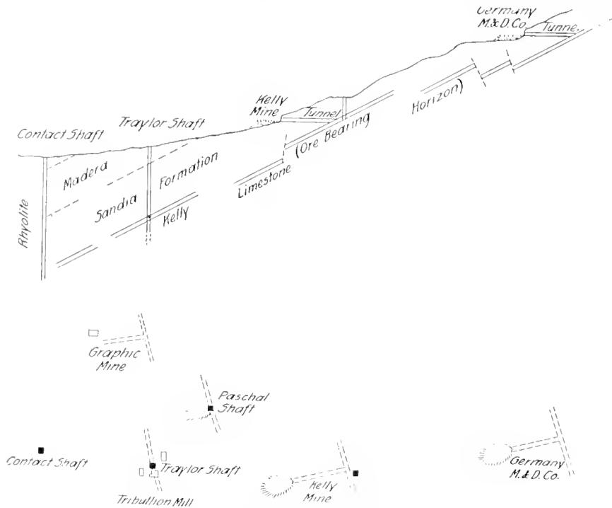
FIG. 3. SECTION AND PLAN OF WORKINGS ON KELLY LIMESTONE, MAGDALENA DISTRICT, N. MEX.
