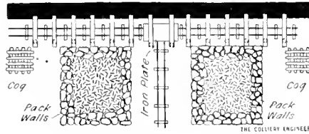
FIG. 2. PLAN SHOWING PACKS, TIMBER AND TRAMROAD
