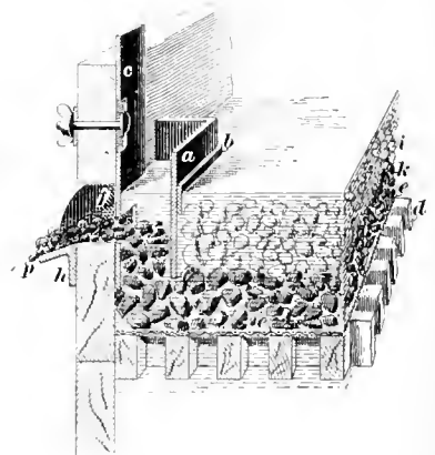
FIG. 1. THE HEBERLE GATE
