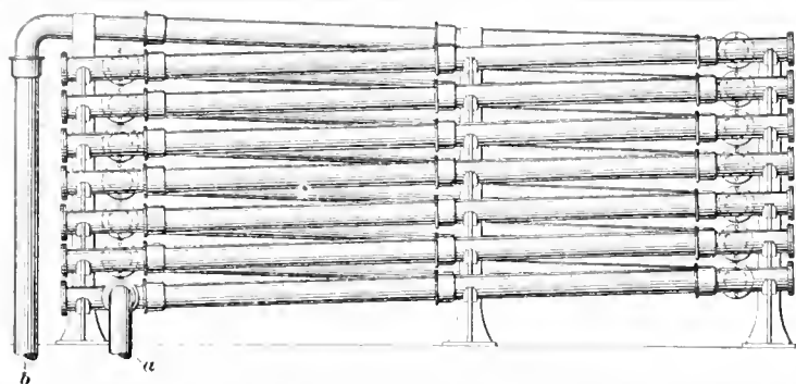
FIG. 2. HORIZONTAL PIPE CONDENSER
