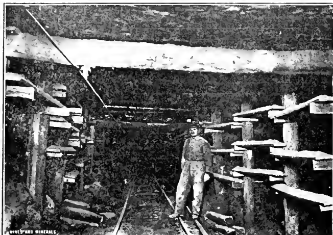
FIG. 2. ADOBE DUST ON SHELVES ON SIDES OF AIRWAY
