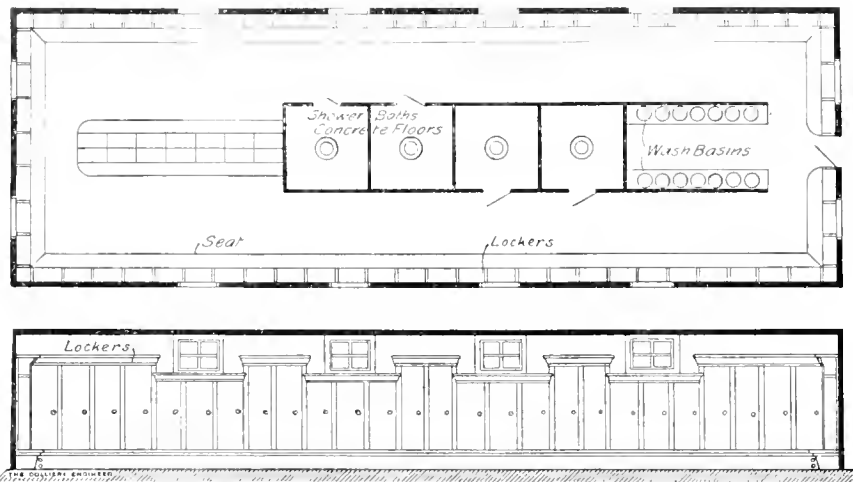
FIG. 1. PLAN AND ELEVATION OF BATH HOUSE
