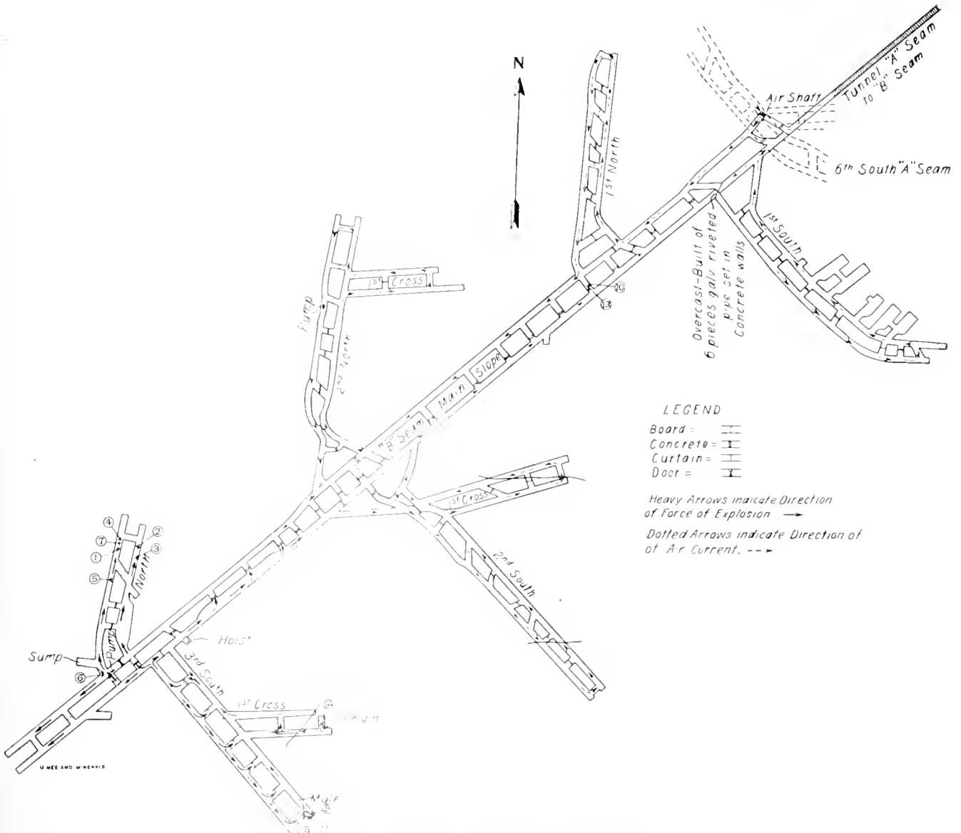
FIG. 1. PLAN OF WORKINGS IN B SEAM, HASTINGS MINE
