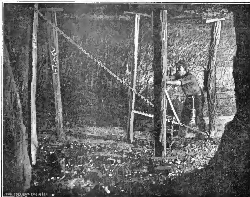
FIG. 4. PROP PULLING MACHINE
