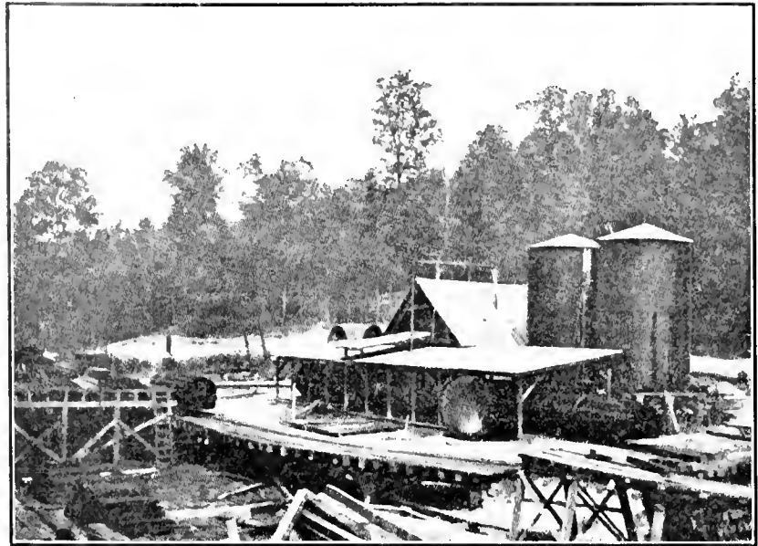
FIG. 4. WOOD-PRESERVING PLANT AT McADORY, ALA.
