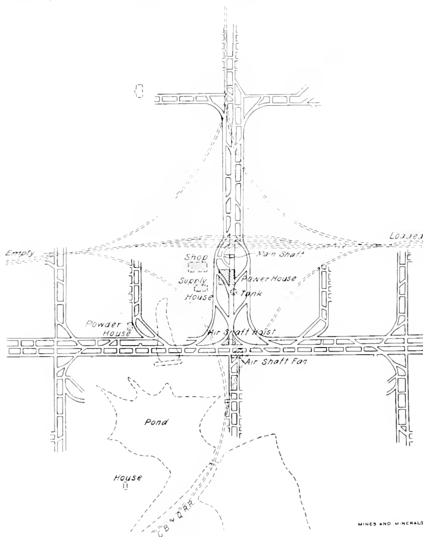
FIG. 5. SURFACE AND UNDERGROUND PLAN, SURFACE WORKS SHOWN DOTTED
