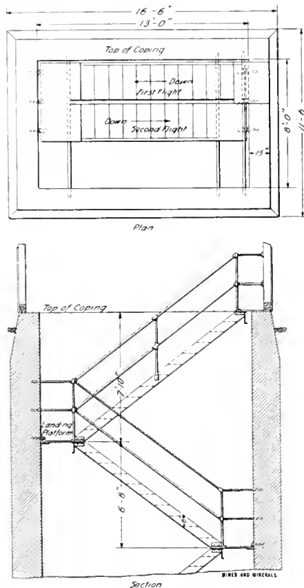
FIG. 3. SHAFT AND STAIRWAY
