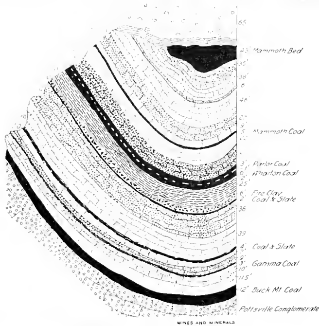
FIG. 2. SECTION AT DERRINGER
