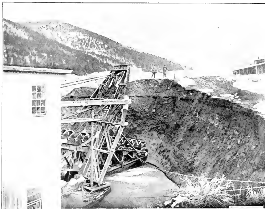
FIG. 4. DREDGE ATTACKING HIGH BANK ON FRENCH CREEK
