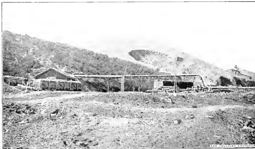
FIG. 1. CULM PILE BEING FLUSHED INTO HOLMES SEAM WORKINGS AT TUNNEL RIDGE COLLIERY
