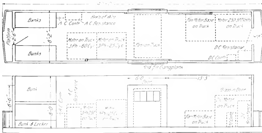
FIG. 4. PLAN AND ELEVATION OF C. F. & I. CO., EMERGENCY CAR
