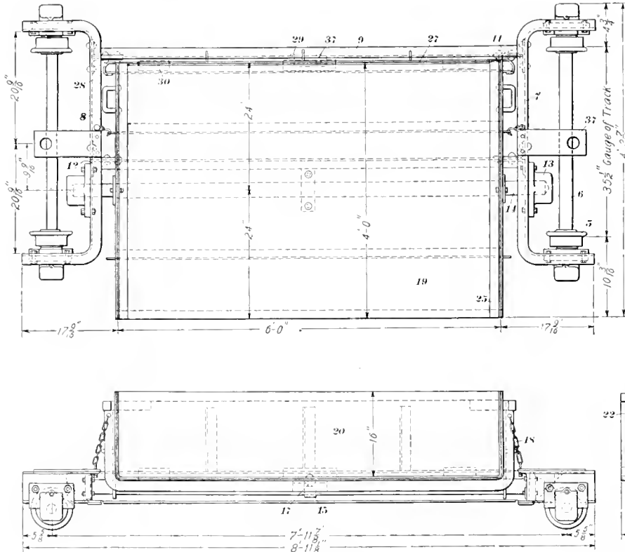
FIG. 5. BUGGY FOR LOW PLACES. FOR EXPLANATION OF NUMBERS SEE TABLE 1
