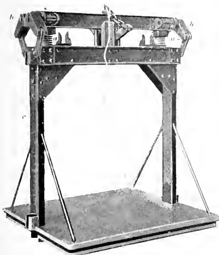
FIG. 1. SAFETY CATCH ON CAGE
