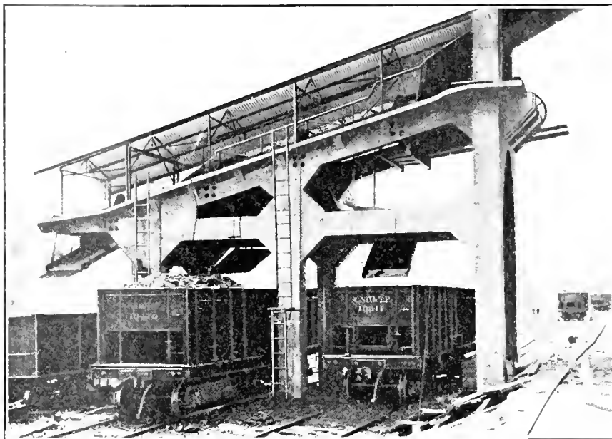
FIG. 5. STEARNS TIPPIE, CHUTE END
