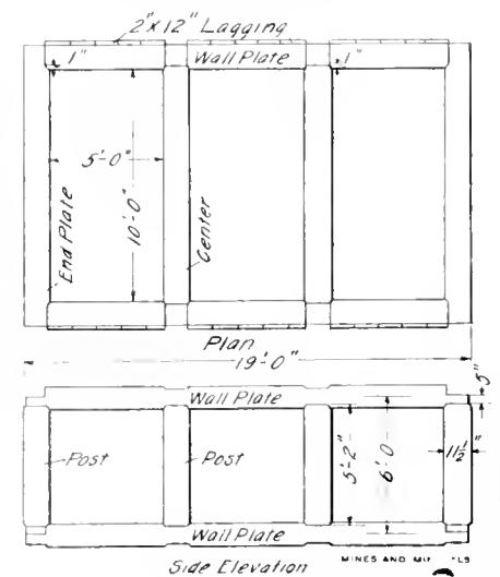
FIG. 6. ELLISON SHAFT TIMBERING
