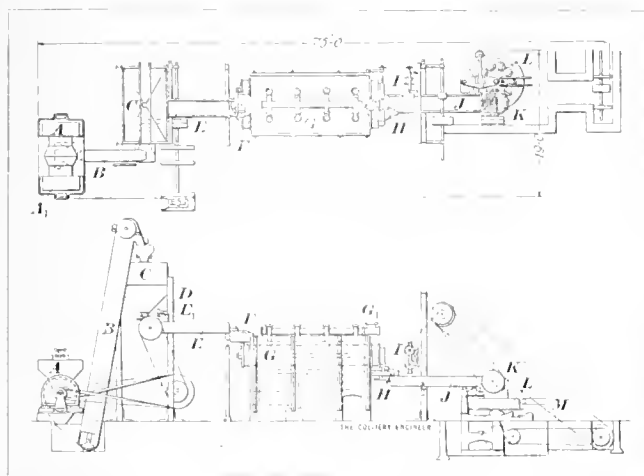
FIG. 1. BRIQUETTING PLANT
