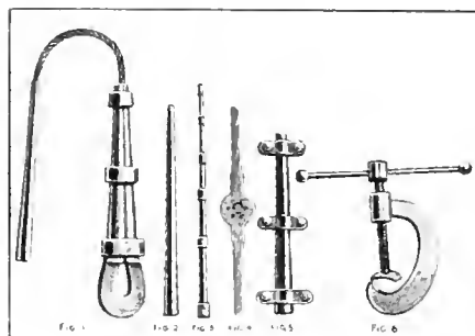
TOOLS FOR SOCKETING WINDING ROPE
