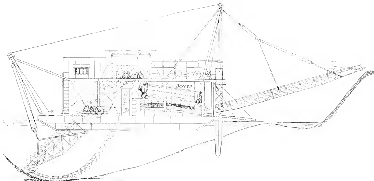
FIG. 1. SECTIONAL VIEW OF DREDGE
