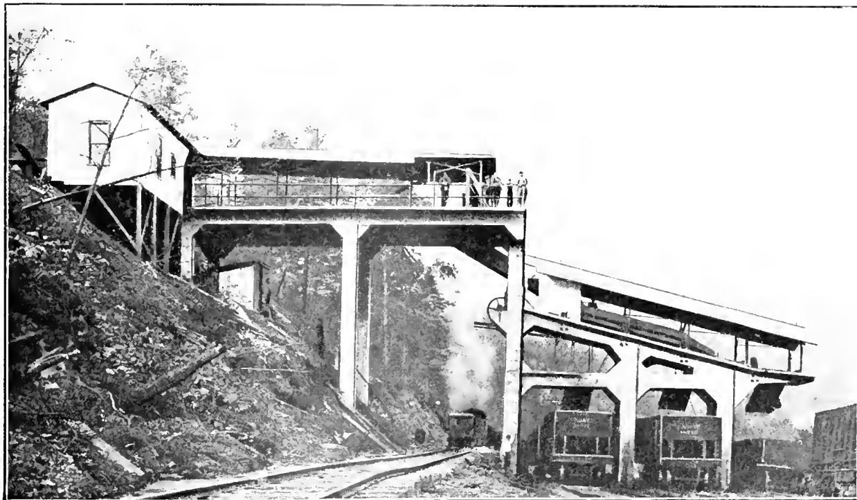
FIG. 1. CONCRETE TIPPIL AT MINE OF STEARNS COAL CO.
