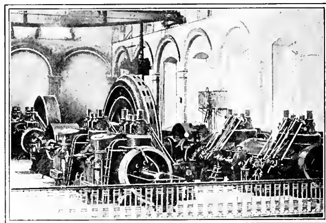
FIG. 2. TWIN TANDEM GAS ENGINES 2,400 HORSEPOWER AT BARGOED
