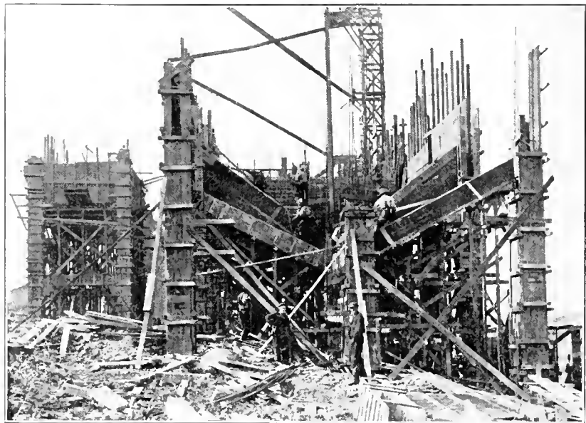
FIG. 2. COAL POCKETS, UNDERWOOD BREAKER
