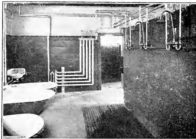
FIG. 2. INTERIOR OF BATH HOUSE
