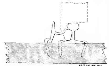
ARRANGEMENT OF RAILS
