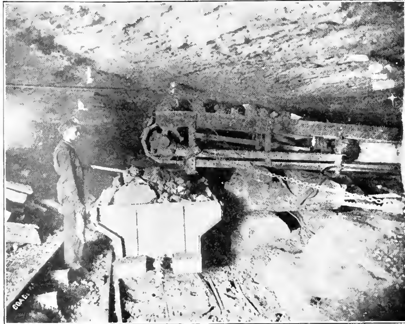
FIG. 4. HEAD END OF MAIN CONVEYER
