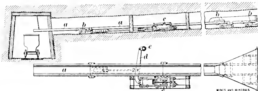
FIG. 5. EICHHOFF CONVEYER SYSTEM
