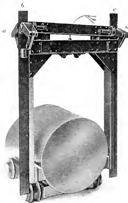
FIG. 2 SAFETY CATCH ON SKIP
