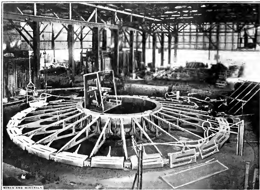
FIG. 2. WALKER CASTING MACHINE
