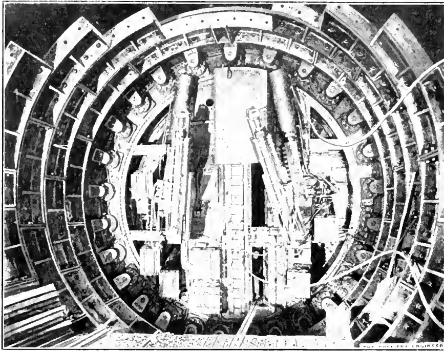
FIG. 3. SHIELD IN PENNSYLVANIA TUNNELS SHOWING CIRCULAR ROW OF JACKS AND TUNNEL LINING
