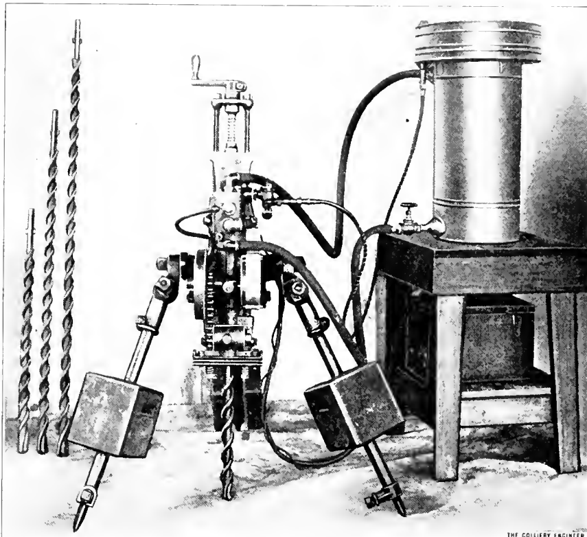
FIG. 6. GASOLINE ROCK DRILL
