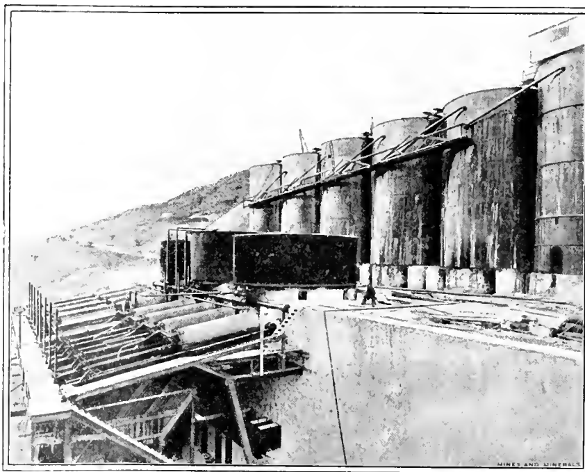
FIG. 1. PACHUCA TANKS, AT RIGHT
