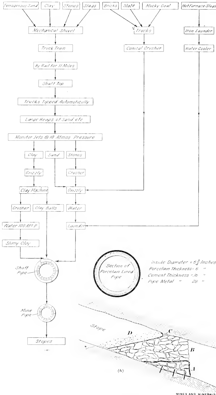
FIG. 3. FLOW SHEET AND SECTION OF BARRICADE
