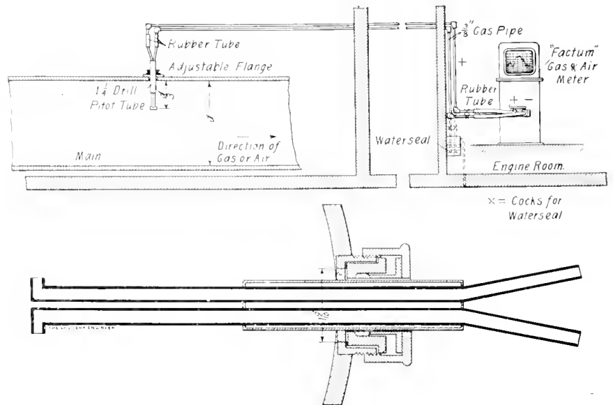
FIG. 2. METHOD OF INSTALLING AIR METER
