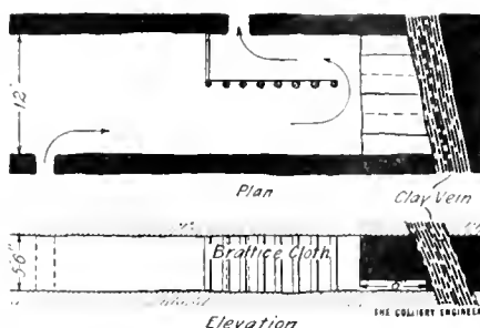
FIG. 2. FACE OF NO. 12 ENTRY
