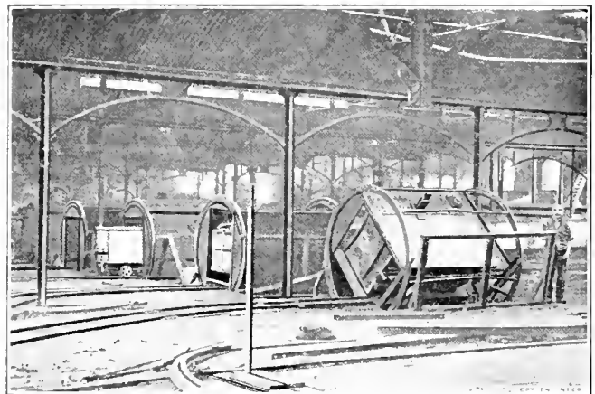
FIG. 2. ROTARY TIPPLES
