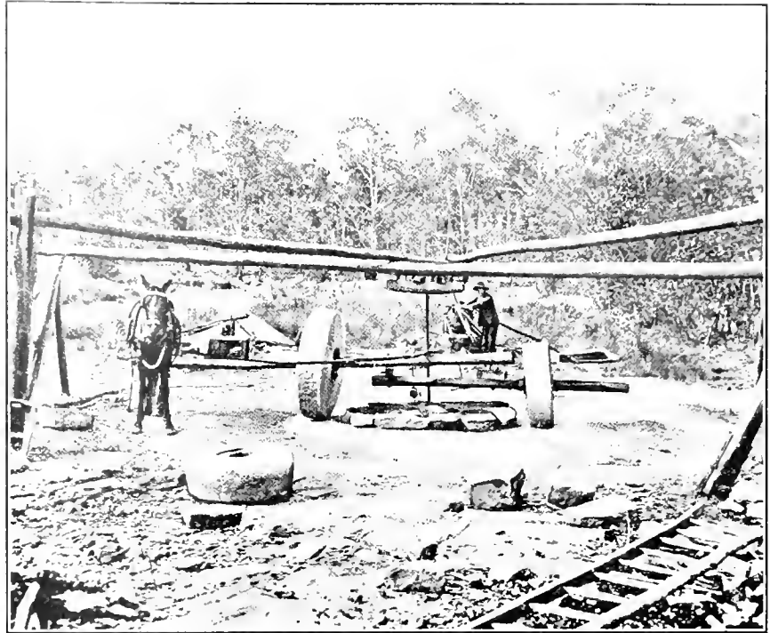
FIG. 5. HOME-MADE CHILEAN MILL
