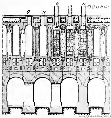
FIG. 4. CROSS SECTION THROUGH THE OVENS
