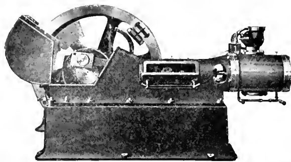
FIG. 5. THE BROWNELL ENGINE
