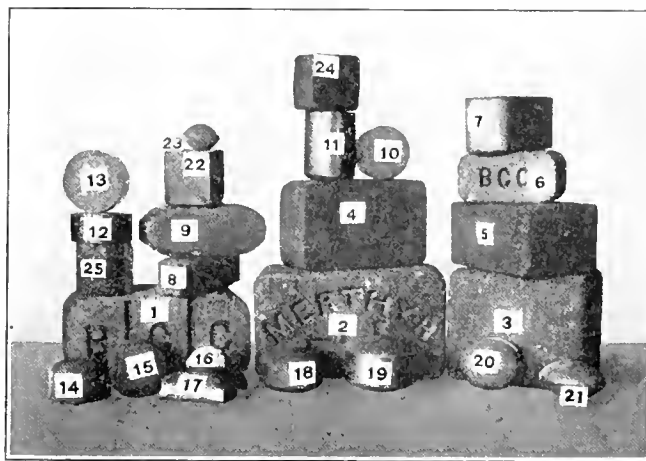
FIG. 2. SHOWING FORMS OF BRIQUETS
