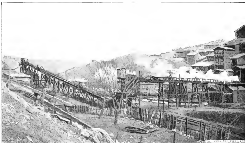
FIG. 5. CONVEYER LINES AT SHENANDOAH CITY COLLIERY
