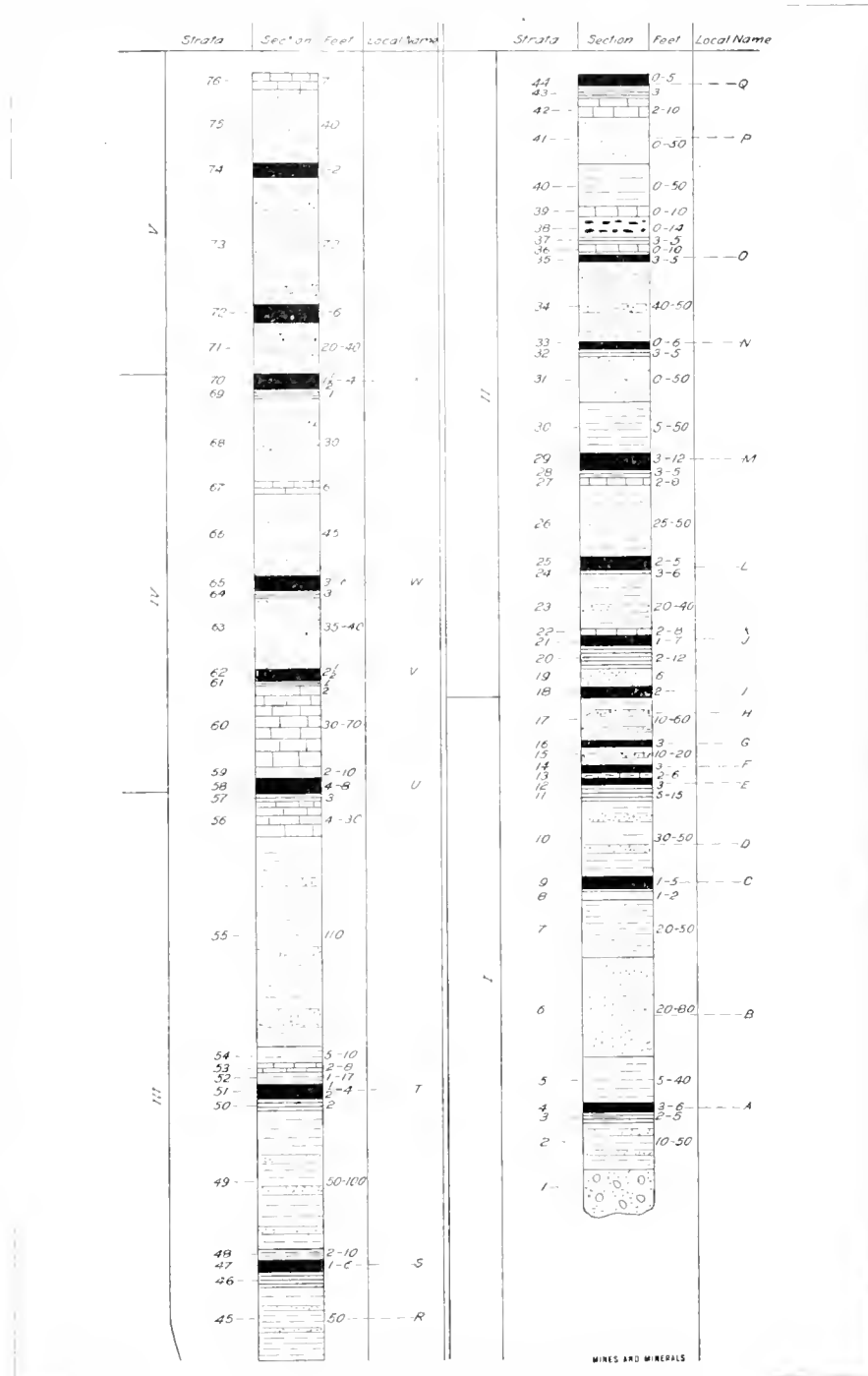
FIG. 2. SECTION OF OHIO COAL STRATA. FOR SIGNIFICANCE OF NUMBERS, LETTERS, ETC., SEE LEGEND ACCOMPANYING
