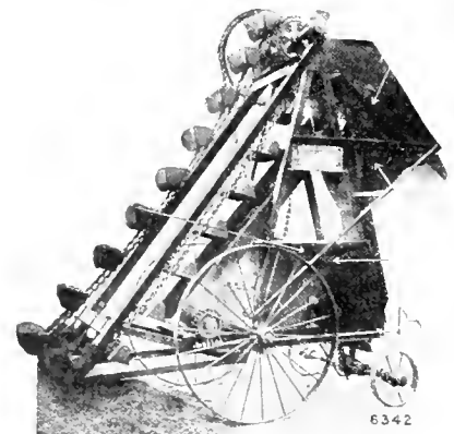
FIG. 5. PORTABLE COAL LOADER
