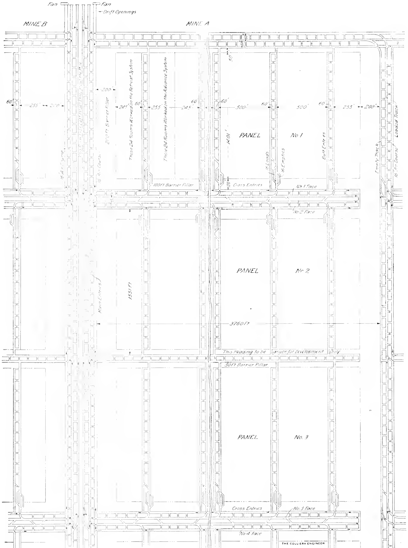
FIG. 4. PLAN OF PANEL SYSTEM OF MINING
