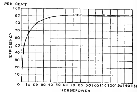
FIG. 4. EFFICIENCY CURVE OF ELECTRIC MOTOR
