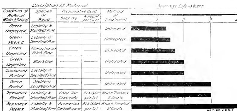
FIG. 1. SHOWING LIFE OF TREATED AND UNTREATED GANGWAY SETS
