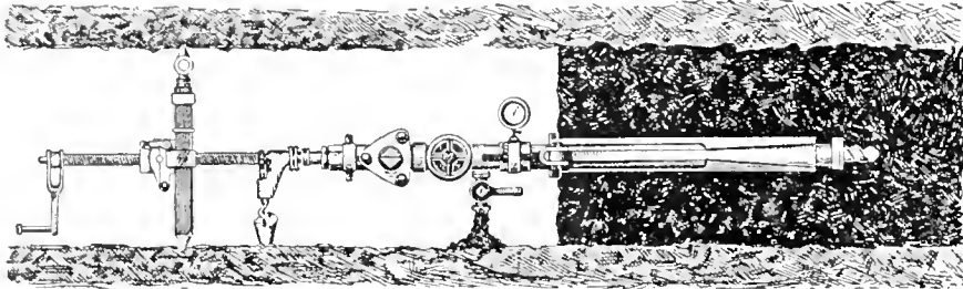
MACHINE FOR TAPPING WATER UNDER PRESSURE, IN PLACE
