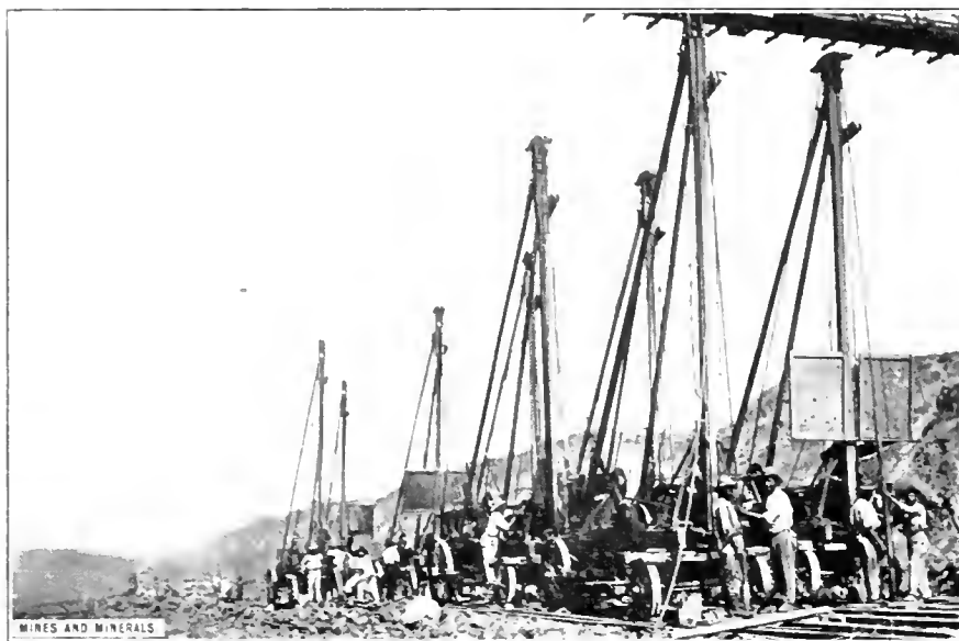
FIG. 3. CHURN DRILLS ON PANAMA CANAL
