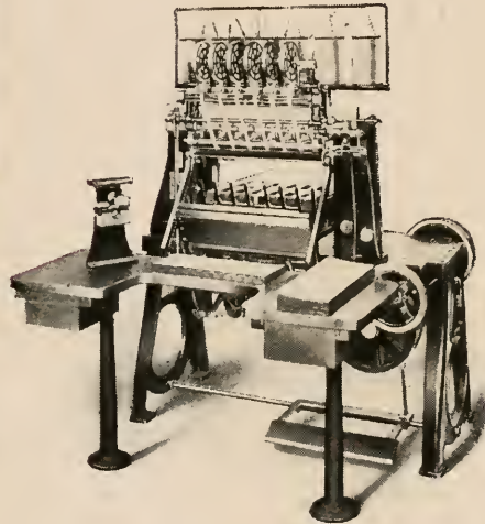
Smyth No. 4 and 6 Book Sewing Machine,
