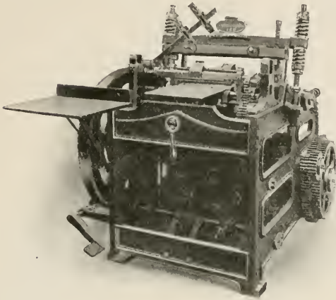
Rounds and Backs Books in one continuous operation, 600-700 per hour.
