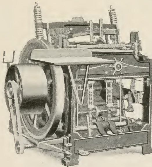
CRAWLEY ROUNDING and BACKING MACHINE No. 357.
