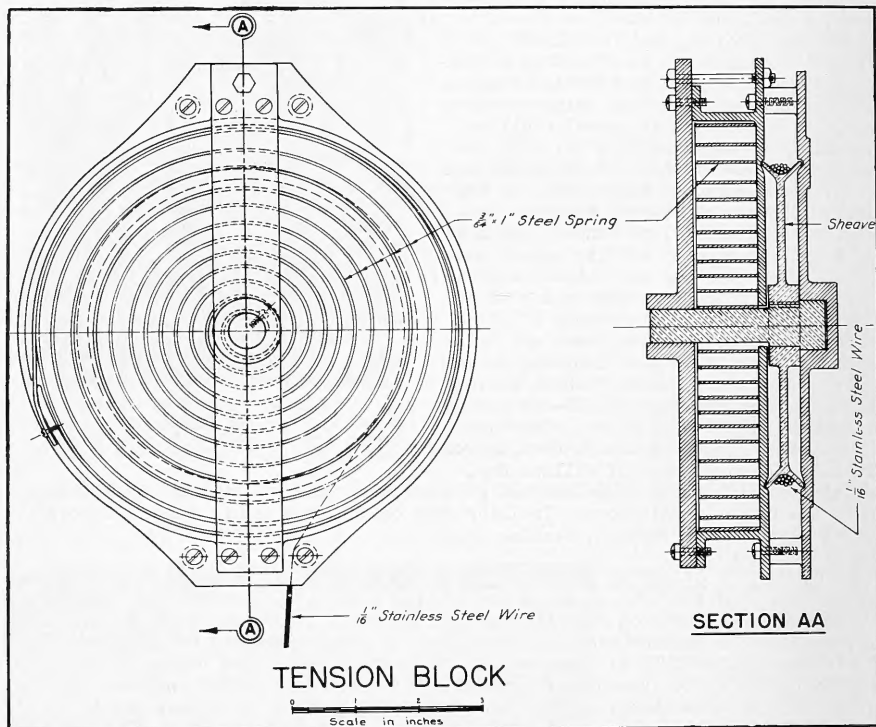
FIG. 5 - DETAIL DRAWING OF THE TENSION BLOCK.
