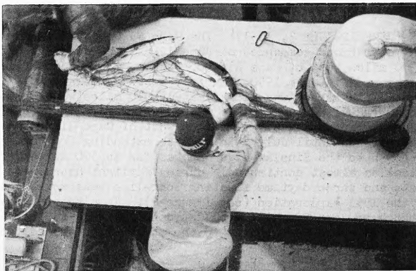
FIG. 3 - REMOVING ALBACORE FROM THE GILL NET. ROLLER AT RIGHT TAKES OFF FROM THE MAIN WINCH.
