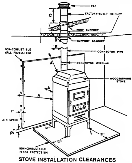
Figure 2109-4 CLEARANCES FOR SOLID FUEL BURNING APPLIANCES
