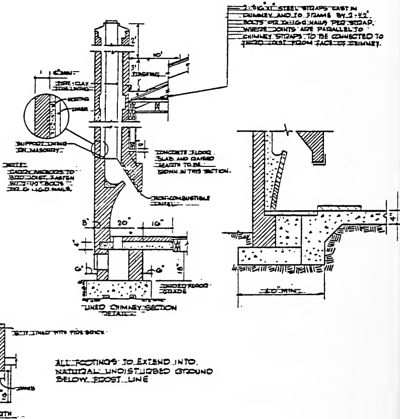
Figure 2108-3 FIREPLACE CONSTRUCTION DETAILS
