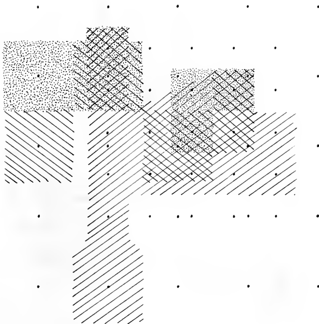
FIGURE 11. OVERLAPPING OF FIELD RANGES
