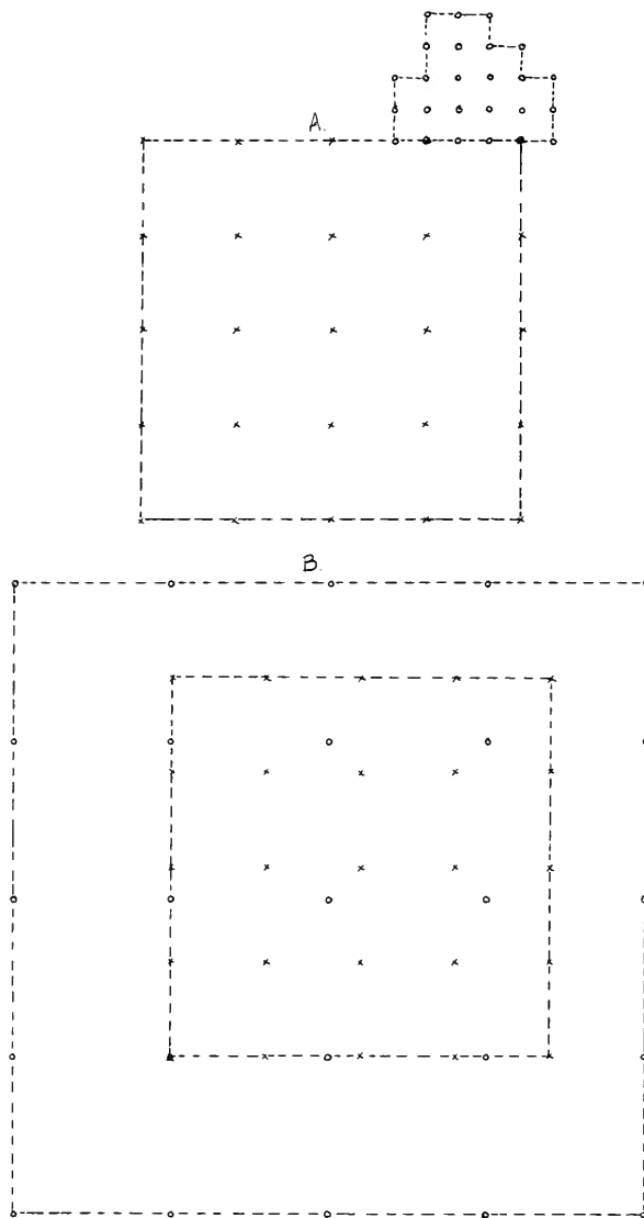
FIGURE 5. INITIAL AND ADJUSTED GRID LOCATIONS OF FOREST (A) AND FIELD (B)
