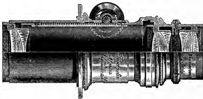
Illustration No. 96 Voigtlander Telephoto Lens
