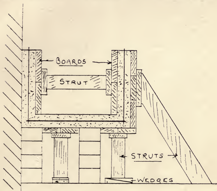
SECTION OF MANGER SHOWING NECESSARY WOOD STRUTTING FOR CONSTRUCTION.
