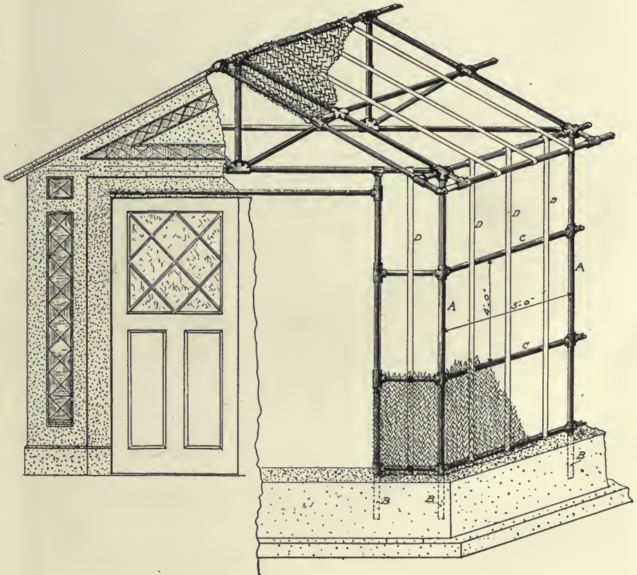
Diagram of Pipe Frame Garage.
