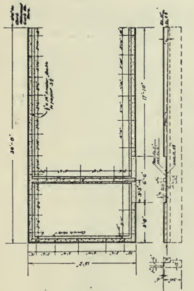
GARAGE FOUNDATION. SCALE \frac{1}{2} " = 1 FT.
