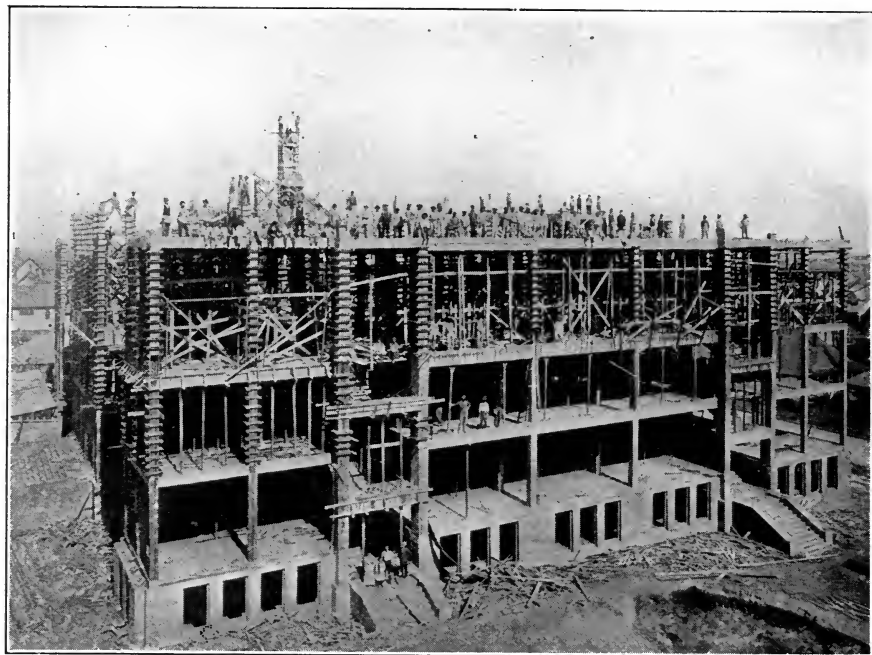
FIG. 9.—HIGH SCHOOL, FORT WORTH, TEXAS. CONCRETE FLOORS AND SKELETON.
