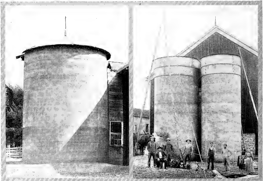
Northern Wisconsin's First Monolithic Silo—built by G. W. Graham of Roberts, with Wisconsin Farmers' Institute silo forms. (See illustration on page 56.)
