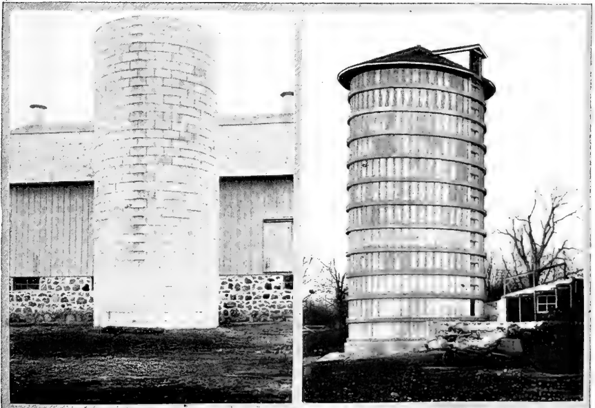
Hurst Reinforced Concrete Block Silo, built on J. W. Cooper's farm at Whitewater, Wisconsin, by Chas. B. Hurst Co., Chicago.
