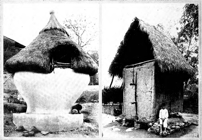
Mexican circular silo made of adobe, which successfully keeps green fodder in the drier parts of Mexico, where the material is not disintegrated by rain.
