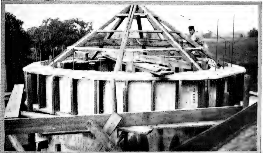
Framing for Constructing a Concrete Roof on the concrete silo; wall forms in position. The illustration is of the University of Wisconsin forms.
