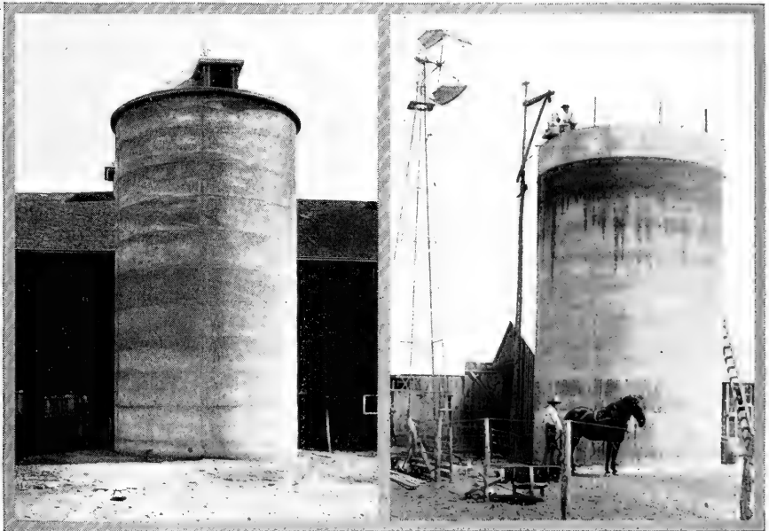
Monolithic Concrete Silo built by S. E. Griffith for S. L. Covey, Belvidere, Illinois; looks and is substantial
