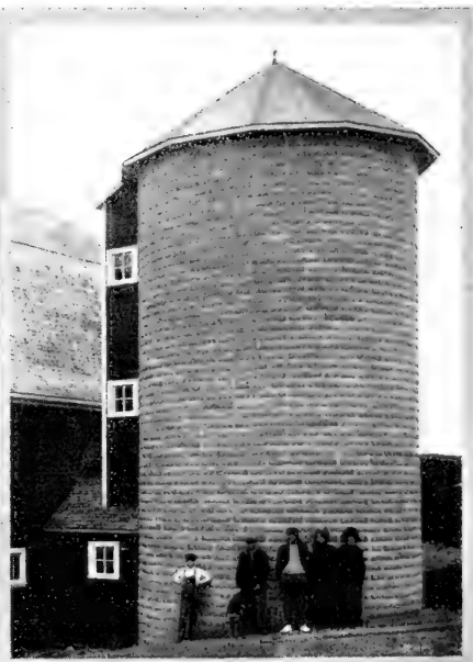
F. W. Merrill's Concrete Block Silo, built by owner, Kaneville, Illinois.
