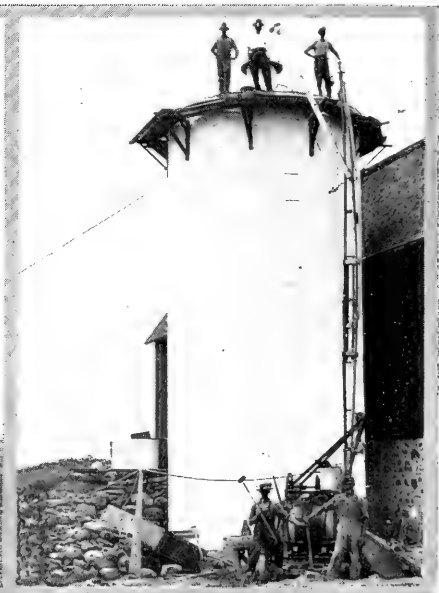
Monolithic Concrete Silo built by Peter Oskoe, Neenah, Wisconsin, for Emil Black.
