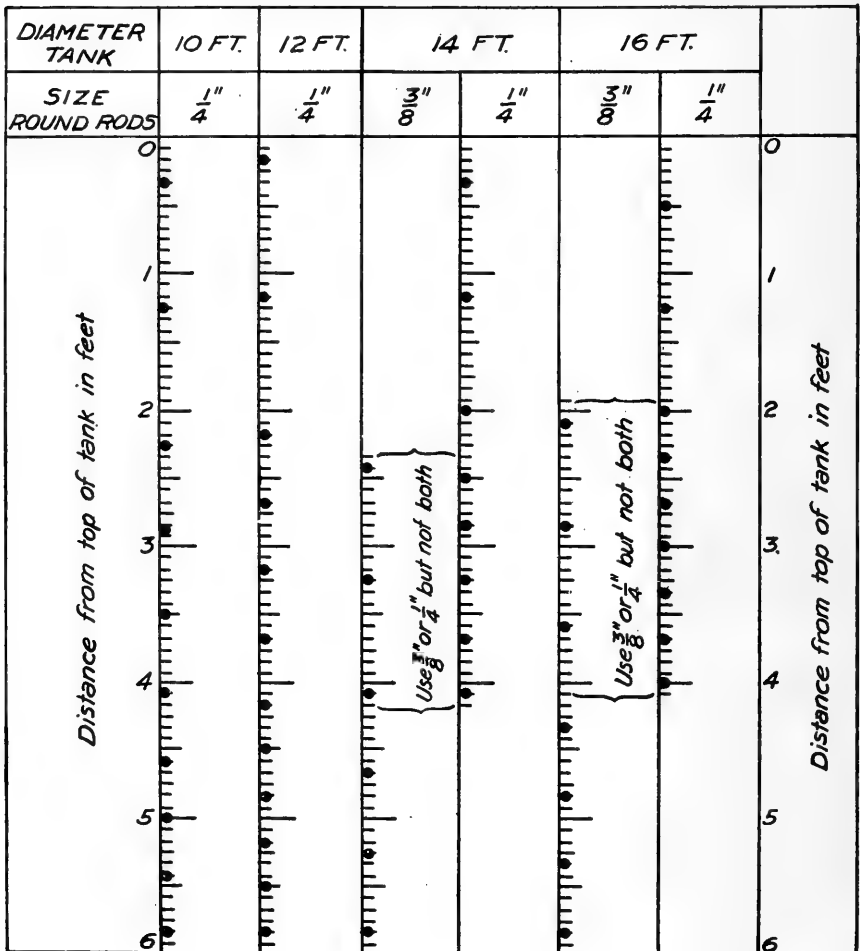
Chart Showing Horizontal Tank Reinforcing
