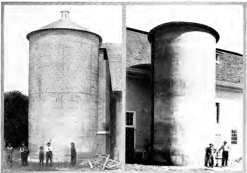
A Minnesota Concrete Silo built by farmer A. L. Liske of Henderson, Minnesota, who used home-made forms.
