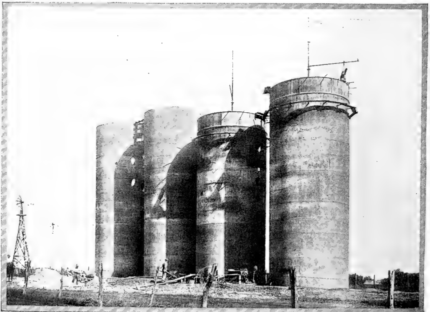
Four in a Row—all reinforced concrete silos, near Manhattan, Kansas (16 feet by 60 feet inside dimensions), built for H. G. Adams, Maple Hill. Probably the largest silos west of the Mississippi River.
