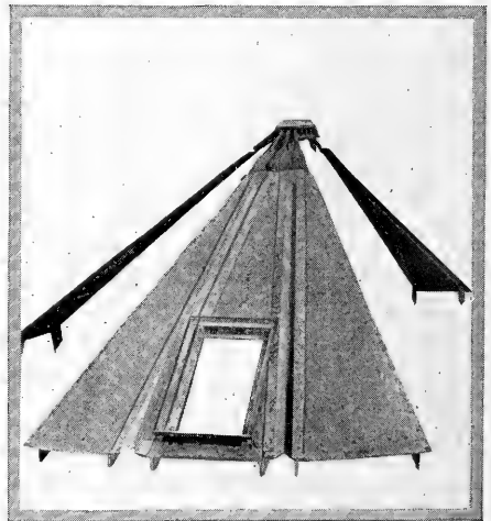
Detail of Roof Forms (patented) of W. H. Warford, Geneva, Illinois, a successful silo contractor who has built a number of good concrete roofs on concrete silos with this form.
