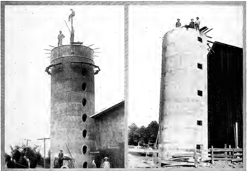
Frank Leach's Monolithic Silo (dimensions 14 feet by 48 feet) near Chesterfield, Illinois, built by Perry Duckles, Carlinville, Illinois. Polk forms used.
