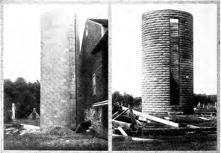
No trouble about concrete block silos standing when empty. H. M. Ashfy of Geneva, Iowa, owns the silo illustrated above; built by G. C. Harvey of Geneva.
