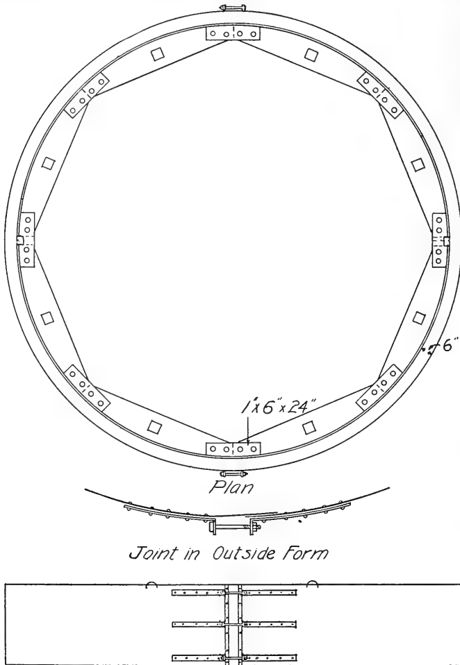
Plan of home-made wall forms, and details of outside form.
