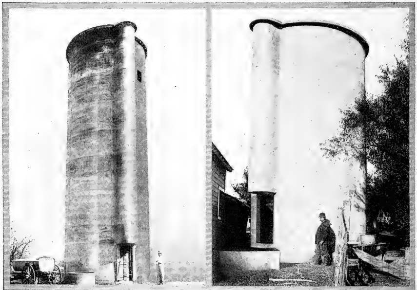
Reinforced concrete silos are popular in Kansas. This one is 12 feet by 32 feet; capacity 75 tons, on the Newtown Farm, Winfield, Kansas. Concrete chute and roof. Monsco forms used.
