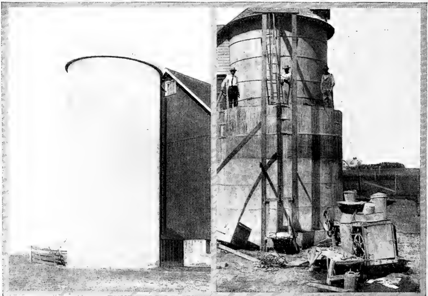
Concrete Roof constructed with Warford's forms. Silo on George Harvey's farm near Batavia, Illinois.
