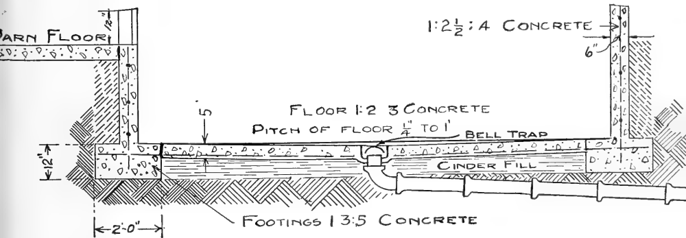
Concrete Silo Foundation or Footing and Concrete Floor, suitable for either monolithic or block silo, showing drain with bell trap; an important detail not to be needlessly overlooked.
