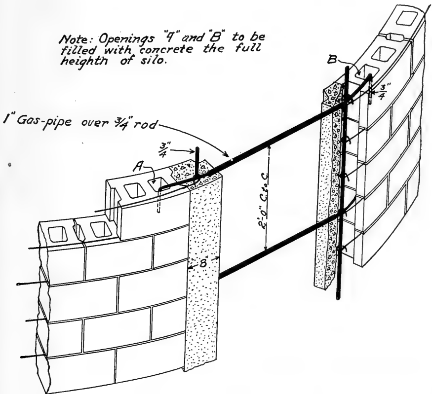
Continuous Door Opening for a Concrete Block Silo, showing the method of fastening reinforcing rods to the door frames and anchoring rods in the end blocks.
