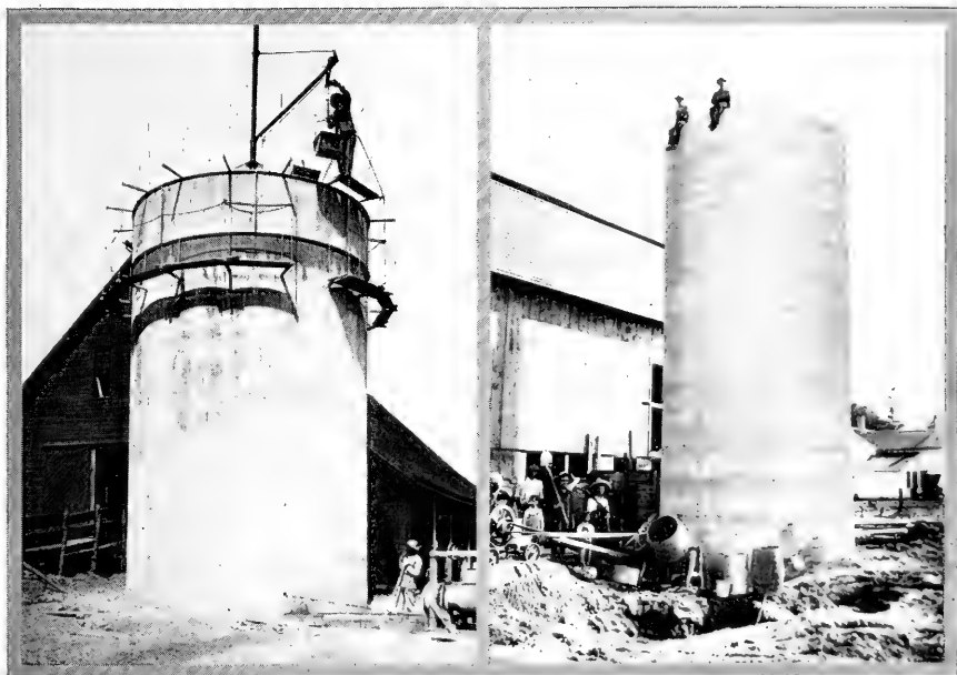
Wisconsin leads in cows and silos. Concrete silo on W. H. Butler's farm at Ripon, Wisconsin.
