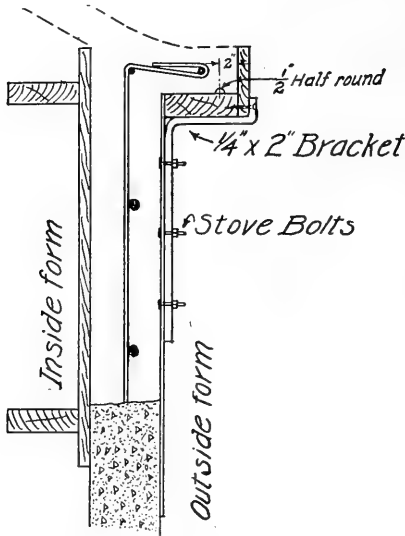
Forms in place for Top section and Cornice
