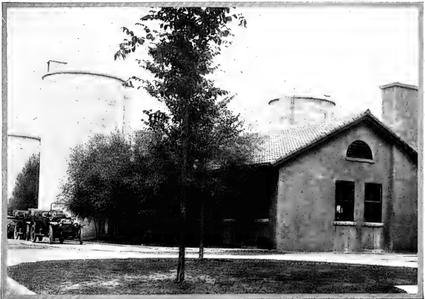
Two of the Six Reinforced Monolithic Concrete Silos at Arcady Farm, Lake Forest, Illinois, owned by Arthur Meeker.
