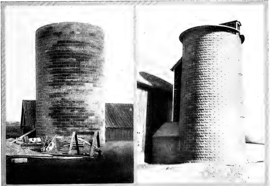
Excellent Concrete Block Silo in the heart of the butter district near Elgin, Illinois.
