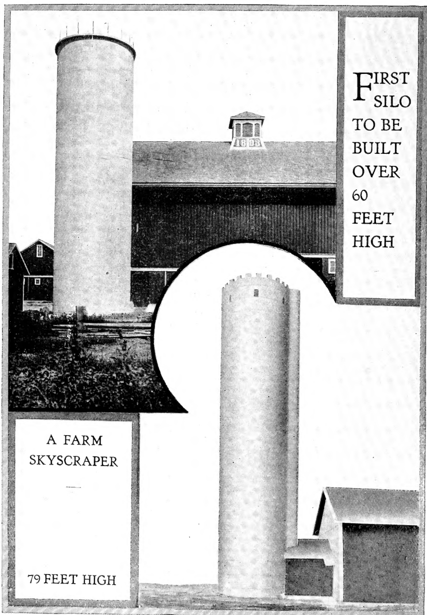
Wilson Bros. Concrete Silo, Sugar Grove, Illinois. Inside dimensions 16x64 feet; built in 1912. Polk forms used. W. H. Warford, contractor.
