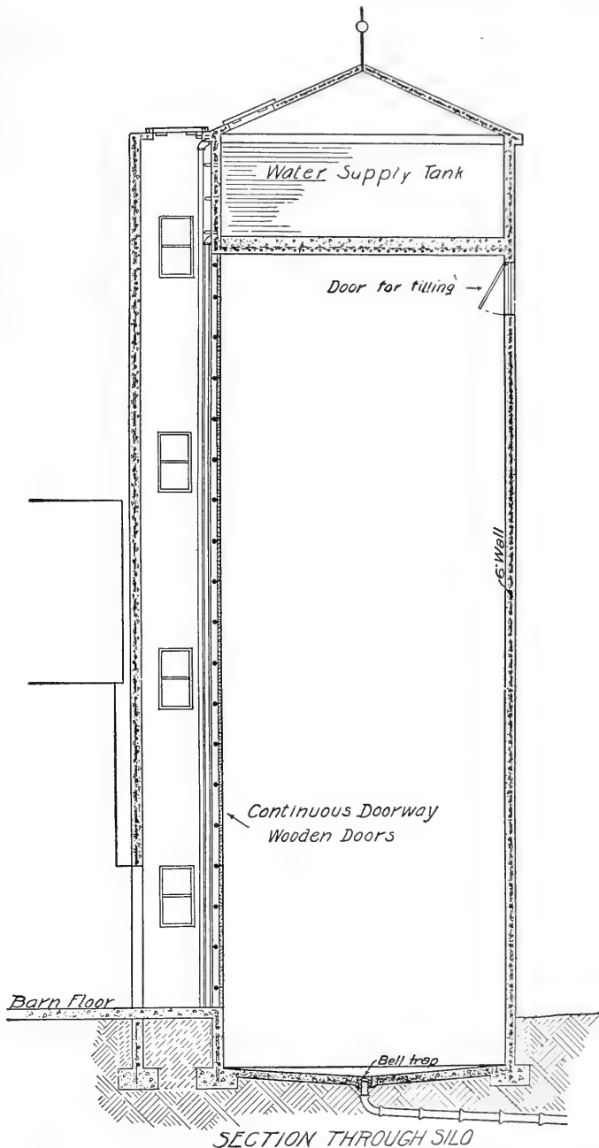
SECTION THROUGH SILO Sectional View of a Reinforced Monolithic Silo, showing water supply tank, roof, chute, concrete drain tile, and other essential details
