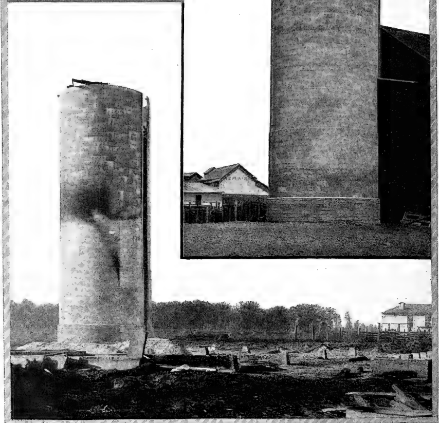
Before and After a Disastrous Fire on farm of A. B. Main, Delaware, Ohio; adjoining barn contained 180 tons of hay. Burned in Autumn of 1910; 530 tons of silage absolutely uninjured in silo, so that Mr. Main was not compelled to sacrifice 80 head of cattle which he was feeding at that time. The silo is 20x60 feet in size and was built by the Perfect Cement Silo and Cistern Co., Delaware, Ohio.
