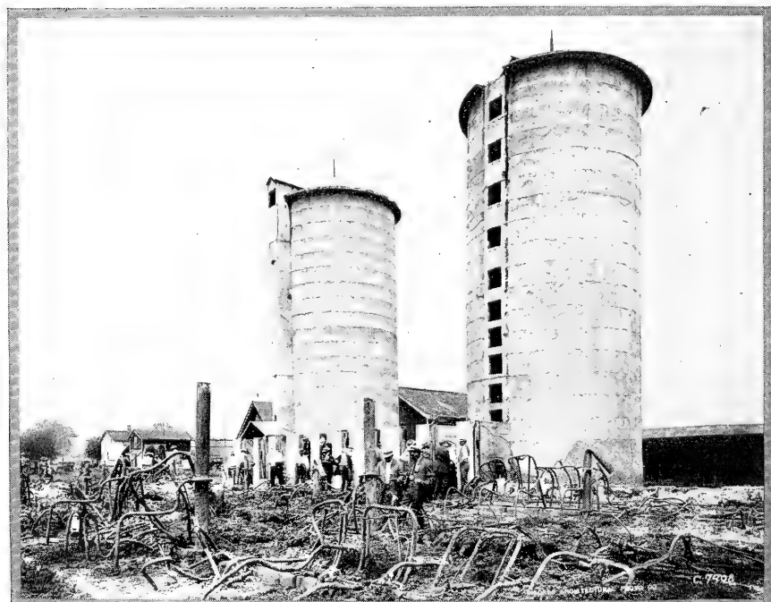
Concrete Silos on Dunham Farm, Wayne, Illinois, which successfully resisted a disastrous fire which destroyed the adjoining dairy barn in the summer of 1913.
