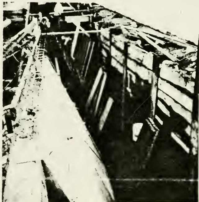
Earth support system at Washington Street Project, Everett, Mass.
