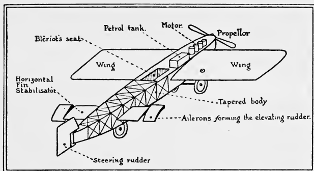
FIG. 75B. Blériot's monoplaner
