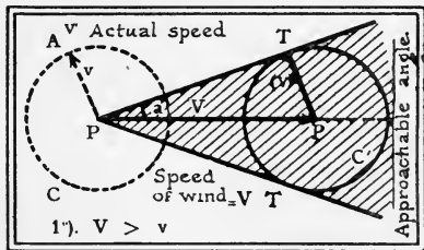
FIG. 21. Instance where the independent speed is less than the wind
