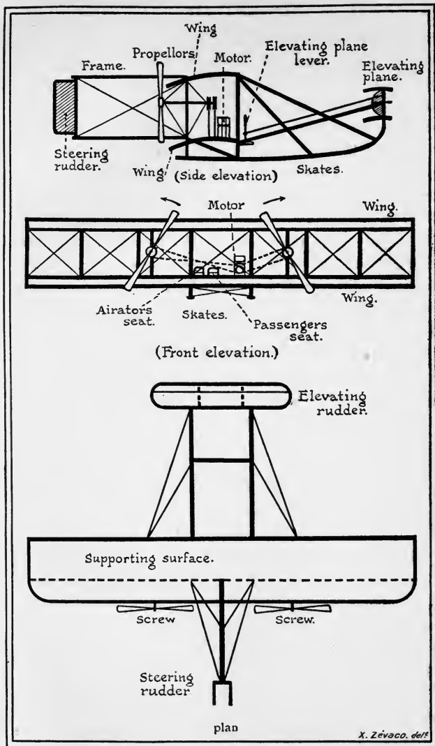
FIG. 71. The Wright Brothers' aeroplane
