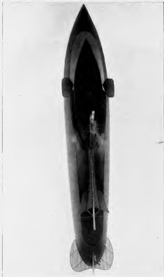
THE DIRIGIBLE "PATRIE" SEEN FROM BELOW. THE HORIZONTAL STABILISING EMPENNAGE CAN BE DISTINGUISHED AS WELL AS THE ELEVATING RUDDER IN FRONT
