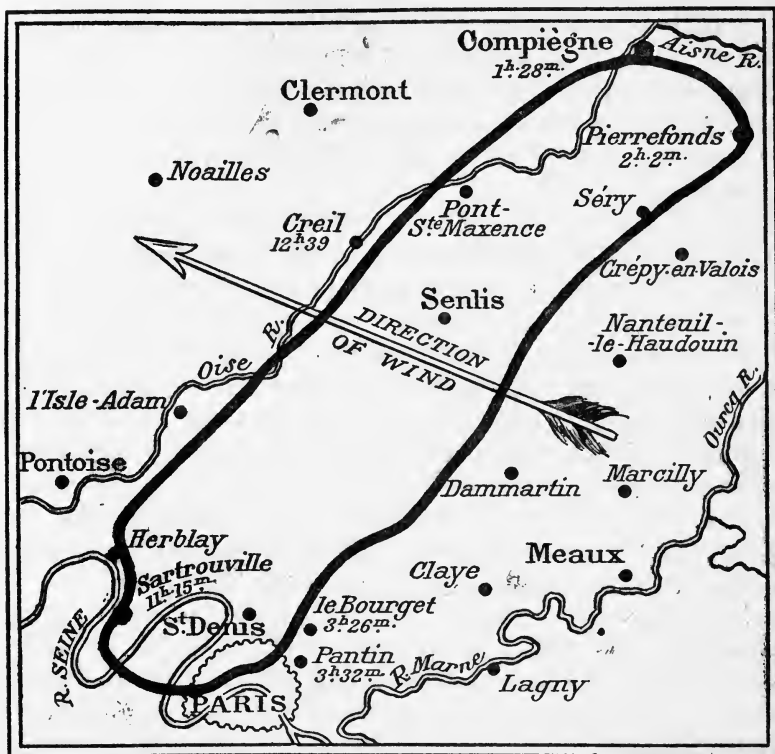
FIG. 26. Voyage of the Clément-Bayard (Nov. 1908)
