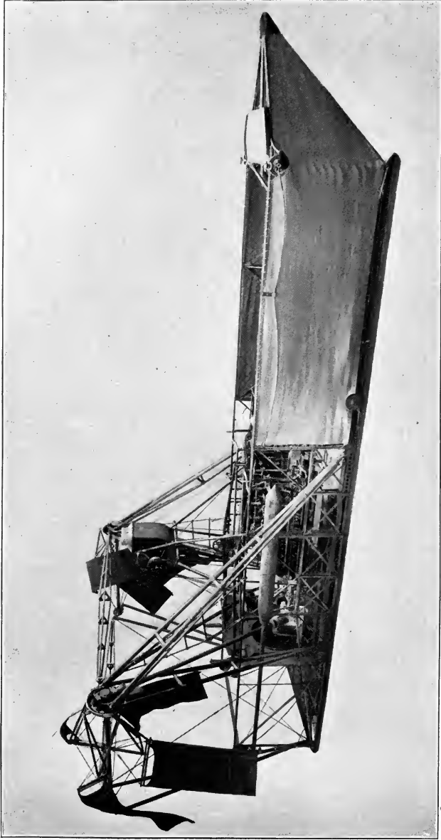
THE CAR OF THE "PARSEVAL," Showing blades of propellers, which fold over when at rest
