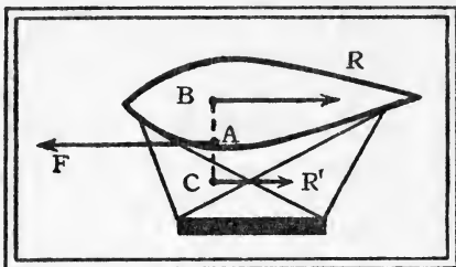
FIG. 16. Point for applying the propelling effort
