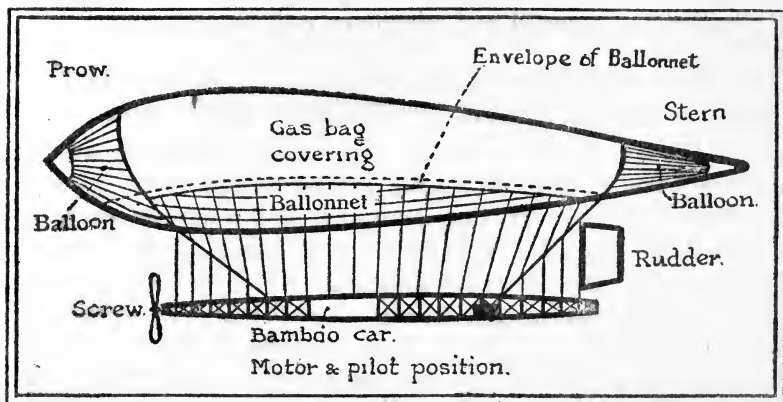
FIG. 30. The balloon La France , designed by Captains Renard and Krebs (1884)
