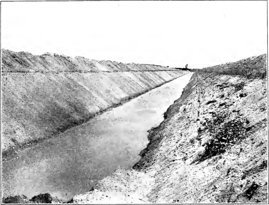
LOWER YELLOWSTONE PROJECT, MONTANA Finished Portion of the Main Canal. Sixty Miles in Length
