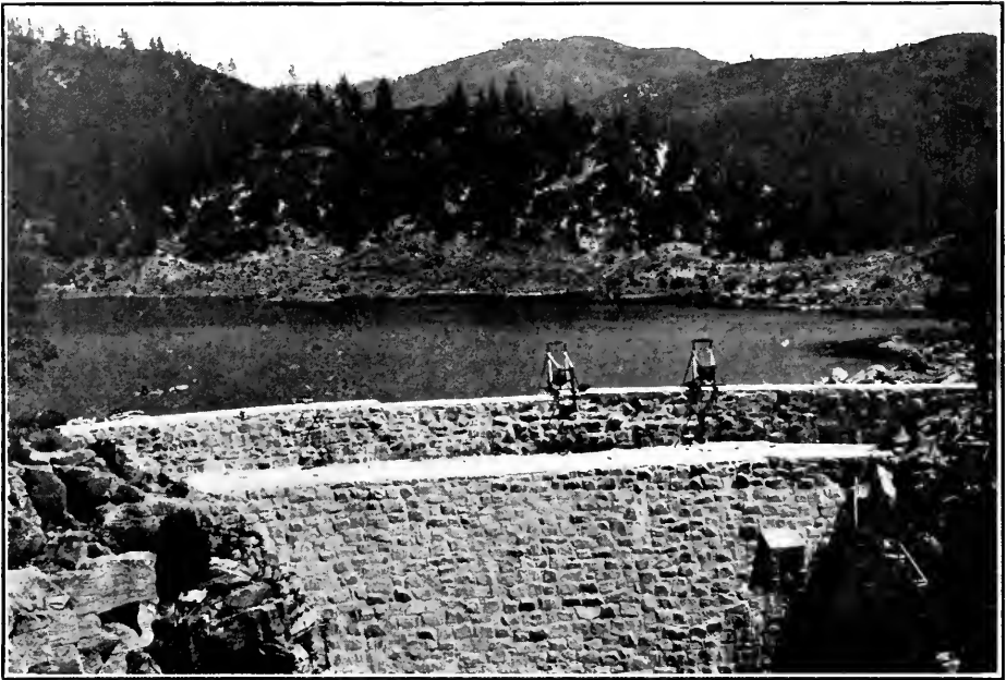
SCENE IN THE NEW CLEVELAND NATIONAL FOREST Hemeh Reservoir Dam. Altitude, 4,500 Feet
