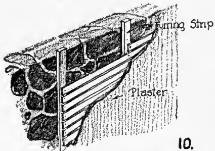
Wood furring Strips
