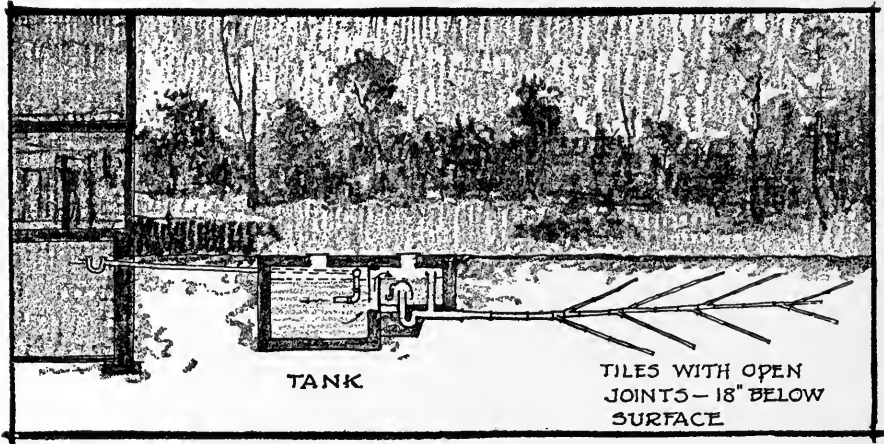
- SMALL SEWAGE DISPOSAL PLANT -
