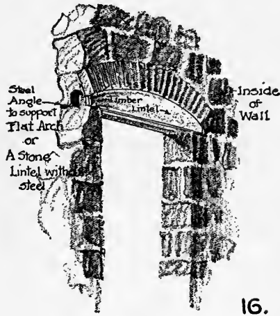
Lintel Construction
