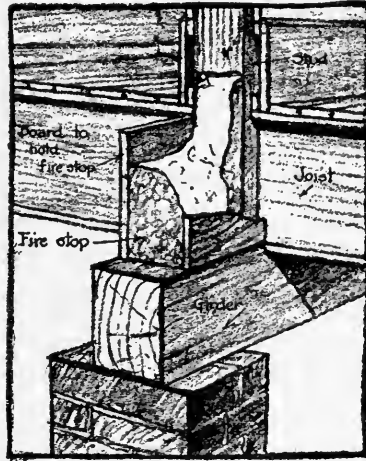
Fire stop for interior bearing partition of studs. Fig. 4
