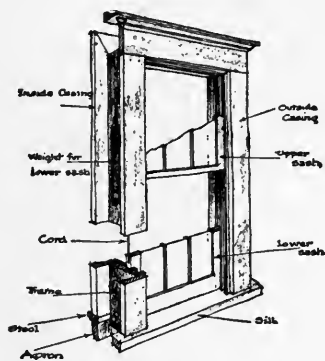
Modern Double-hung Window
