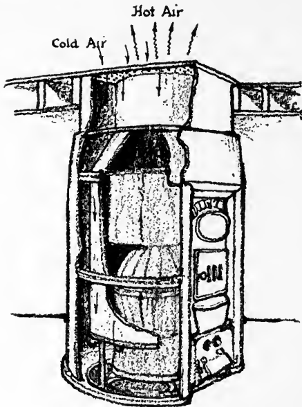
Pipeless Furnace
