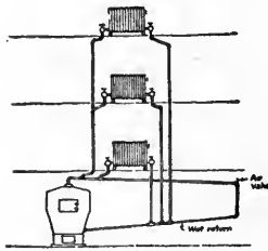
Steam Heat - Two-pipes
