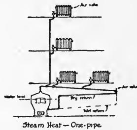
Steam Heat - One-pipe
