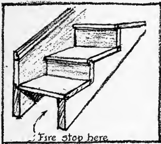
Fire stop here Fig 9
