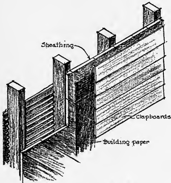
CLAPBOARDS OVER WOODEN STUDS
