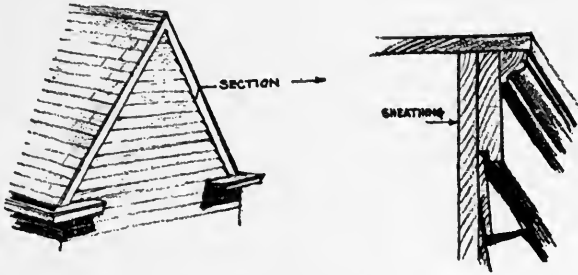
FLAT TREATMENT OF GABLE END.
