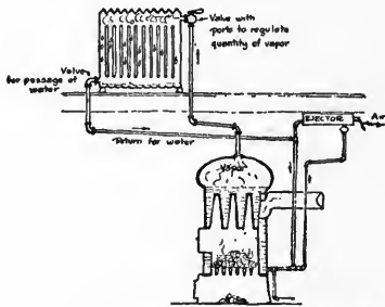
Simplified diagram of Vapor-vacuum system
