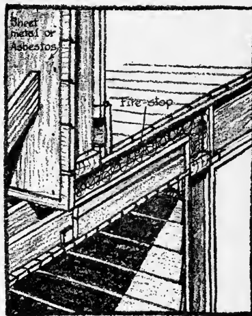
Fire stop in ceiling of porch roof where 2nd floor projects over. Fig 6
