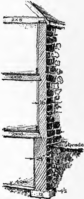
Thickness of rubble stone wall
