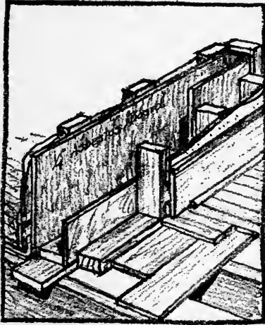
Fire-stop of sliding door Fig 7
