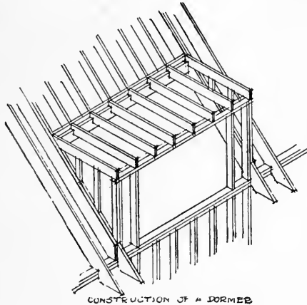
CONSTRUCTION OF A DORMER
