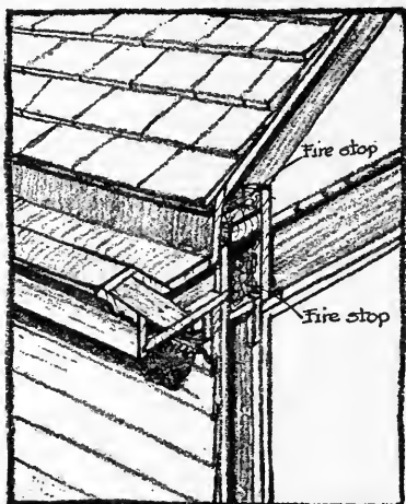
Fire stop at end of rafters Fig 5
