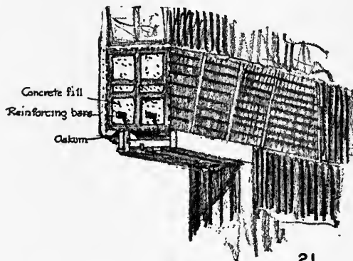
Construction of lintel
