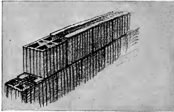
Showing the use of metal lath in the joints of vertically webbed hollow tile, to prevent the dripping of the mortar into the voids and also allow the separation of mortar joint
