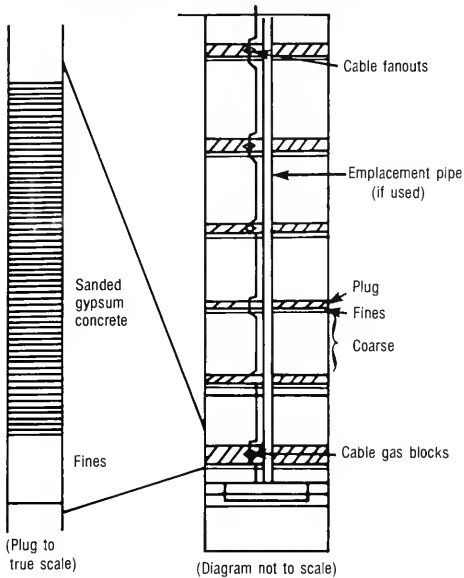
Figure 3-4—"Typical" Stemming Plan
