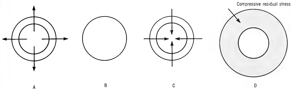
Figure 3-1—Formation of Stress "Containment Cage"
