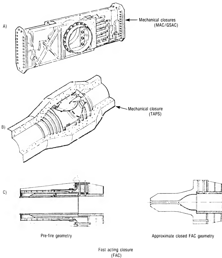
Figure 3-7—Vessel I Closures
