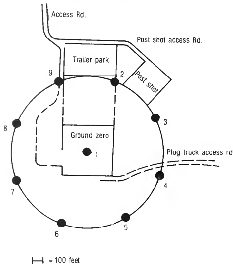
Figure 4-5—Typical RAMs Array for Vertical Drill-Hole Shot
