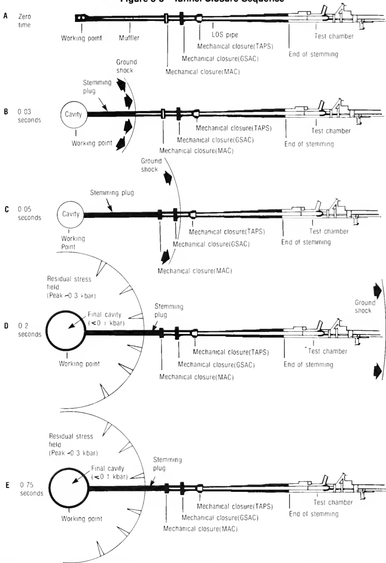
Figure 3-8—Tunnel Closure Sequence
