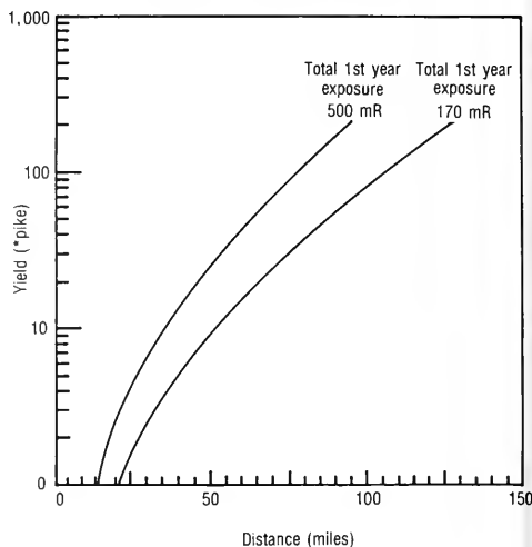
Figure 4-4—Yield v. Distance
