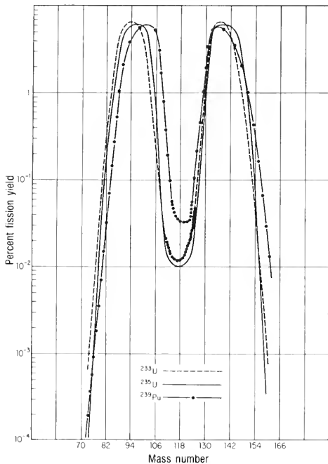
Figure 4-1—The Typical Bimodal Curve for Fission-Product Yield
