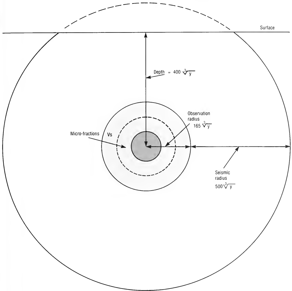
Figure 3-10—Radius of Decrease in Rock Strength
