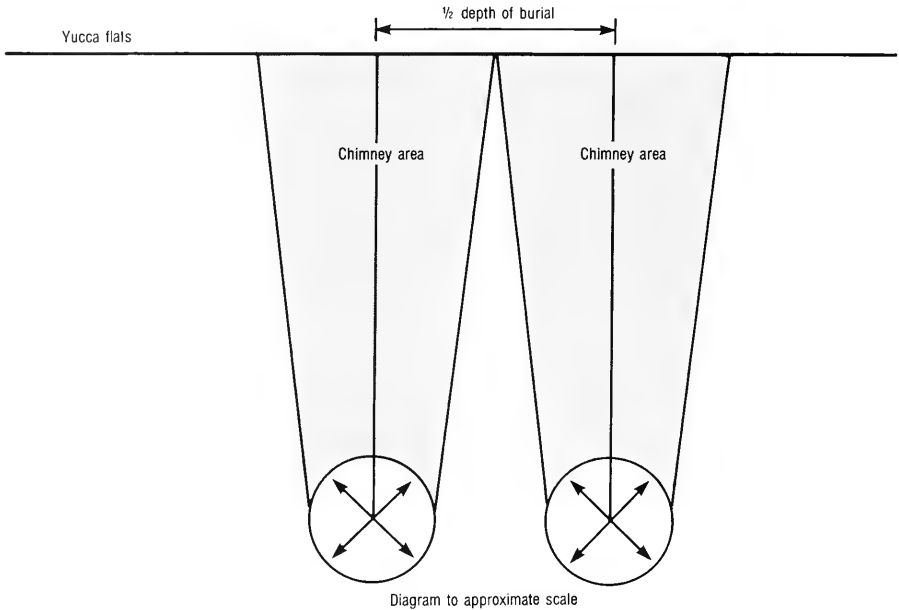
Figure 3-2—Minimum Shot Separation for Drill Hole Tests
