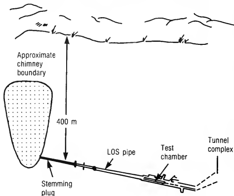
Figure 3-9—Typical Post-Shot Configuration
