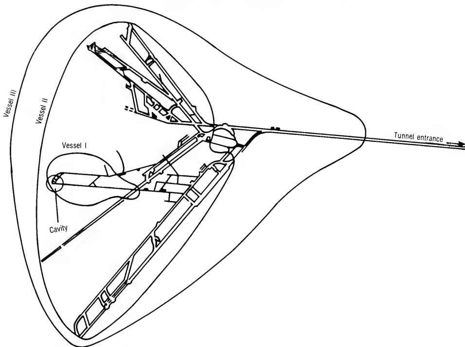
Figure 3-5—Three Redundant Containment Vessels (Plan View)
