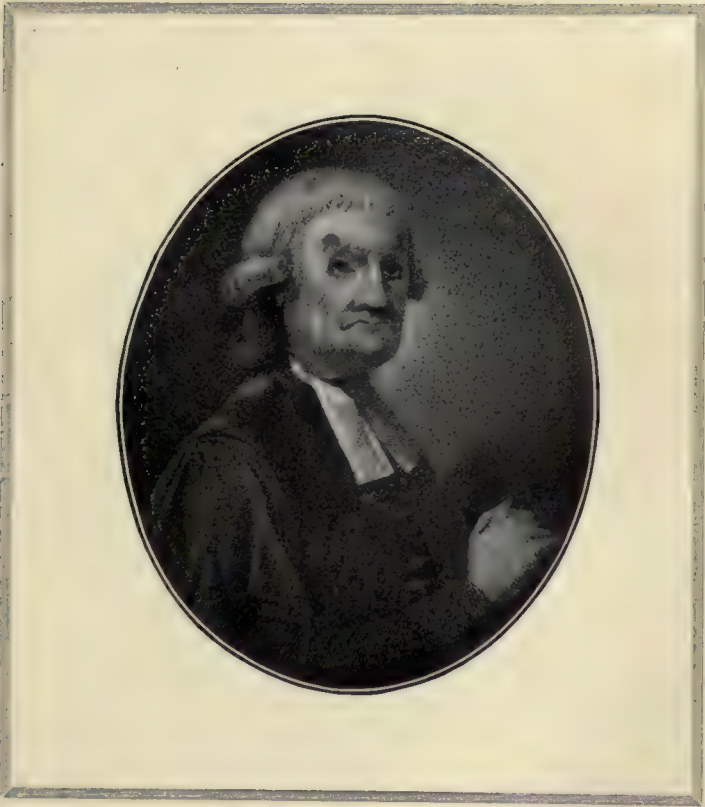
JOHN WITHERSPOON
