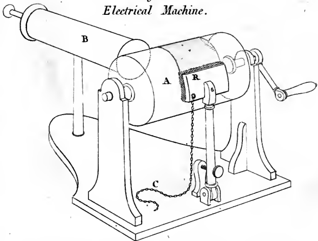
Fig. 3. A the Cylinder. B the Conductor. R the Rubber. C the Chain. Fig. 1. 2. & 4. Voltaic Batteries
