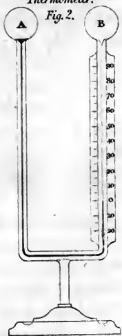
Differential Thermometer.
