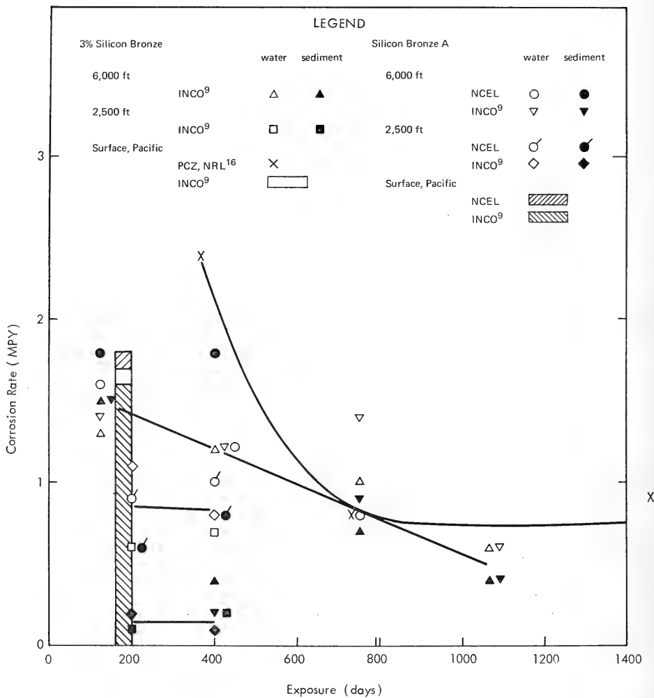
Figure 28. Corrosion rates of silicon bronzes.
