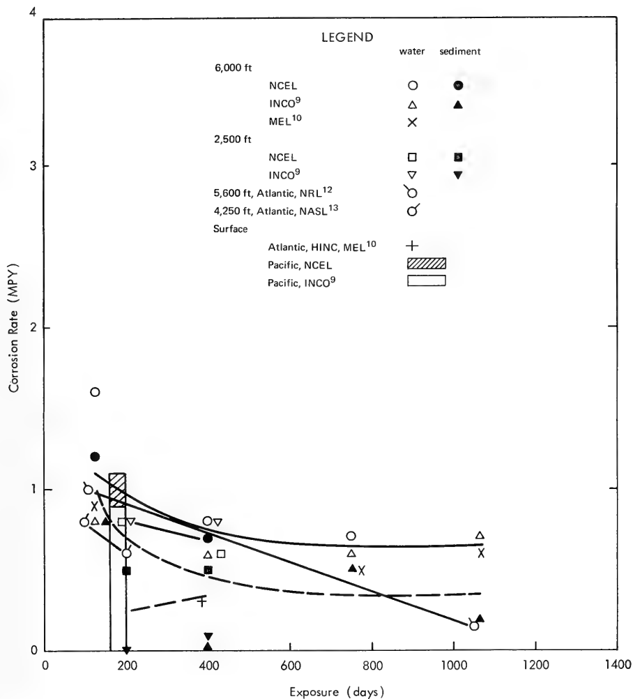
Figure 35. Corrosion rates of 90-10 copper-nickel alloy.
