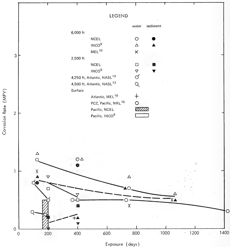
Figure 36. Corrosion rates of 70-30 copper-nickel alloy containing 0.5% iron.
