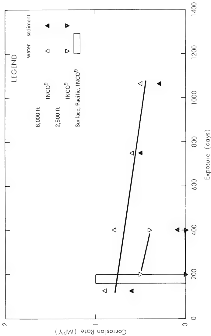
Figure 43. Corrosion rates of 62 Cu - 25 Ni - 8 Zn - 5 Pb alloy.
