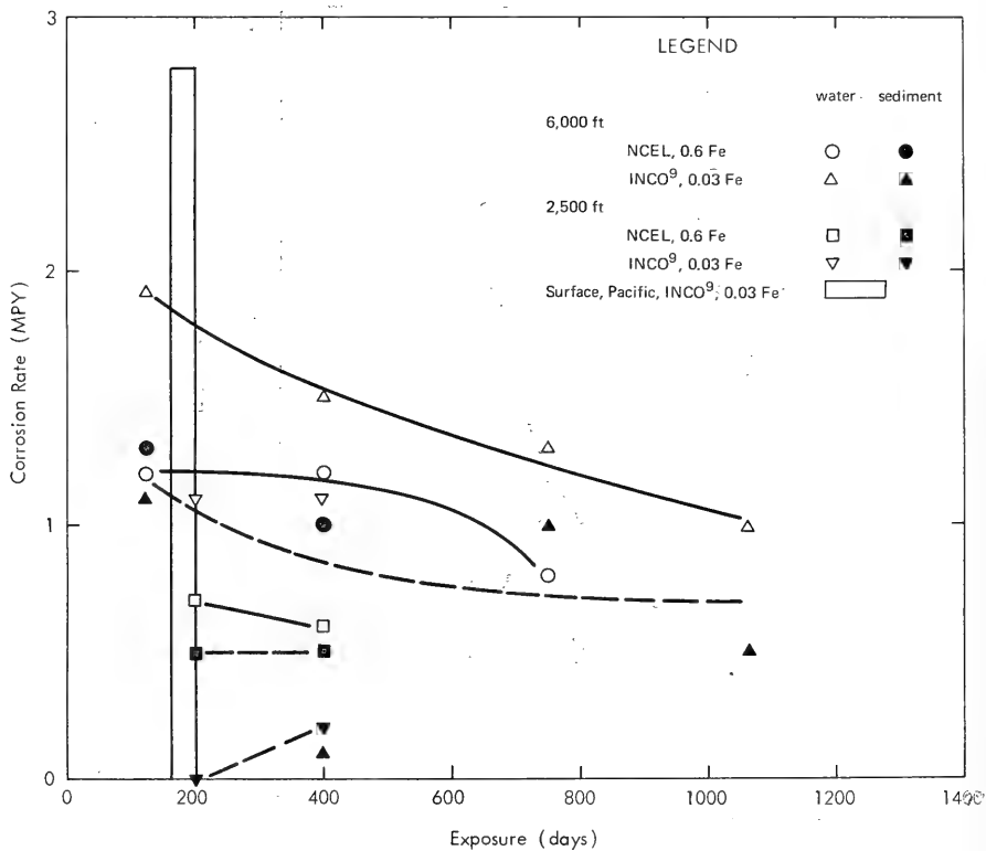
Figure 40. Corrosion rates of 80-20 copper-nickel alloy.
