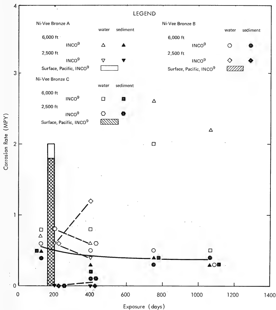
Figure 29. Corrosion rates of Ni - Vee bronzes.
