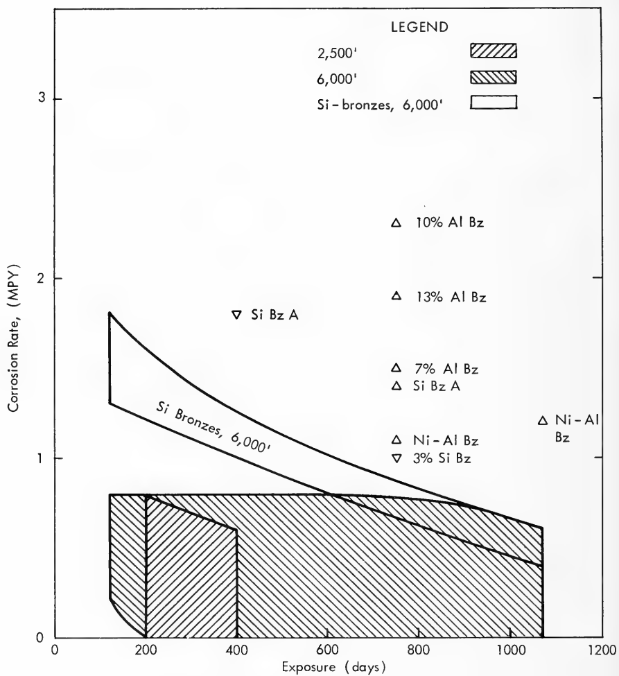
Figure 30. Corrosion rates of bronzes.
