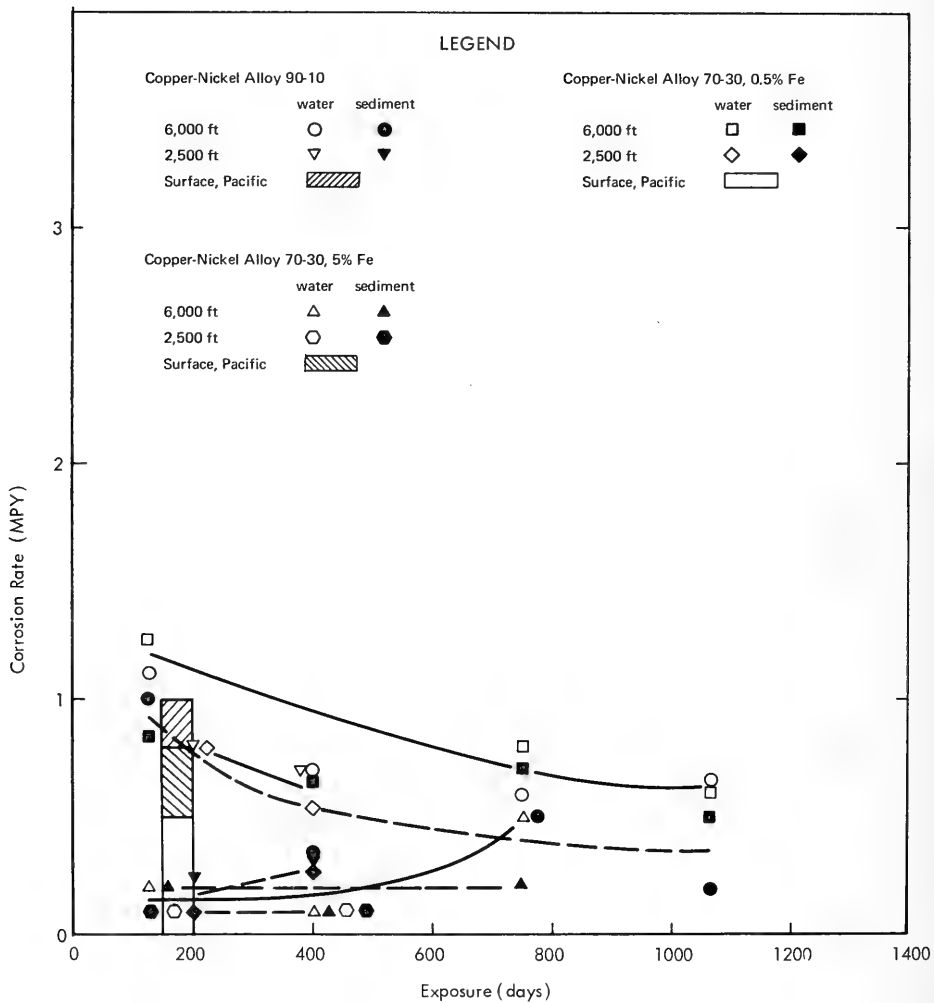
Figure 38. Corrosion rates of copper-nickel alloys.
