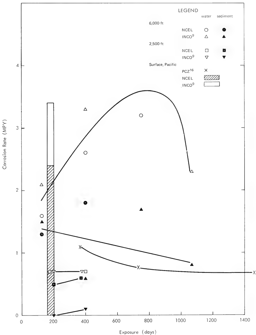
Figure 9. Corrosion rates of Muntz Metal.
