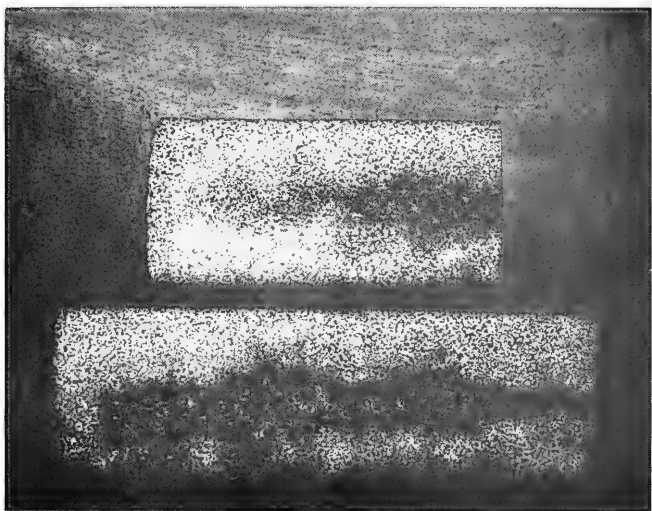
Figure 14. Dezincified nickel-manganese bronze, 751 days, 5640 feet. X3.
