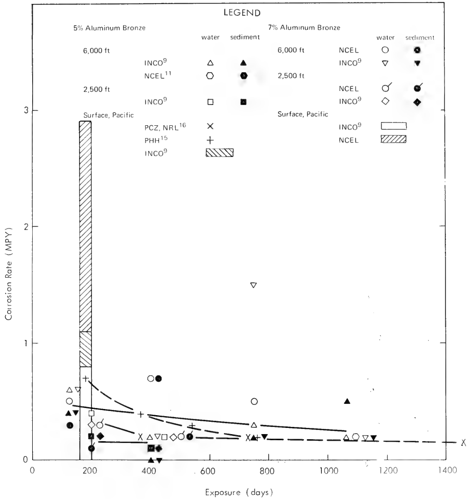
Figure 25. Corrosion rates of wrought aluminum bronzes.
