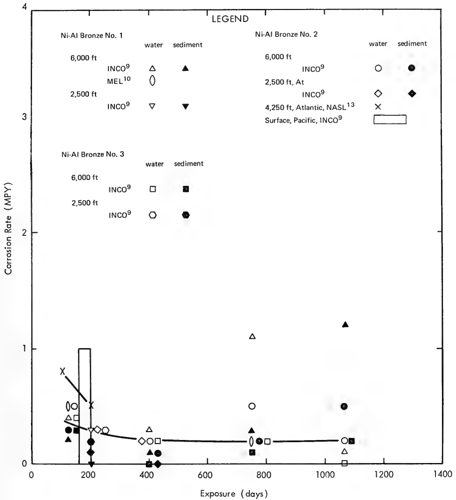
Figure 27. Corrosion rates of nickel - aluminum bronzes.
