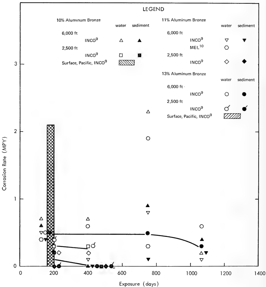
Figure 26. Corrosion rates of cast aluminum bronzes.
