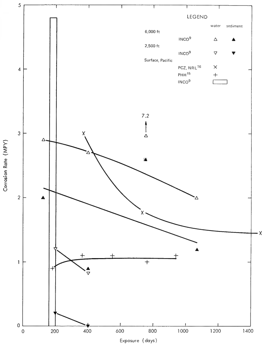
Figure 12. Corrosion rates of manganese bronze.
