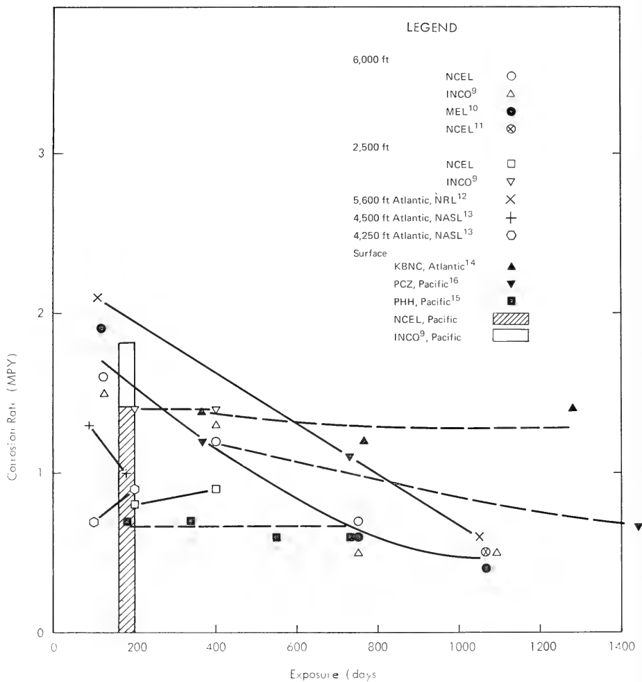
Figure 3. Corrosion rates of copper in sea water.
