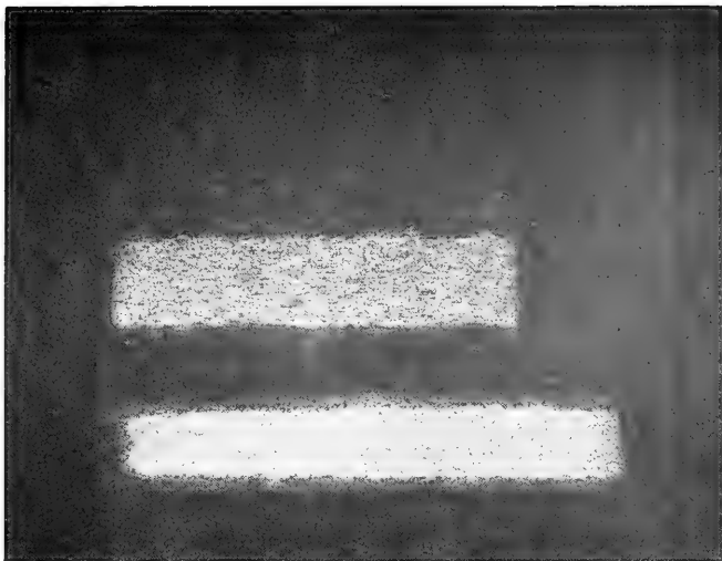
Figure 10. Dezincified Muntz metal, 751 days, 5640 feet. X3.
