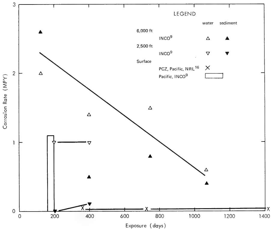
Figure 42. Corrosion rates of 65 - 18 nickel - silver alloy.
