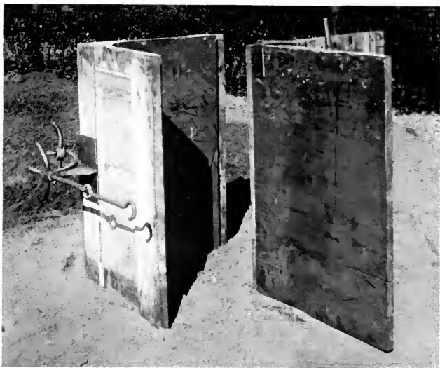
MARK V SHUTTERING.
