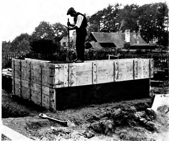
THE BEGINNING OF A PISE FRUIT-HOUSE
