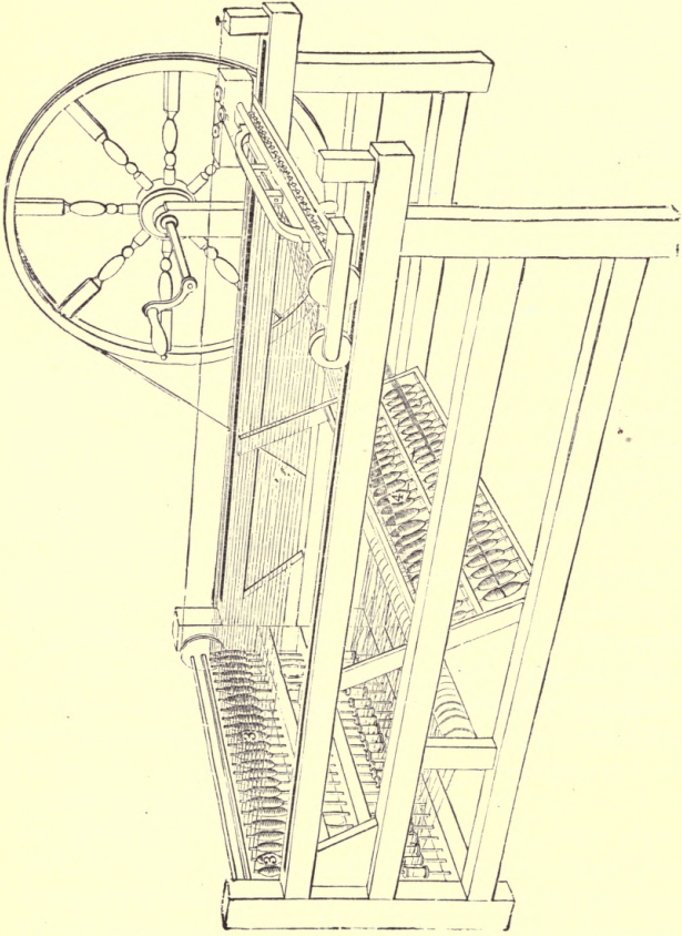
HARGREAVES'S SPINNING JENNY.
