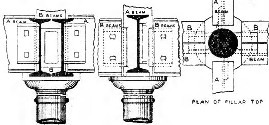
DETAILS OF PILLARS
