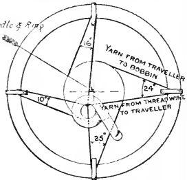
INCORRECT SETTING.
