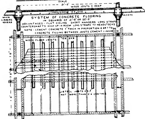
SYSTEM OF CONCRETE FLOORING FOR COTTON SPINNING MILL.
