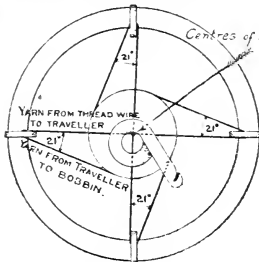
CORRECT SETTING.
