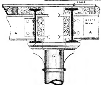
DETAIL SHOWING CONNECTION OF 2-16x5 1/2 BEAMS ON PILLAR TOP
