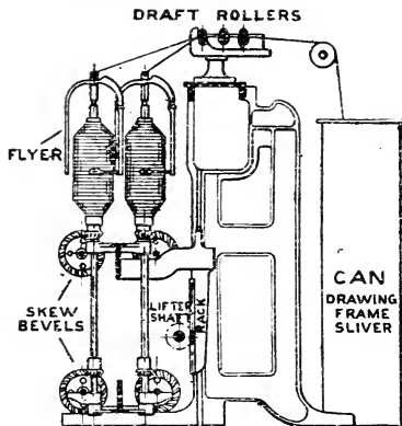
SECTION OF SLUBBING FRAME.
