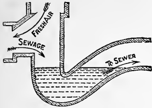
BUCHAN'S No. 1 TRAP.
