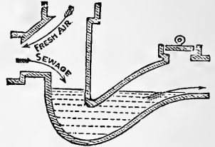
BUCHAN'S No. 2 TRAP.
