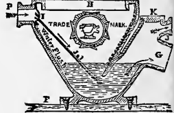
No. 1002. P. Trap Style, 'Carmichael' Closet. (Simple and Efficient.)
