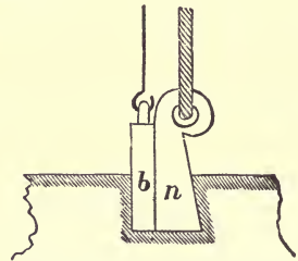
FIG. 119—A line attached to the straight piece, b , admits of the latter being drawn out, allowing the piece, n , to be removed.
