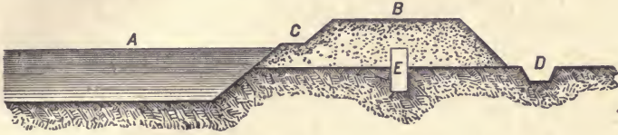
FIG. 233.—A, water-way. B, towpath. C, berm. D, side-drain. E, puddling of clay.
