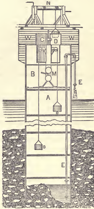
FIG. 151—Represents vertical section of a pneumatic pile.
