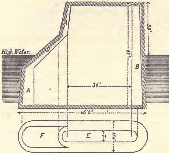
FIG. 160—Represents longitudinal section, elevation, and plan of a pier of the Potomac aqueduct bridge.
