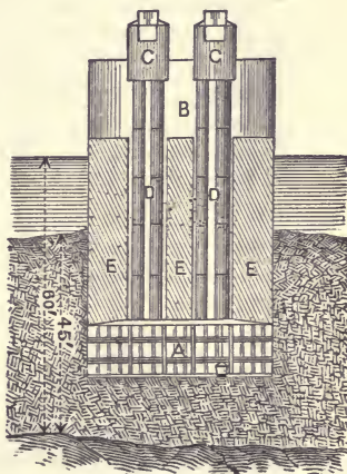
FIG. 153—Represents a vertical section of caisson and masonry of pier during the process of sinking.
