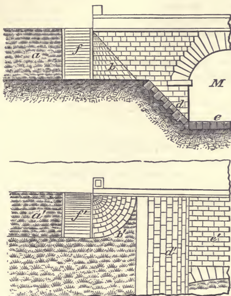
FIG. 164.—Plan and elevation showing a method of arranging the embankments where there are no wing-walls.
