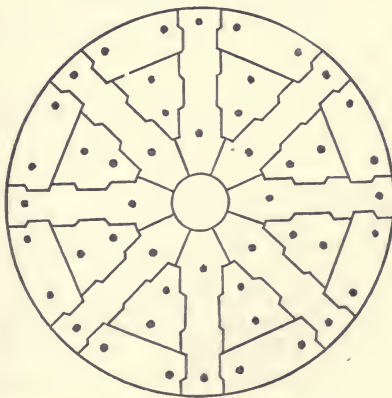
FIG 115.—Plan of twenty-second course, showing the method of dovetailing the stones.
