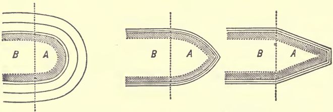
FIG. 159.—A, horizontal sections of starling. B, same of pier.
