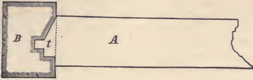
FIG. 52.—A, the cross-beam. B, cross-section of main beam. t, the tenon.
