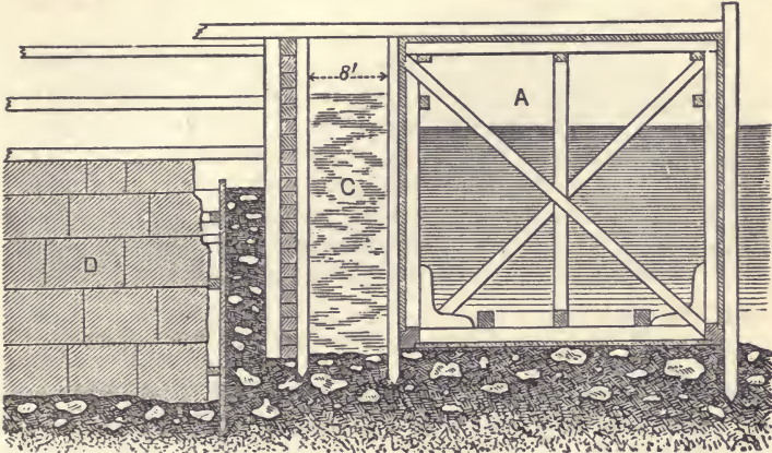
FIG. 149—Represents a cross-section of a caisson dam. A, cross-section of caisson. C, puddling. D, foundation courses of the pier.
