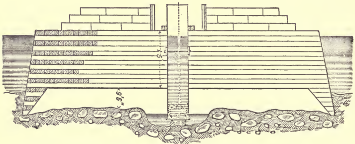
FIG. 155—Represents section through water shaft of the Brooklyn caisson, showing method of removing boulders or other heavy materials.
