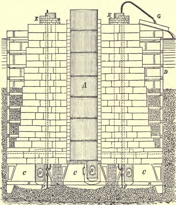
FIG. 154 —Represents a section of the caisson used in construction of east pier of the bridge over the Mississippi River, at St. Louis, Mo.
