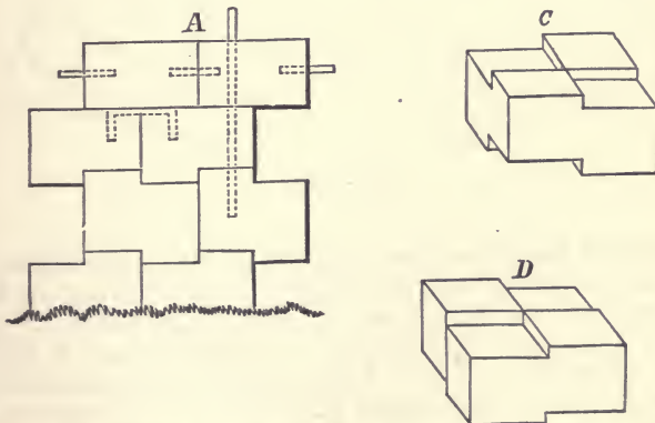
FIG. 112—Represents an elevation A, and perspective views C and D, of two of the blocks of a wall in which the blocks are fitted with indents, and connected with bolts and cramps of metal.
