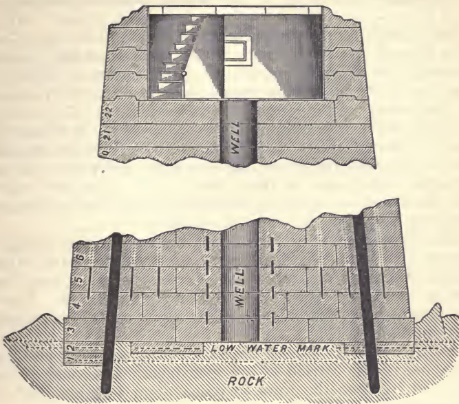
FIG. 114.—Vertical section showing foundation courses, metal fastenings, and the first story above the foundation courses.
