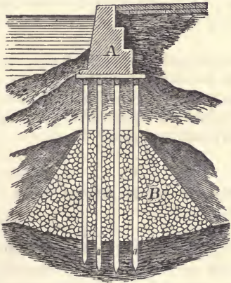
FIG. 145—Represents the manner of using loose stone to sustain piles and prevent them from yielding laterally.
