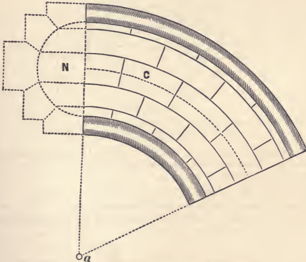
FIG. 82.—N, right section of an annular arch. C, plan of soffit.
