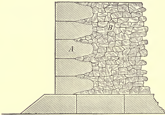
Fig. 110—Represents a section of wall with facing of ashlar and a backing of rubble.
