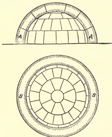
FIG. 83.—A, vertical section and elevation of a circular dome. B, B, horizontal section and plan of its soffit.
