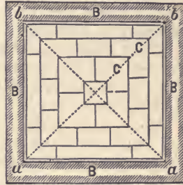
FIG. 81—Represents a horizontal section through the walls supporting the arch and plan of the soffit of a cloistered arch. B, B, the walls of the enclosure or abutments of the arches. ab , curves of intersection of the soffits. c, c , groin stones.
