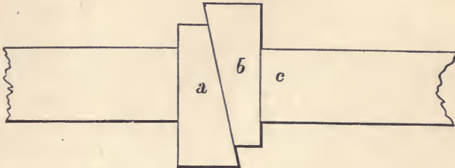
FIG. 63—Represents the folding wedges , a , b , let into a notch in the beam c .
