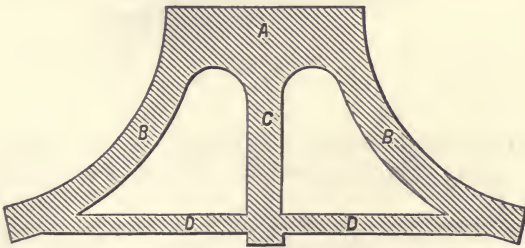
FIG. 162—Represents a horizontal section of an abutment, A, with curved wing-walls, B, B, connected with a central buttress, C, by a cross tie-wall, D.
