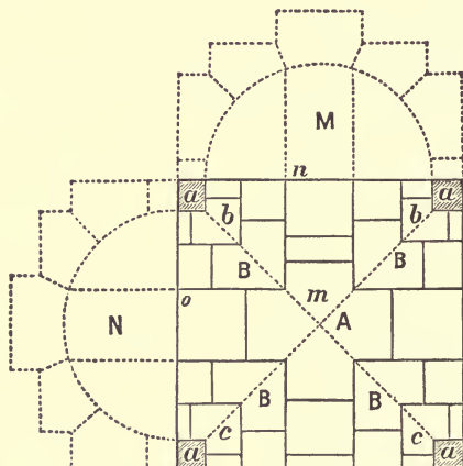
FIG. 80—Represents the plan and the right sections M and N of the cylinders forming a groined arch.
