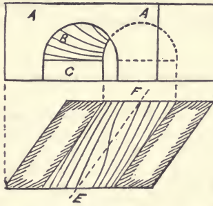
FIG. 130.—Elevation and plan of an oblique cylindrical arch, with the edges of the coursing joints constructed by the logarithmic method.
