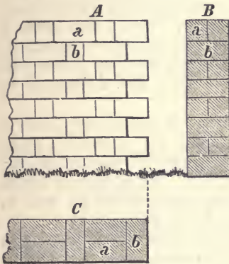
FIG. 111—Represents an elevation A, vertical section B, and horizontal section C, of a wall arranged as headers and stretchers.
