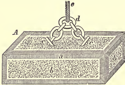
FIG. 117—Represents a perspective view of the tacking for hoisting a block of stone, A, with draughts around the edges of its faces, and the intermediate space axed or knotted.
