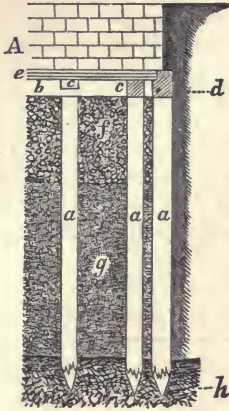
FIG. 144—Represents a grillage and platform fitted on piles.
