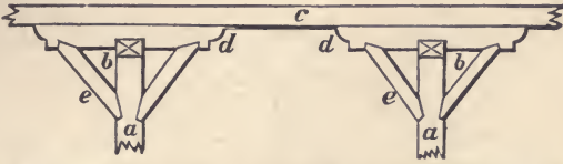
FIG. 66—A horizontal beam, c , resting on vertical posts, a a , with corbels, d d , and struts, e e .
