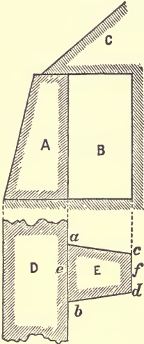
FIG. 94—Represents a section A and plan D of a wall, and an elevation B and plan E of a trapezoidal counterfort.
