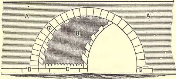
FIG. 131.—Elevation of an oblique cylindrical arch with helical joints. a , voussoirs of cut stone. c, c , bottom course of stone voussoirs cut to receive the brick courses. C , face of the abutment. D , ends of the abutments.
