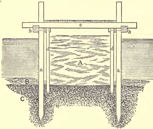
FIG. 48—Represents a section of a coffer-dam. a , common piles. b , wale or string pieces. c , cross pieces. d , sheet piles. A, puddling. B, mud and loose soil. C, firm soil.
