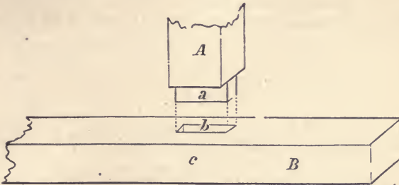
FIG. 50—Represents a mortise and tenon joint when the axes of the beams are perpendicular to each other. a , tenon on the beam A . b , mortise in the beam B . c , pin to hold the parts together.
