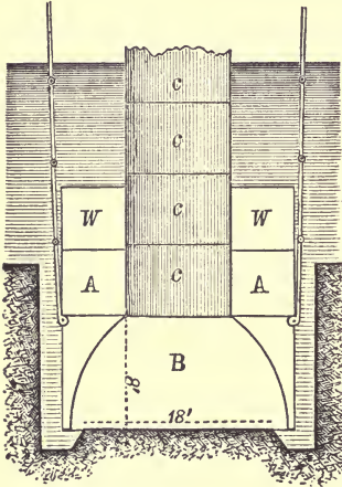
FIG. 156—Represents section of movable pneumatic caisson. B, working chamber. A, chamber for water, or for compressed air. W, chamber for iron ballast. c, c, elevation of lengths of the iron cylinder.
