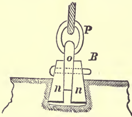
FIG. 118—Represents the common iron lewis B.
