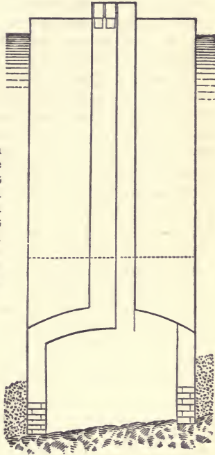
FIG. 152—Represents a longitudinal section through the axis of the cylinder. The cylinder was 37 feet in diameter, about 100 feet high, made of boiler iron, and weighed nearly 300 tons. The rock on which it was to rest was about 90 feet below the surface of the water, overlaid with about 20 feet of loose sand and mud. The rock surface had a slight slope, to which the bottom of the cylinder was made to fit.
