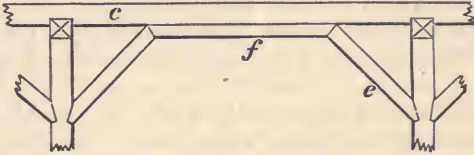
FIG. 67—A horizontal beam, c , strengthened by a straining beam, f .
