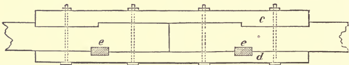
FIG. 44—Represents a fished joint in which the side pieces c and d are either let into the beams or secured by keys e, e .
