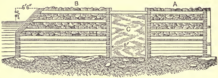
FIG. 150—Represents a cross-section of a crib-work dam. A, inner row of cribs. B, outer row of cribs. C, puddling.
