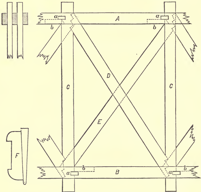
FIG. 184—Represents a panel of Long's truss.
