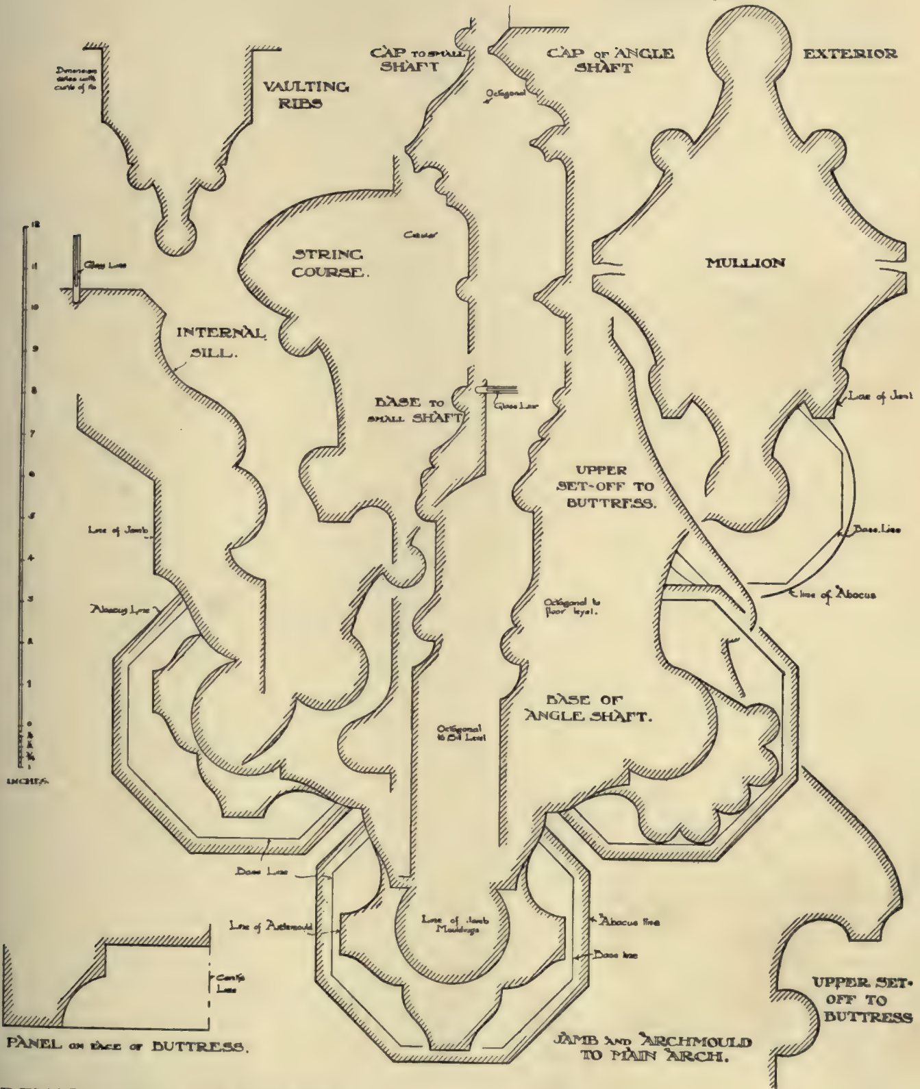
DETAILS OF BAY WINDOW
