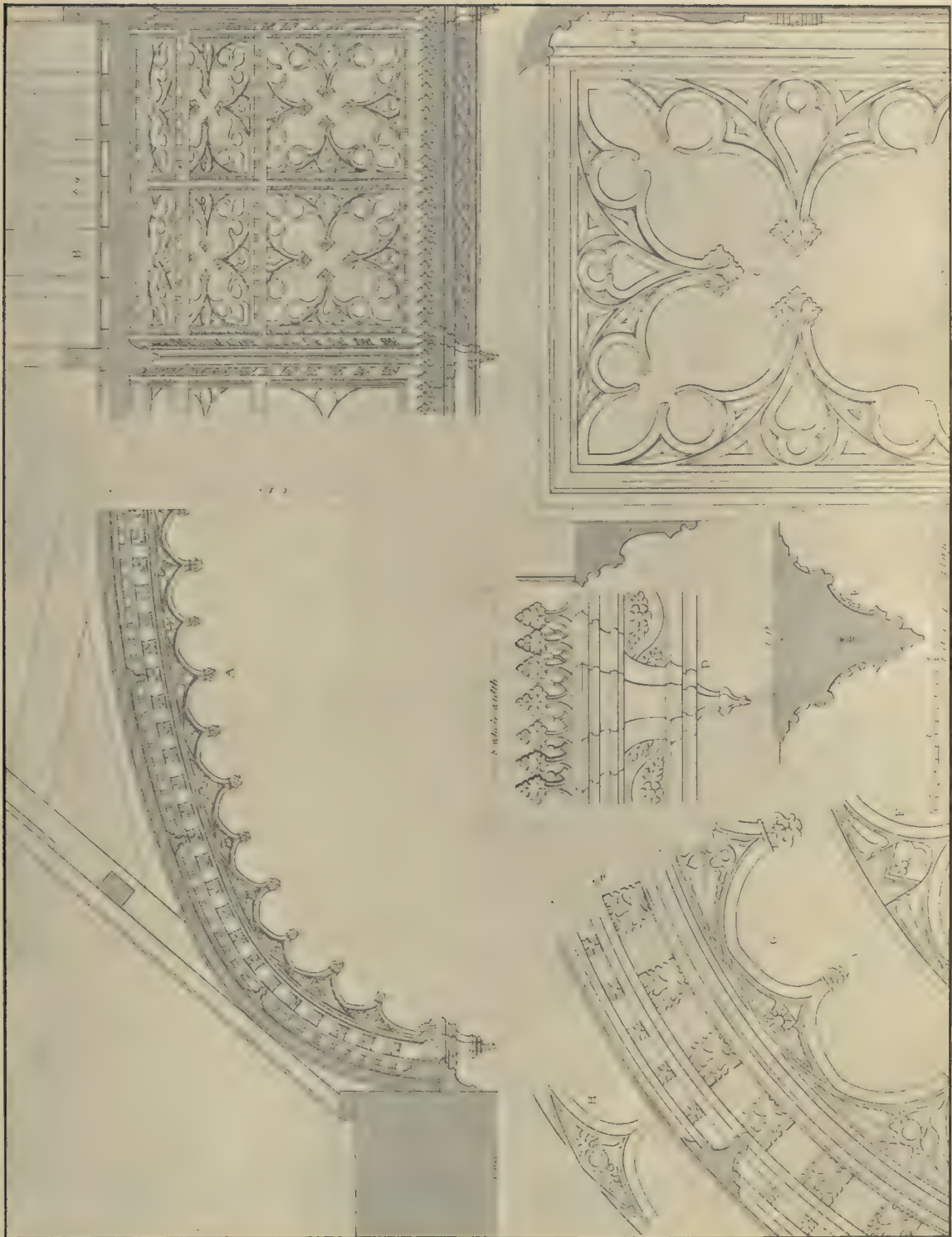
DETAILS OF ROOF OVER GREAT CHAMBER (PUGIN), 1825
