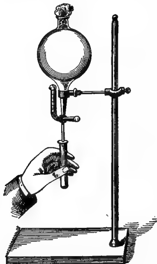
FIG. 14.—Apparatus for delivering measured quantities of media into tubes.
