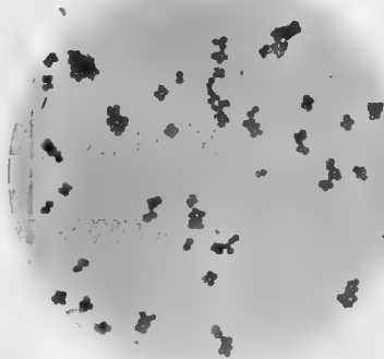
FIG. 70. — Micrococcus tetragenus ; young culture on agar, showing tetrads. Stained with weak carbol-fuchsin. \times 1000 .
