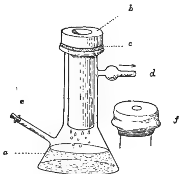
FIG. 42.—Muencke's modification of Chamberland's filter.
