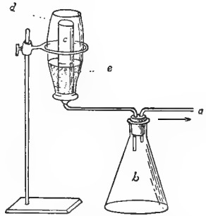
FIG. 40.—Chamberland's bougie arranged with lamp funnel for filtering a small quantity of fluid.
