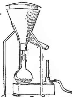
FIG. 9.—Hot-water funnel.
