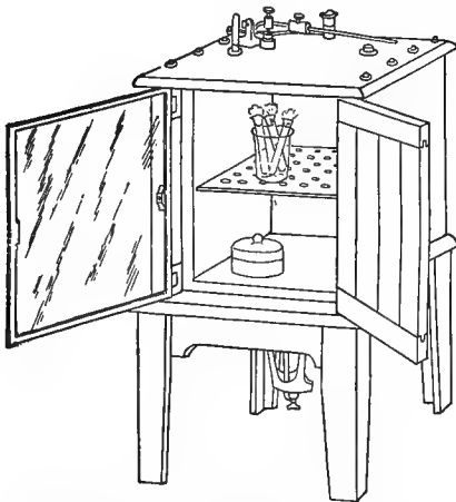
FIG. 48.—Hearson's incubator for use at 37° C.
