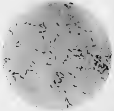
FIG. 95.—Smegma bacilli. Film preparation of smegma. Ziehl-Neelsen stain. \times 1000 .
