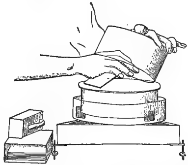
FIG. 21. — Koch's levelling apparatus. Hands shown in second position just as the plate is lowered on to the ground-glass surface. By executing the transference of the plate from the box in this way, the surface which was undermost in the latter is uppermost in the leveller, and thus never meets a current of air which might contaminate it.
