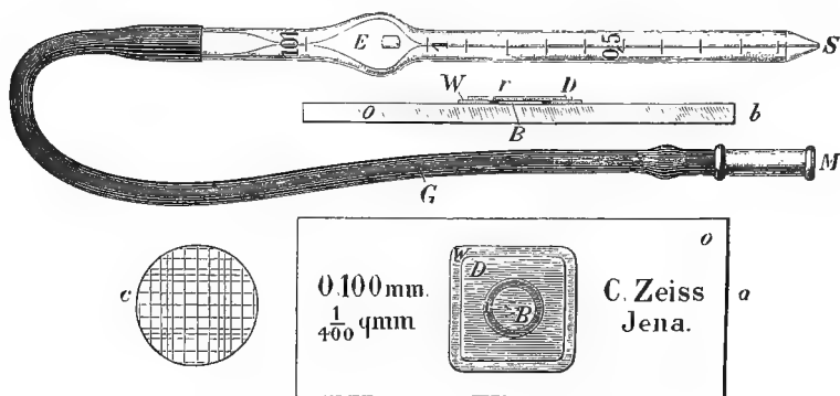
FIG. 44.—THOMA'S HÆMOCYTOMETER.
