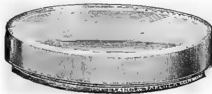
FIG. 19.—PETRI'S DISH.
