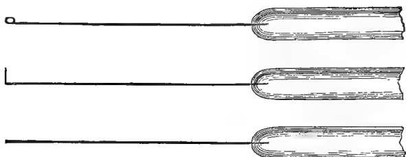
FIG. 8.—PLATINUM NEEDLES.
