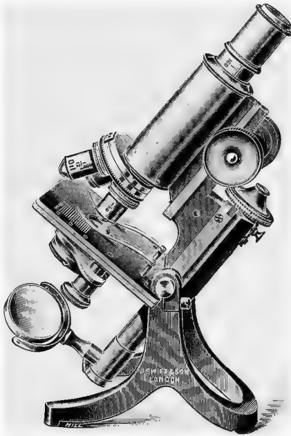
FIG. 2.—BACTERIOLOGICAL MICROSCOPE.
