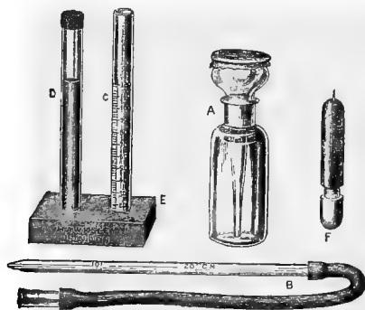
FIG. 42.—GOWERS' HÆMOGLOBINOMETER.
