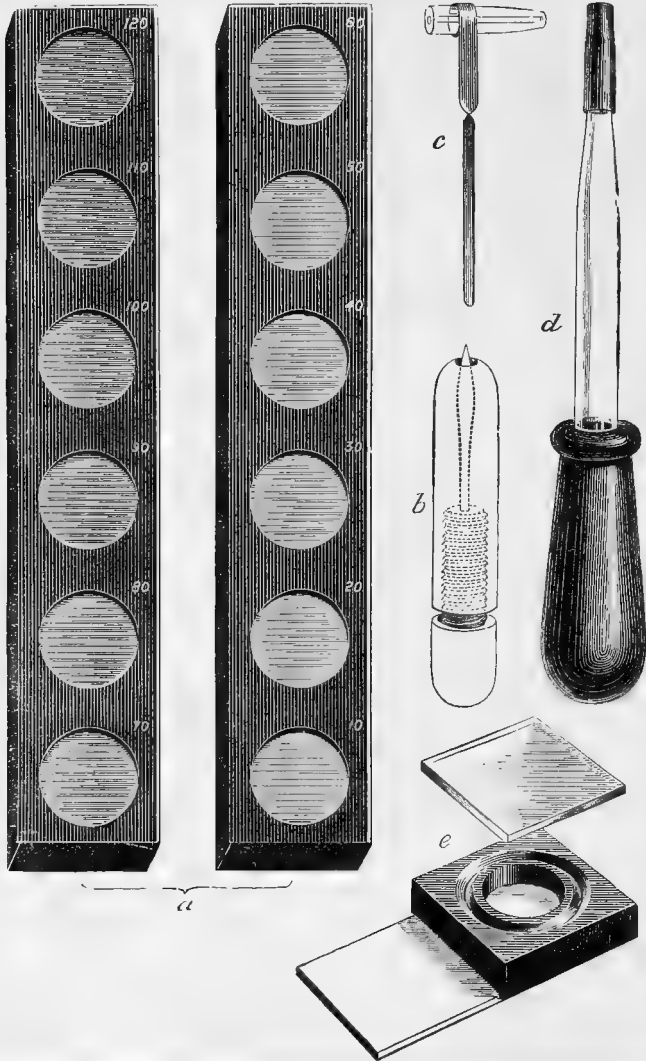
FIG. 43.—OLIVER'S HÆMOGLOBINOMETER.
