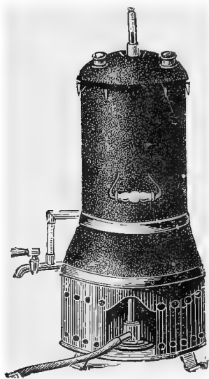
FIG. 7.—STEAM STERILIZER.
