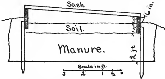
Figure 25.—Cross section of hotbed.
