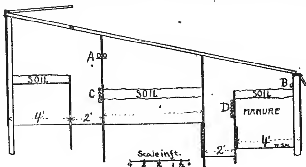
Figure 33.—Cross section of lean-to greenhouse.
