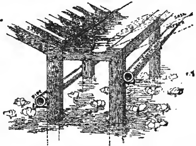
Figure 32.—Valley in market gardeners' greenhouse showing the way the sashbars are attached to the plate.
