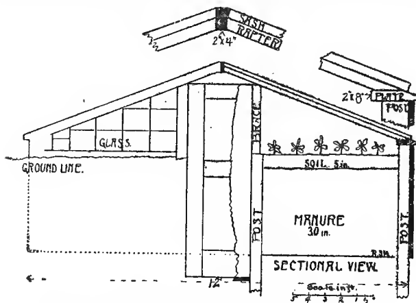
Figure 29.—Sectional view of hotbed greenhouse.
