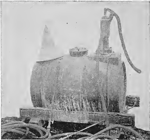
Figure 15 —Barrel spray pump, showing cone shaped strainer to the left.
