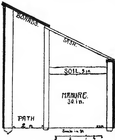
Figure 30.—Cross section of lean-to greenhouse hotbed.
