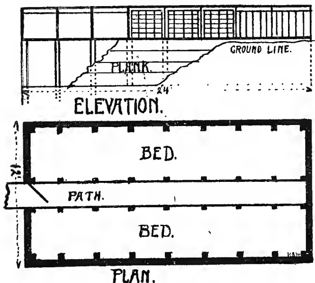
Figure 28.—Plan and elevation of hotbed greenhouse.
