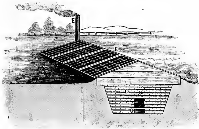
Figure 26.—Fire hotbed.
