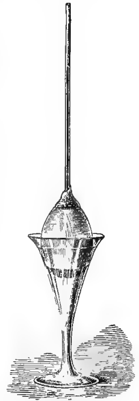
FIG. 40.—EGG PREPARED SO AS TO ILLUSTRATE OSMOTIC ACTION. (Flint.)
