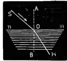
FIG. 369.—DIAGRAM ILLUSTRATING REFRACTION OF LIGHT. (Ganot.)
