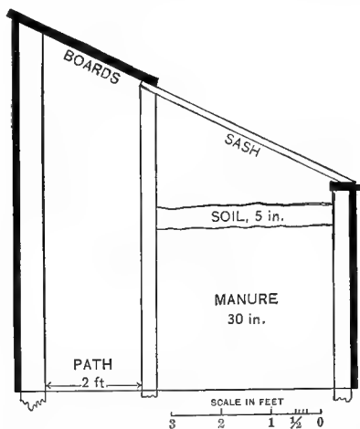
FIG. 104.—Permanent, lean-to hot-bed. (After Green.)
