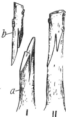
FIG. 95.—Diagram illustrating mode of tongue-grafting. I. Stock a and scion b separate. II. The same fitted together before being bound and waxed.
