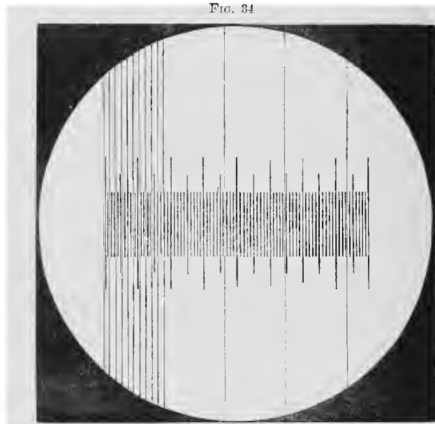
Lines of stage micrometer viewed with an ocular micrometer
