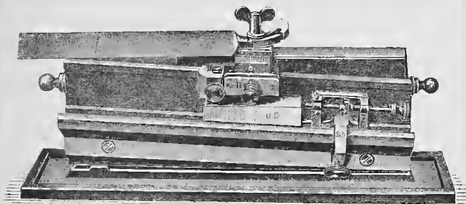
Inclined plane microtome
